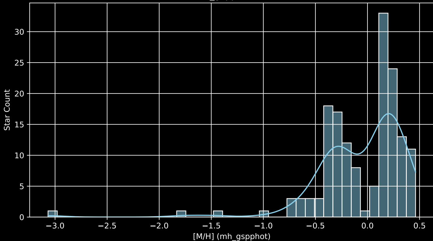
Gaia Cluster: [Platais_8 [M/H] (mh_gspphot) (n= 158)
