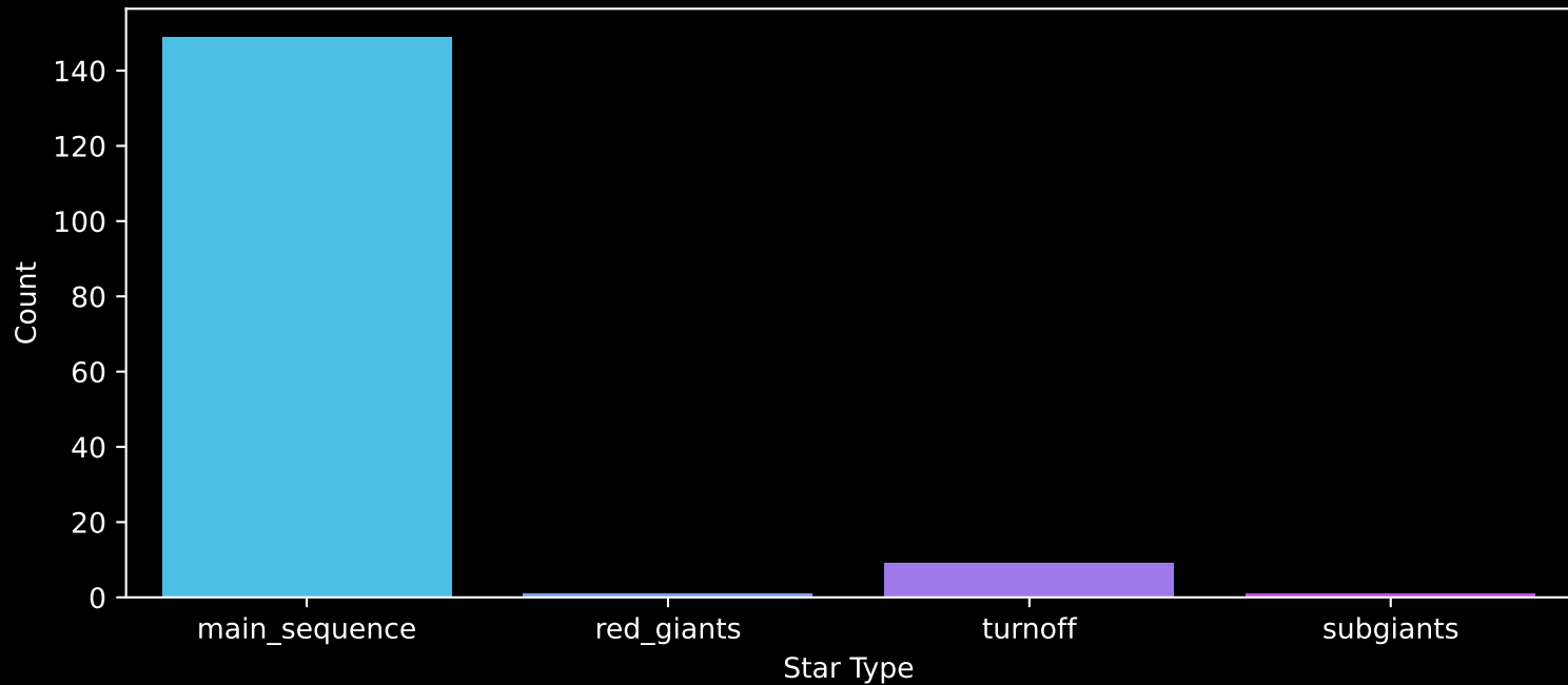
Gaia Cluster: [Platais_8] Count plot of Star Type
