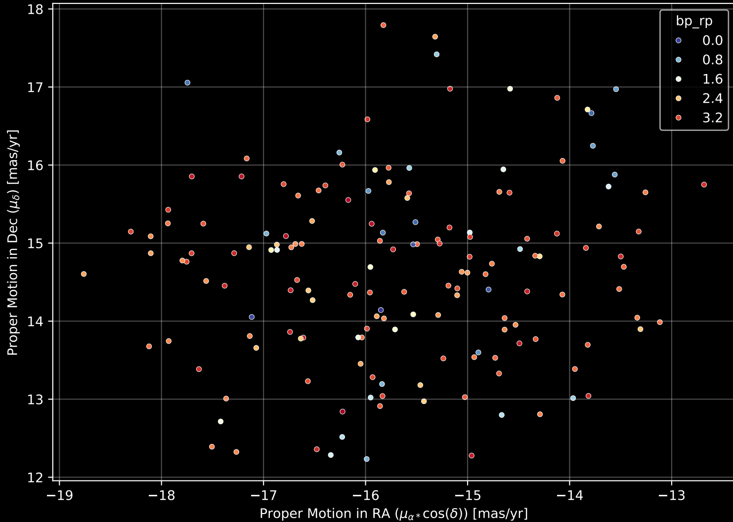
Gaia Cluster: [Platais_8] Proper Motion Diagram (n= 160)
