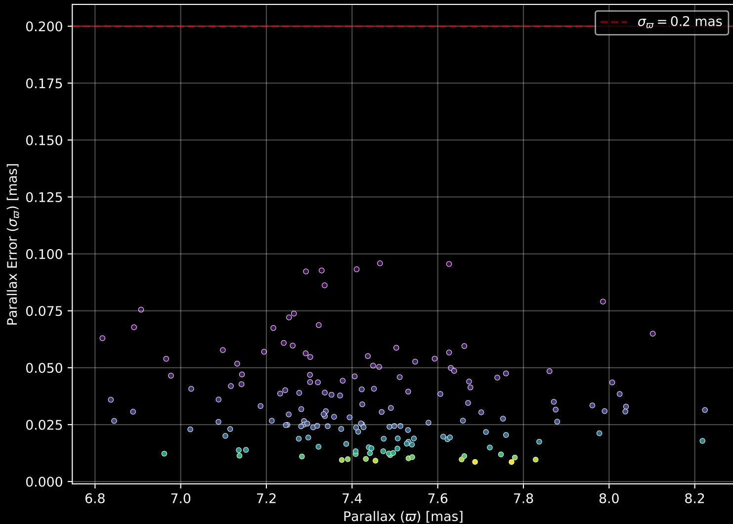
Gaia Cluster: [Platais_8] Parallax Quality (n= 160)
