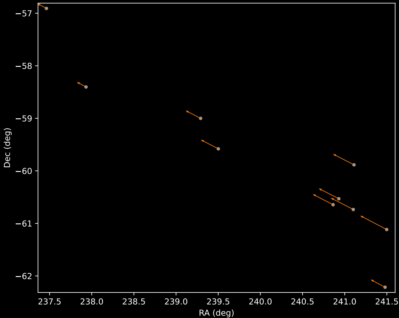
Gaia DR3 Cluster 2 Proper Motion Vectors (n=10)
