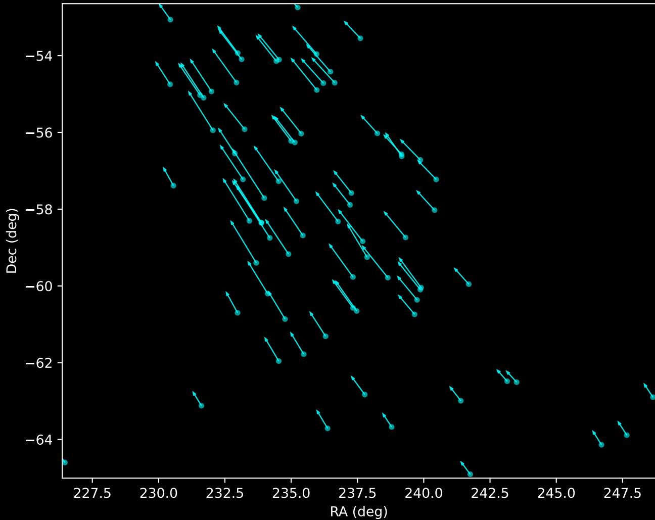
Gaia DR3 Noise Stream Proper Motion Vectors (n=74)
