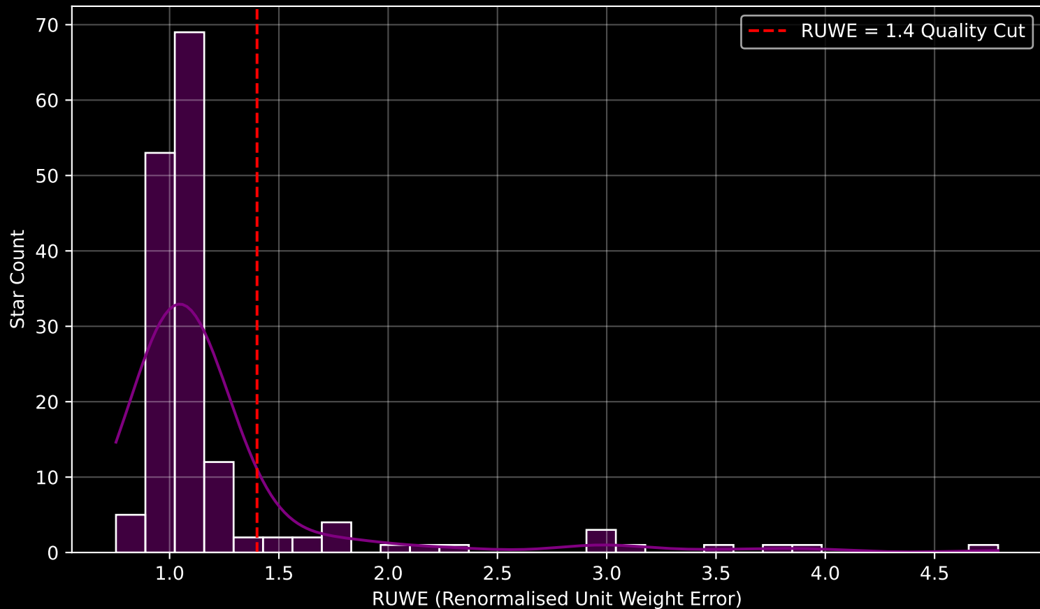
Gaia Cluster: [Platais_8] RUWE Distribution (n= 160)
