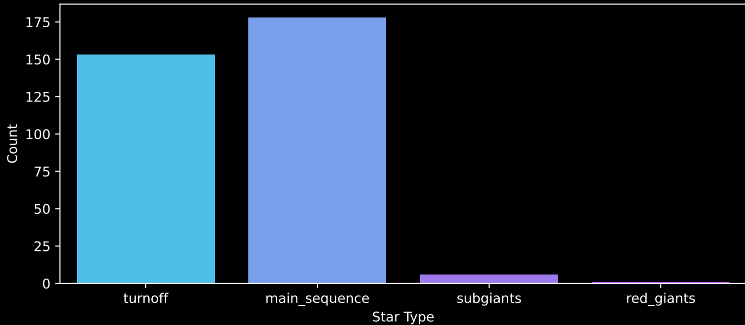
Gaia Cluster: [Pozzo_1] Count plot of Star Type
