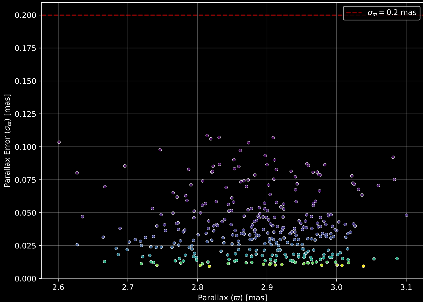
Gaia Cluster: [Pozzo_1] Parallax Quality (n= 338)
