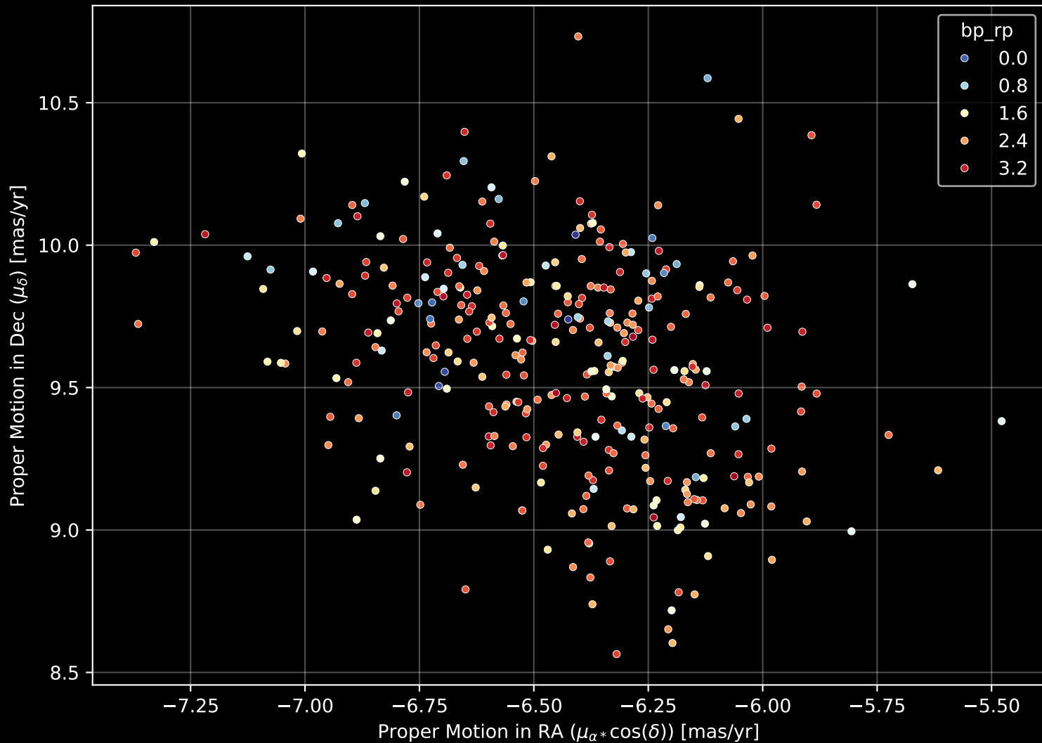
Gaia Cluster: [Pozzo_1] Proper Motion Diagram (n= 338)
