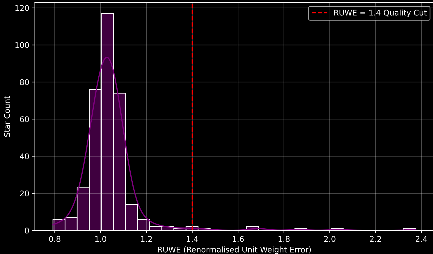
Gaia Cluster: [Pozzo_1] RUWE Distribution (n= 336)
