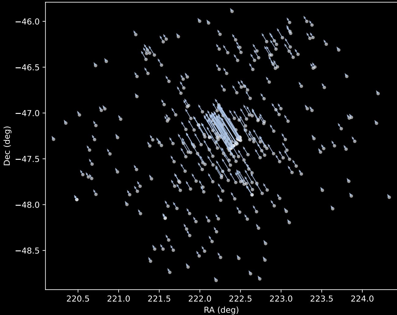
Gaia DR3 Cluster 1 Proper Motion Vectors (n=307)
