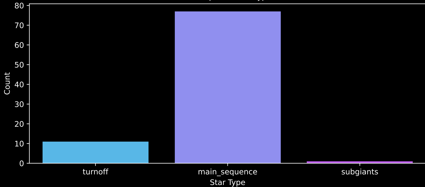
Gaia Cluster: [RSG_1] Count plot of Star Type
