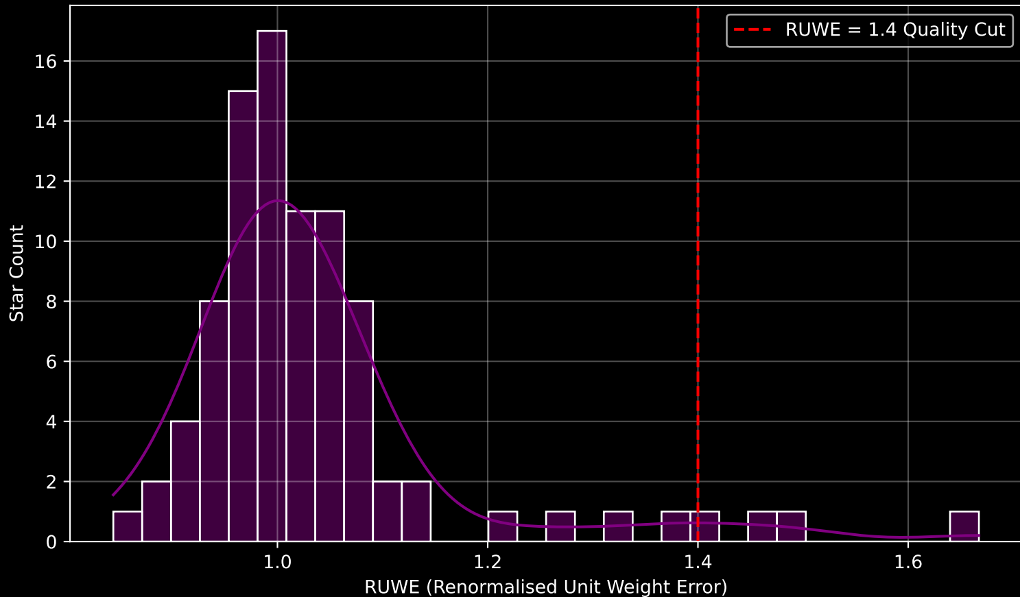
Gaia Cluster: [RSG_1] RUWE Distribution (n= 89)
