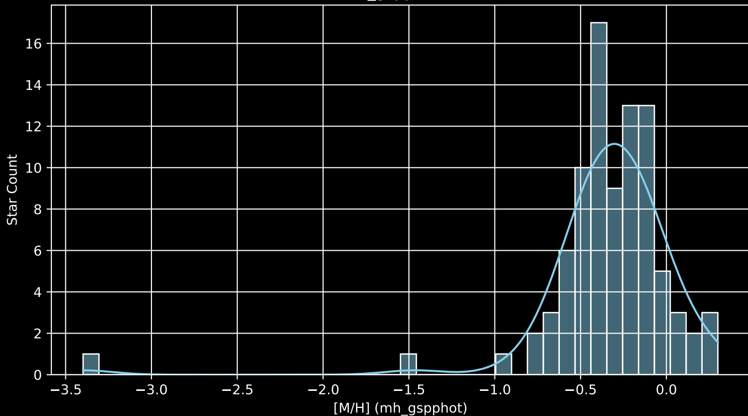
Gaia Cluster: [RSG_1 [M/H] (mh_gspphot) (n= 89)
