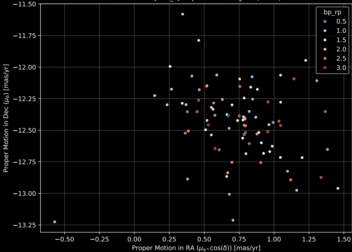
Gaia Cluster: [RSG_1] Proper Motion Diagram (n= 89)
