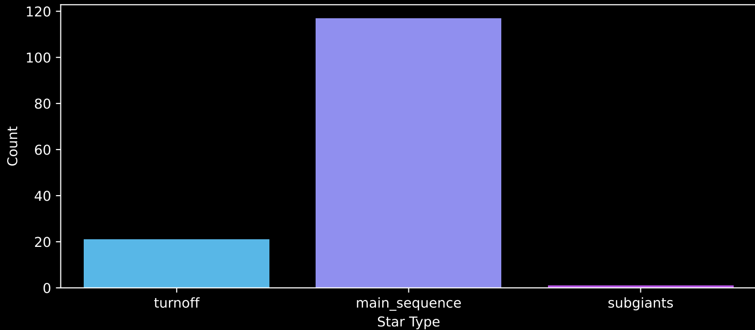
Gaia Cluster: [RSG_5] Count plot of Star Type
