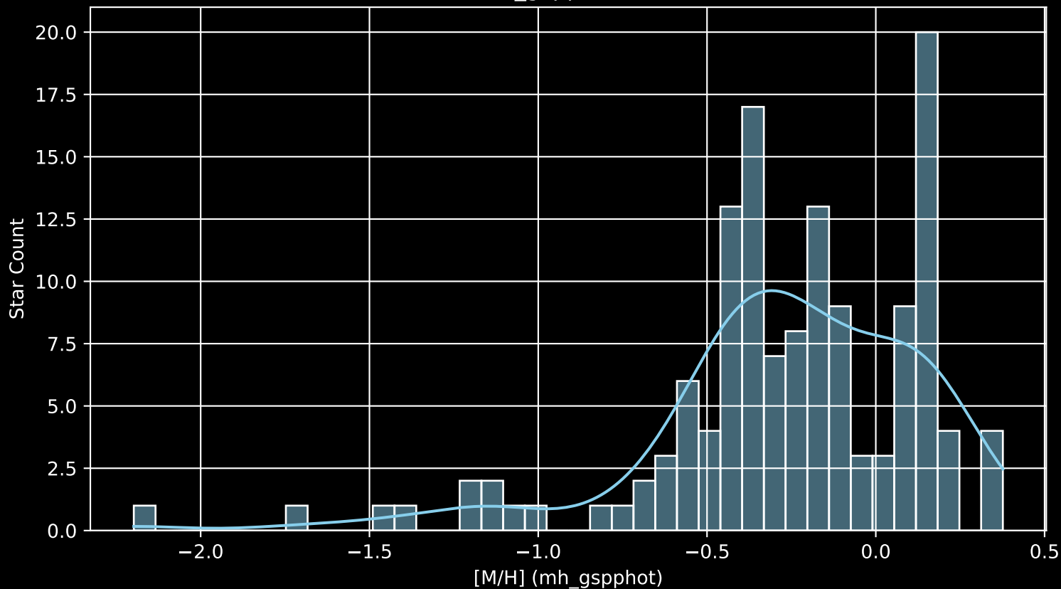
Gaia Cluster: [RSG_5 [M/H] (mh_gspphot) (n= 137)
