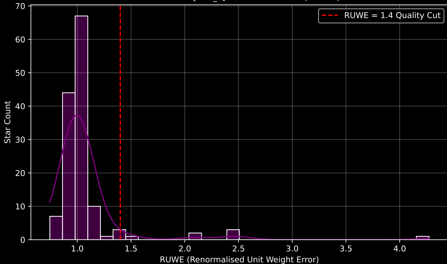
Gaia Cluster: [RSG_5] RUWE Distribution (n= 139)
