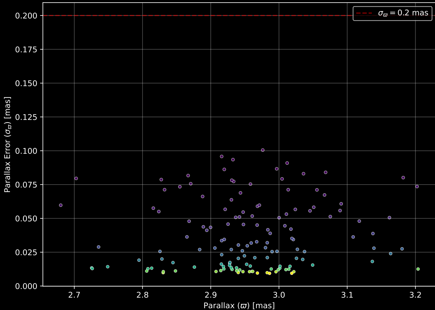
Gaia Cluster: [RSG_5] Parallax Quality (n= 139)
