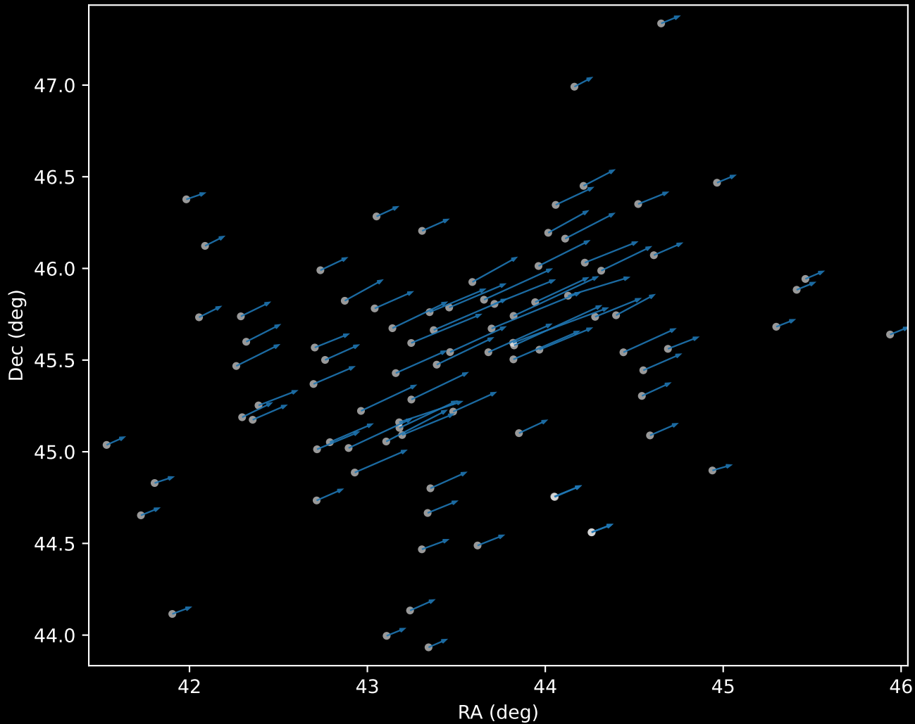
Gaia DR3 Cluster 0 Proper Motion Vectors (n=89)
