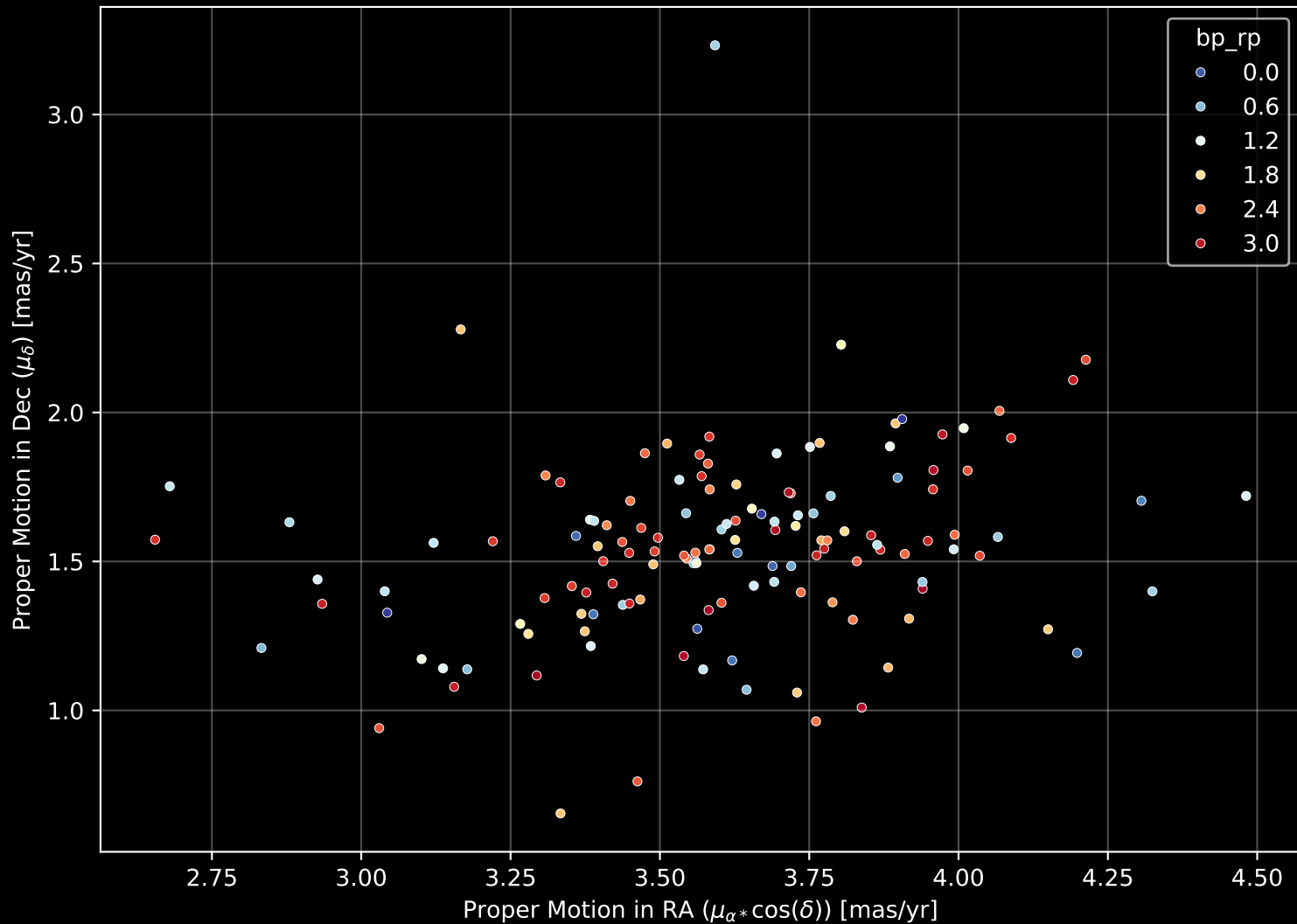
Gaia Cluster: [RSG_5] Proper Motion Diagram (n= 139)
