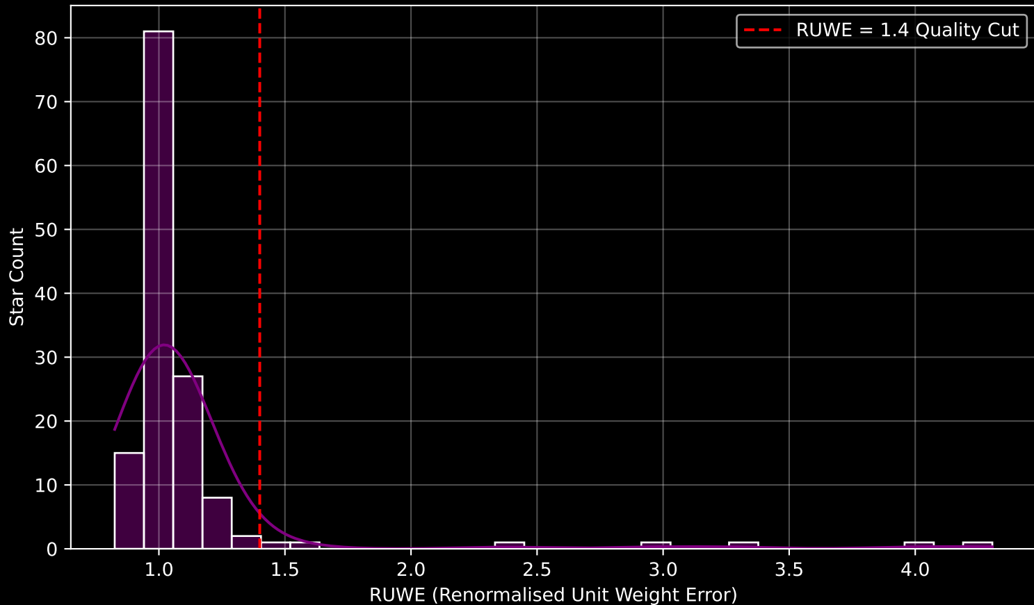
Gaia Cluster: [RSG_7] RUWE Distribution (n= 140)
