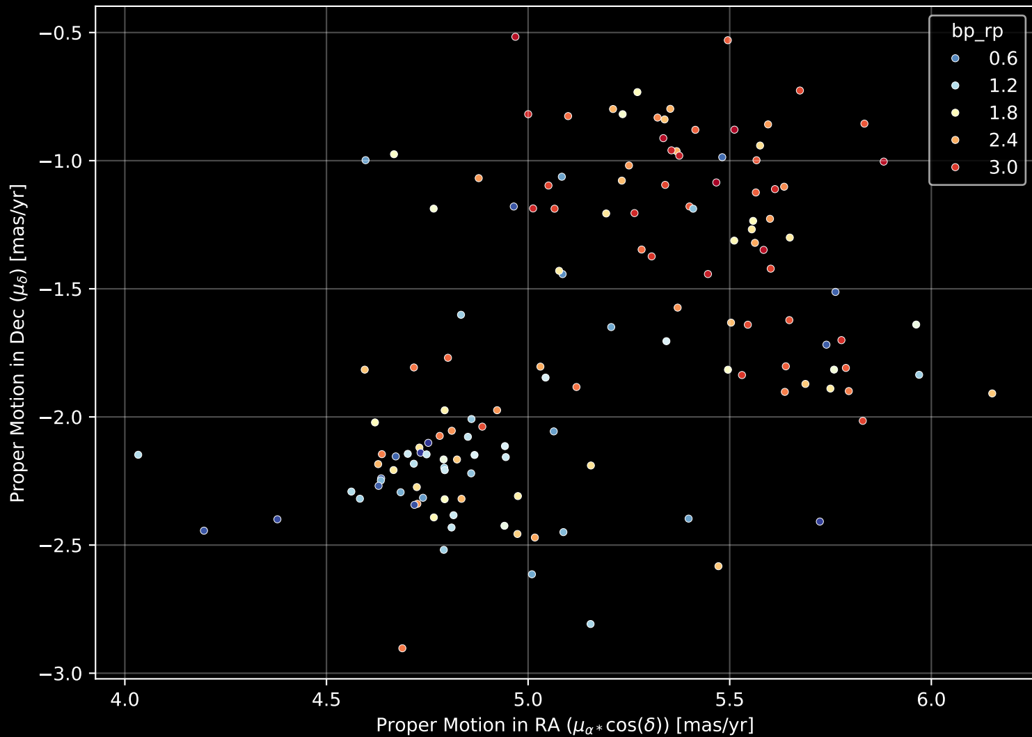
Gaia Cluster: [RSG_7] Proper Motion Diagram (n= 143)
