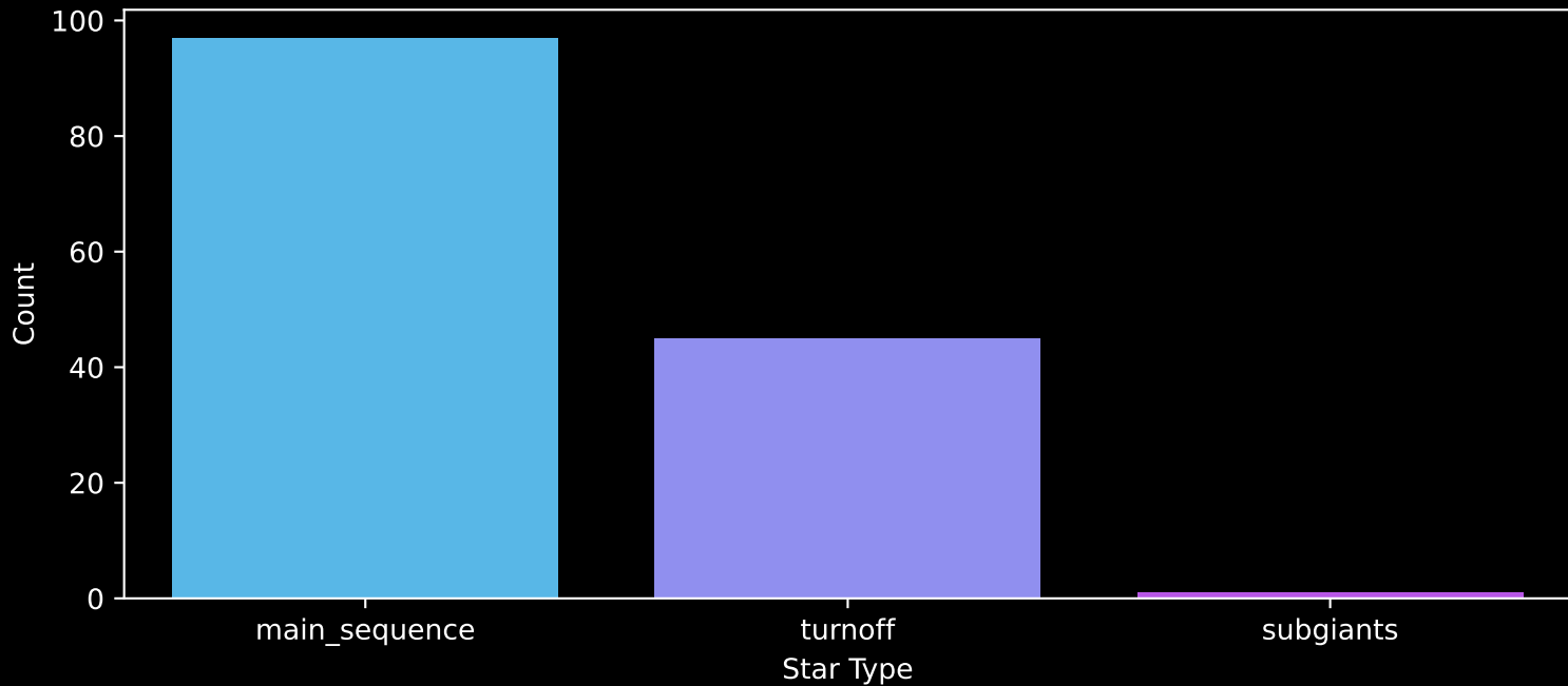
Gaia Cluster: [RSG_7] Count plot of Star Type
