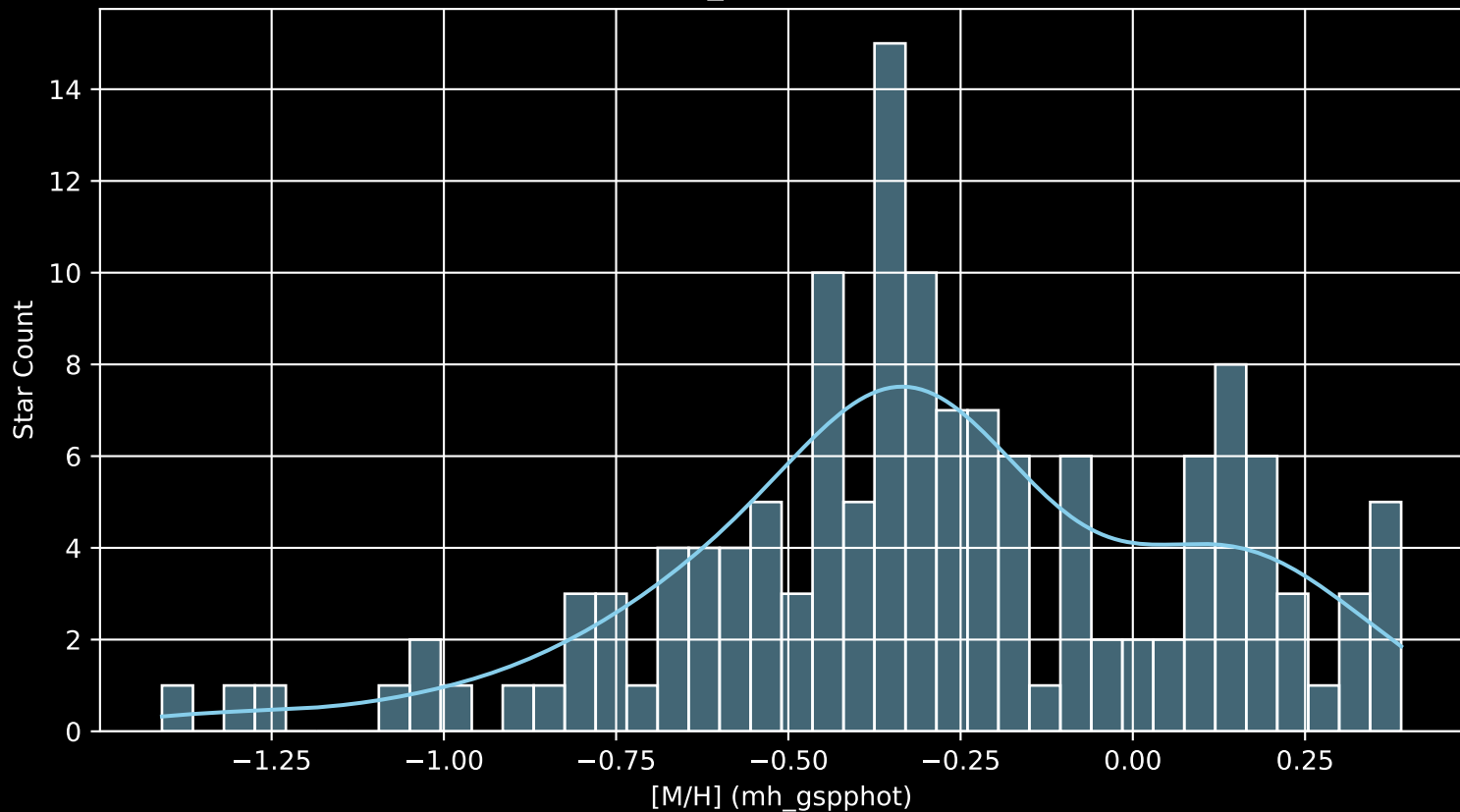
Gaia Cluster: [RSG_7 [M/H] (mh_gspphot) (n= 141)
