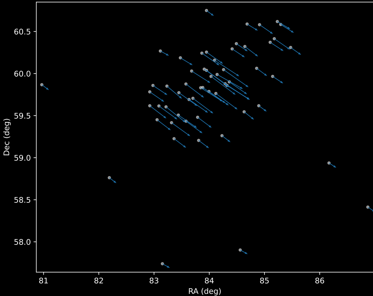
Gaia DR3 Cluster 0 Proper Motion Vectors (n=57)
