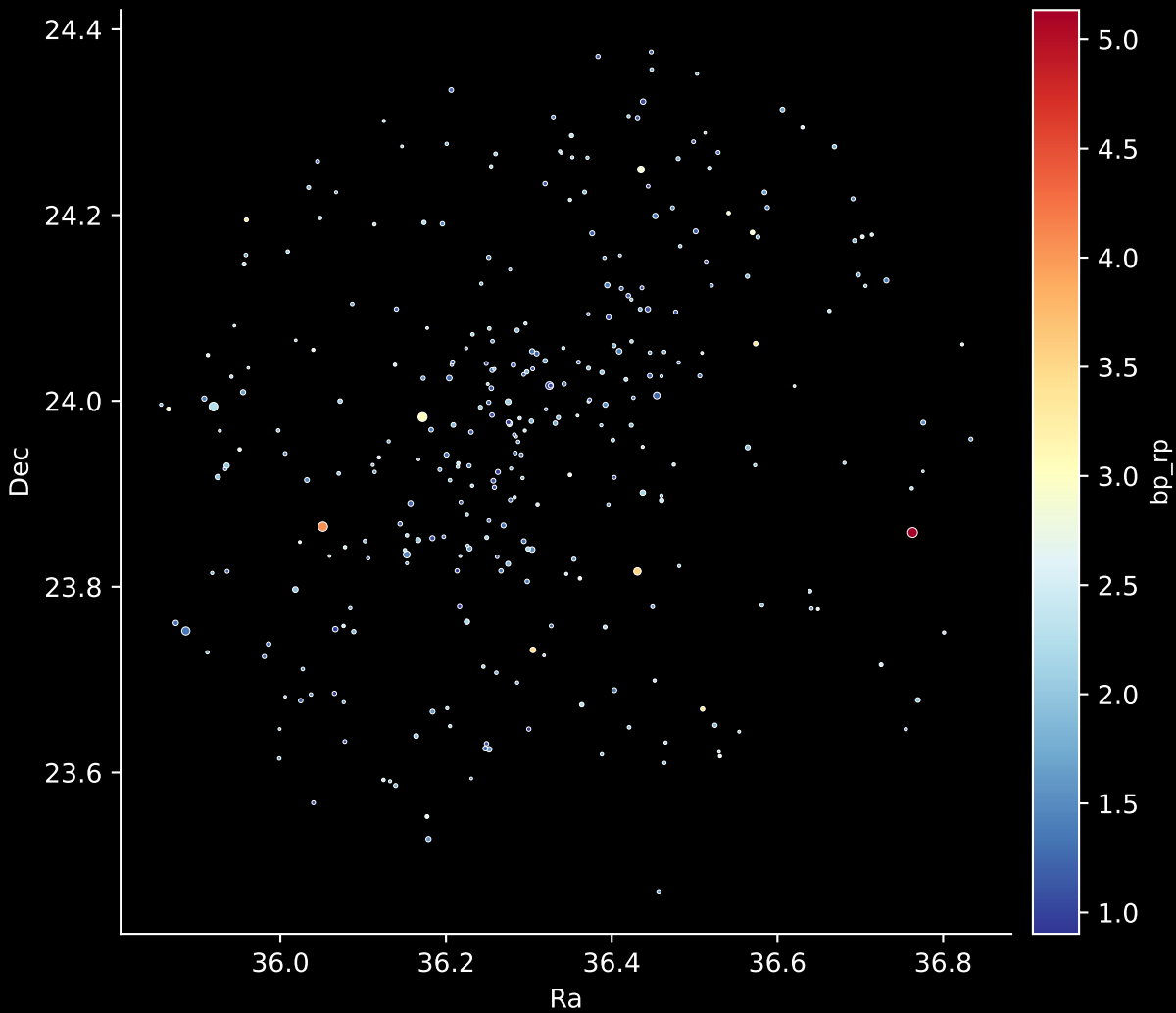
Gaia Cluster: [Roslund_2] Stars: 317
