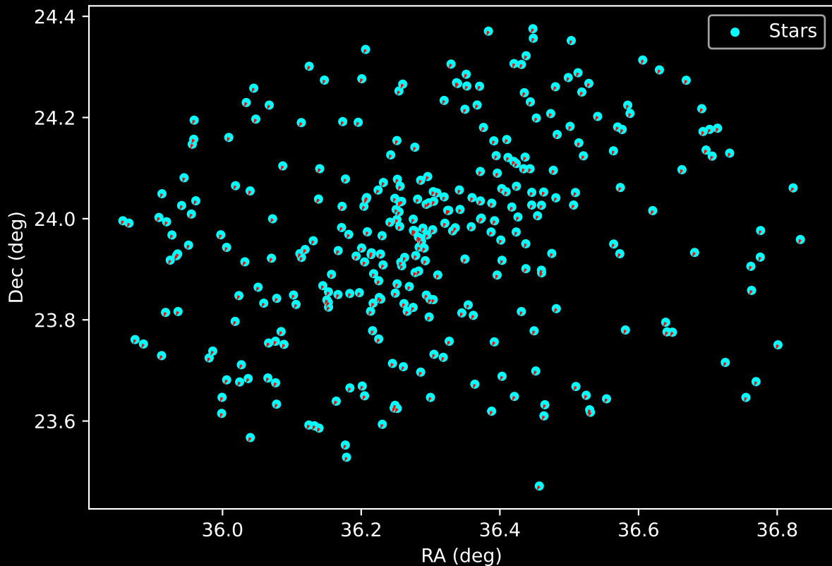
Gaia Cluster: [Roslund_2] Proper Motion Vectors for Gaia Star Field (n= 317)
