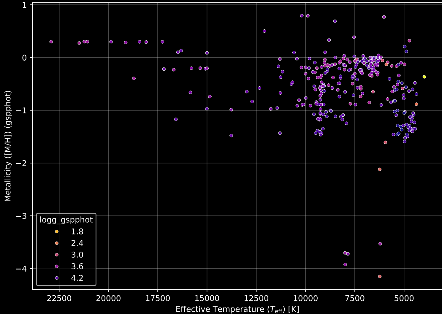
Gaia Cluster: [Roslund_2] Stellar Population Parameters (n= 317)
