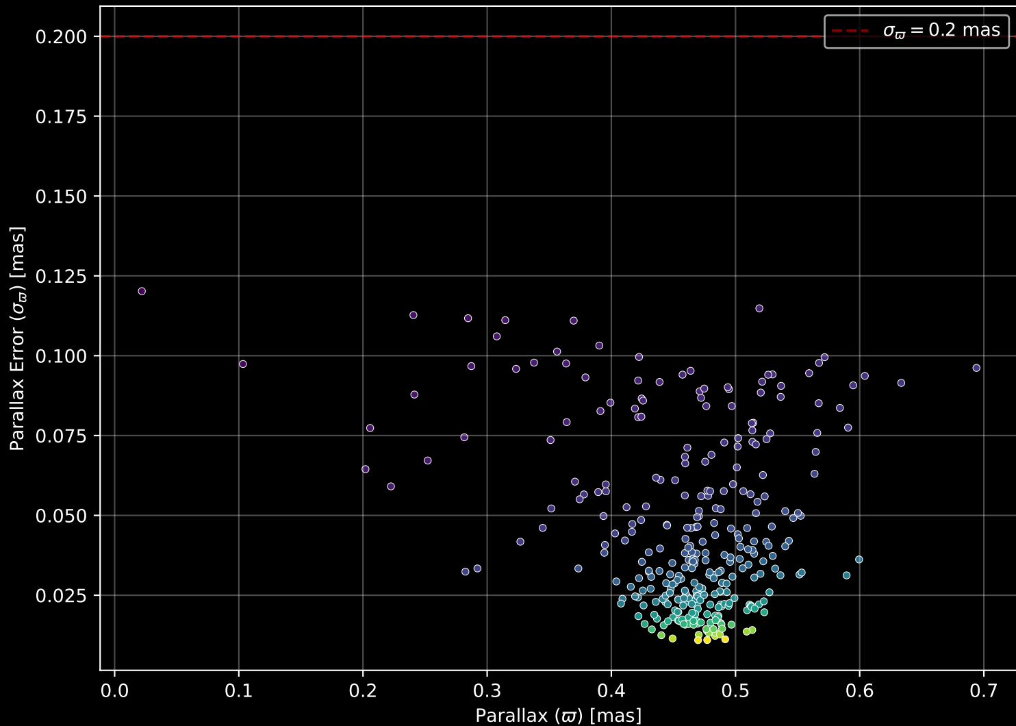
Gaia Cluster: [Roslund_2] Parallax Quality (n= 317)
