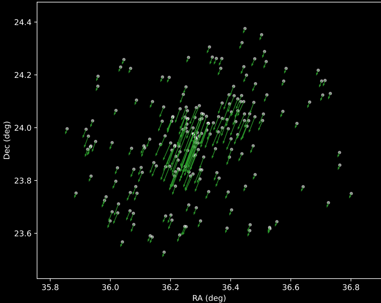
Gaia DR3 Cluster 4 Proper Motion Vectors (n=207)
