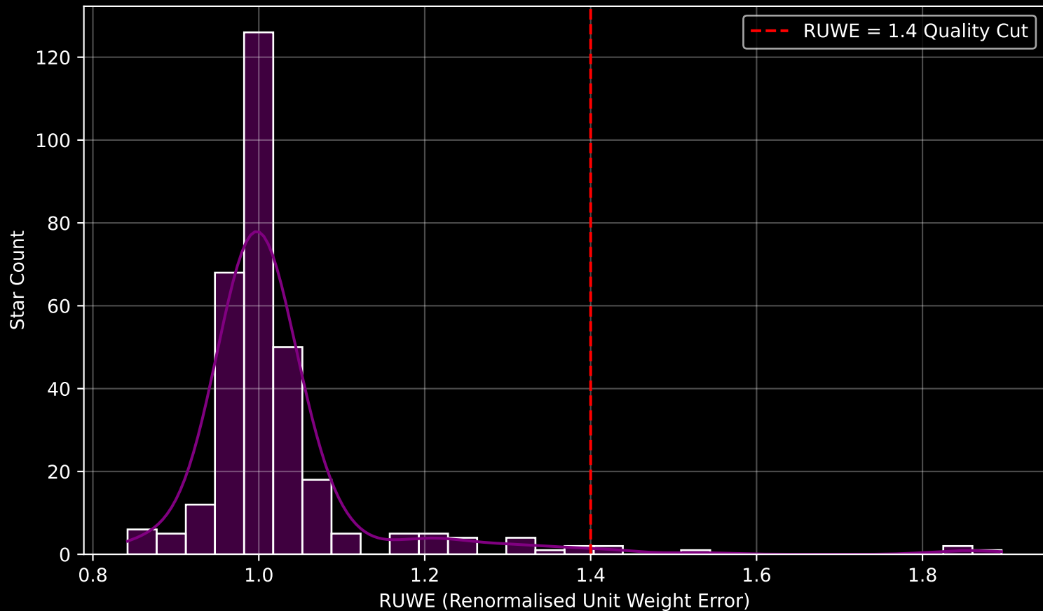
Gaia Cluster: [Roslund_2] RUWE Distribution (n= 317)
