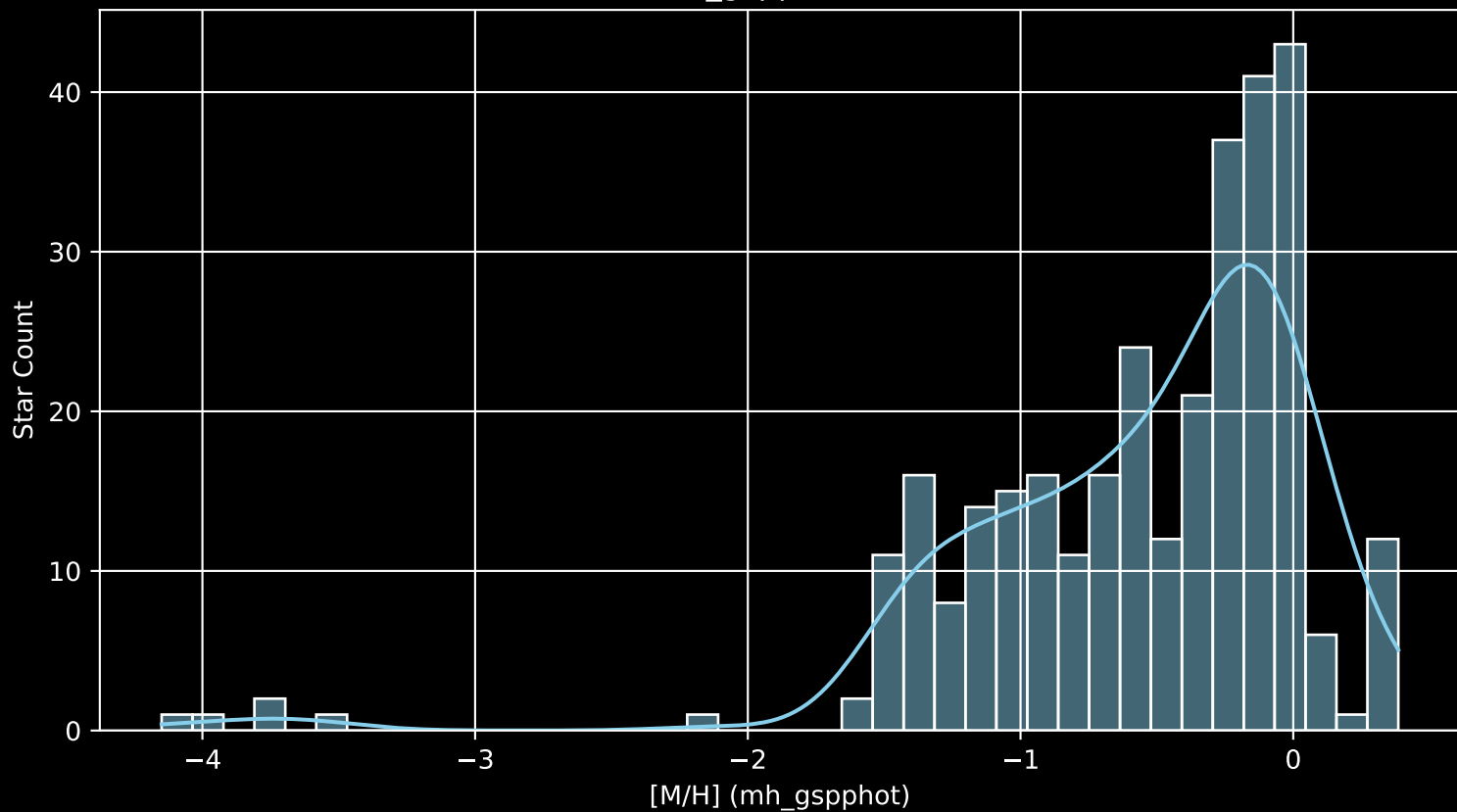
Gaia Cluster: [Roslund_2 [M/H] (mh_gspphot) (n= 312)
