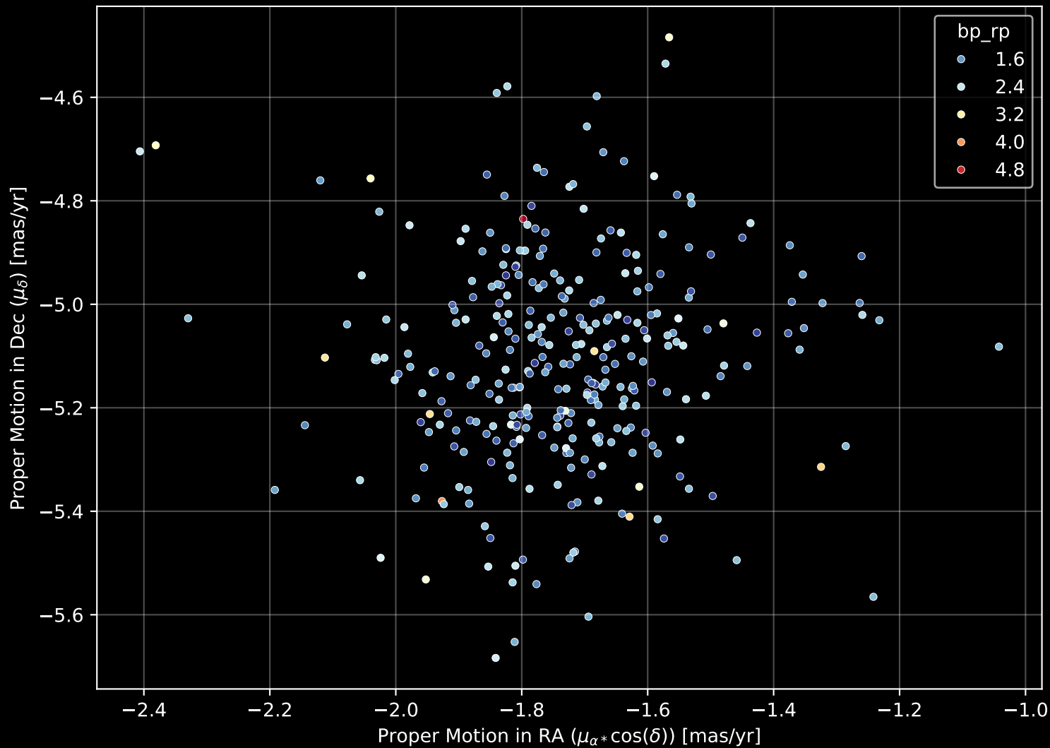
Gaia Cluster: [Roslund_2] Proper Motion Diagram (n= 317)
