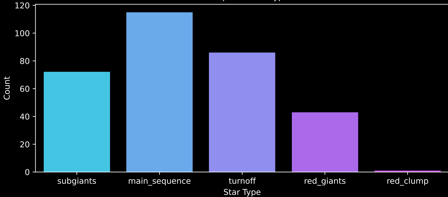
Gaia Cluster: [Roslund_2] Count plot of Star Type
