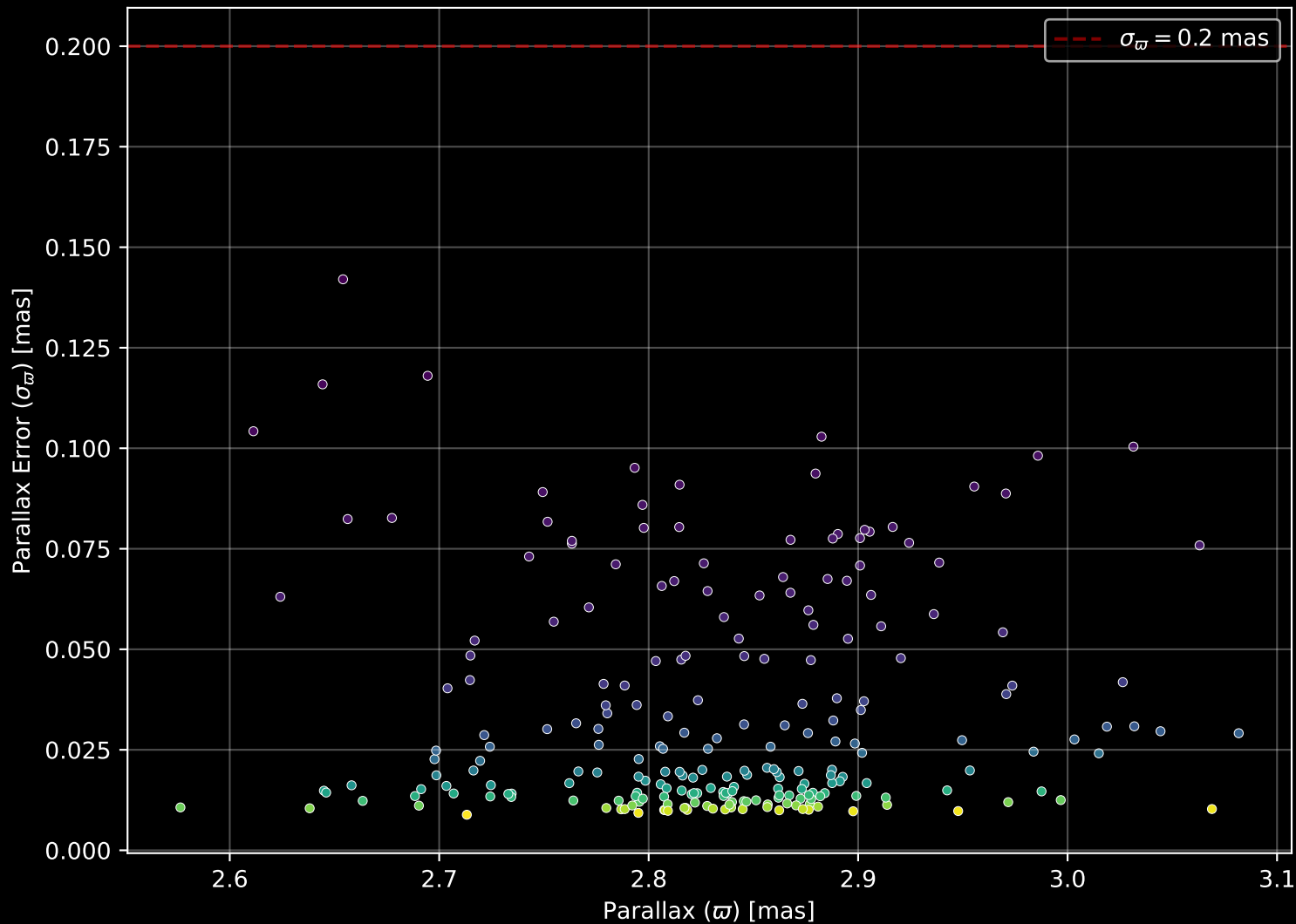
Gaia Cluster: [Roslund_6] Parallax Quality (n= 229)
