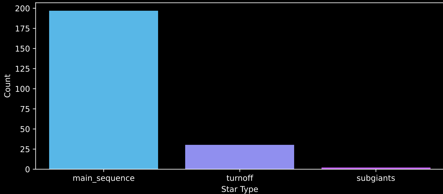
Gaia Cluster: [Roslund_6] Count plot of Star Type
