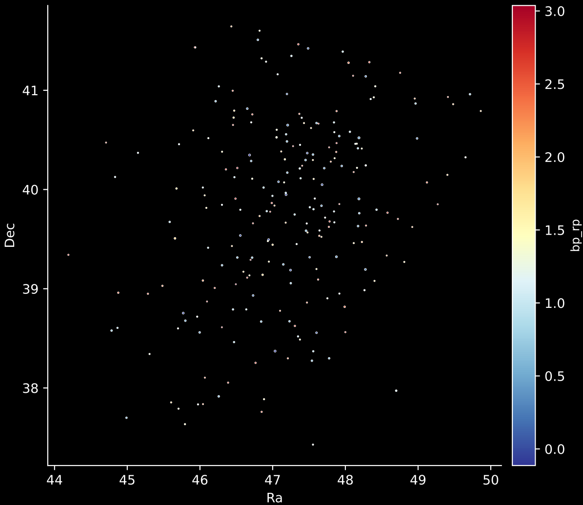
Gaia Cluster: [Roslund_6] Stars: 229
