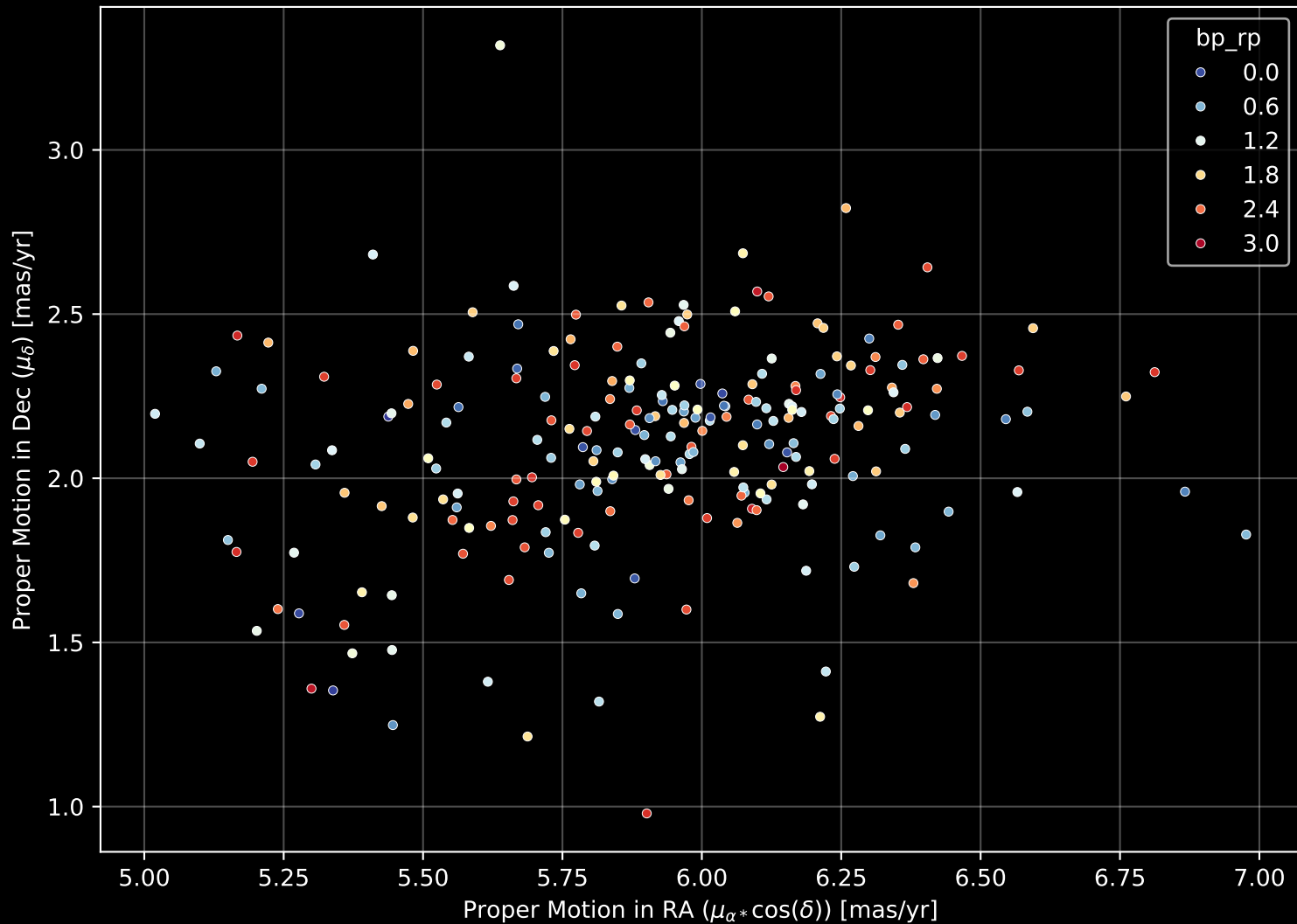
Gaia Cluster: [Roslund_6] Proper Motion Diagram (n= 229)
