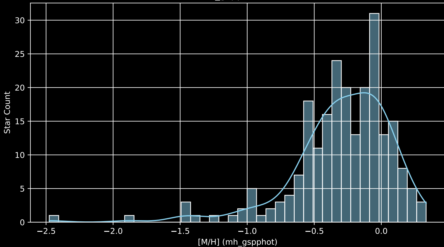
Gaia Cluster: [Roslund_6 [M/H] (mh_gspphot) (n= 229)
