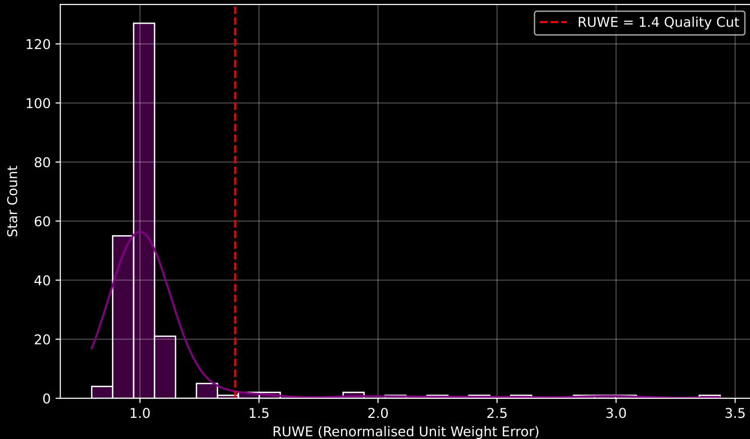
Gaia Cluster: [Roslund_6] RUWE Distribution (n= 227)
