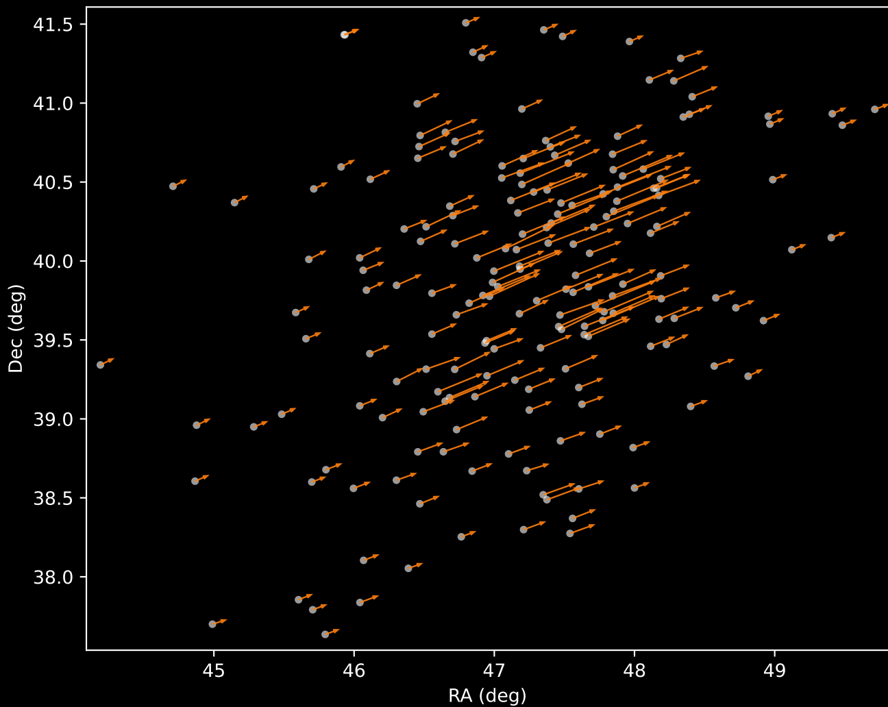
Gaia DR3 Cluster 2 Proper Motion Vectors (n=188)
