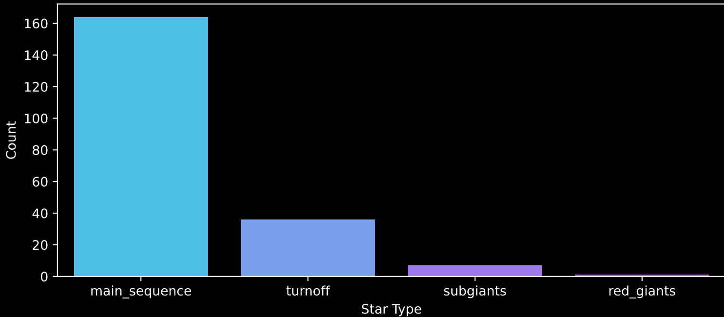
Gaia Cluster: [Roslund_7] Count plot of Star Type
