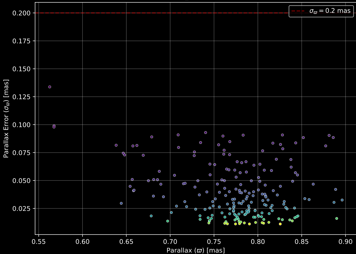
Gaia Cluster: [Roslund_7] Parallax Quality (n= 208)
