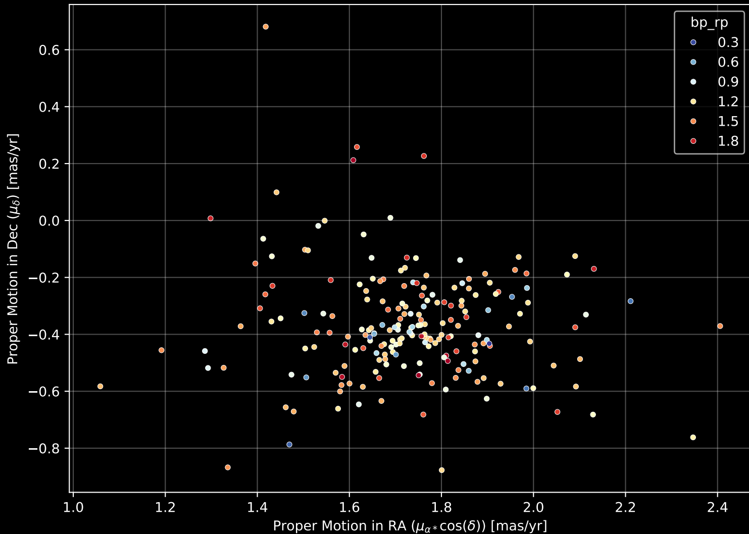
Gaia Cluster: [Roslund_7] Proper Motion Diagram (n= 208)
