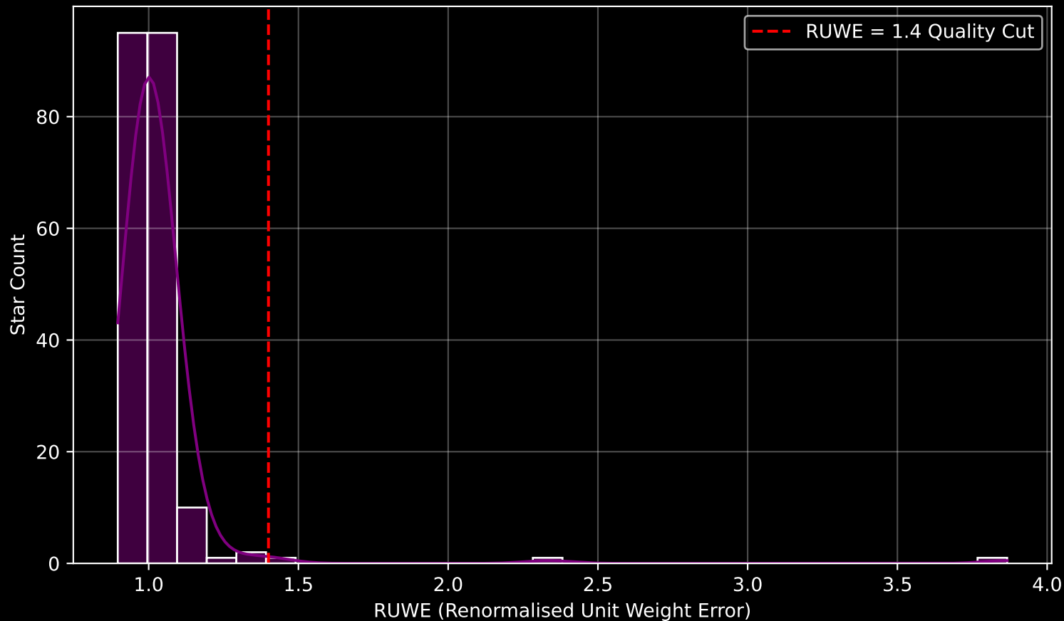
Gaia Cluster: [Roslund_7] RUWE Distribution (n= 206)
