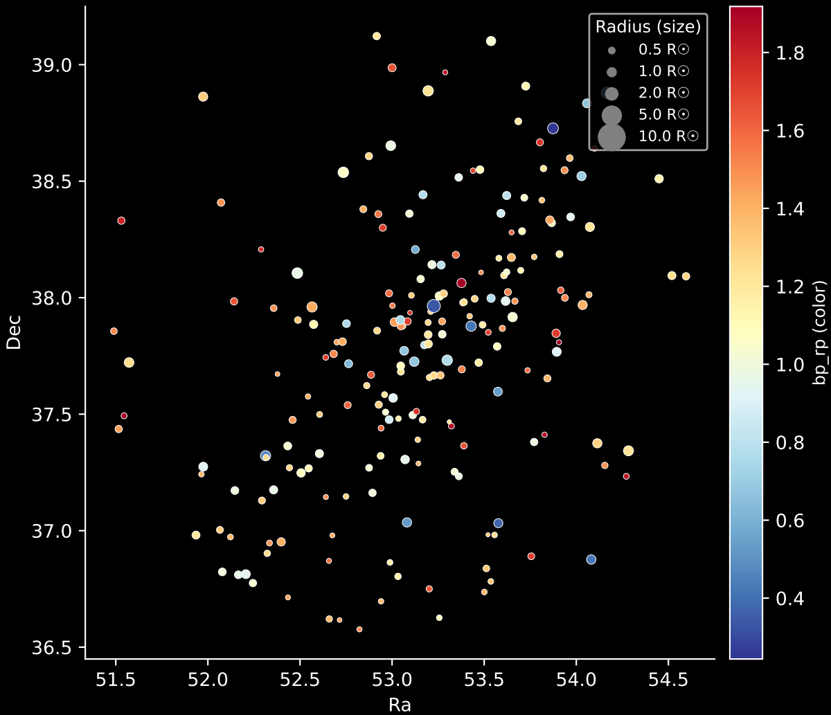
Gaia Cluster: [Roslund_7] Stars: 208
