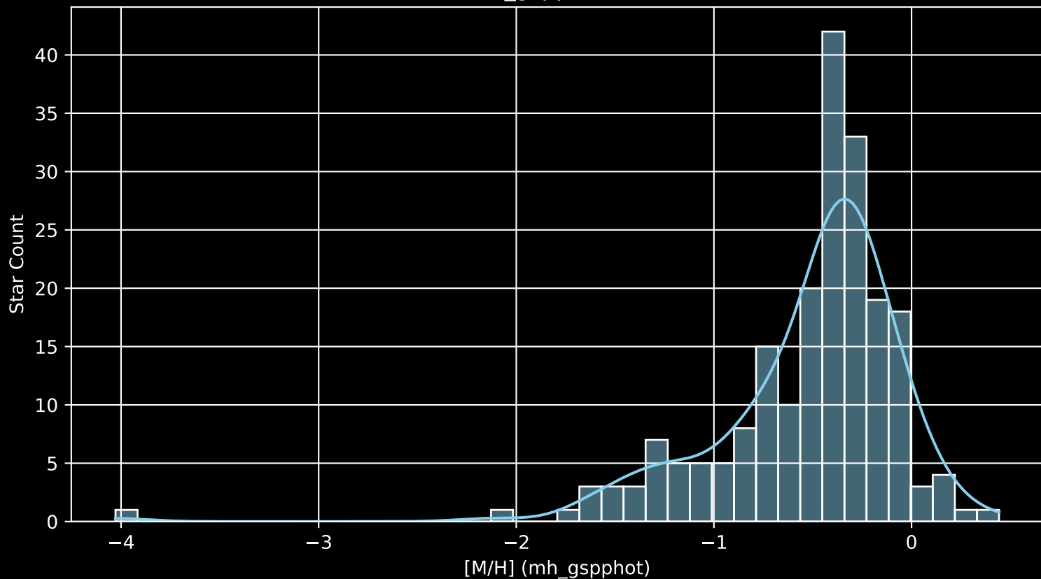
Gaia Cluster: [Roslund_7 [M/H] (mh_gspphot) (n= 208)
