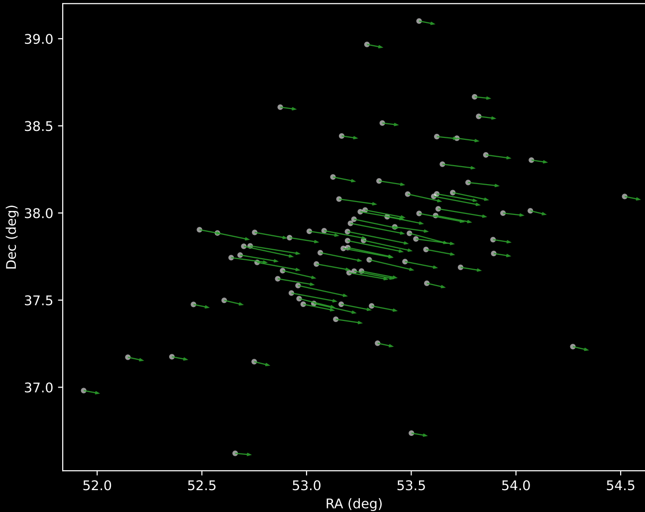
Gaia DR3 Cluster 4 Proper Motion Vectors (n=82)
