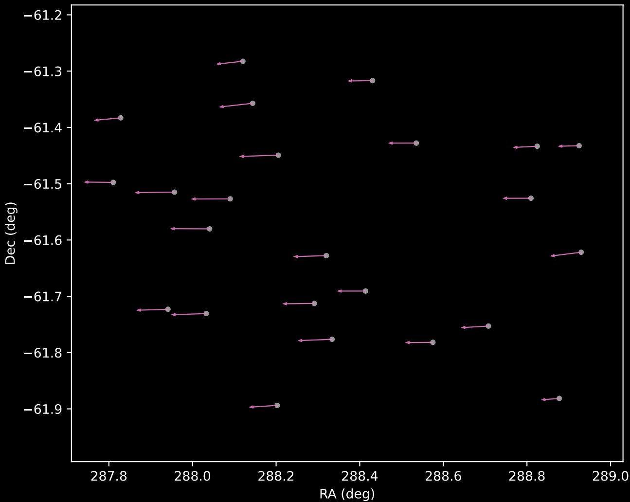
Gaia DR3 Cluster 12 Proper Motion Vectors (n=24)
