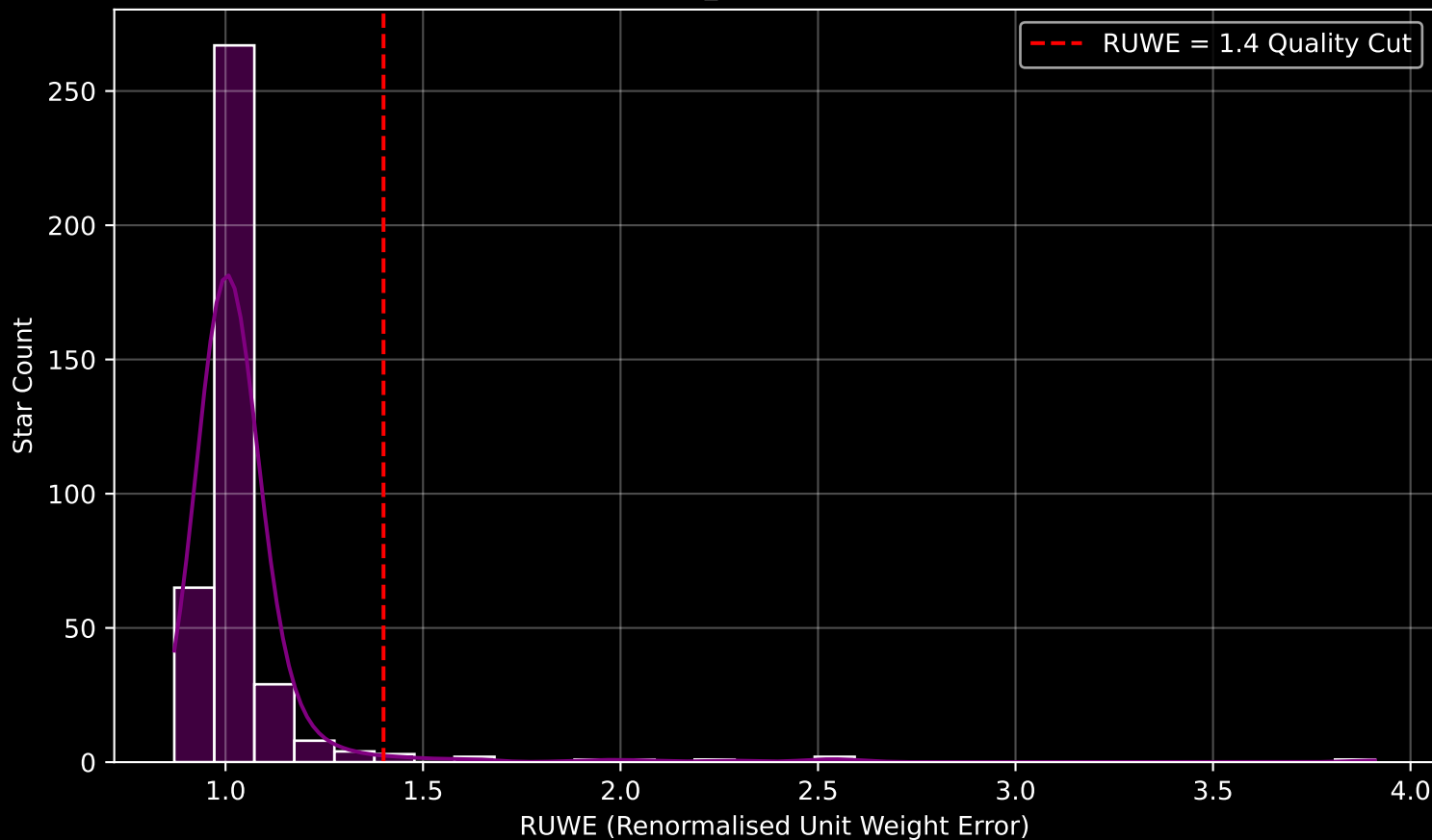
Gaia Cluster: [Ruprecht_105] RUWE Distribution (n= 384)
