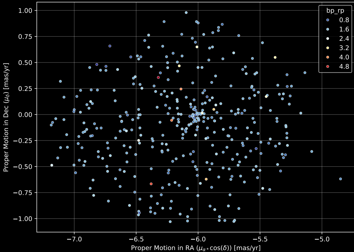
Gaia Cluster: [Ruprecht_105] Proper Motion Diagram (n= 385)
