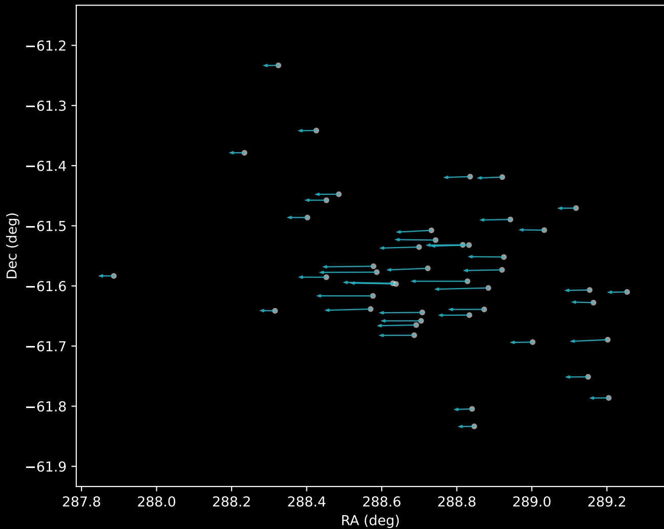
Gaia DR3 Cluster 18 Proper Motion Vectors (n=45)
