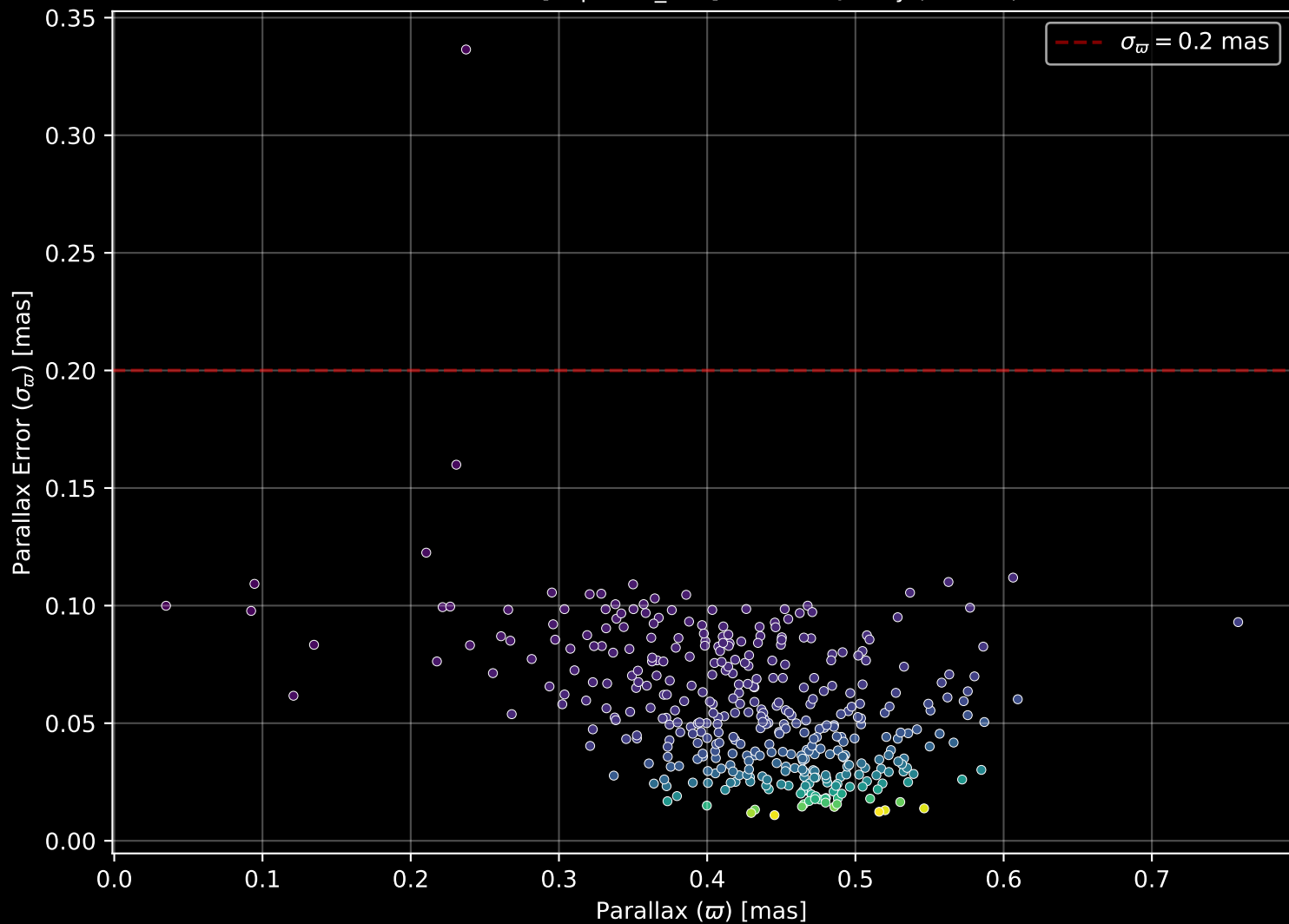
Gaia Cluster: [Ruprecht_105] Parallax Quality (n= 385)
