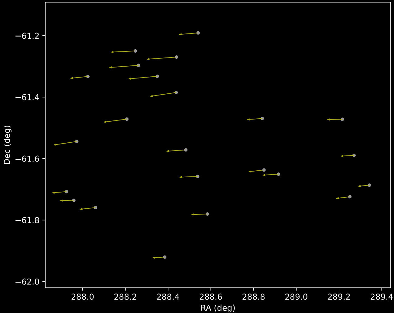
Gaia DR3 Cluster 16 Proper Motion Vectors (n=23)
