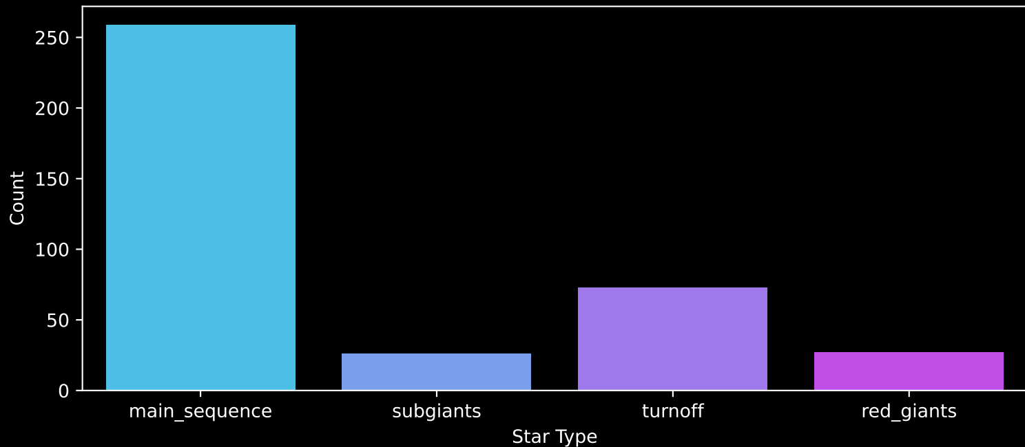
Gaia Cluster: [Ruprecht_105] Count plot of Star Type
