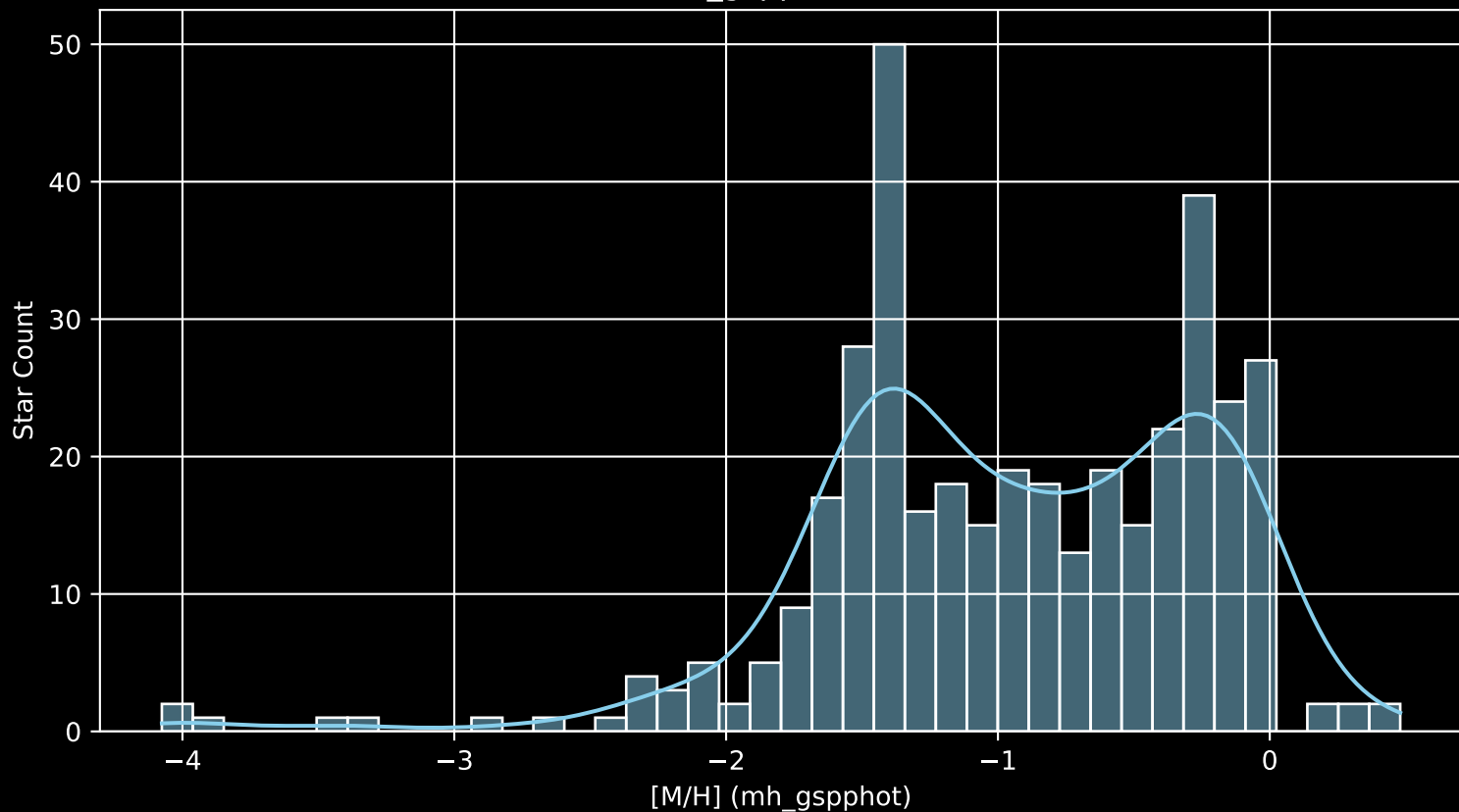
Gaia Cluster: [Ruprecht_105 [M/H] (mh_gspphot) (n= 382)
