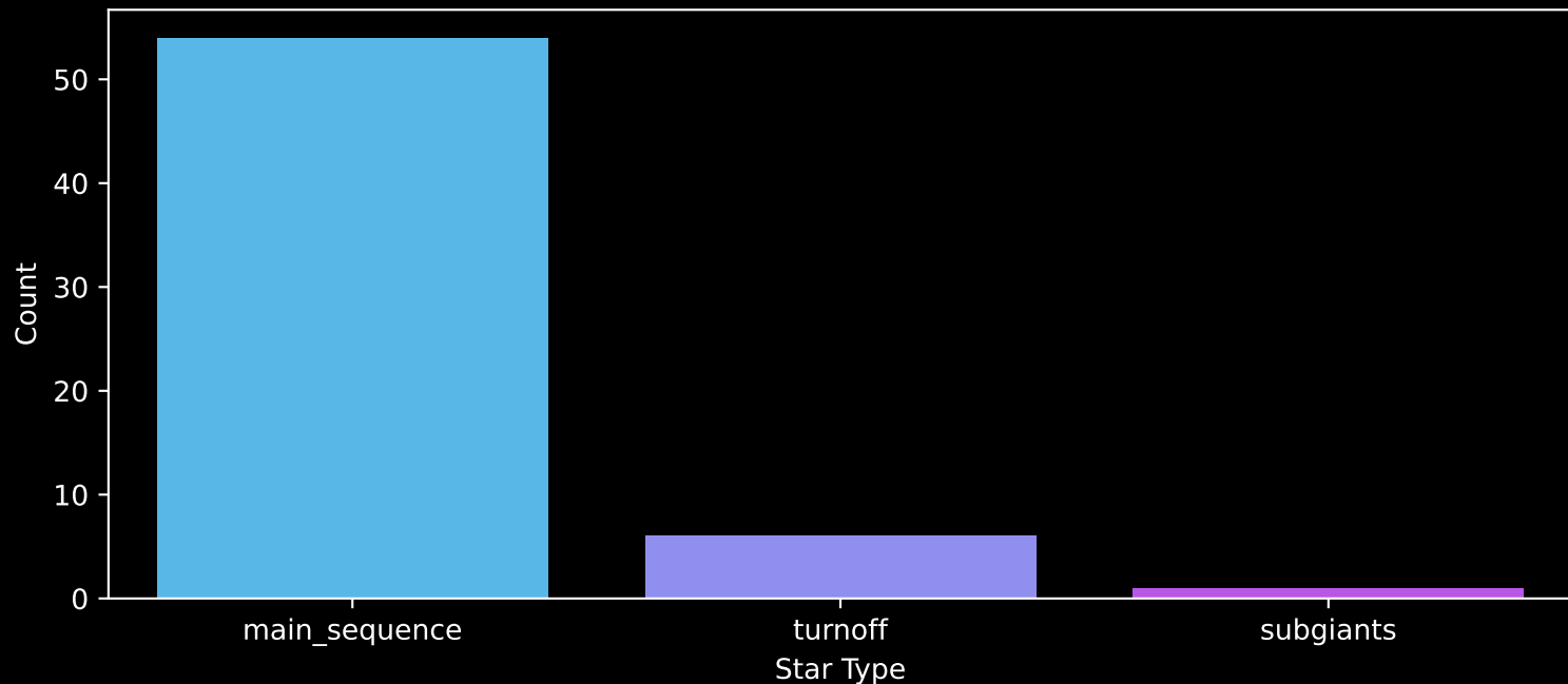
Gaia Cluster: [Ruprecht_108] Count plot of Star Type
