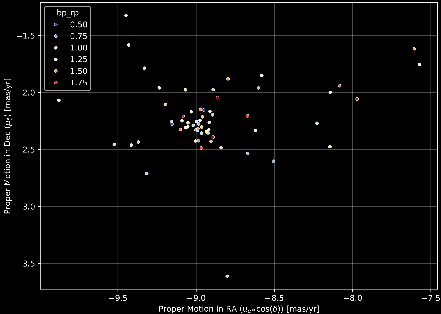
Gaia Cluster: [Ruprecht_108] Proper Motion Diagram (n= 61)
