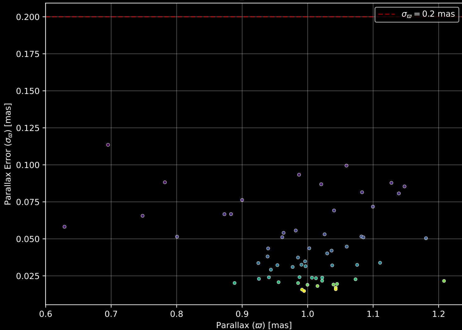
Gaia Cluster: [Ruprecht_108] Parallax Quality (n= 61)
