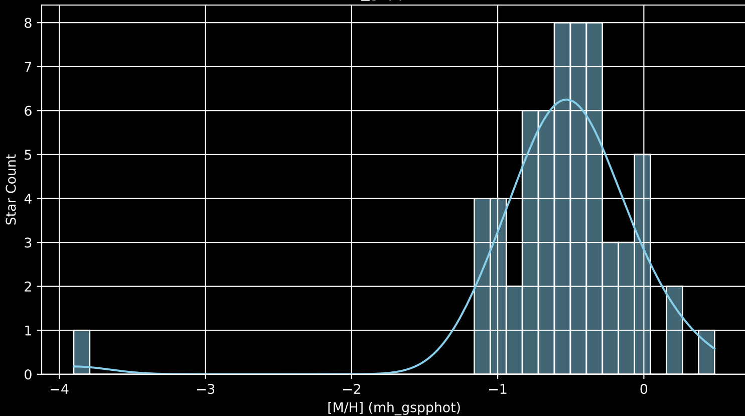
Gaia Cluster: [Ruprecht_108 [M/H] (mh_gspphot) (n= 61)
