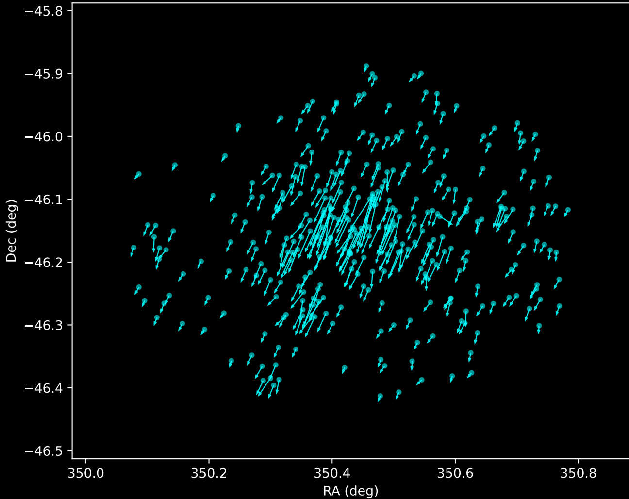
Gaia DR3 Noise Stream Proper Motion Vectors (n=321)
