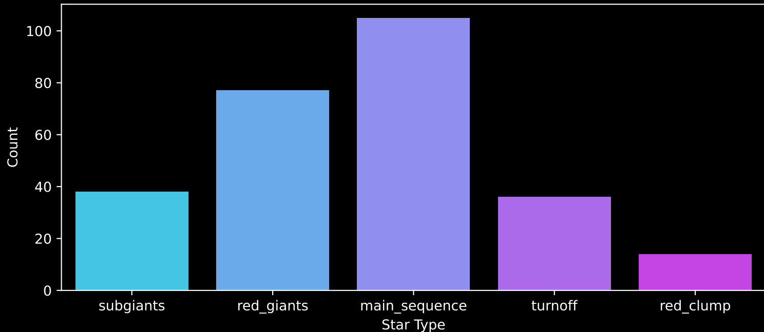
Gaia Cluster: [Ruprecht_126] Count plot of Star Type
