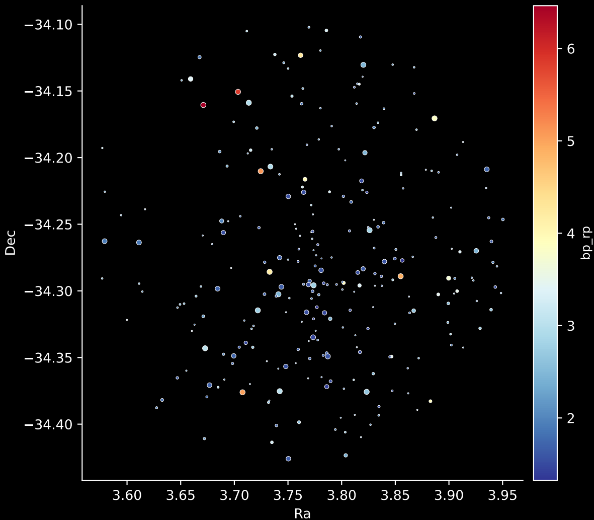
Gaia Cluster: [Ruprecht_126] Stars: 270
