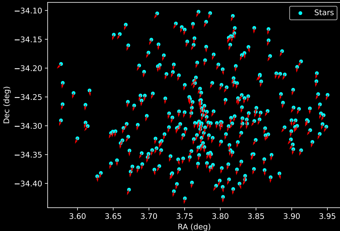
Gaia Cluster: [Ruprecht_126] Proper Motion Vectors for Gaia Star Field (n= 270)
