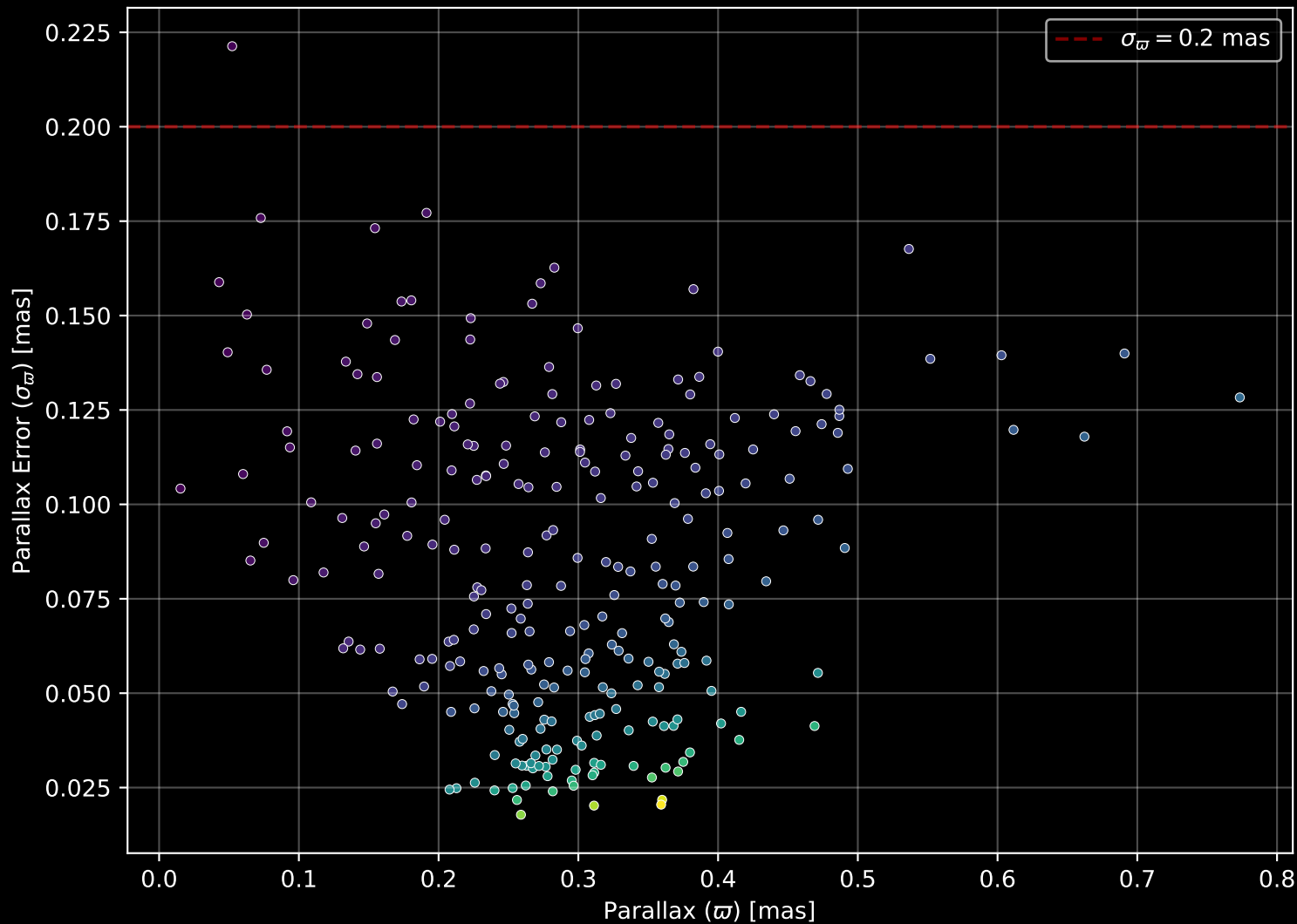
Gaia Cluster: [Ruprecht_126] Parallax Quality (n = 270)
