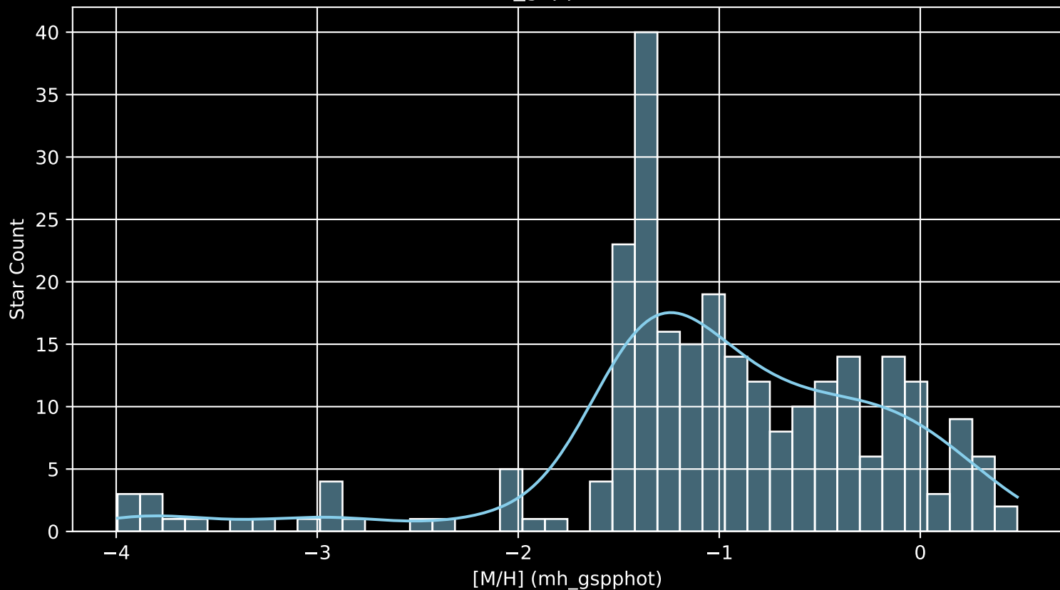
Gaia Cluster: [Ruprecht_126 [M/H] (mh_gspphot) (n= 264)
