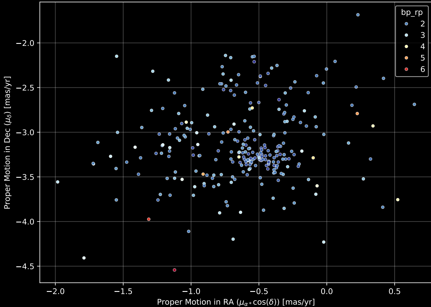
Gaia Cluster: [Ruprecht_126] Proper Motion Diagram (n= 270)
