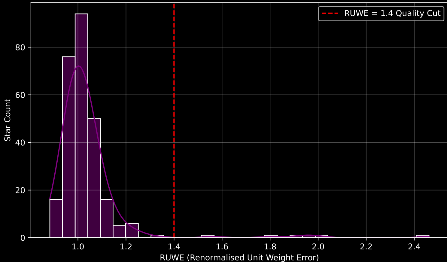
Gaia Cluster: [Ruprecht_126] RUWE Distribution (n= 270)
