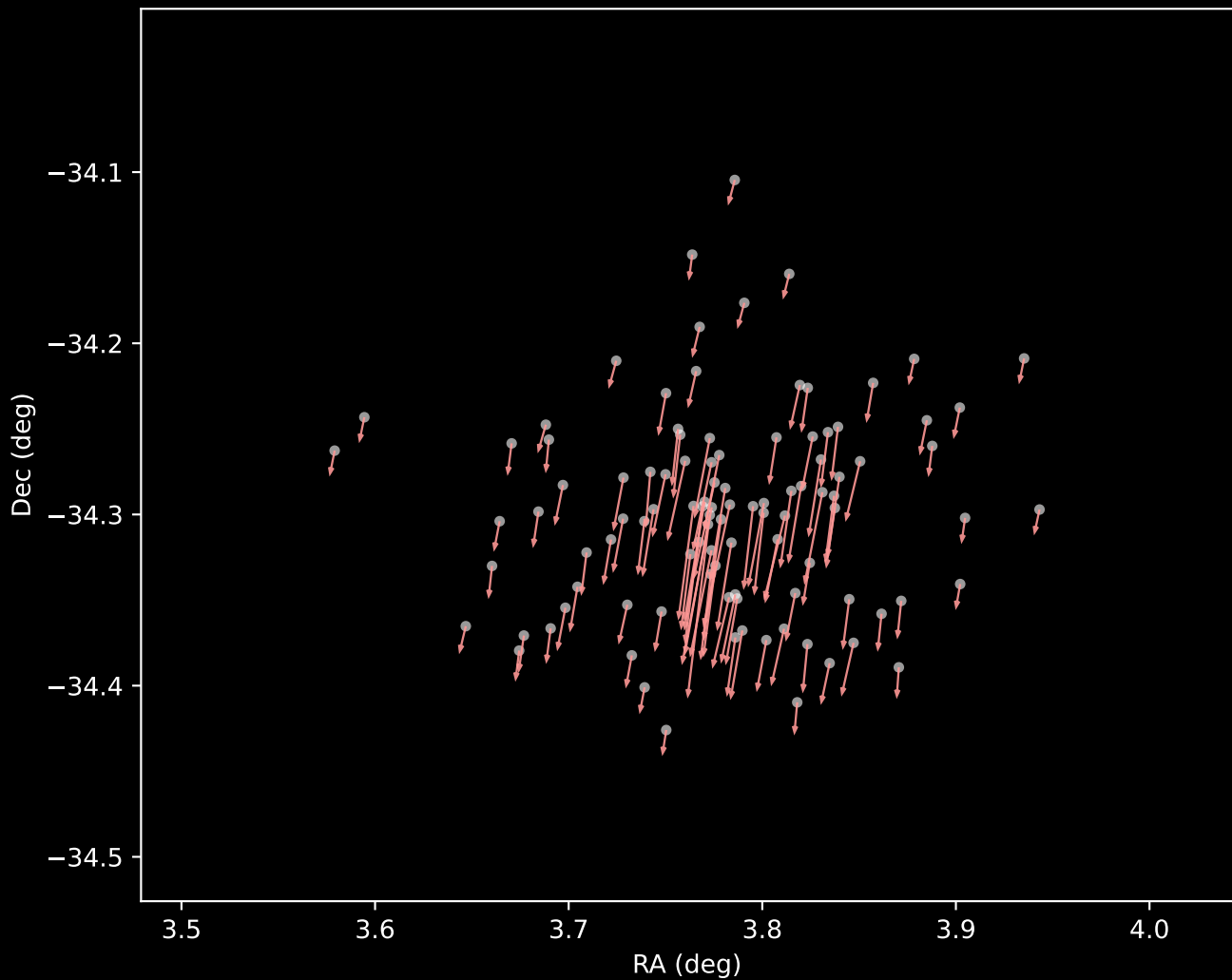
Gaia DR3 Cluster 7 Proper Motion Vectors (n=103)
