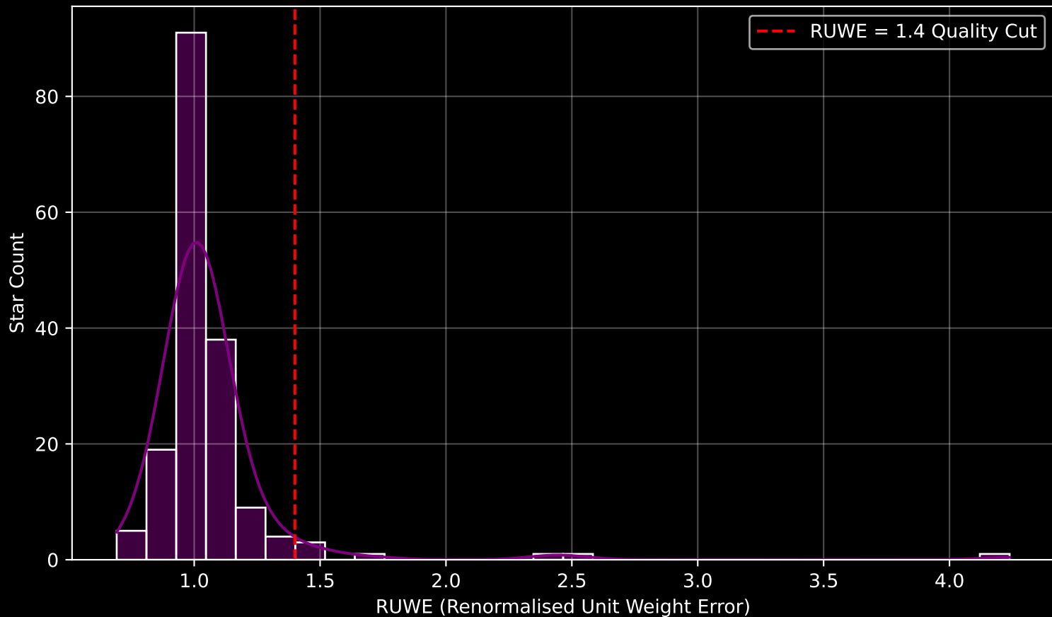
Gaia Cluster: [Ruprecht_127] RUWE Distribution (n= 173)
