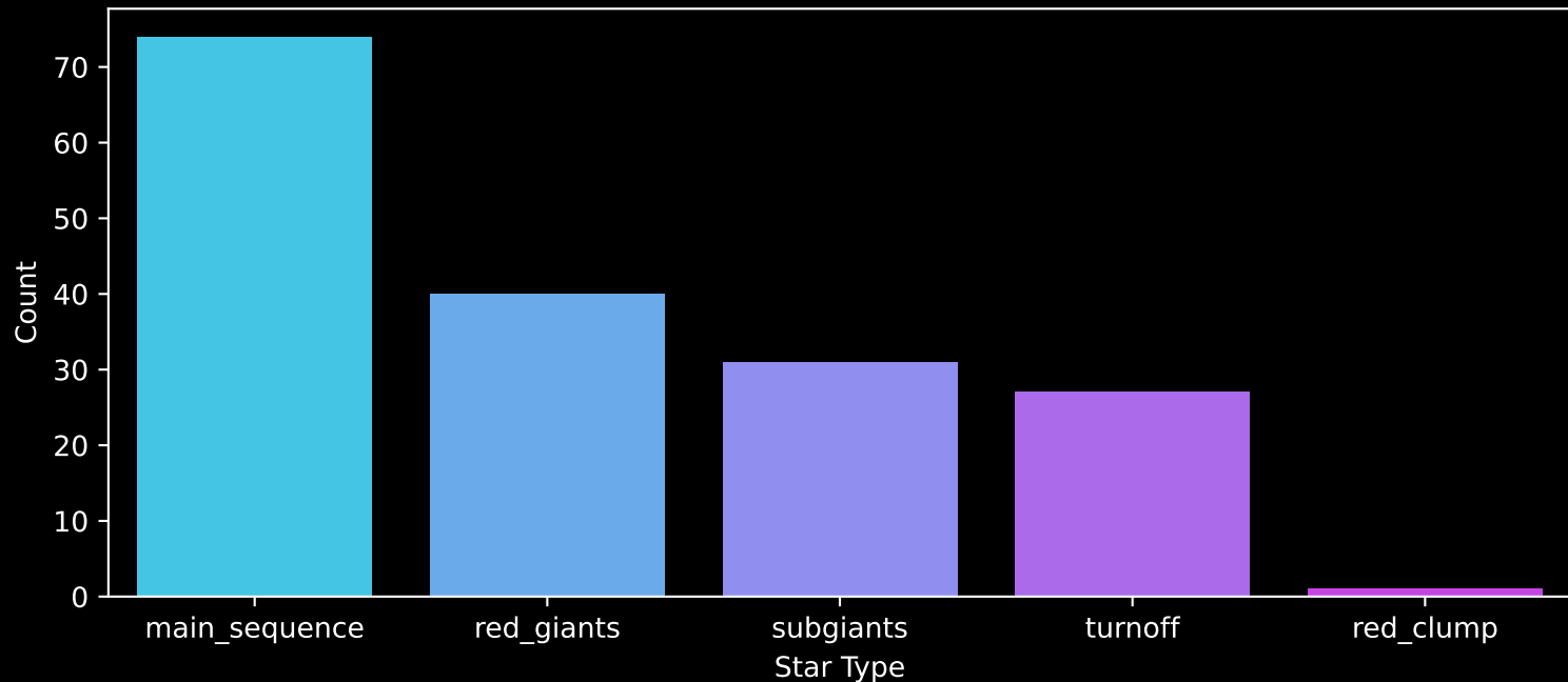
Gaia Cluster: [Ruprecht_127] Count plot of Star Type
