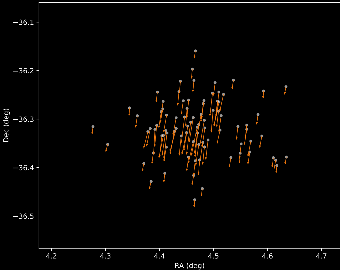
Gaia DR3 Cluster 2 Proper Motion Vectors (n=85)
