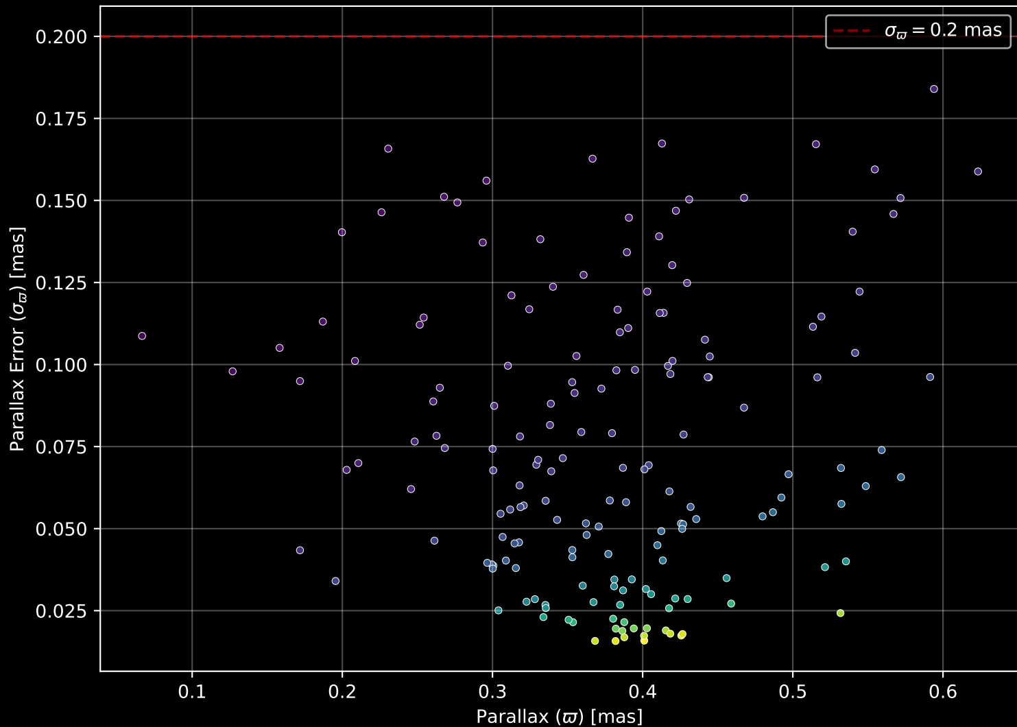
Gaia Cluster: [Ruprecht_127] Parallax Quality (n= 173)
