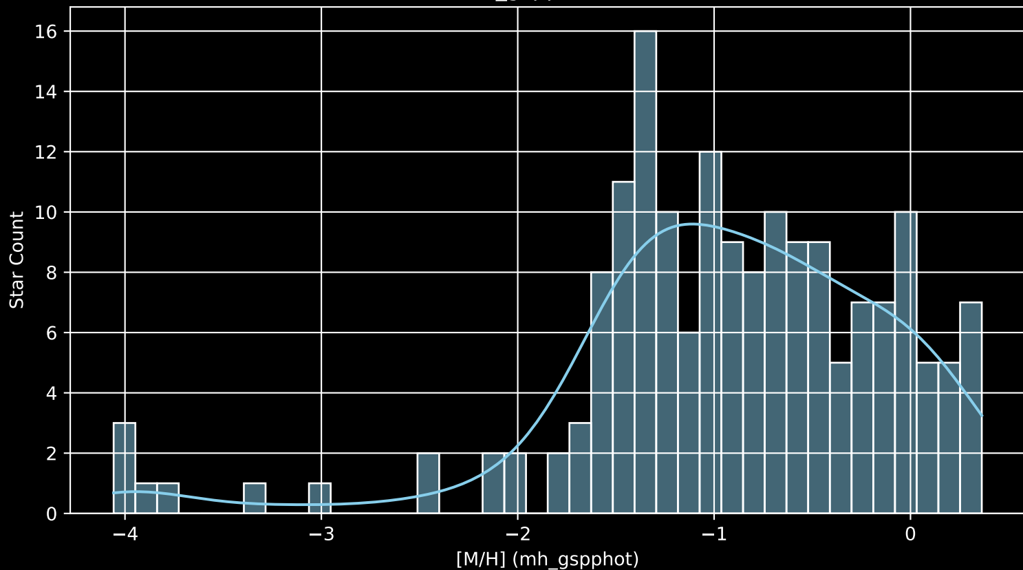
Gaia Cluster: [Ruprecht_127 [M/H] (mh_gspphot) (n= 172)
