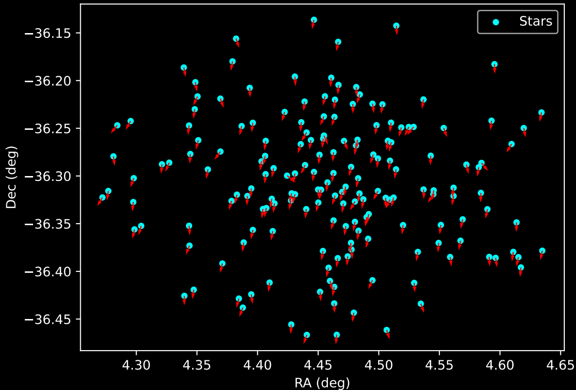
Gaia Cluster: [Ruprecht_127] Proper Motion Vectors for Gaia Star Field (n= 173)
