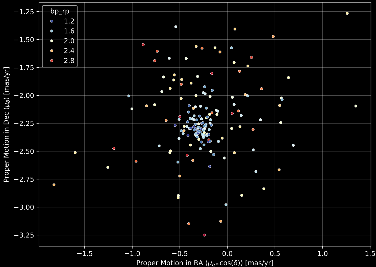
Gaia Cluster: [Ruprecht_127] Proper Motion Diagram (n= 173)
