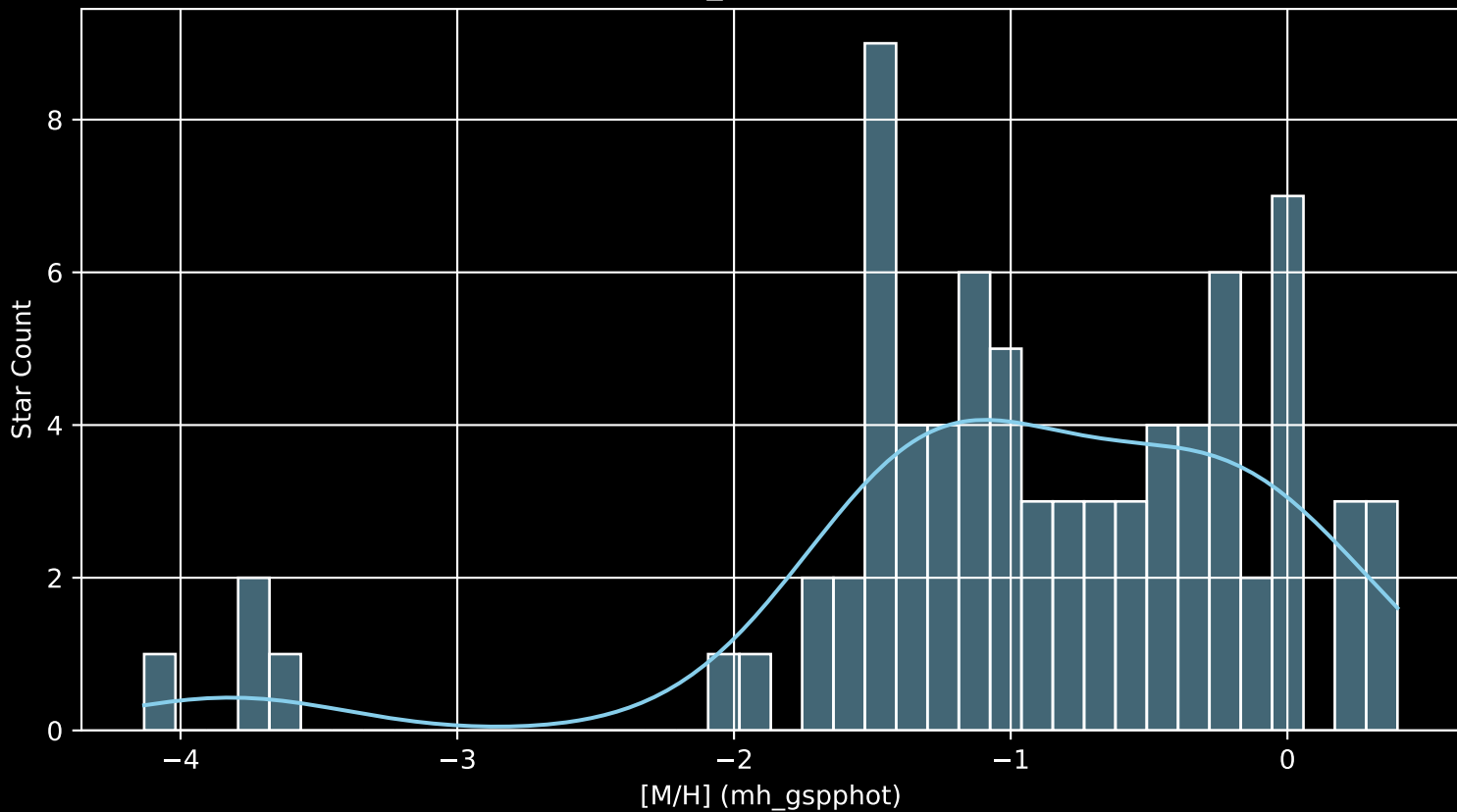
Gaia Cluster: [Ruprecht_130 [M/H] (mh_gspphot) (n= 79)
