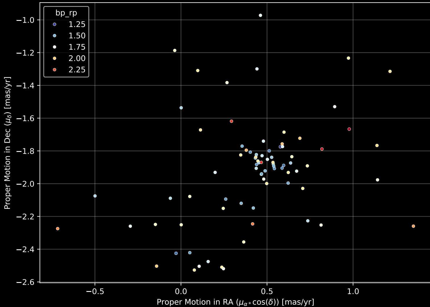
Gaia Cluster: [Ruprecht_130] Proper Motion Diagram (n= 80)
