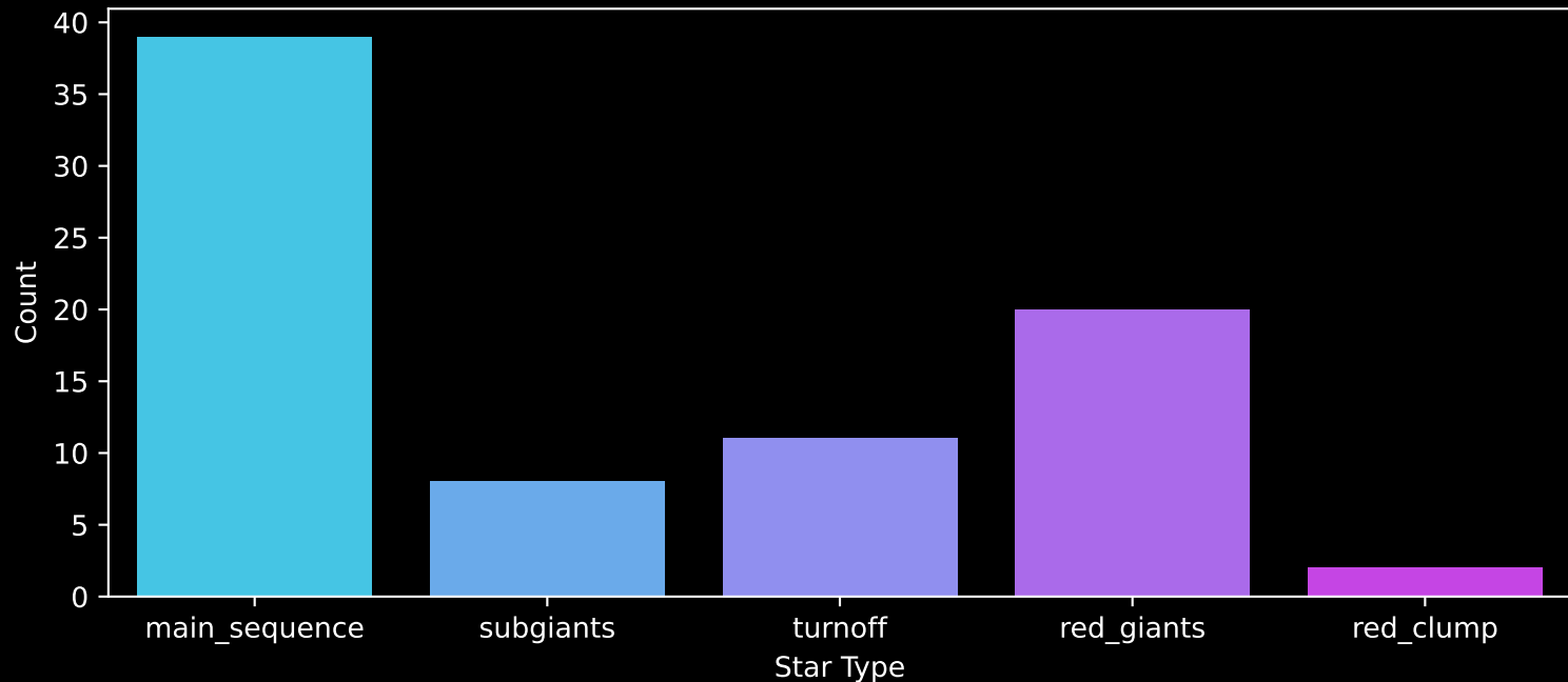
Gaia Cluster: [Ruprecht_130] Count plot of Star Type
