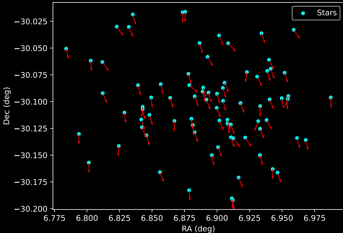
Gaia Cluster: [Ruprecht_130] Proper Motion Vectors for Gaia Star Field (n= 80)
