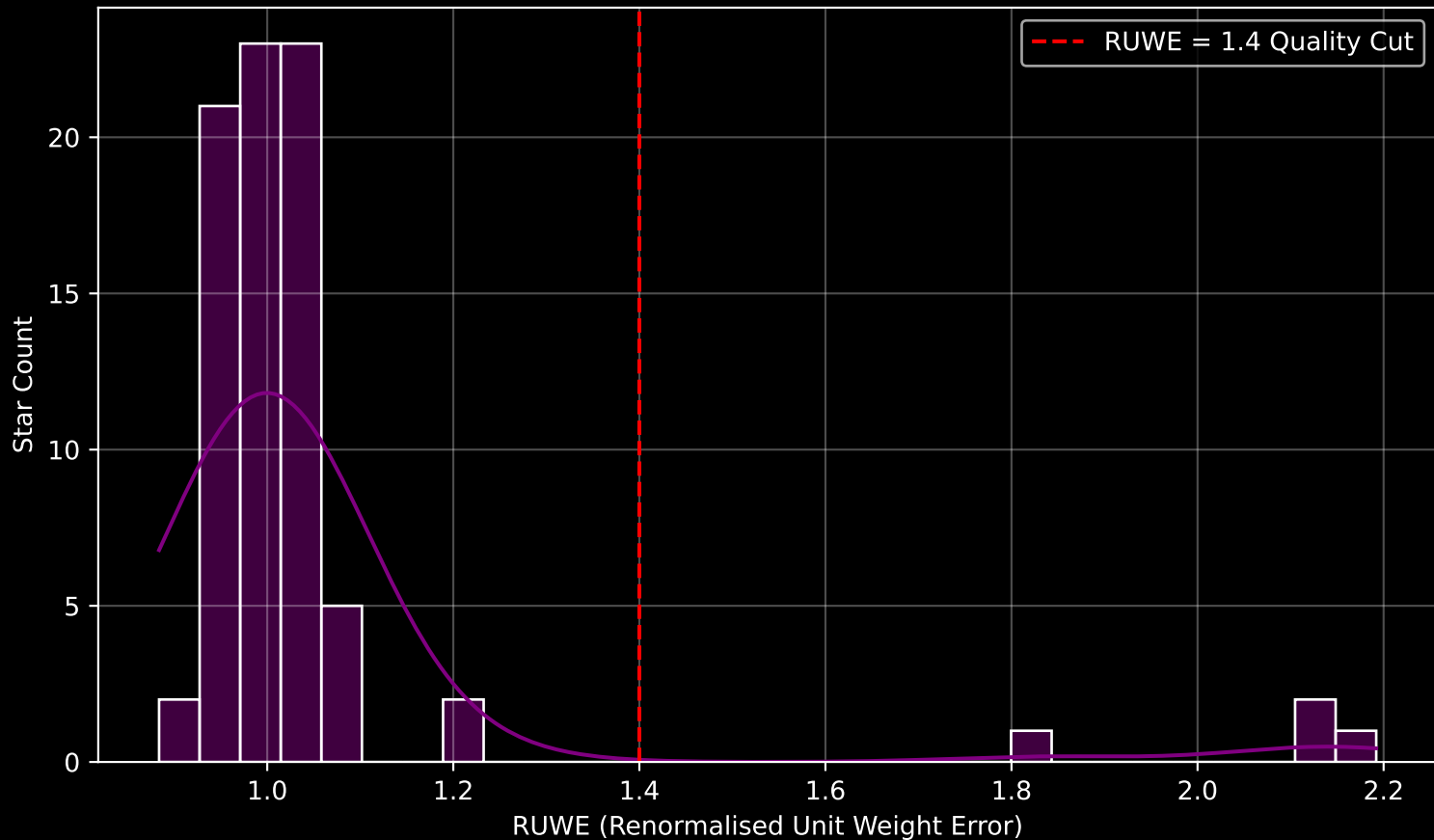
Gaia Cluster: [Ruprecht_130] RUWE Distribution (n= 80)
