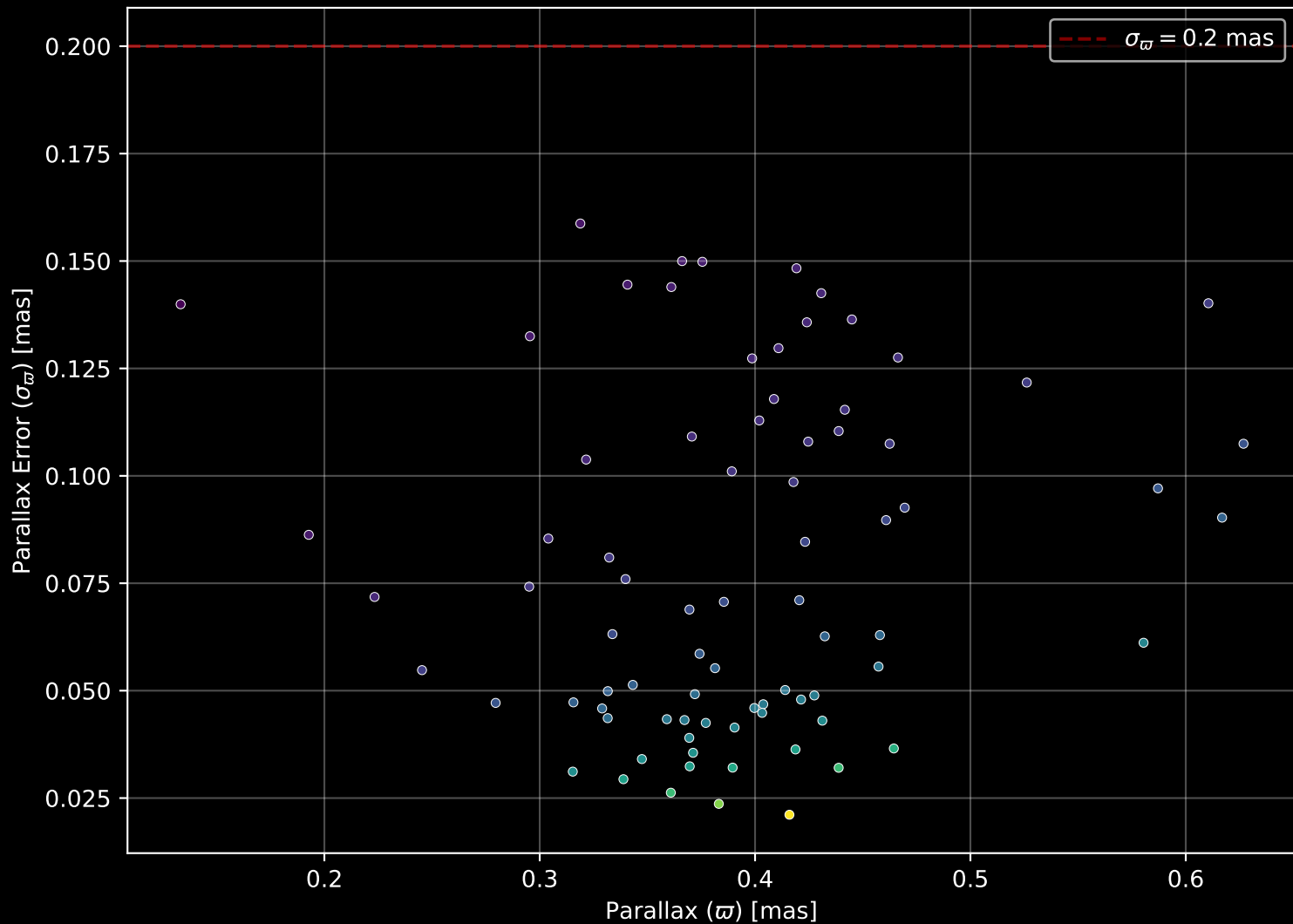
Gaia Cluster: [Ruprecht_130] Parallax Quality (n= 80)
