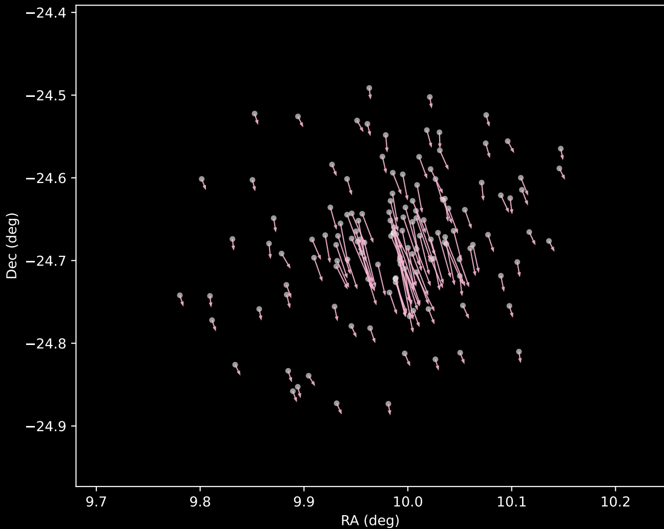
Gaia DR3 Cluster 13 Proper Motion Vectors (n=133)
