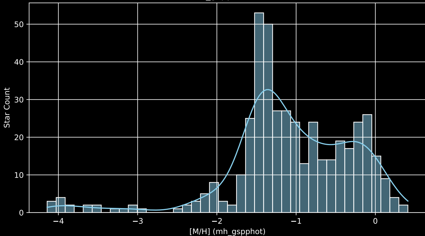
Gaia Cluster: [Ruprecht_138 [M/H] (mh_gspphot) (n= 439)
