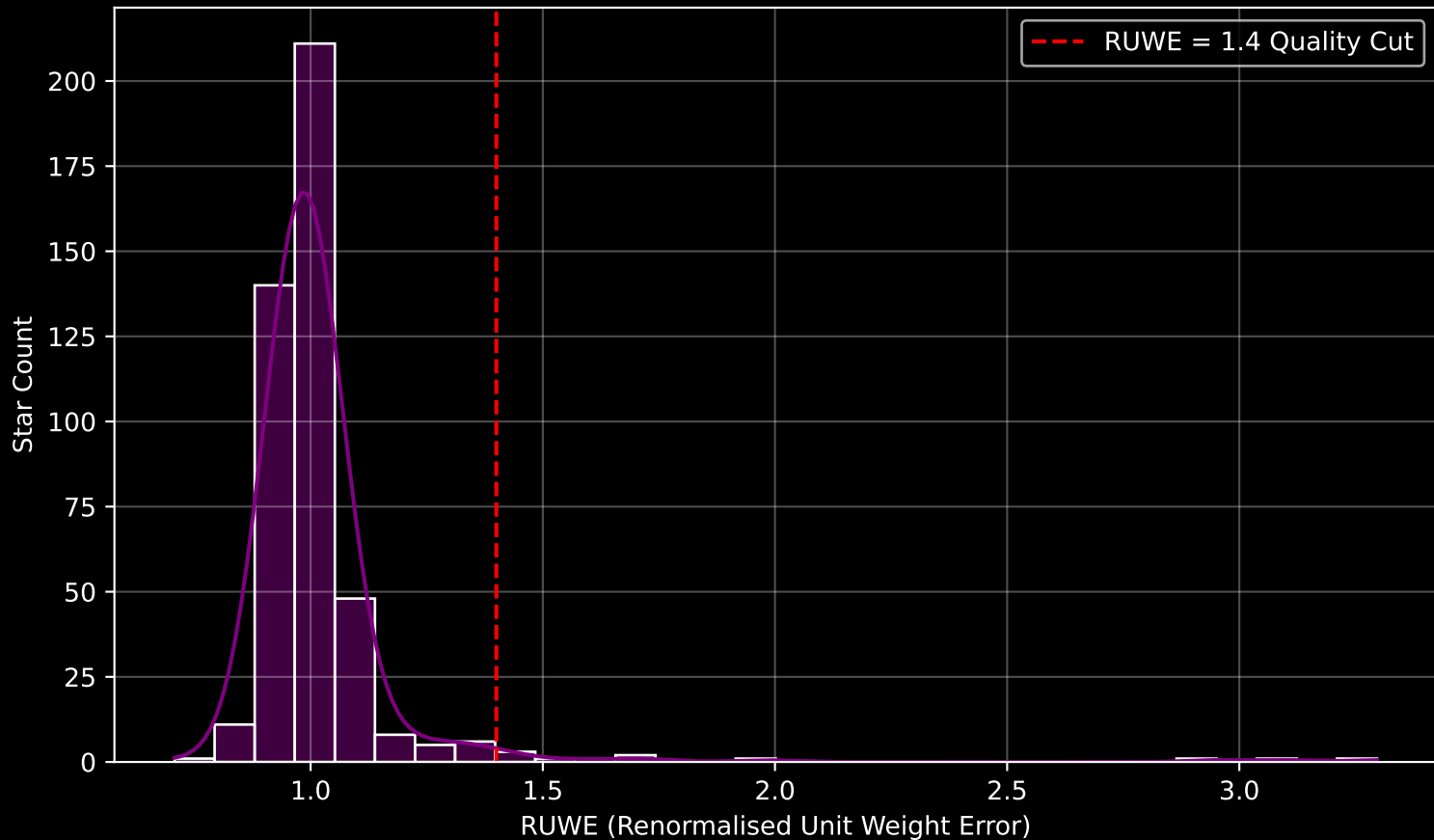
Gaia Cluster: [Ruprecht_138] RUWE Distribution (n= 440)
