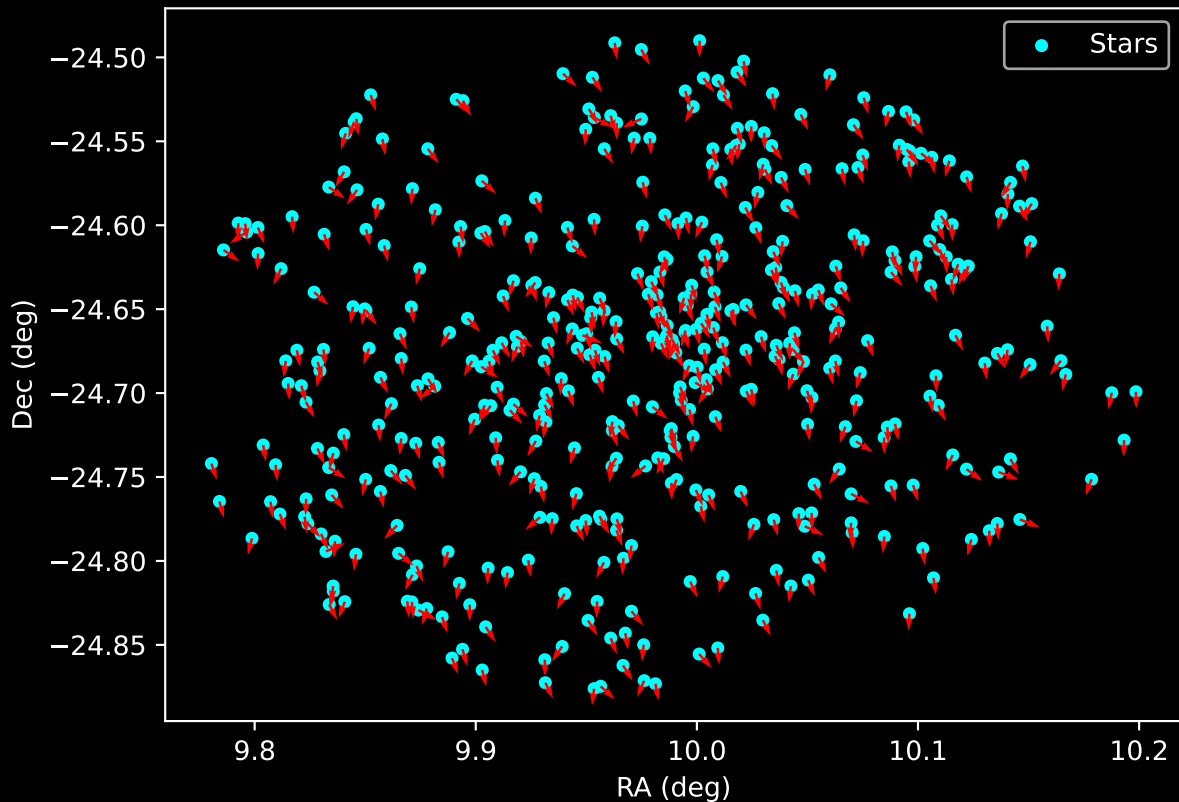
Gaia Cluster: [Ruprecht_138] Proper Motion Vectors for Gaia Star Field (n= 441)
