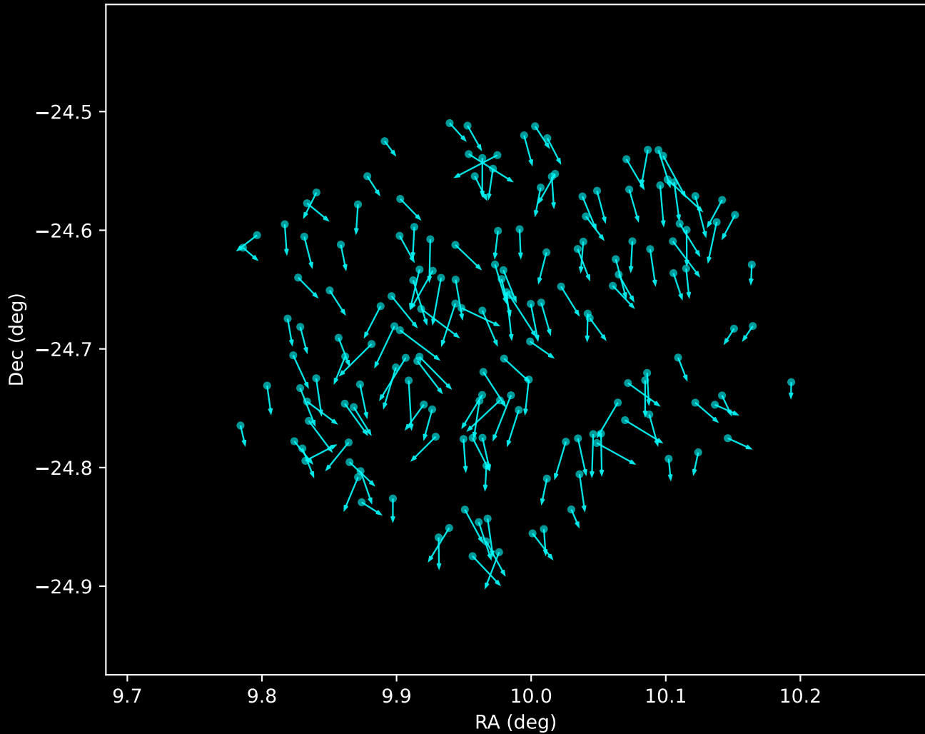
Gaia DR3 Noise Stream Proper Motion Vectors (n=163)
