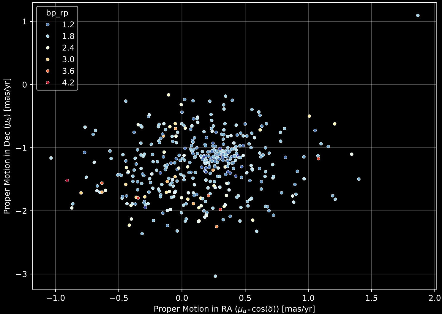
Gaia Cluster: [Ruprecht_138] Proper Motion Diagram (n= 441)
