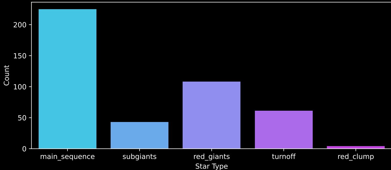
Gaia Cluster: [Ruprecht_138] Count plot of Star Type
