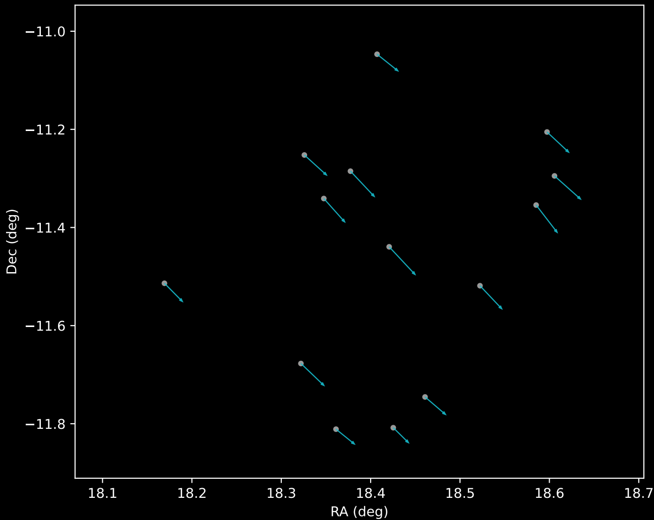
Gaia DR3 Cluster 18 Proper Motion Vectors (n=14)
