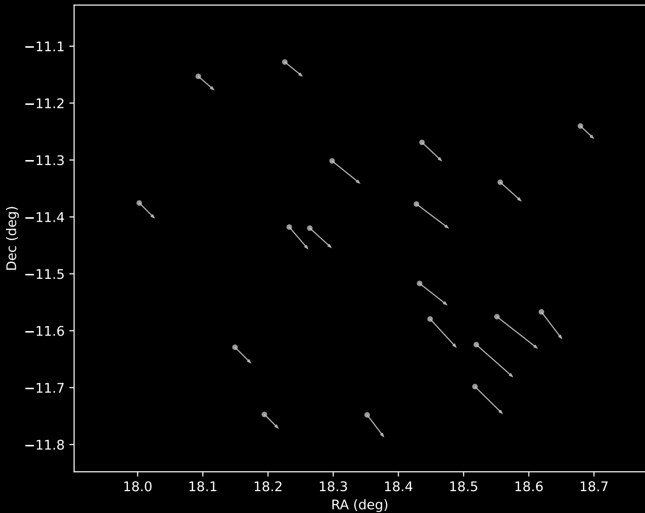
Gaia DR3 Cluster 15 Proper Motion Vectors (n=19)
