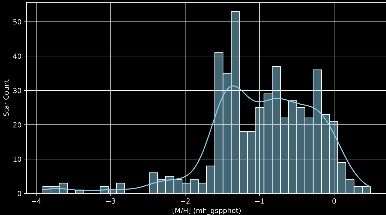
Gaia Cluster: [Ruprecht_144 [M/H] (mh_gspphot) (n= 500)
