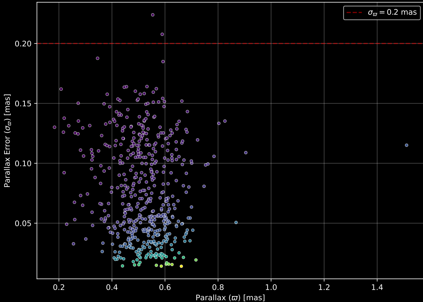
Gaia Cluster: [Ruprecht_144] Parallax Quality (n= 503)
