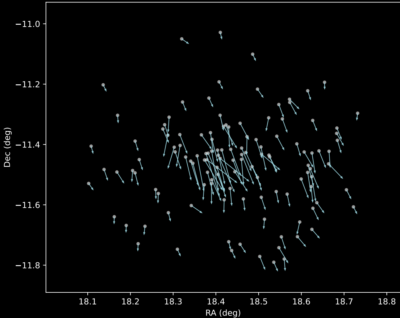
Gaia DR3 Cluster 19 Proper Motion Vectors (n=123)
