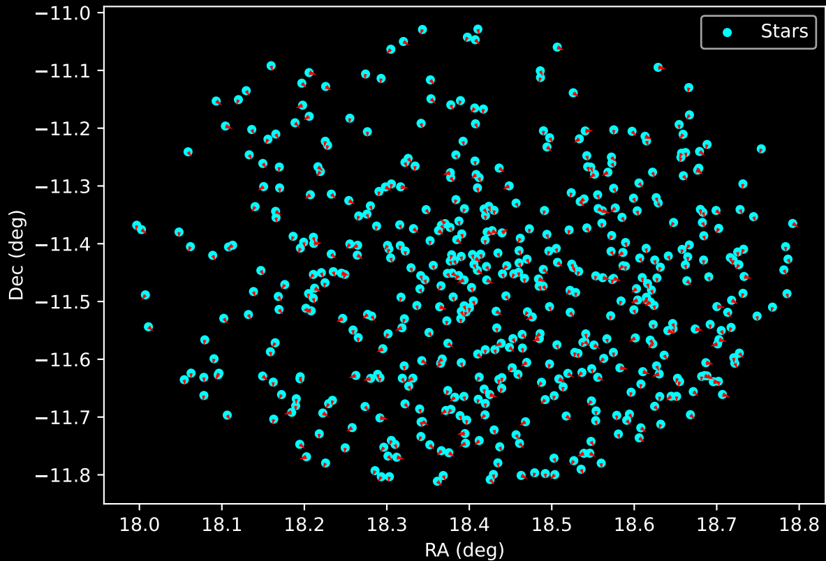
Gaia Cluster: [Ruprecht_144] Proper Motion Vectors for Gaia Star Field (n= 503)
