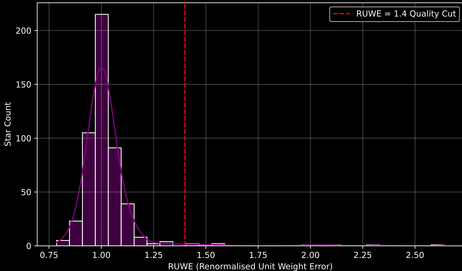
Gaia Cluster: [Ruprecht_144] RUWE Distribution (n= 502)
