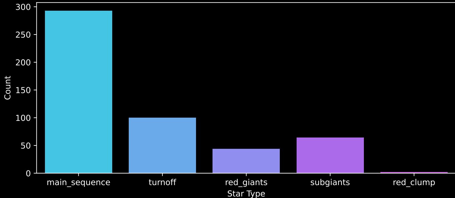
Gaia Cluster: [Ruprecht_144] Count plot of Star Type
