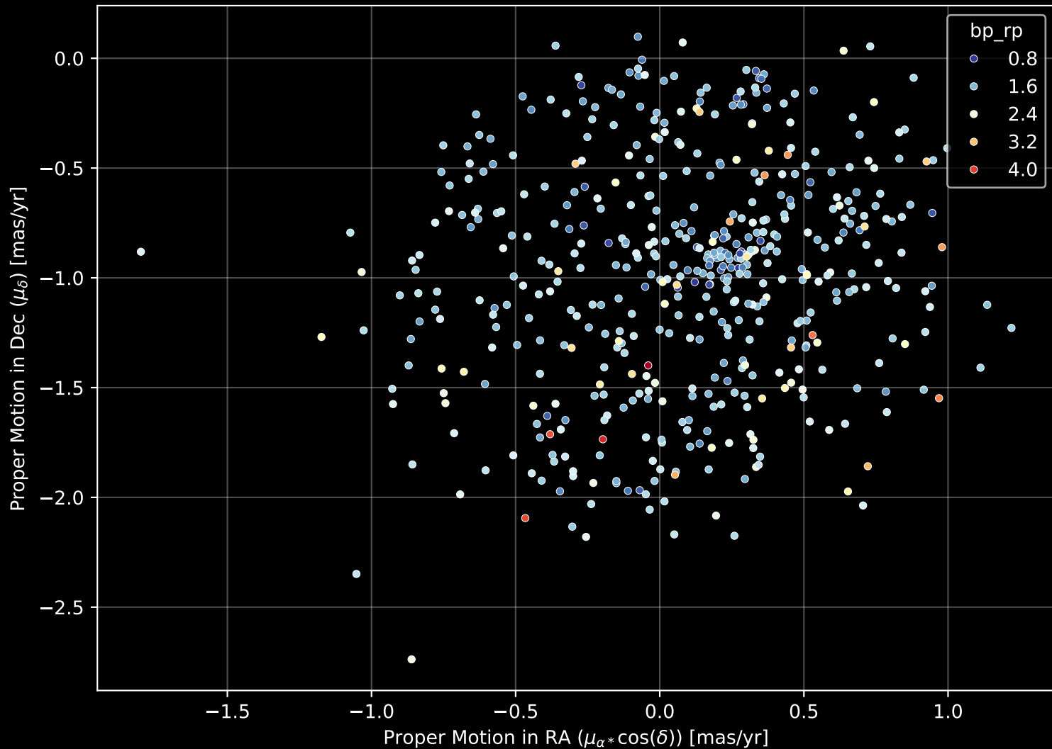
Gaia Cluster: [Ruprecht_144] Proper Motion Diagram (n= 503)
