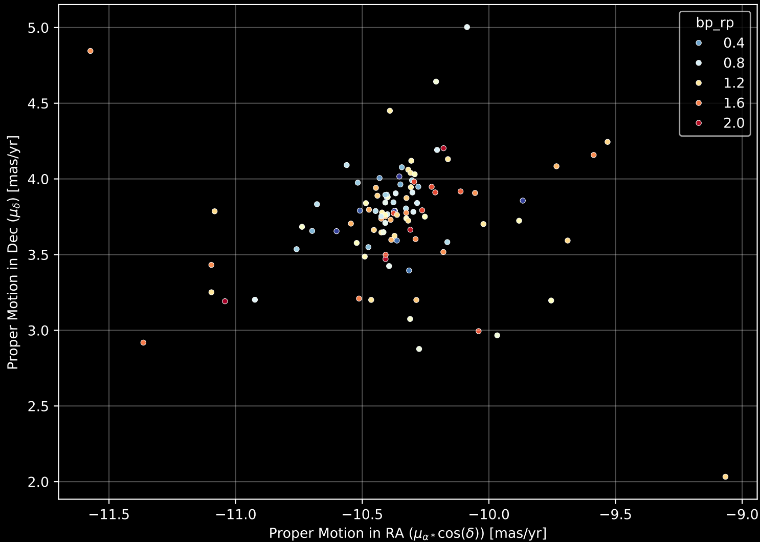
Gaia Cluster: [Ruprecht_161] Proper Motion Diagram (n= 105)
