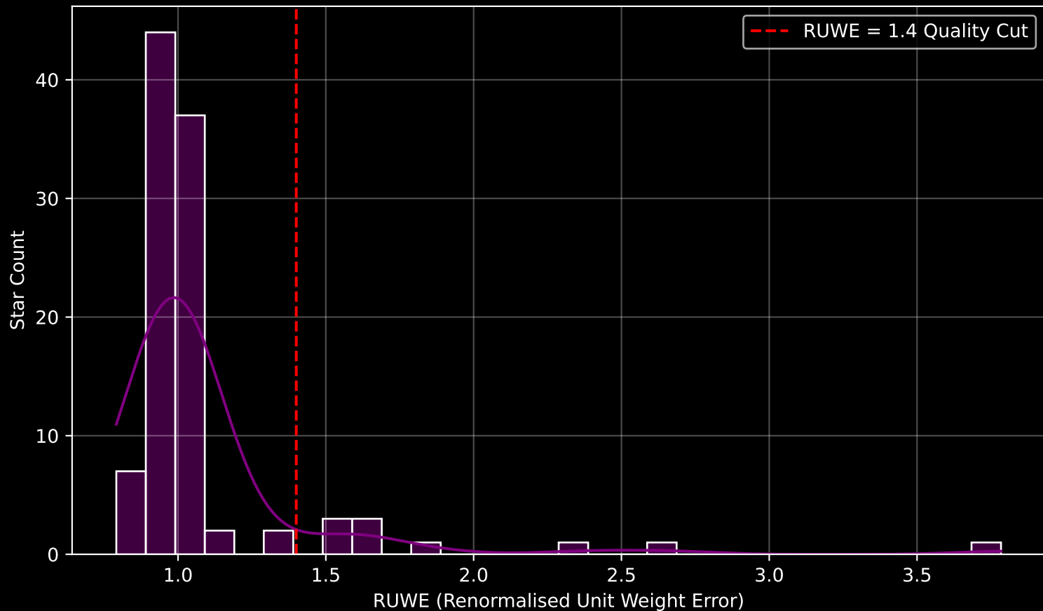
Gaia Cluster: [Ruprecht_161] RUWE Distribution (n= 102)
