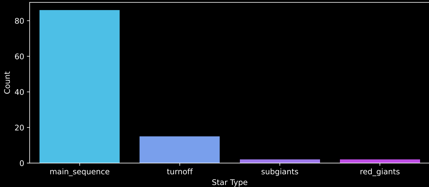
Gaia Cluster: [Ruprecht_161] Count plot of Star Type
