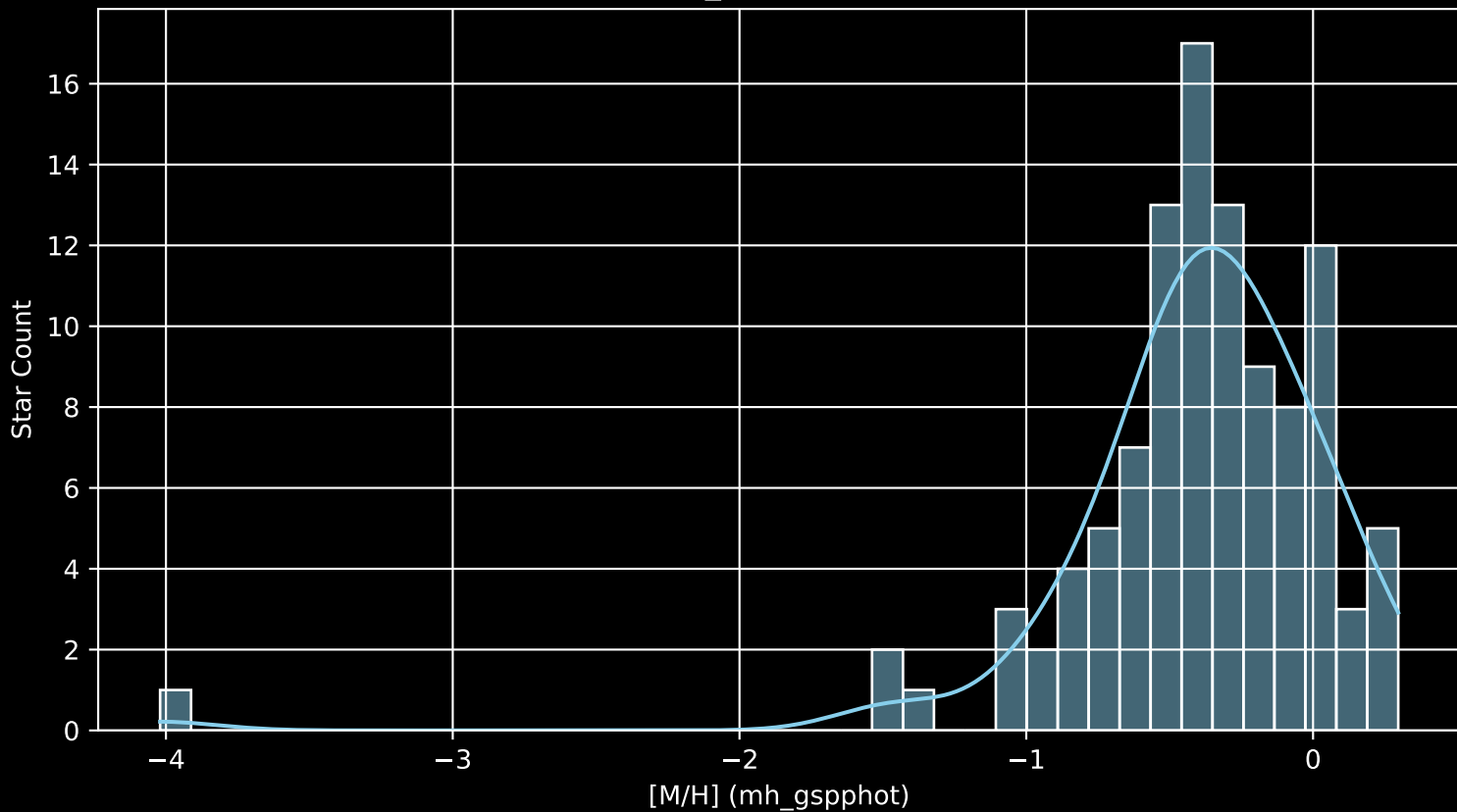
Gaia Cluster: [Ruprecht_161 [M/H] (mh_gspphot) (n= 105)
