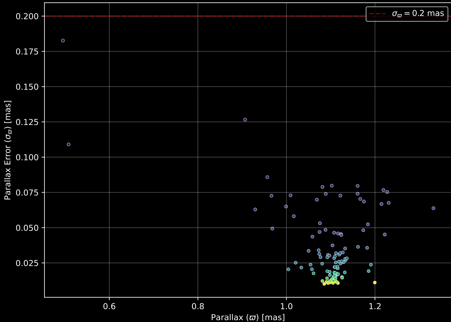
Gaia Cluster: [Ruprecht_161] Parallax Quality (n= 105)
