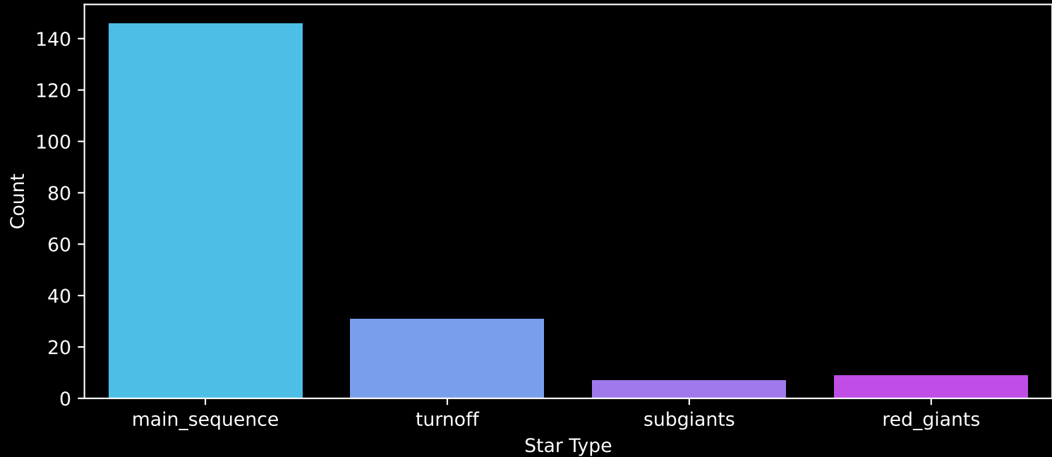
Gaia Cluster: [Ruprecht_167] Count plot of Star Type
