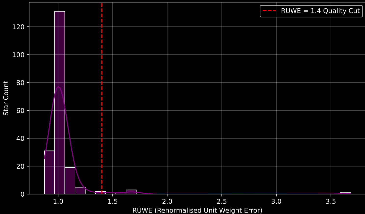
Gaia Cluster: [Ruprecht_167] RUWE Distribution (n= 193)
