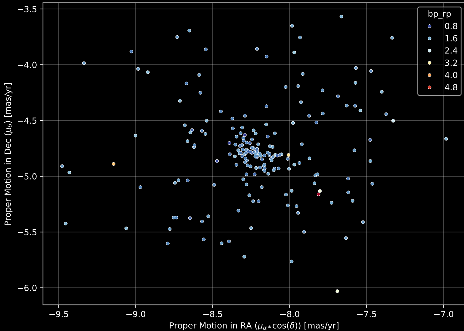
Gaia Cluster: [Ruprecht_167] Proper Motion Diagram (n= 193)
