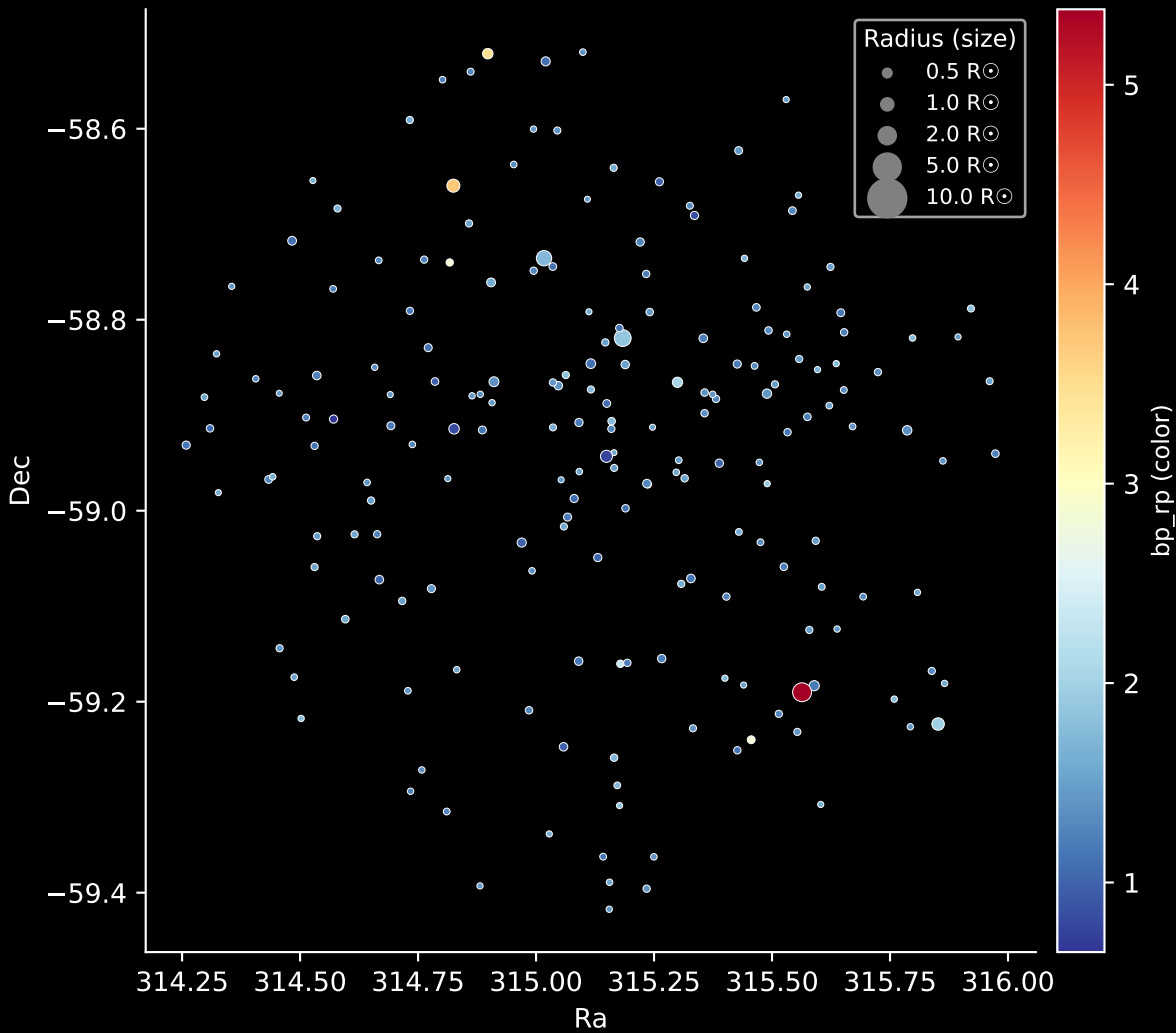
Gaia Cluster: [Ruprecht_167] Stars: 193
