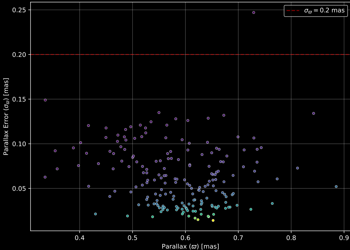
Gaia Cluster: [Ruprecht_167] Parallax Quality (n= 193)
