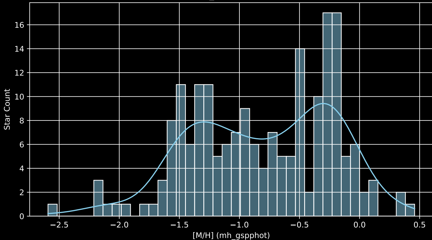
Gaia Cluster: [Ruprecht_167 [M/H] (mh_gspphot) (n= 192)
