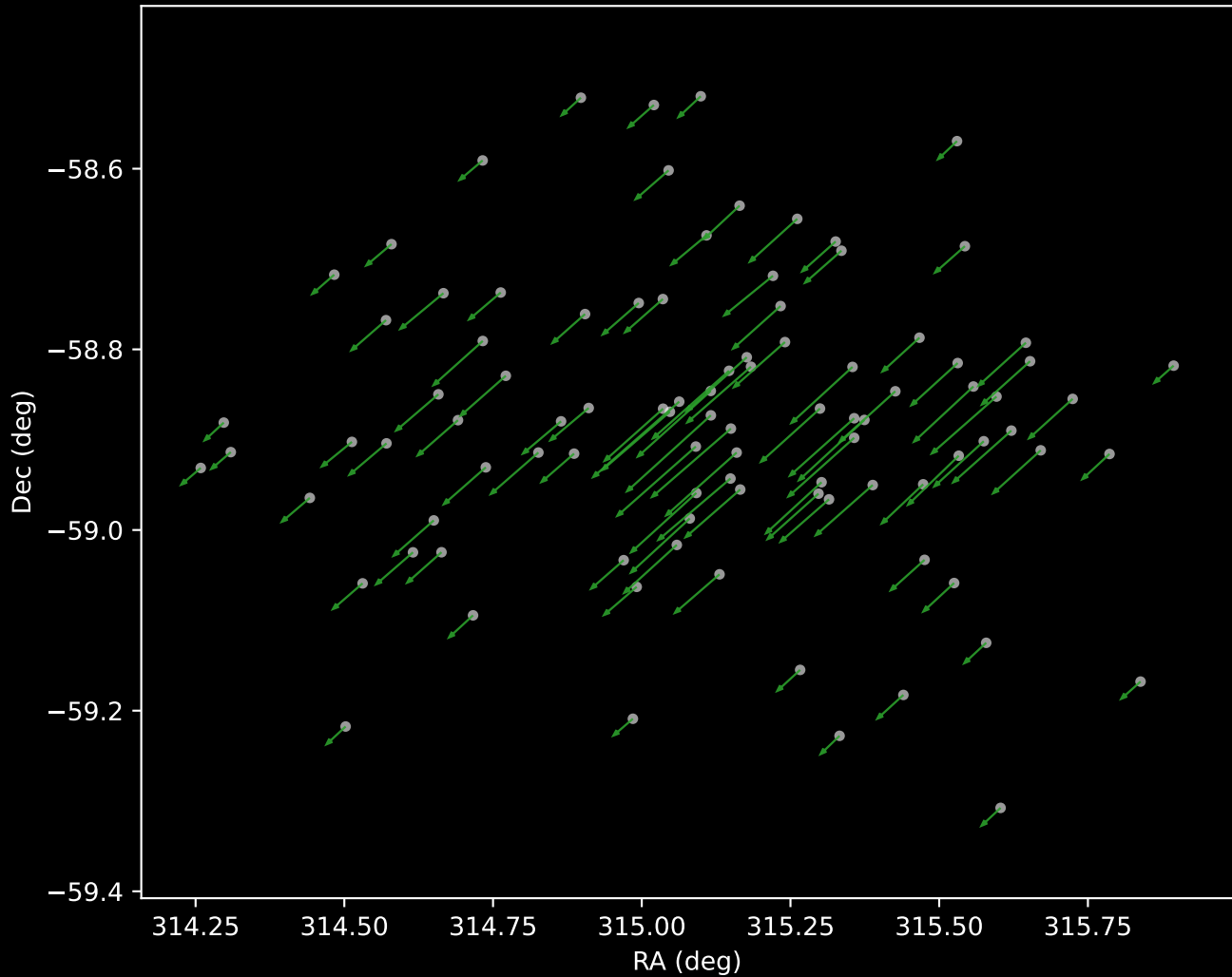
Gaia DR3 Cluster 4 Proper Motion Vectors (n=96)
