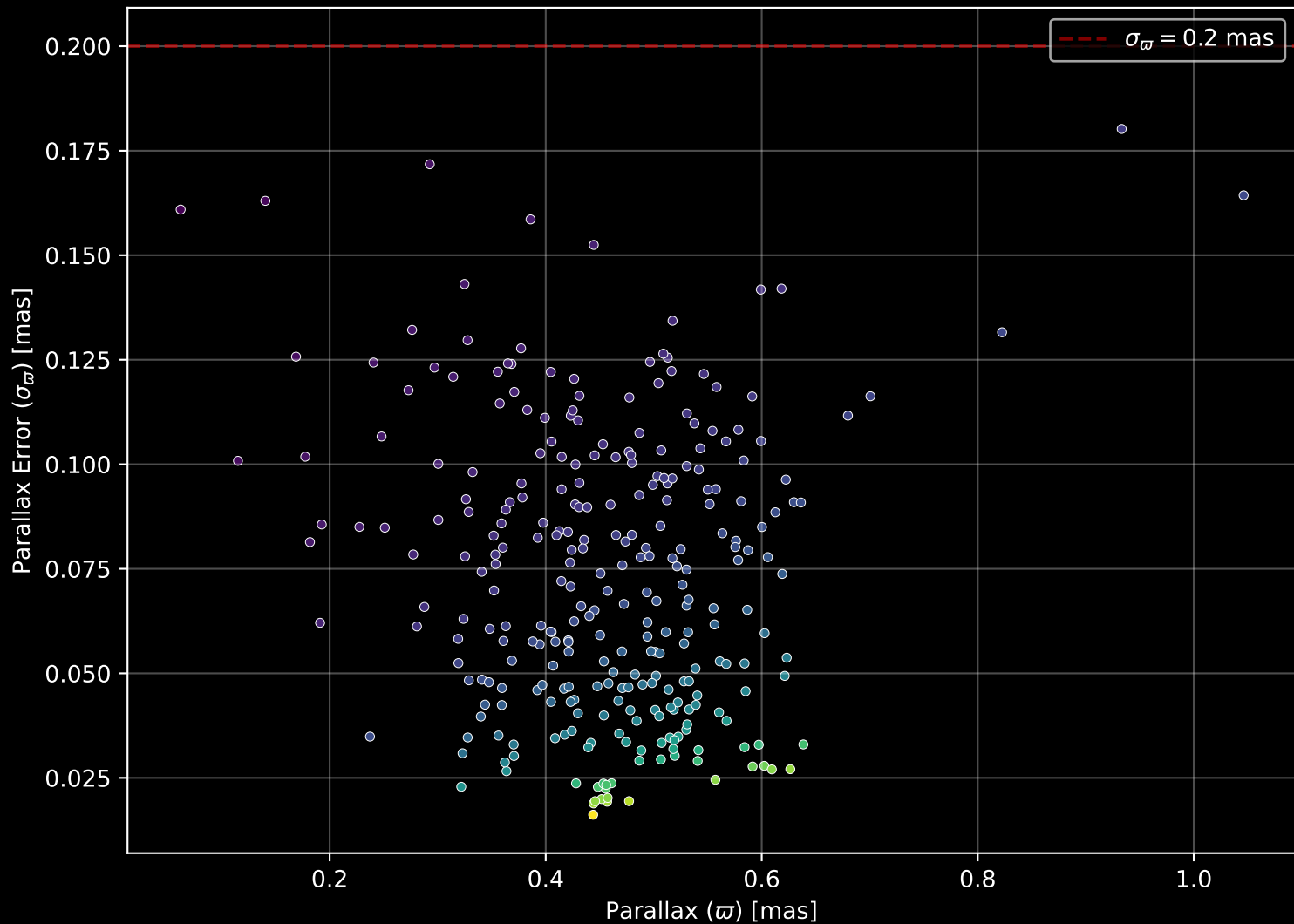
Gaia Cluster: [Ruprecht_170] Parallax Quality (n= 288)
