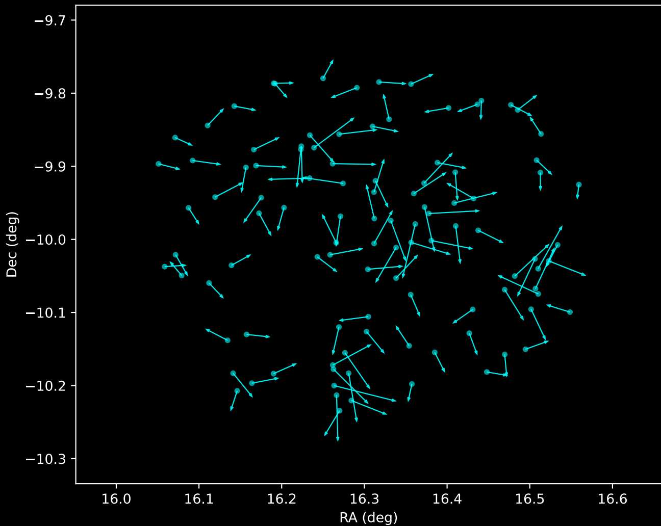
Gaia DR3 Noise Stream Proper Motion Vectors (n=104)
