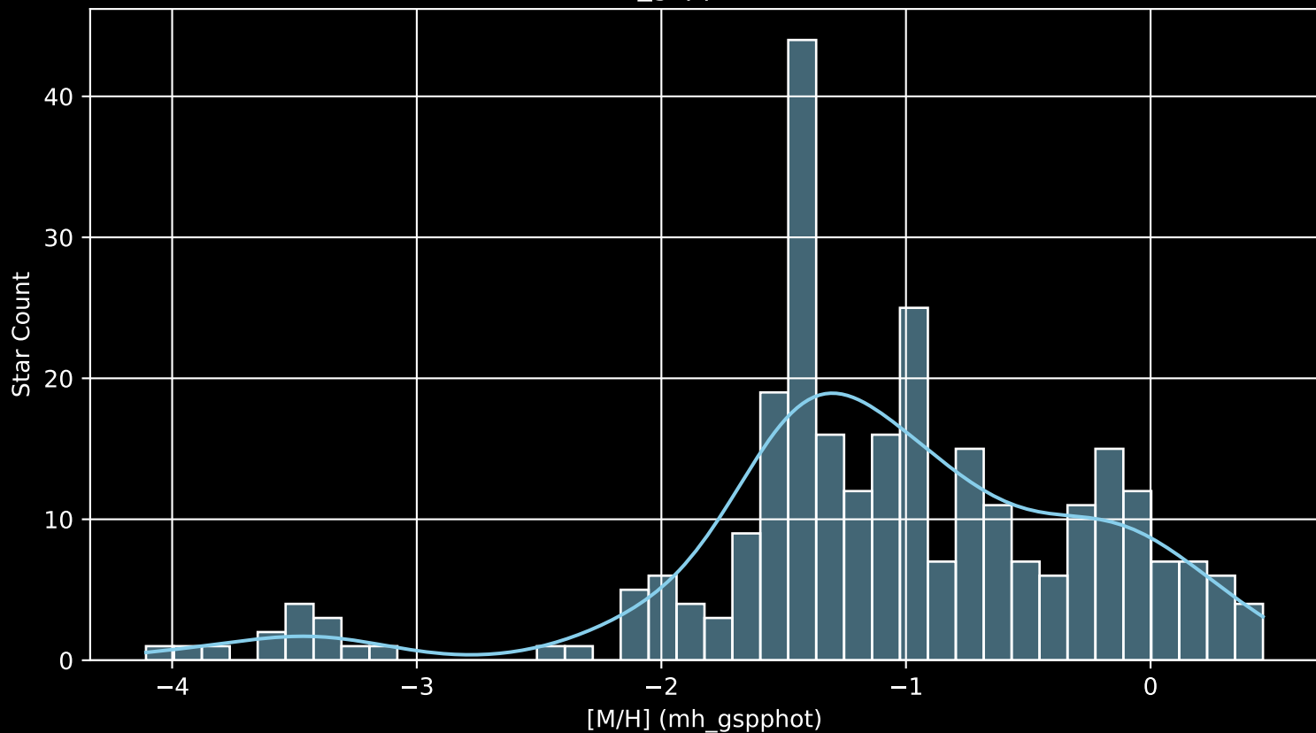
Gaia Cluster: [Ruprecht_170 [M/H] (mh_gspphot) (n= 283)
