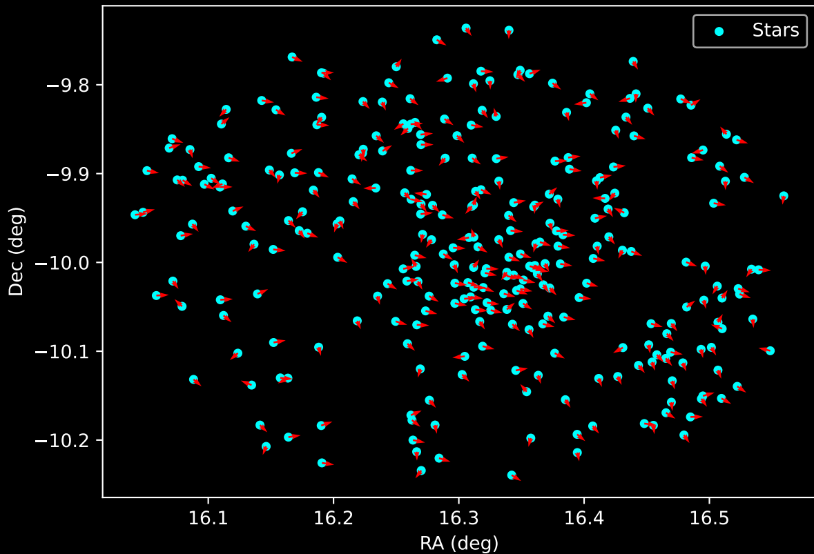
Gaia Cluster: [Ruprecht_170] Proper Motion Vectors for Gaia Star Field (n= 288)
