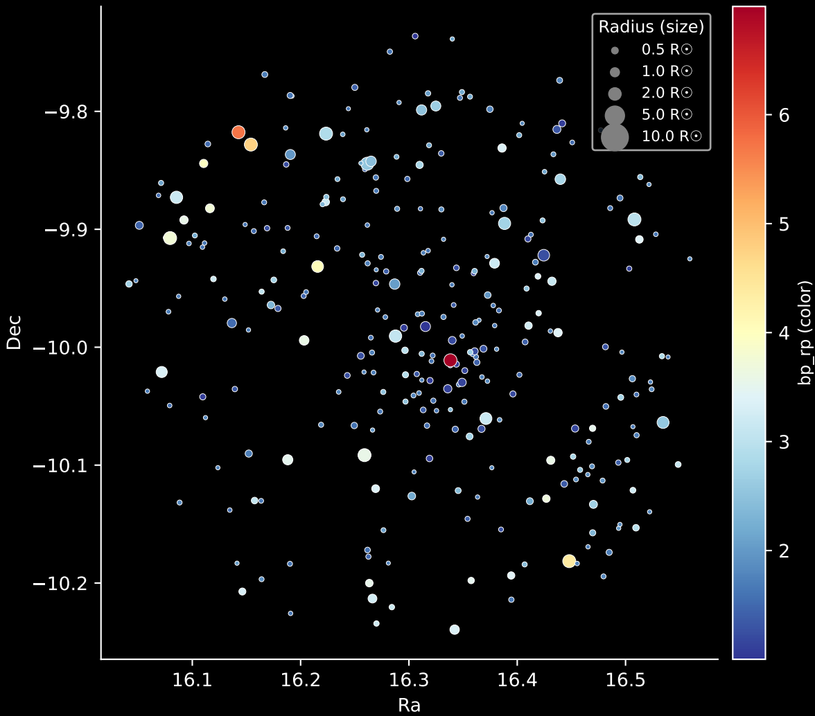
Gaia Cluster: [Ruprecht_170] Stars: 288
