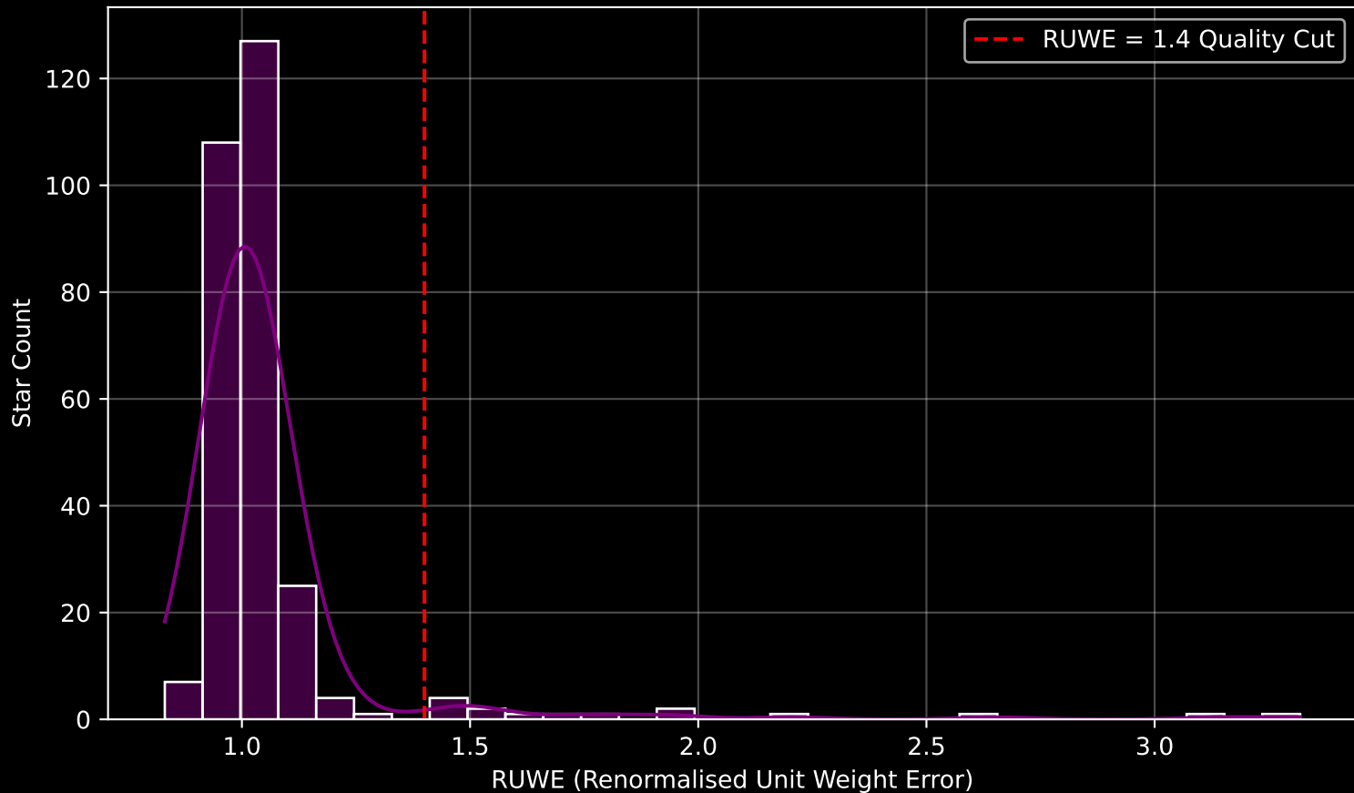
Gaia Cluster: [Ruprecht_170] RUWE Distribution (n= 287)
