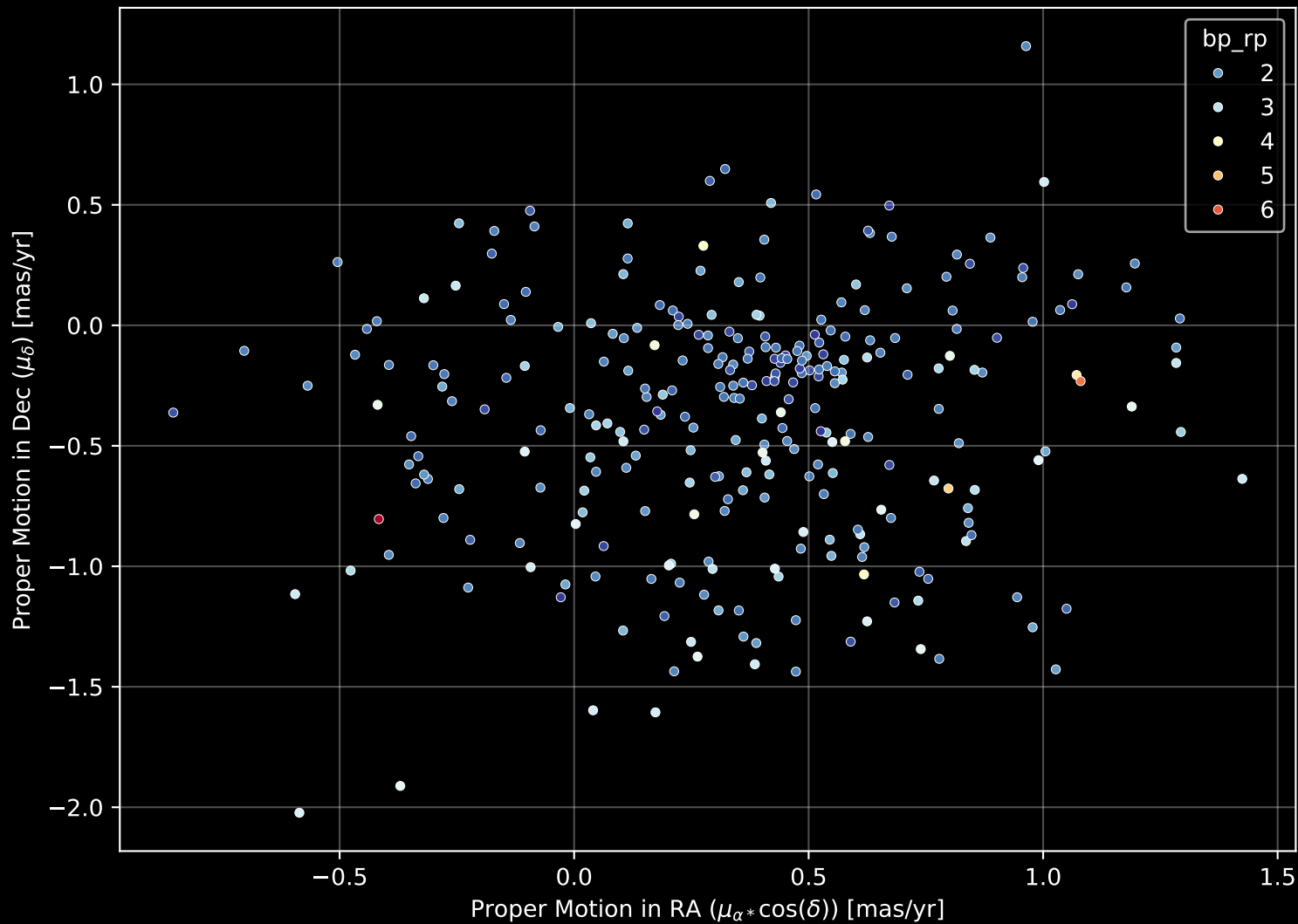
Gaia Cluster: [Ruprecht_170] Proper Motion Diagram (n= 288)
