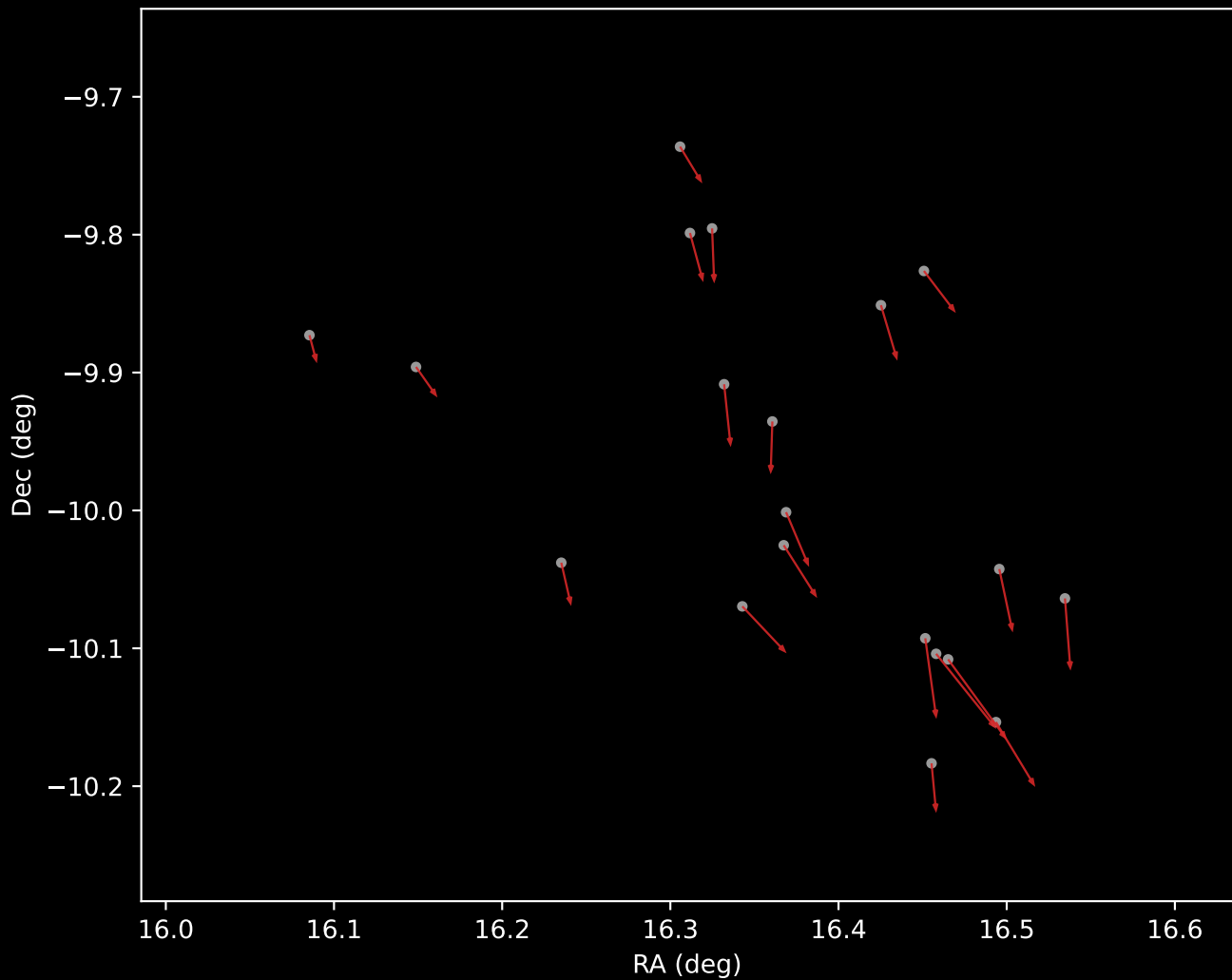
Gaia DR3 Cluster 6 Proper Motion Vectors (n=20)
