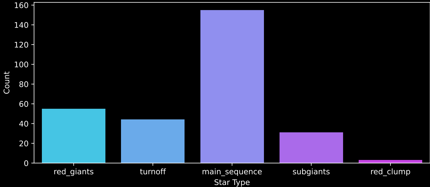
Gaia Cluster: [Ruprecht_170] Count plot of Star Type
