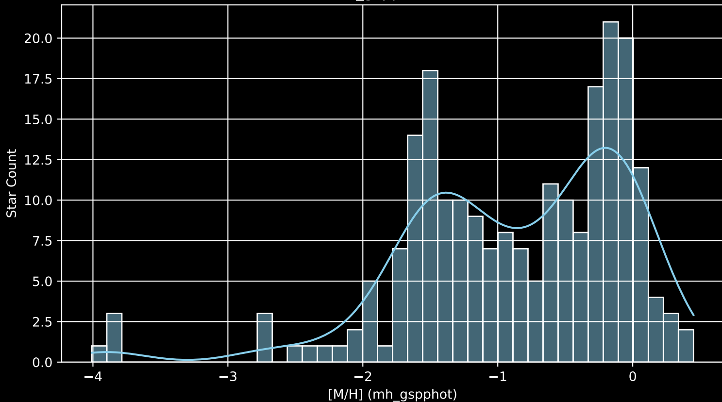
Gaia Cluster: [Ruprecht_172 [M/H] (mh_gspphot) (n= 222)
