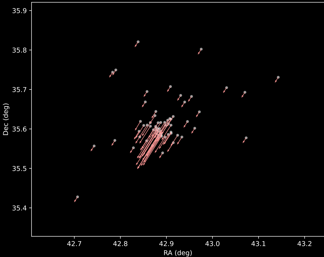
Gaia DR3 Cluster 7 Proper Motion Vectors (n=65)
