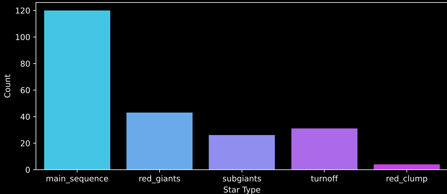
Gaia Cluster: [Ruprecht_172] Count plot of Star Type
