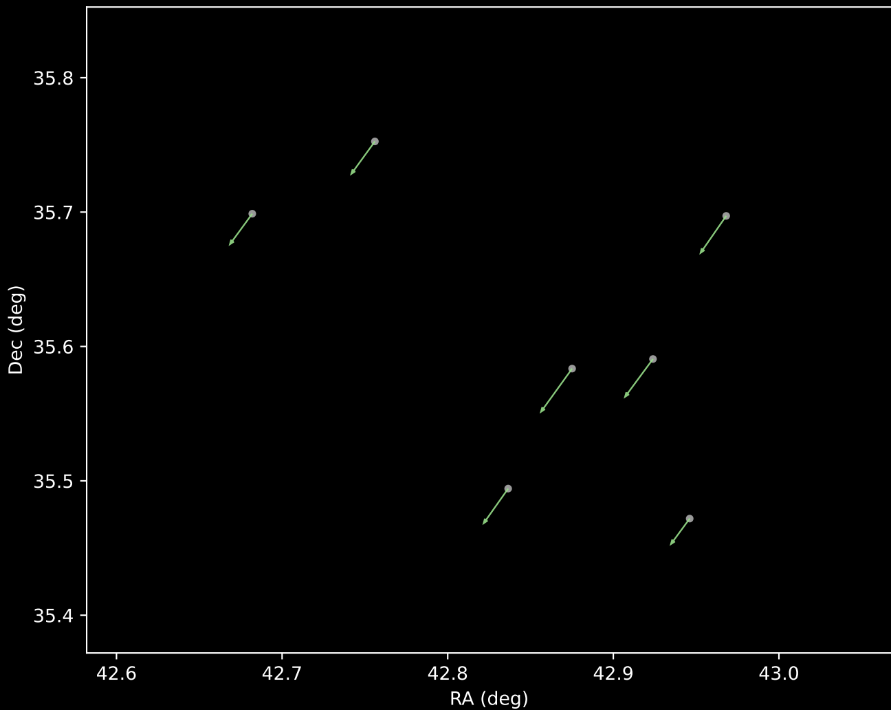
Gaia DR3 Cluster 5 Proper Motion Vectors (n=7)
