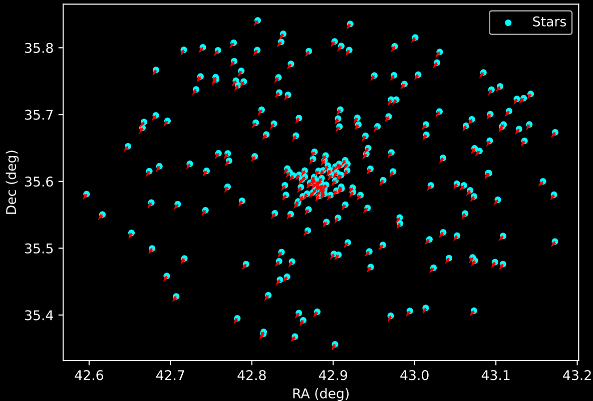
Gaia Cluster: [Ruprecht_172] Proper Motion Vectors for Gaia Star Field (n= 224)
