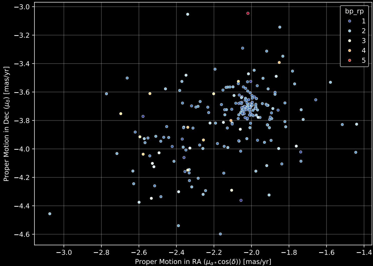
Gaia Cluster: [Ruprecht_172] Proper Motion Diagram (n= 224)
