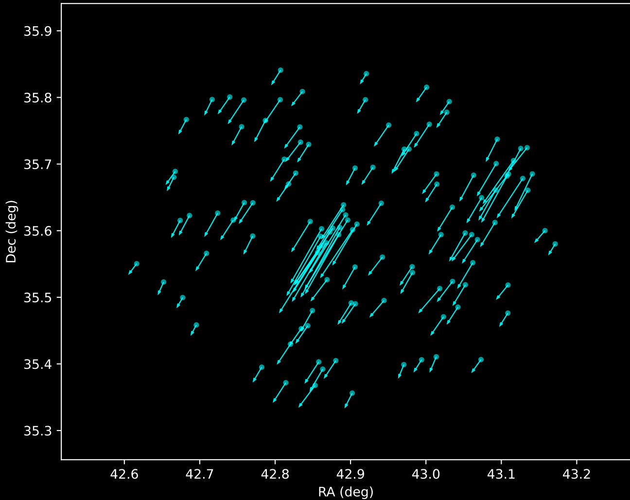
Gaia DR3 Noise Stream Proper Motion Vectors (n=112)
