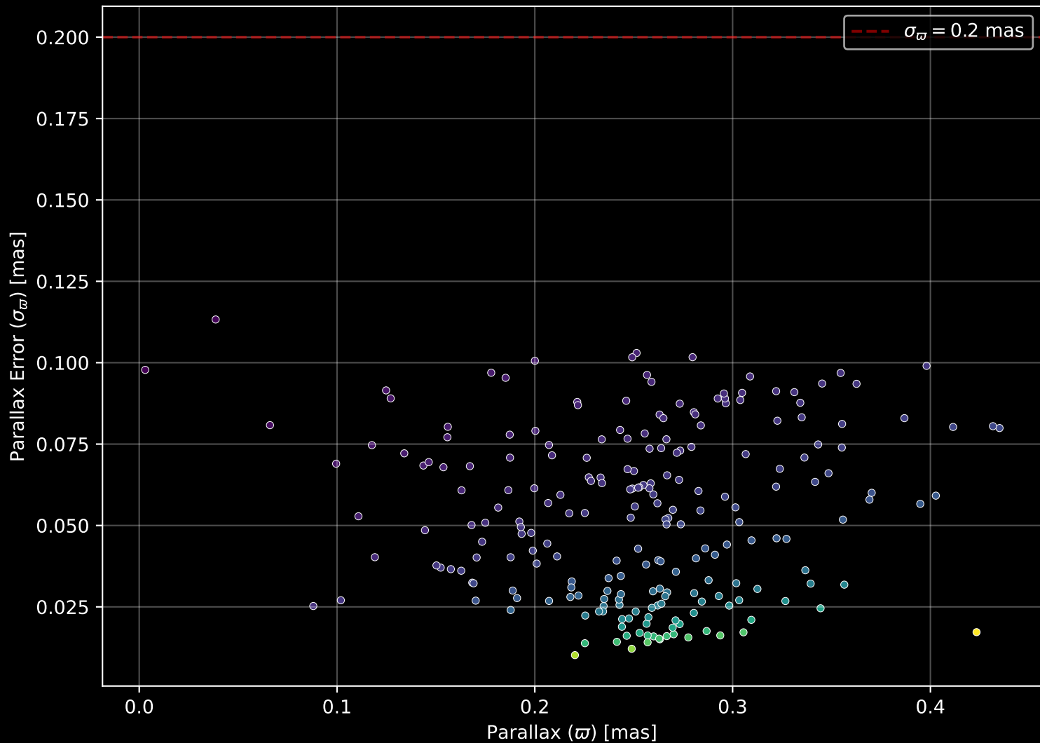
Gaia Cluster: [Ruprecht_172] Parallax Quality (n= 224)
