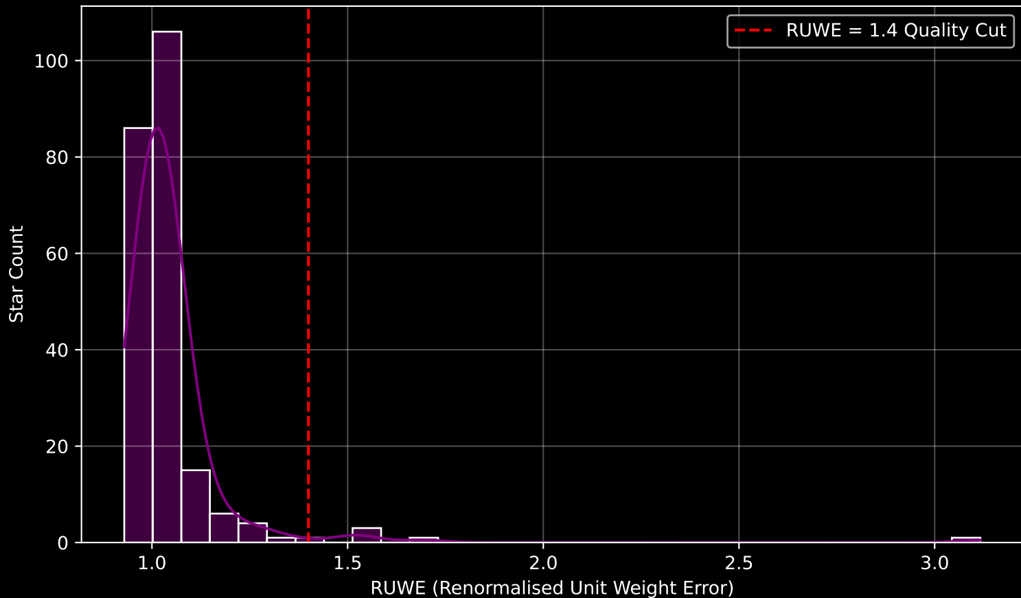
Gaia Cluster: [Ruprecht_172] RUWE Distribution (n= 224)
