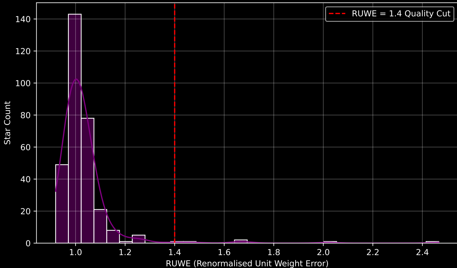
Gaia Cluster: [Ruprecht_174] RUWE Distribution (n= 311)
