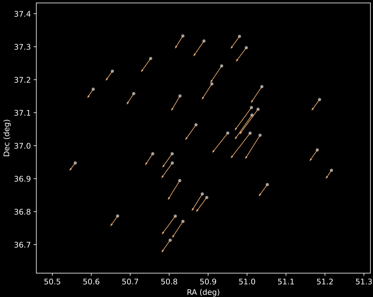
Gaia DR3 Cluster 3 Proper Motion Vectors (n=34)
