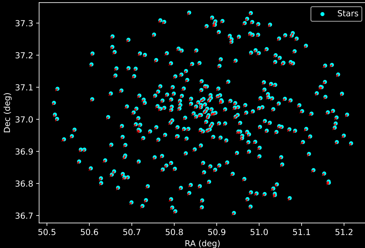
Gaia Cluster: [Ruprecht_174] Proper Motion Vectors for Gaia Star Field (n= 311)
