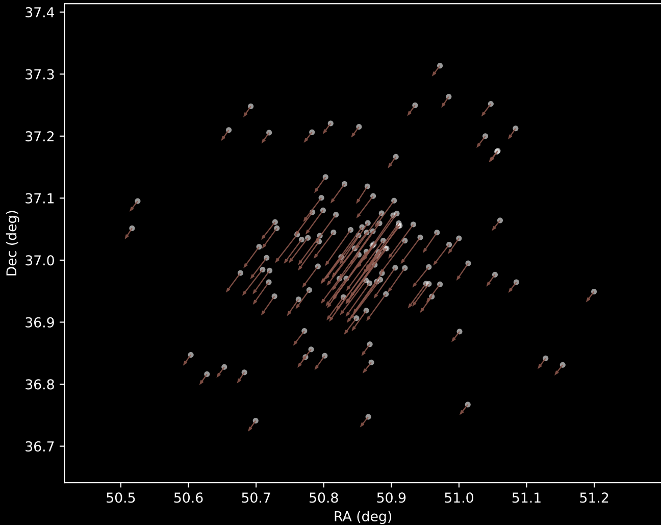
Gaia DR3 Cluster 10 Proper Motion Vectors (n=114)
