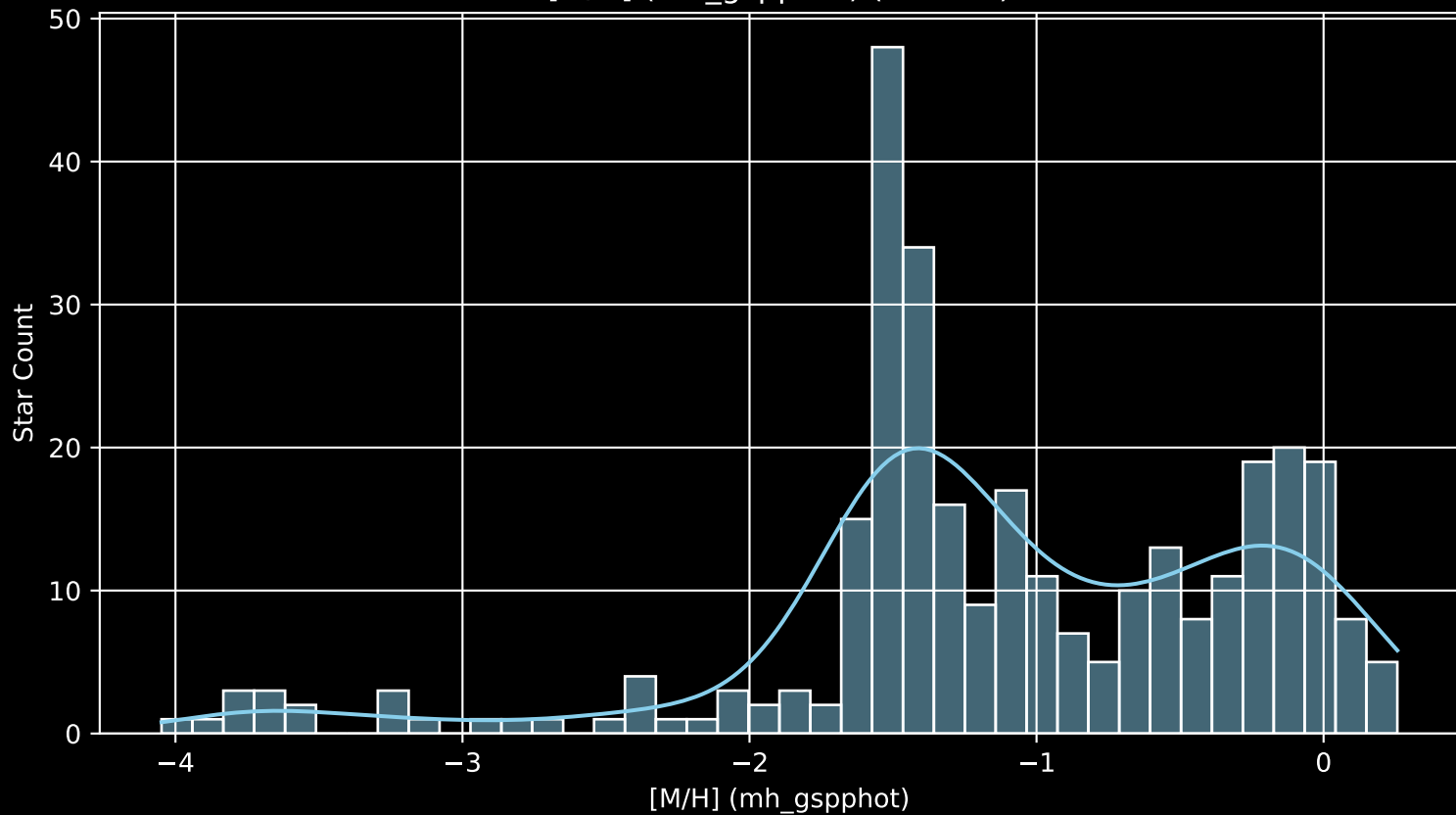
Gaia Cluster: [Ruprecht_174 [M/H] (mh_gspphot) (n= 309)
