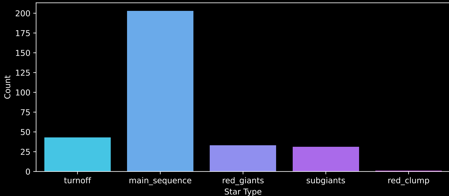
Gaia Cluster: [Ruprecht_174] Count plot of Star Type
