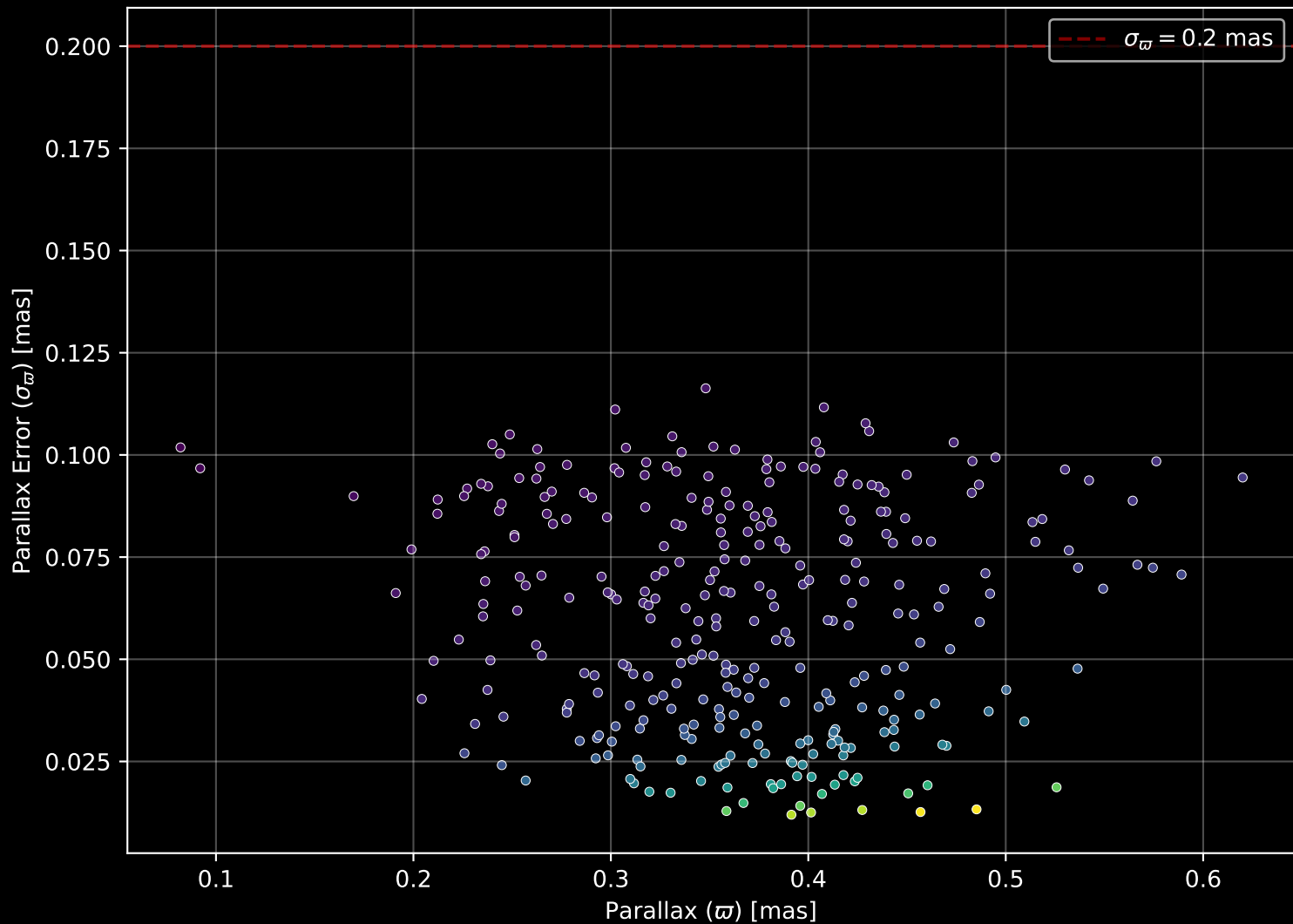
Gaia Cluster: [Ruprecht_174] Parallax Quality (n= 311)
