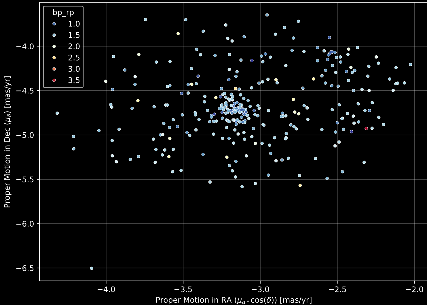
Gaia Cluster: [Ruprecht_174] Proper Motion Diagram (n= 311)
