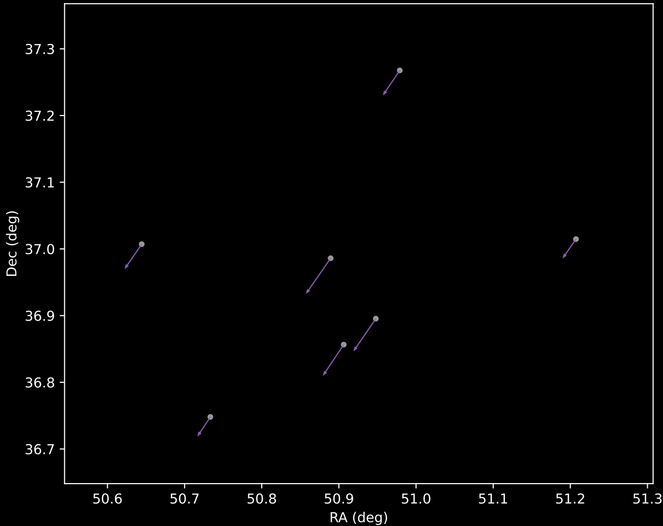
Gaia DR3 Cluster 8 Proper Motion Vectors (n=7)
