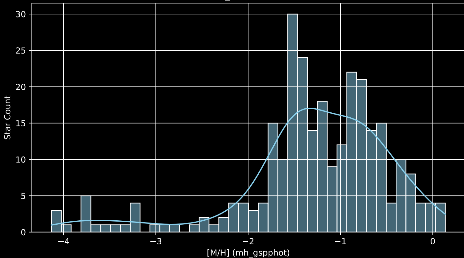
Gaia Cluster: [Ruprecht_18 [M/H] (mh_gspphot) (n= 279)
