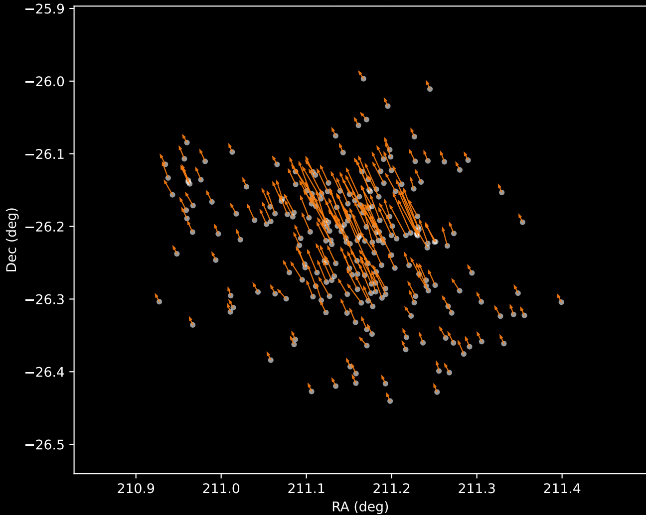
Gaia DR3 Cluster 2 Proper Motion Vectors (n=232)
