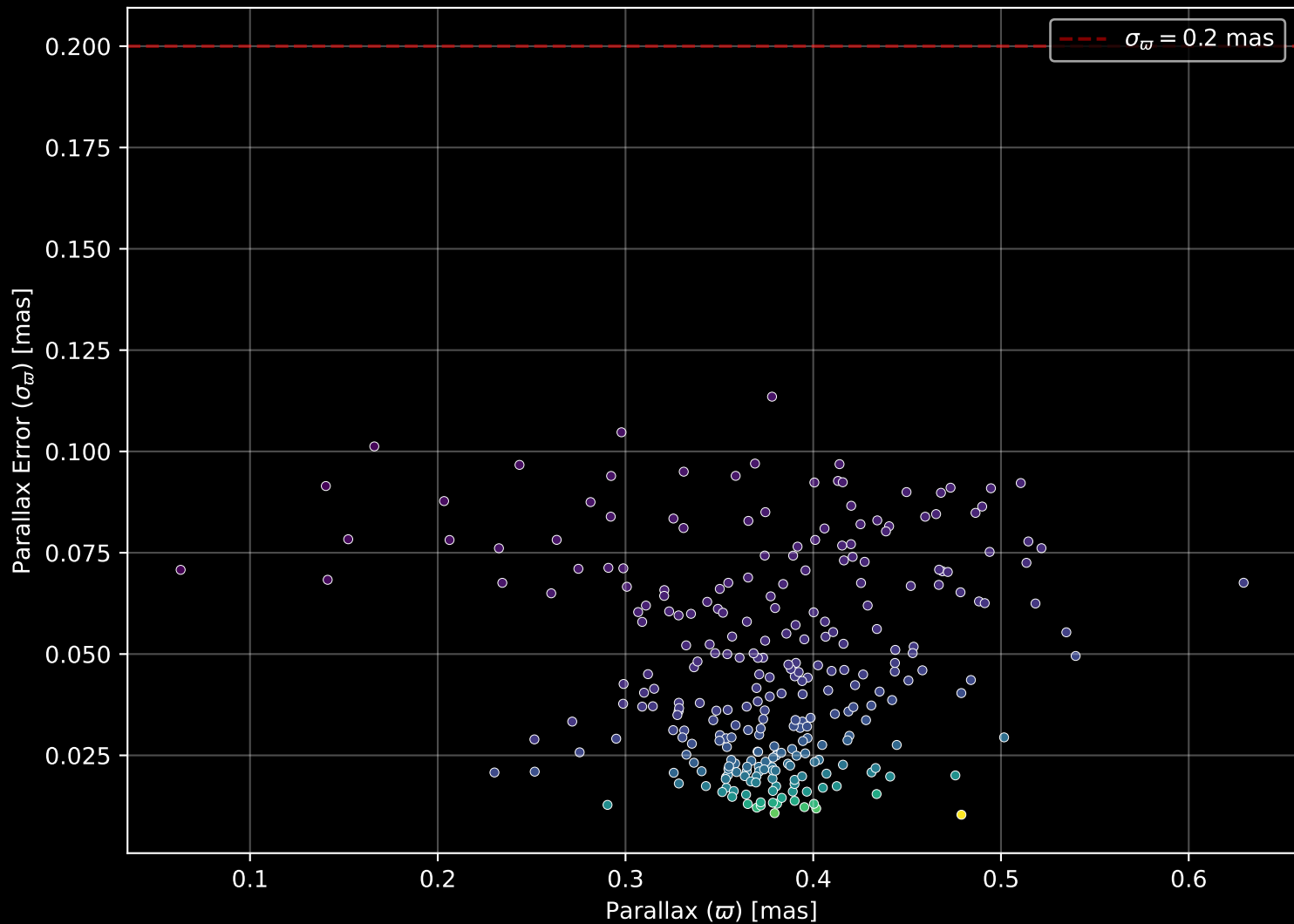
Gaia Cluster: [Ruprecht_18] Parallax Quality (n= 279)
