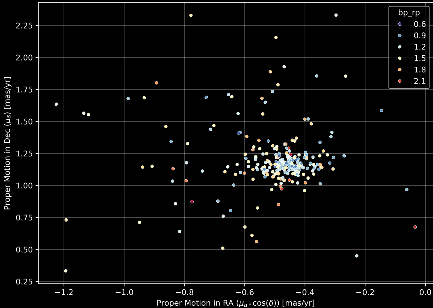
Gaia Cluster: [Ruprecht_18] Proper Motion Diagram (n= 279)
