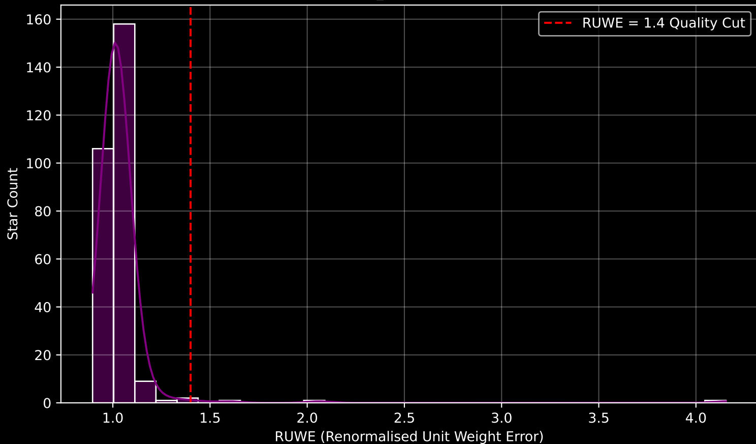
Gaia Cluster: [Ruprecht_18] RUWE Distribution (n= 279)
