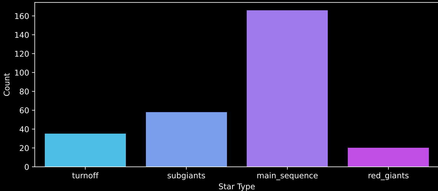
Gaia Cluster: [Ruprecht_18] Count plot of Star Type
