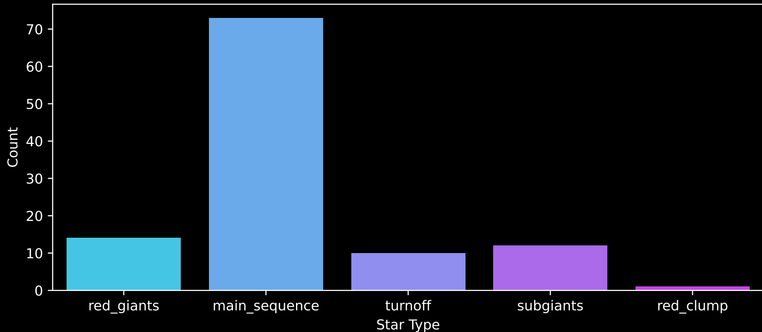
Gaia Cluster: [Ruprecht_32] Count plot of Star Type
