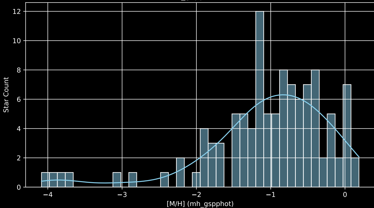
Gaia Cluster: [Ruprecht_32 [M/H] (mh_gspphot) (n= 110)
