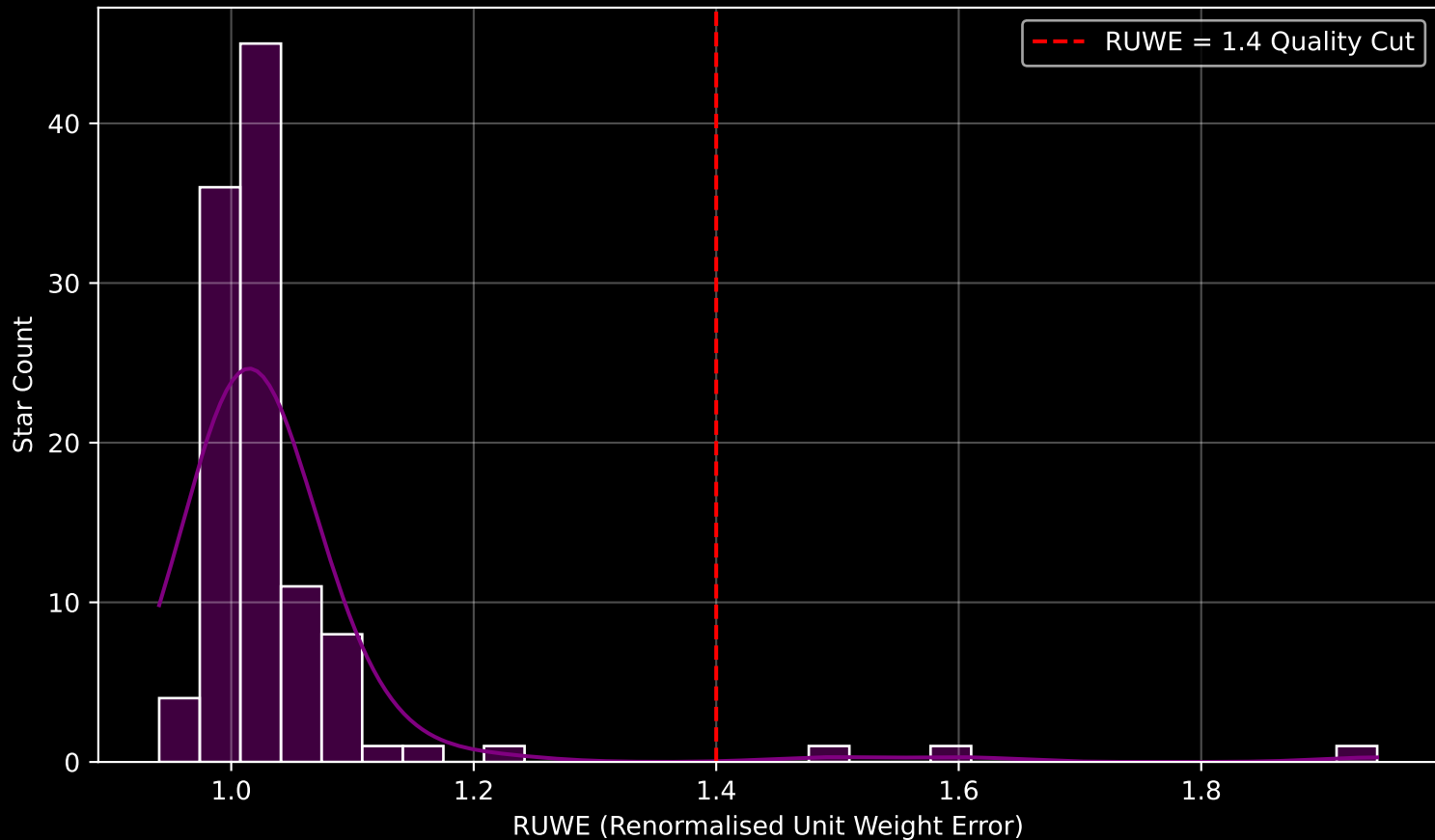
Gaia Cluster: [Ruprecht_32] RUWE Distribution (n= 110)
