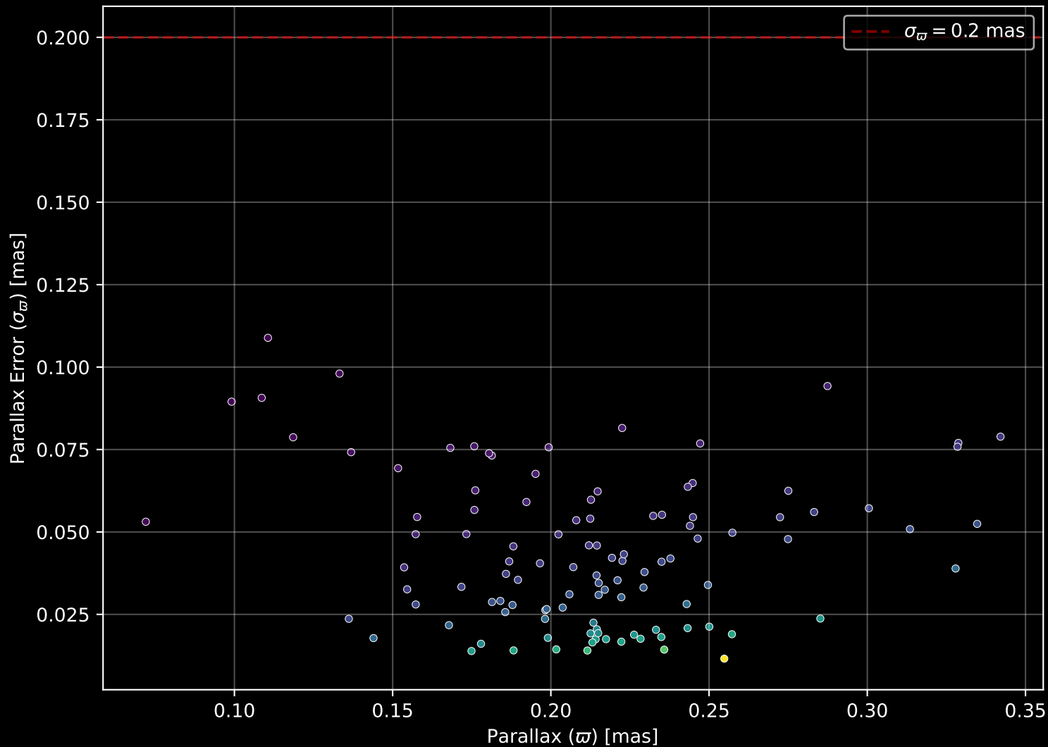
Gaia Cluster: [Ruprecht_32] Parallax Quality (n= 110)
