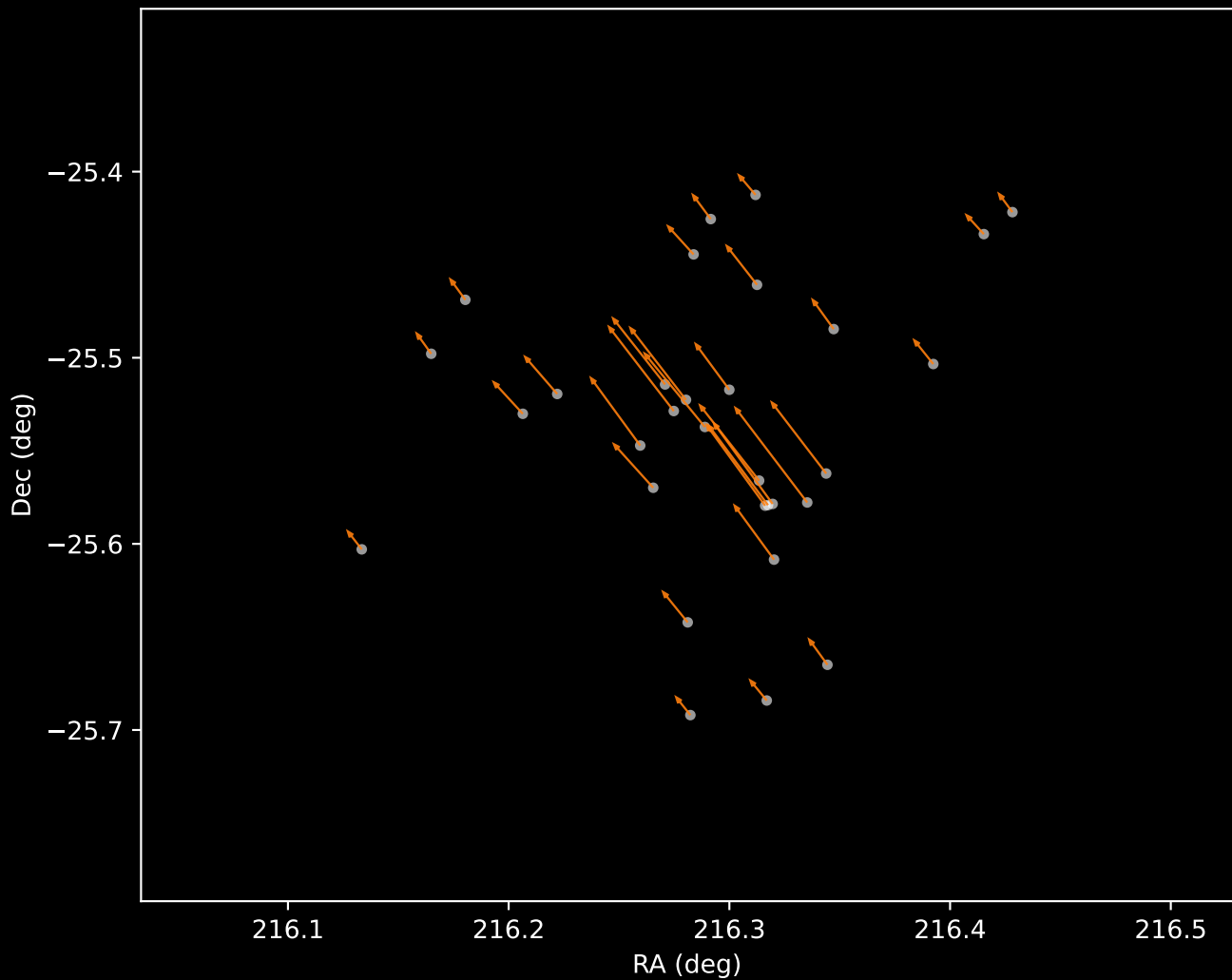
Gaia DR3 Cluster 2 Proper Motion Vectors (n=31)
