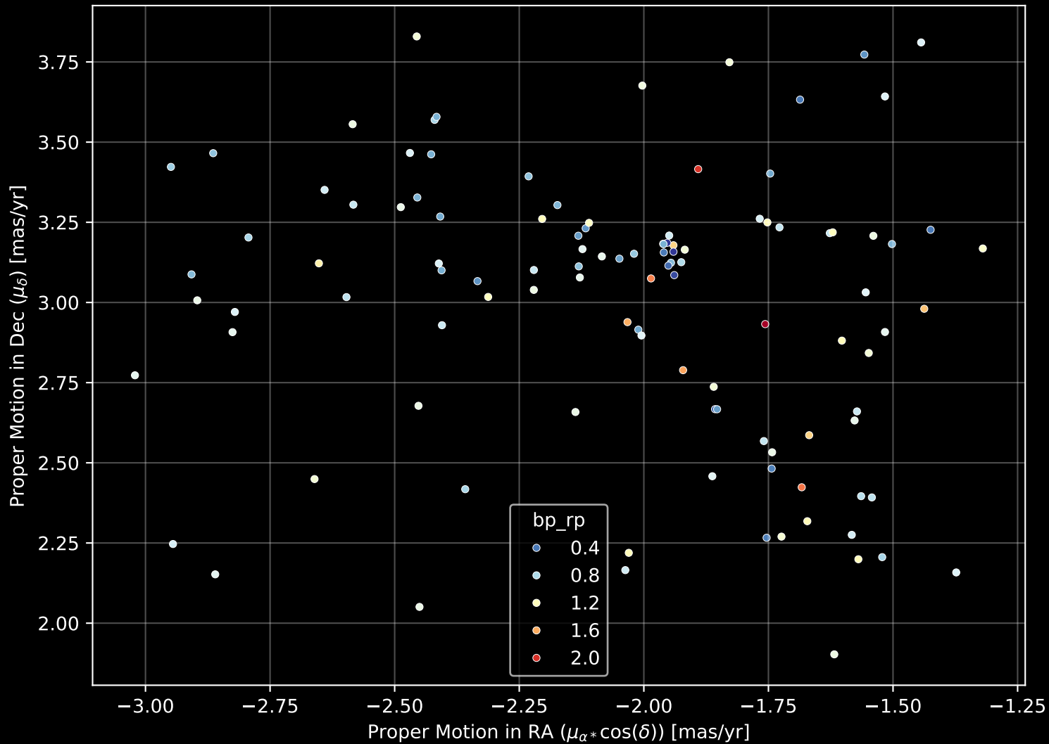
Gaia Cluster: [Ruprecht_32] Proper Motion Diagram (n= 110)
