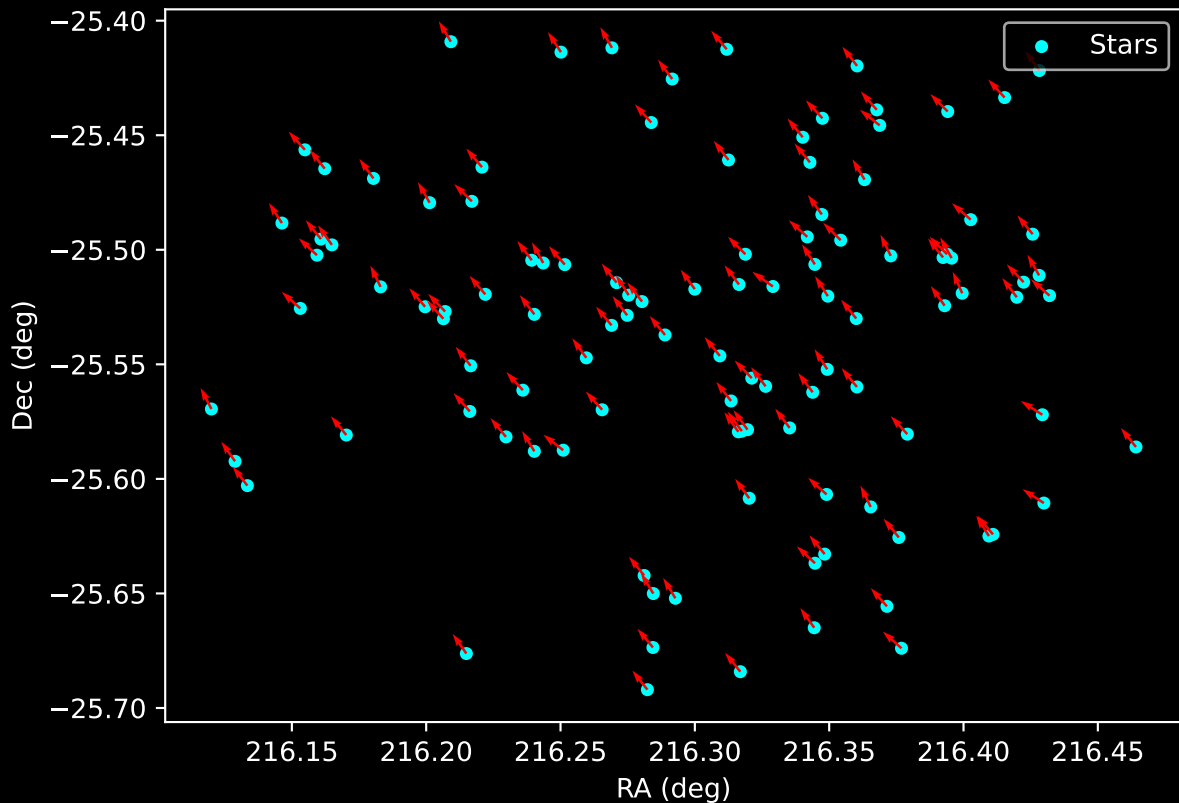
Gaia Cluster: [Ruprecht_32] Proper Motion Vectors for Gaia Star Field (n= 110)
