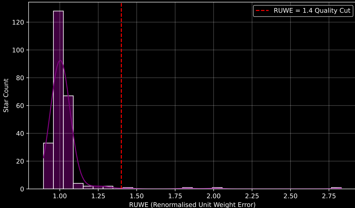
Gaia Cluster: [Ruprecht_33] RUWE Distribution (n= 242)
