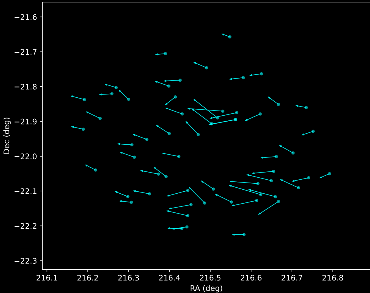
Gaia DR3 Noise Stream Proper Motion Vectors (n=58)
