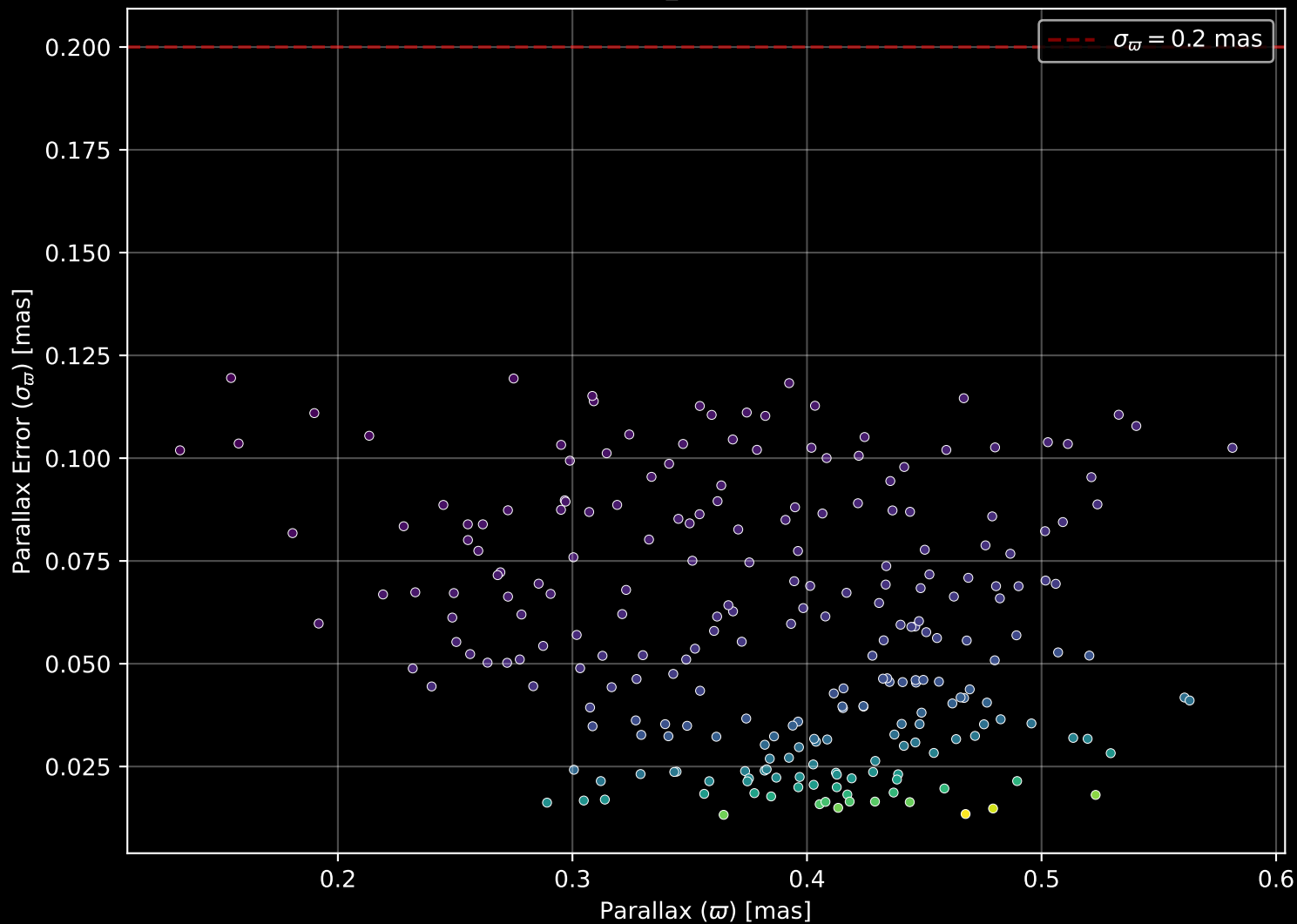
Gaia Cluster: [Ruprecht_33] Parallax Quality (n= 242)
