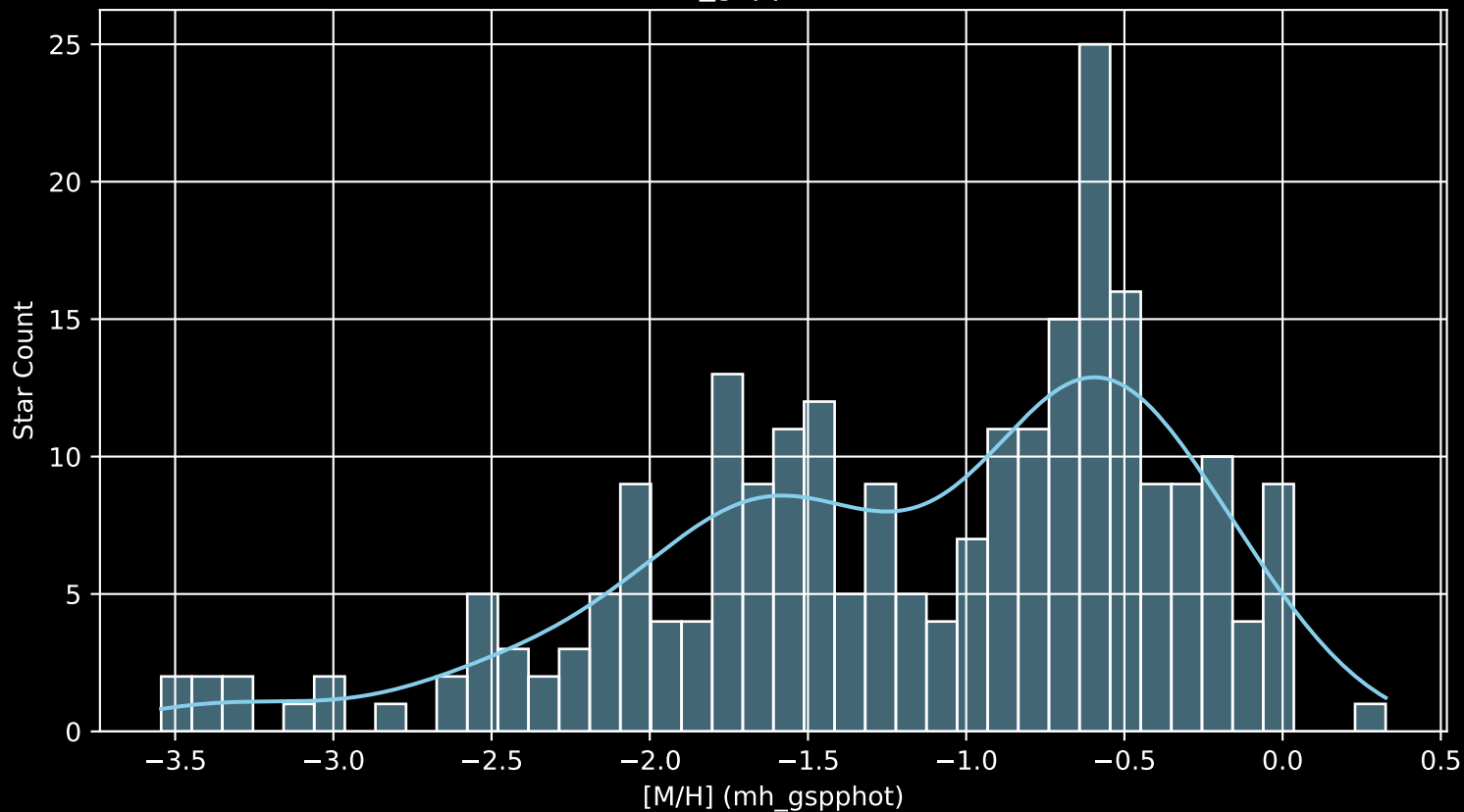
Gaia Cluster: [Ruprecht_33 [M/H] (mh_gspphot) (n= 242)
