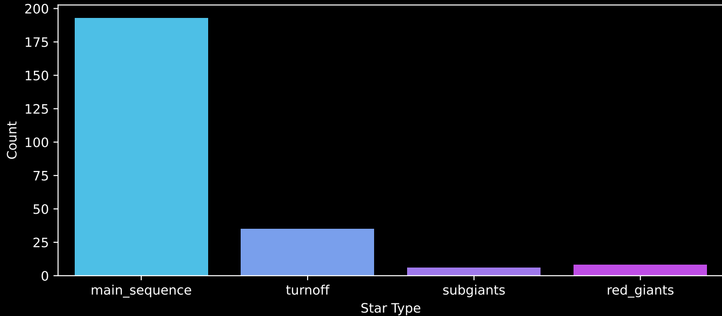
Gaia Cluster: [Ruprecht_33] Count plot of Star Type
