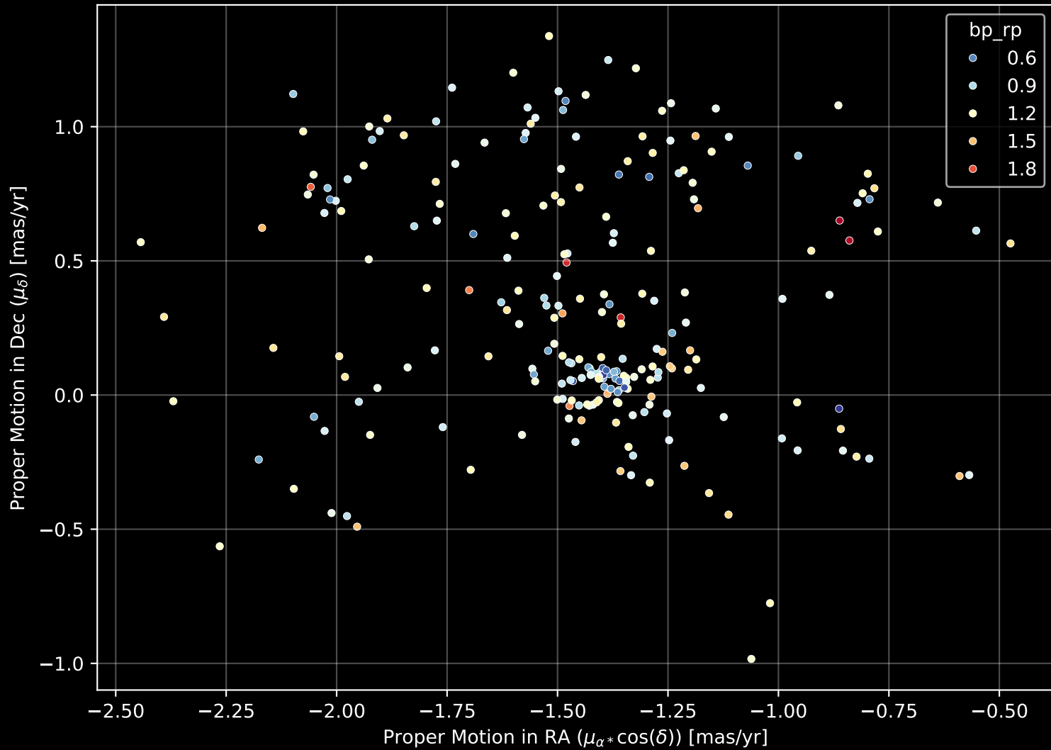
Gaia Cluster: [Ruprecht_33] Proper Motion Diagram (n= 242)
