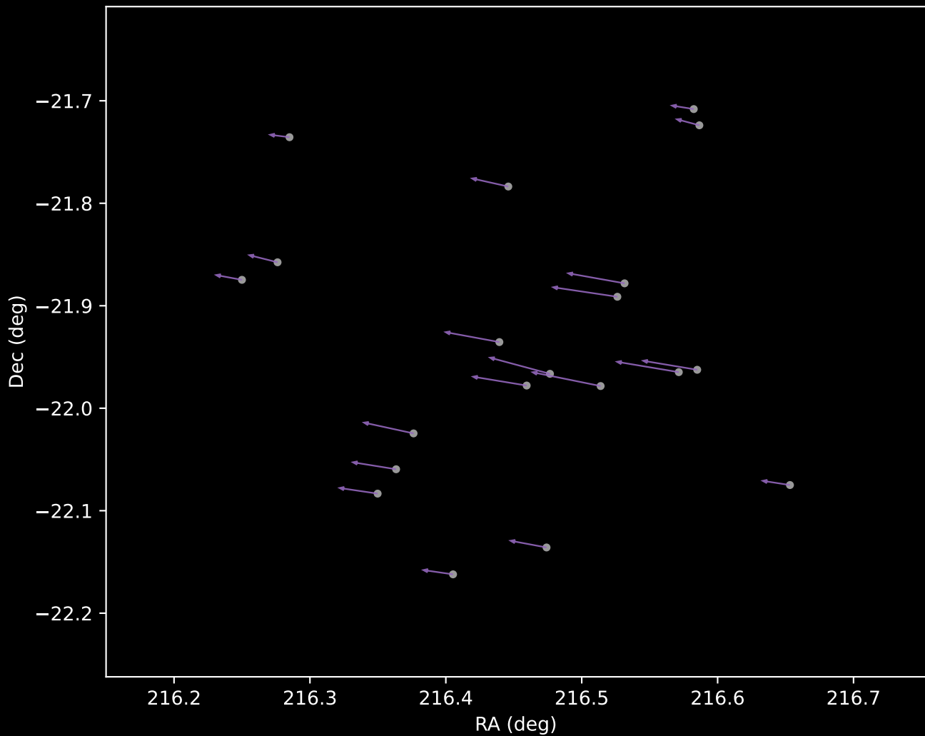
Gaia DR3 Cluster 8 Proper Motion Vectors (n=20)
