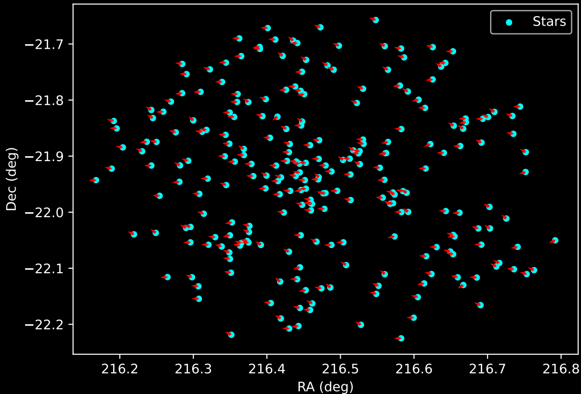
Gaia Cluster: [Ruprecht_33] Proper Motion Vectors for Gaia Star Field (n= 242)
