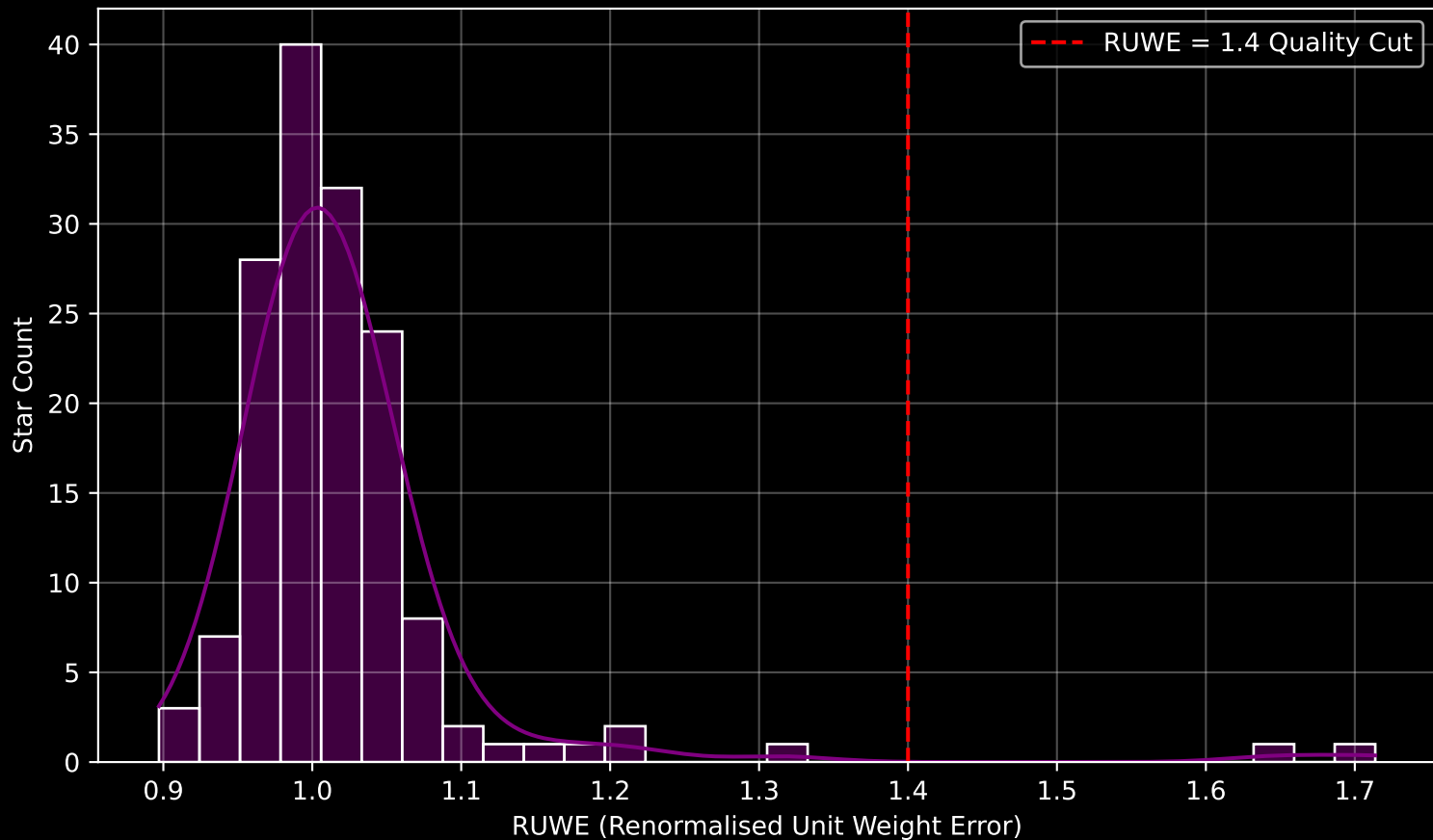
Gaia Cluster: [Ruprecht_36] RUWE Distribution (n= 152)
