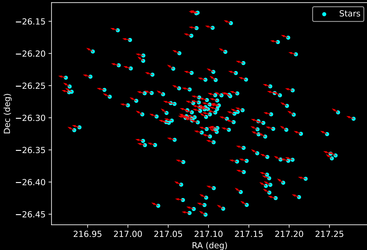
Gaia Cluster: [Ruprecht_36] Proper Motion Vectors for Gaia Star Field (n= 152)
