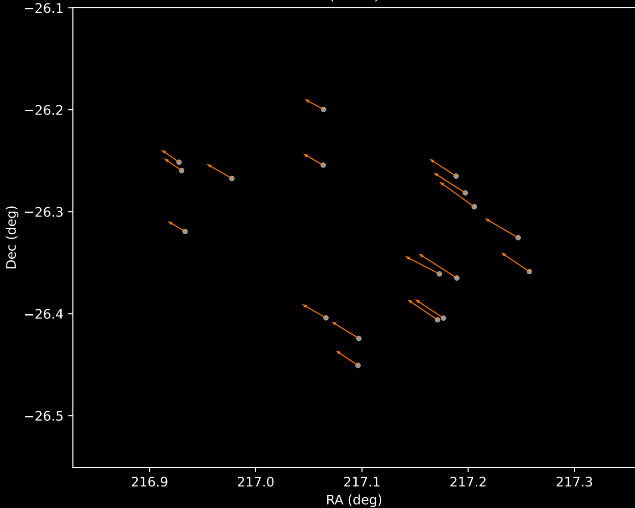
Gaia DR3 Cluster 2 Proper Motion Vectors (n=18)
