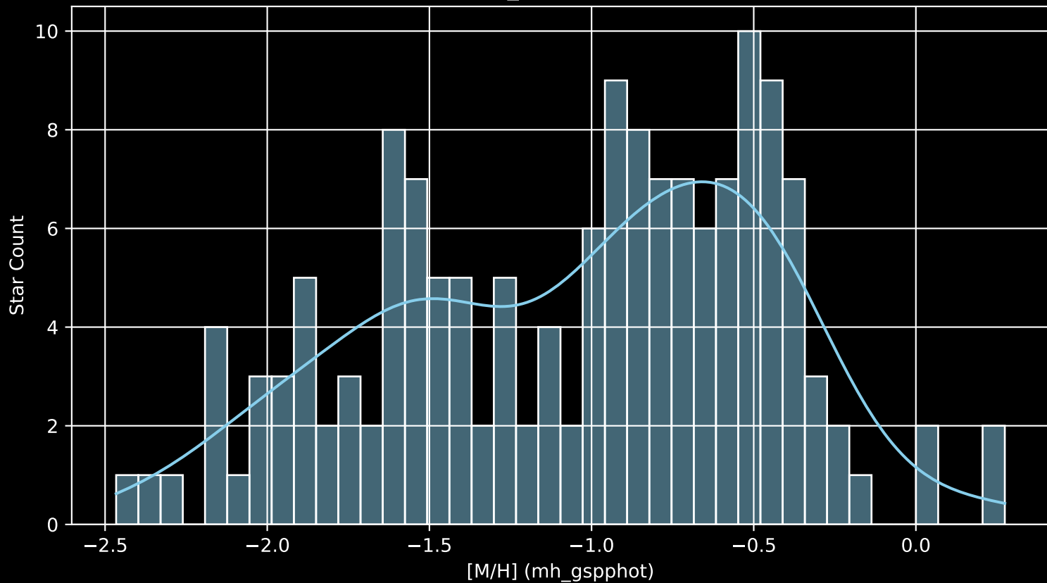
Gaia Cluster: [Ruprecht_36 [M/H] (mh_gspphot) (n= 152)
