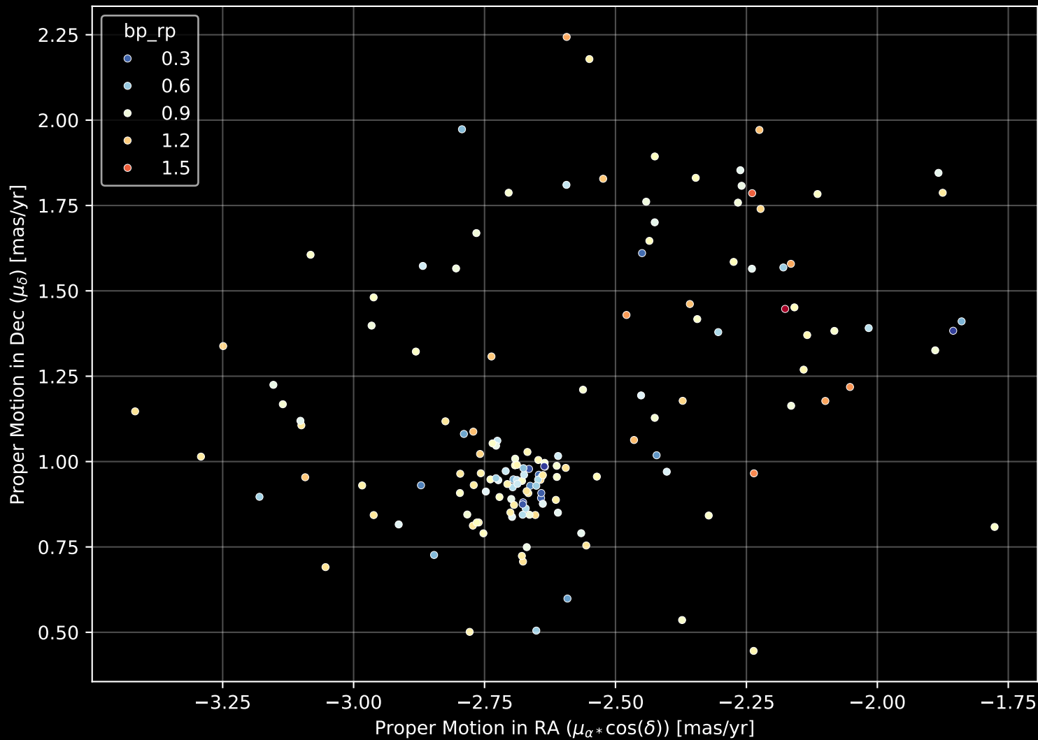
Gaia Cluster: [Ruprecht_36] Proper Motion Diagram (n= 152)
