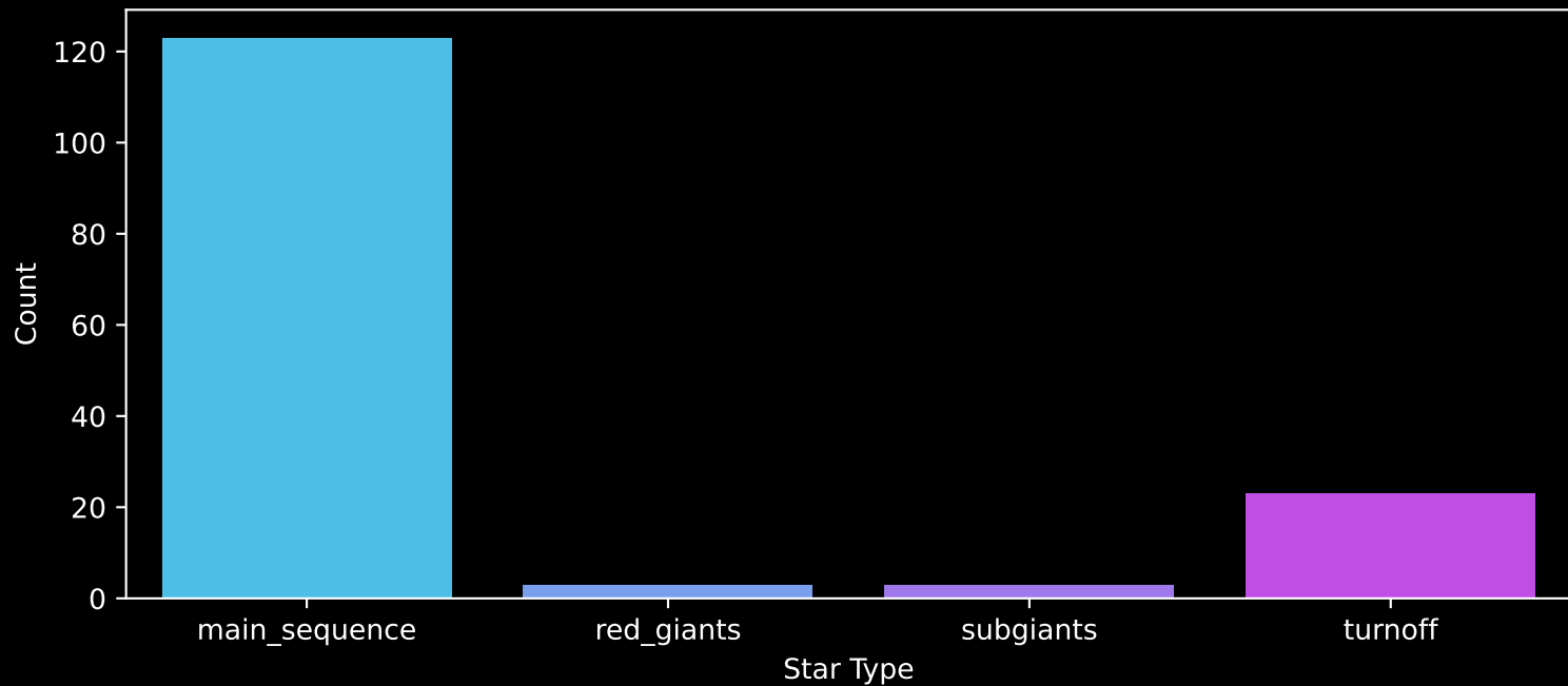
Gaia Cluster: [Ruprecht_36] Count plot of Star Type
