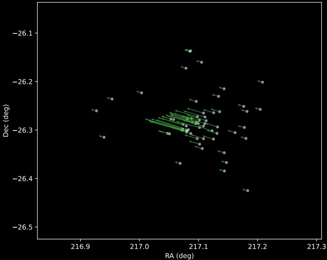
Gaia DR3 Cluster 4 Proper Motion Vectors (n=61)
