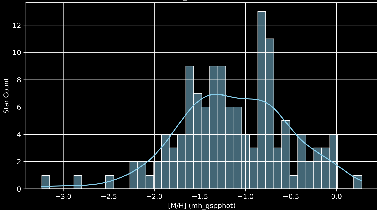
Gaia Cluster: [Ruprecht_37 [M/H] (mh_gspphot) (n= 130)
