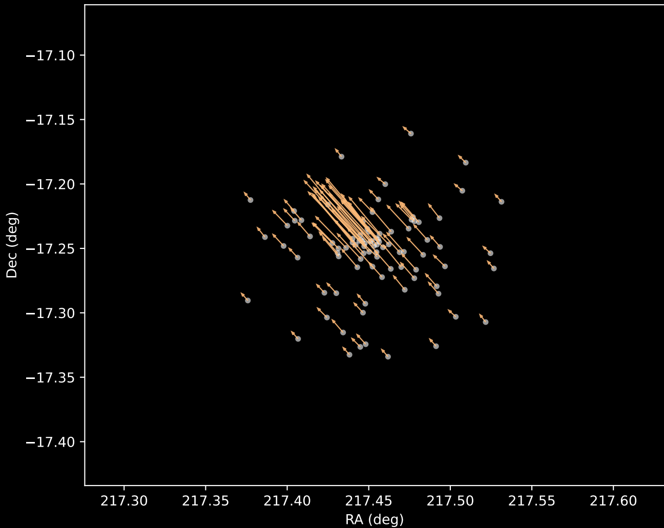
Gaia DR3 Cluster 3 Proper Motion Vectors (n=90)
