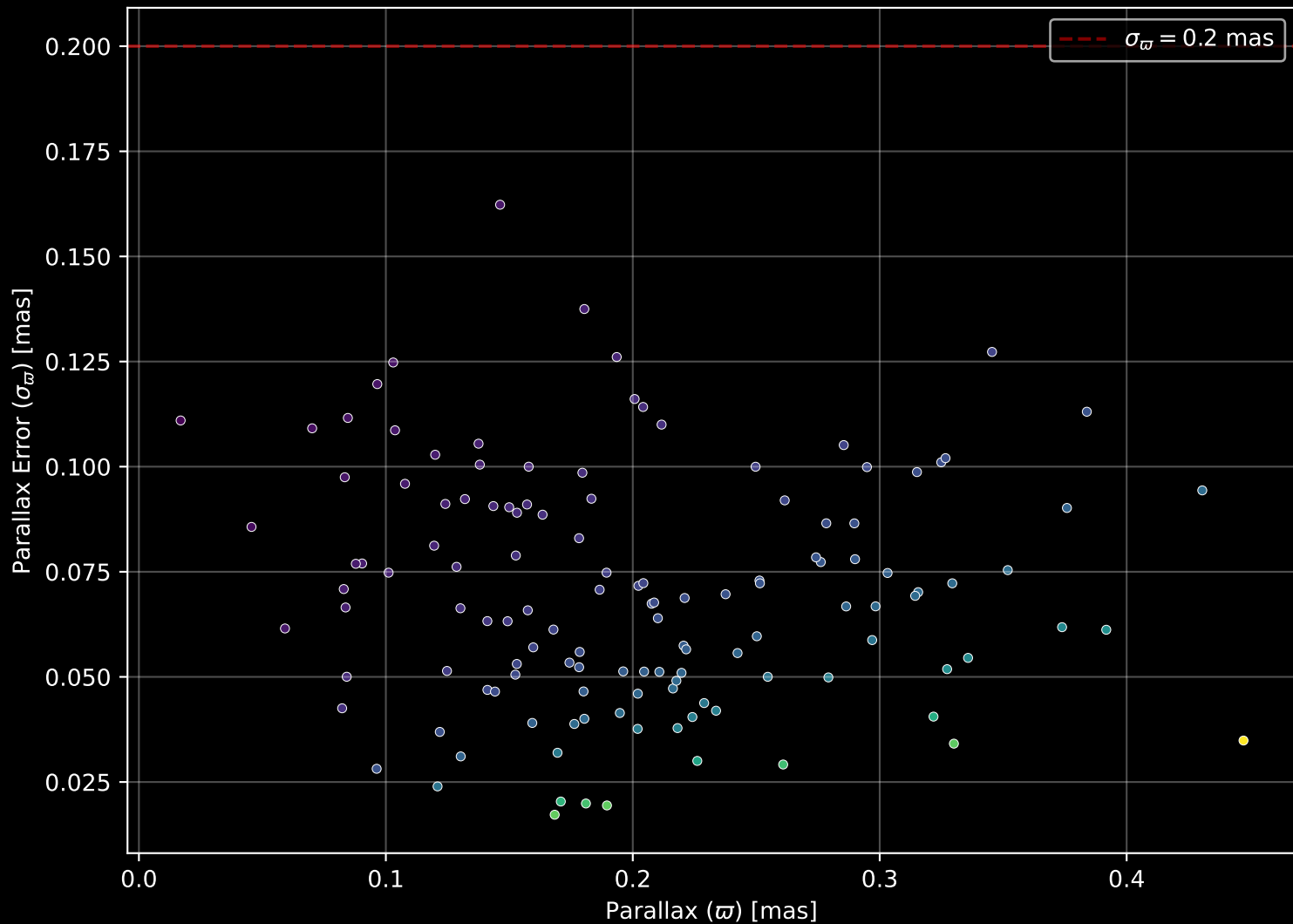
Gaia Cluster: [Ruprecht_37] Parallax Quality (n= 130)
