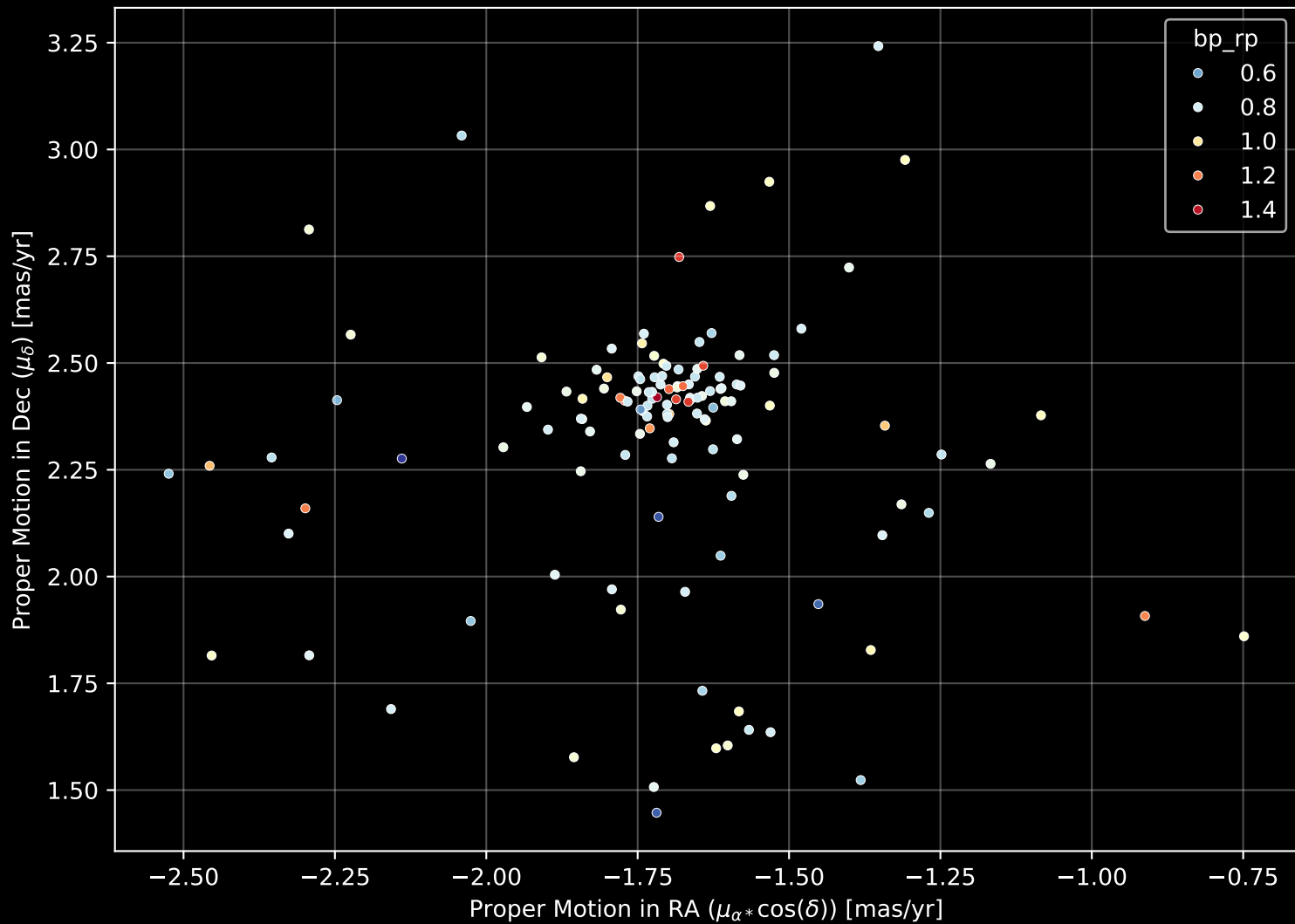
Gaia Cluster: [Ruprecht_37] Proper Motion Diagram (n= 130)
