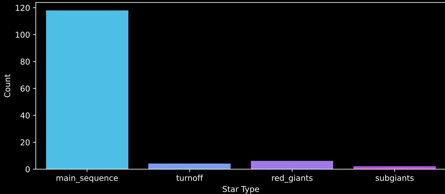
Gaia Cluster: [Ruprecht_37] Count plot of Star Type
