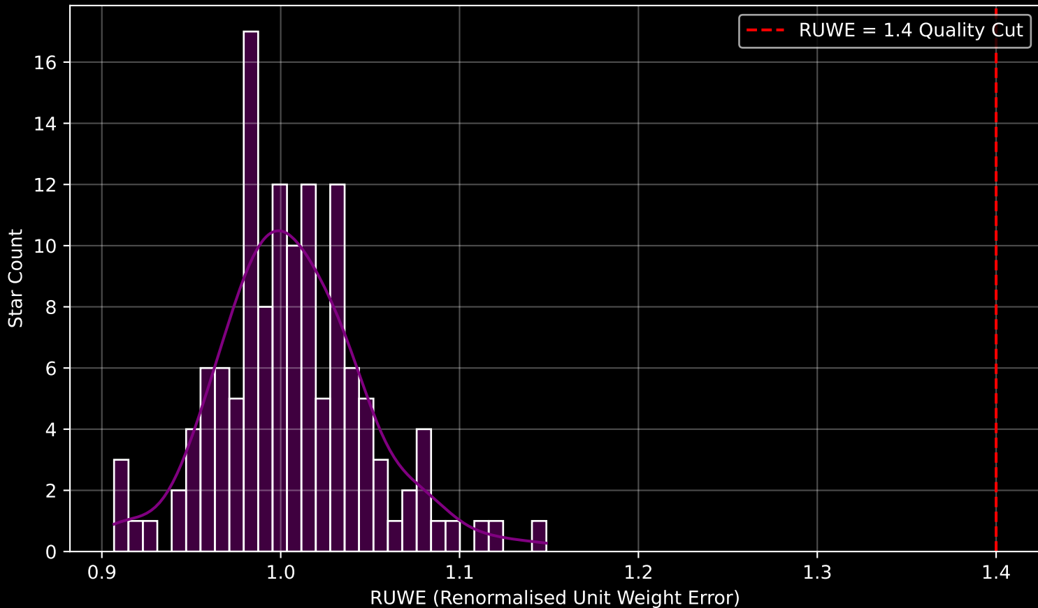
Gaia Cluster: [Ruprecht_37] RUWE Distribution (n= 130)
