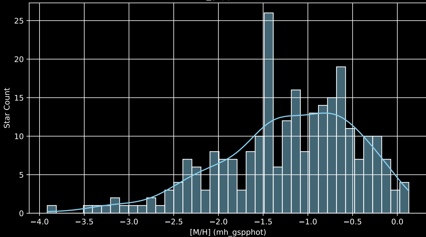
Gaia Cluster: [Ruprecht_42 [M/H] (mh_gspphot) (n= 259)
