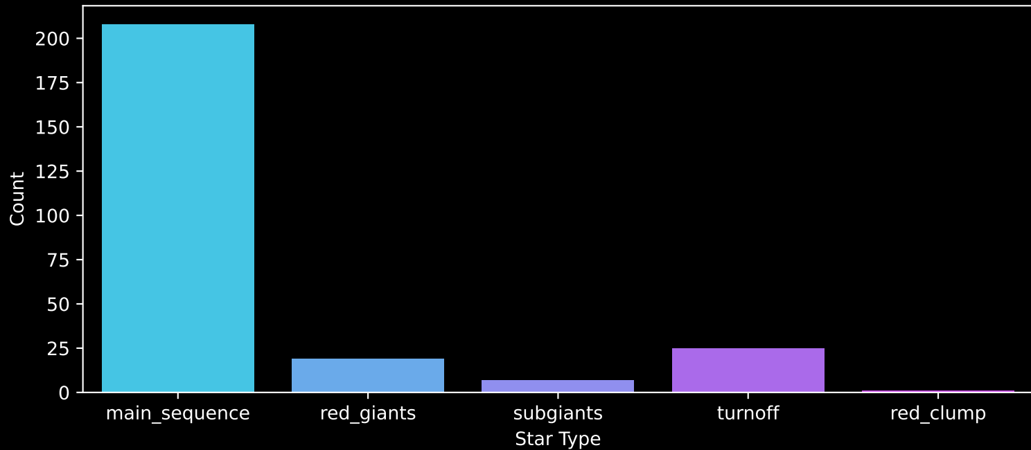
Gaia Cluster: [Ruprecht_42] Count plot of Star Type
