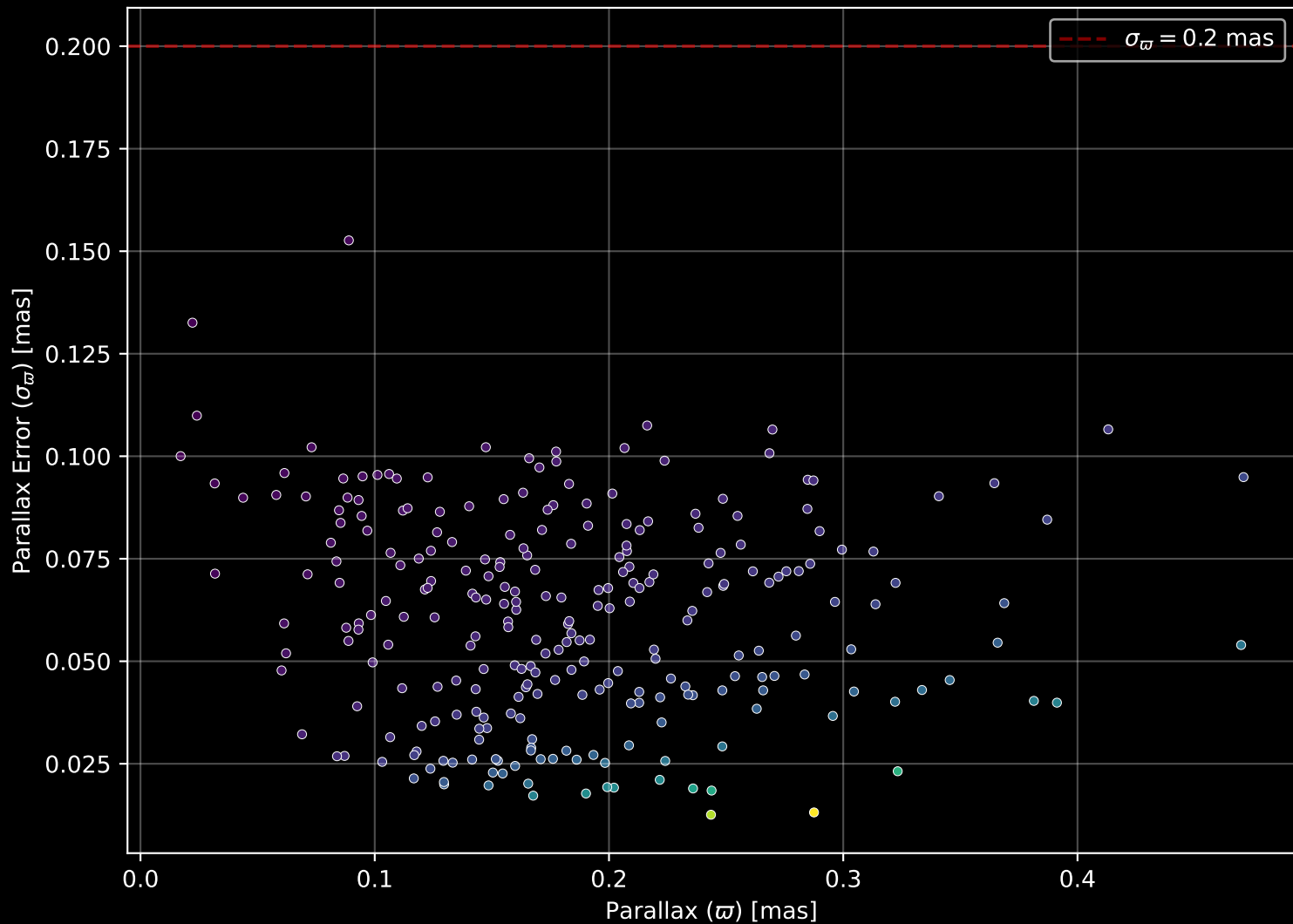
Gaia Cluster: [Ruprecht_42] Parallax Quality (n= 260)
