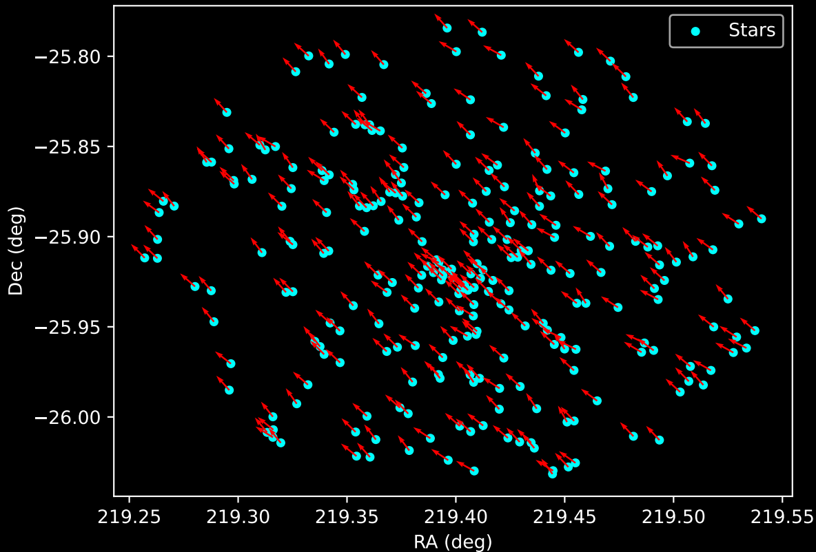
Gaia Cluster: [Ruprecht_42] Proper Motion Vectors for Gaia Star Field (n= 260)
