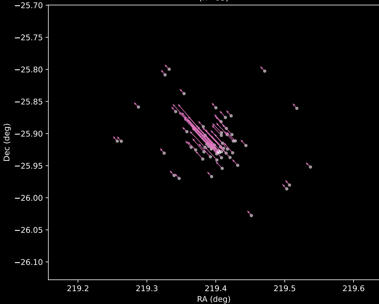
Gaia DR3 Cluster 12 Proper Motion Vectors (n=63)
