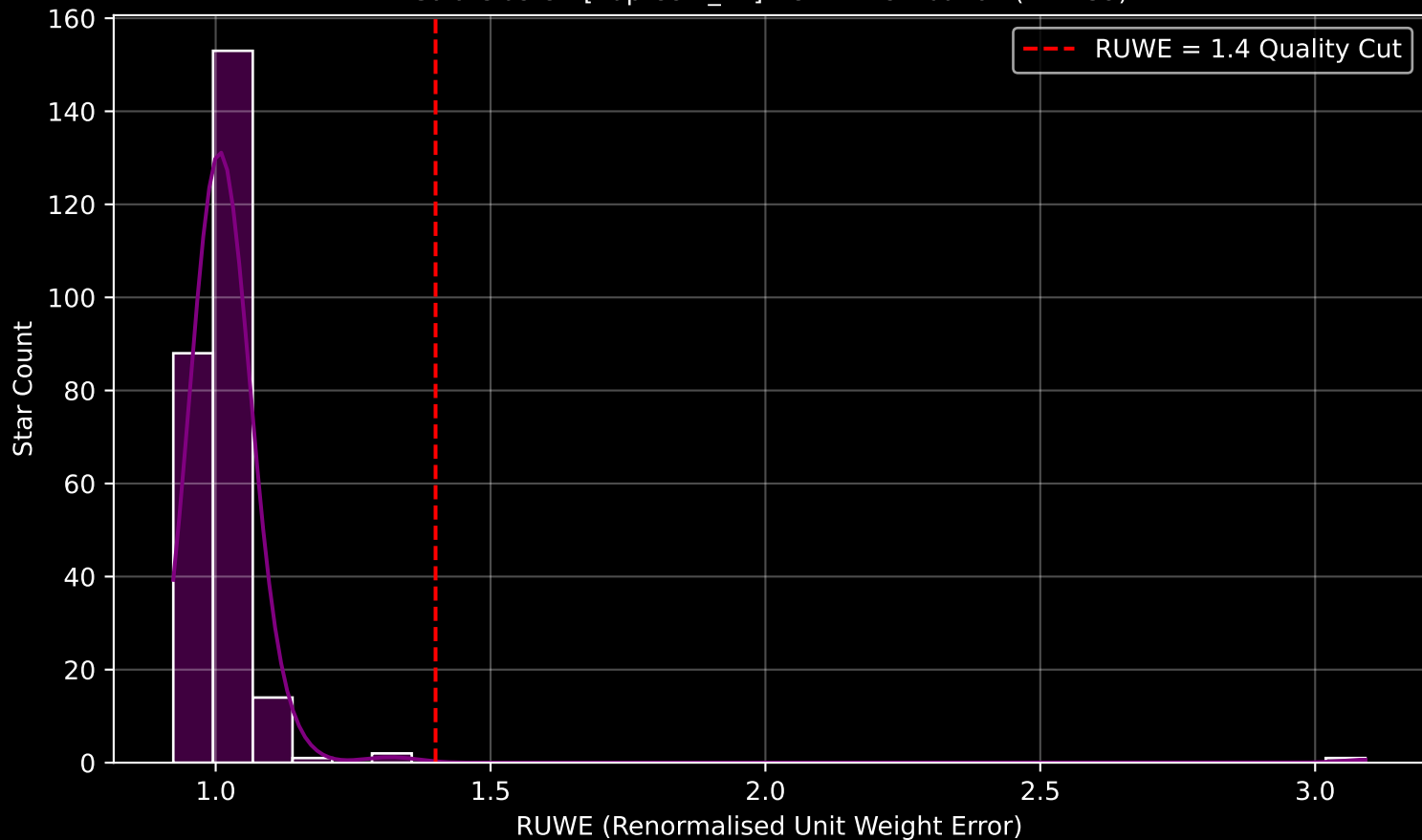
Gaia Cluster: [Ruprecht_42] RUWE Distribution (n= 259)
