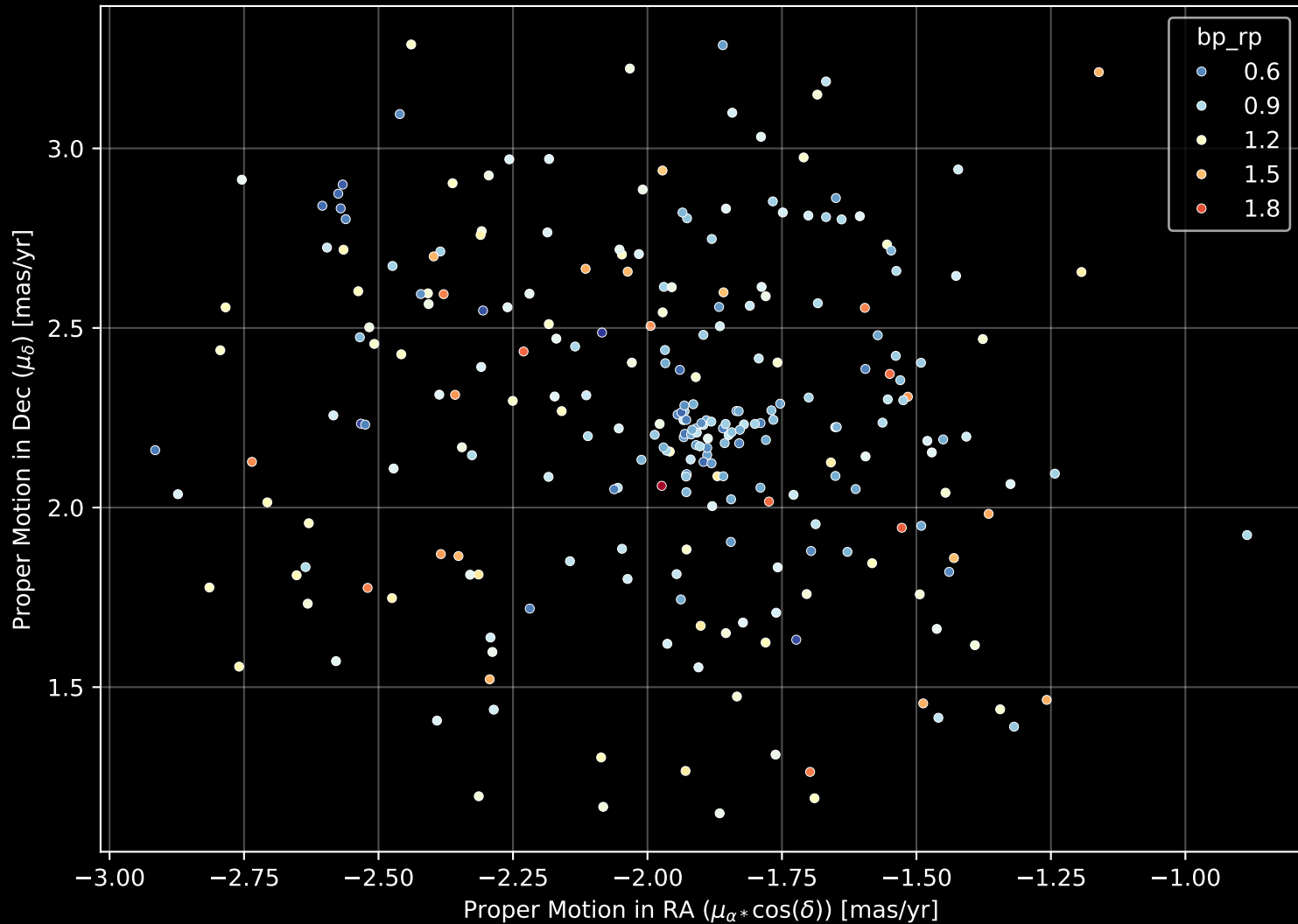
Gaia Cluster: [Ruprecht_42] Proper Motion Diagram (n= 260)
