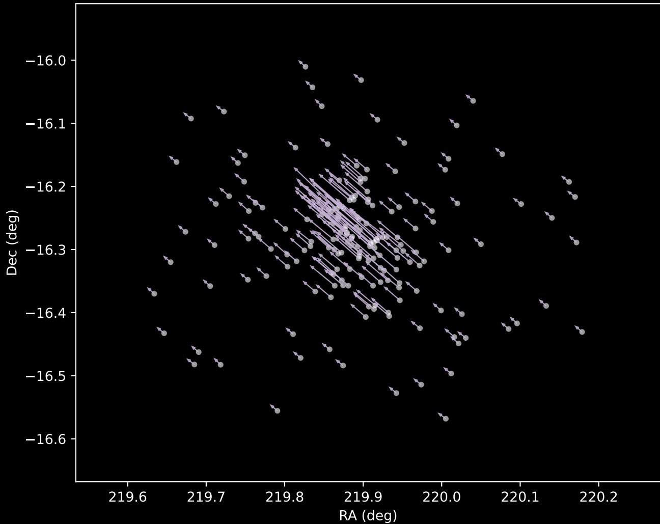
Gaia DR3 Cluster 9 Proper Motion Vectors (n=178)
