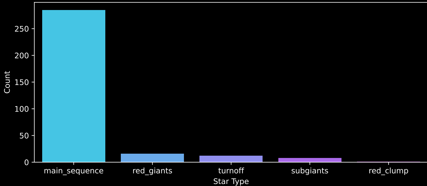
Gaia Cluster: [Ruprecht_45] Count plot of Star Type
