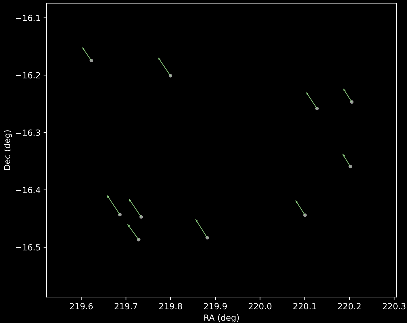
Gaia DR3 Cluster 5 Proper Motion Vectors (n=10)
