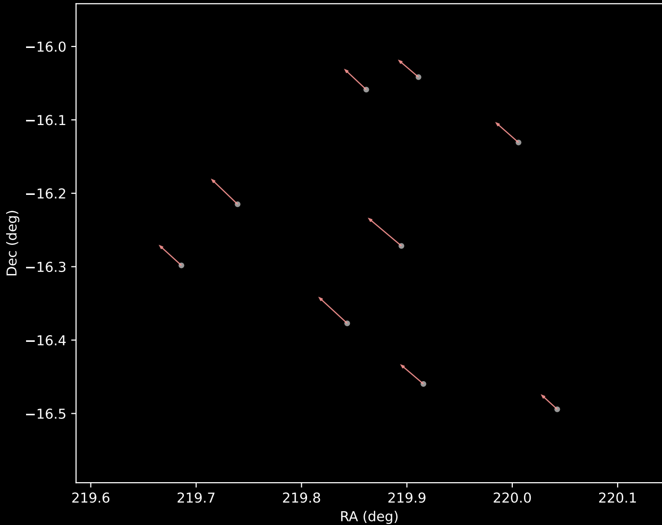
Gaia DR3 Cluster 7 Proper Motion Vectors (n=9)
