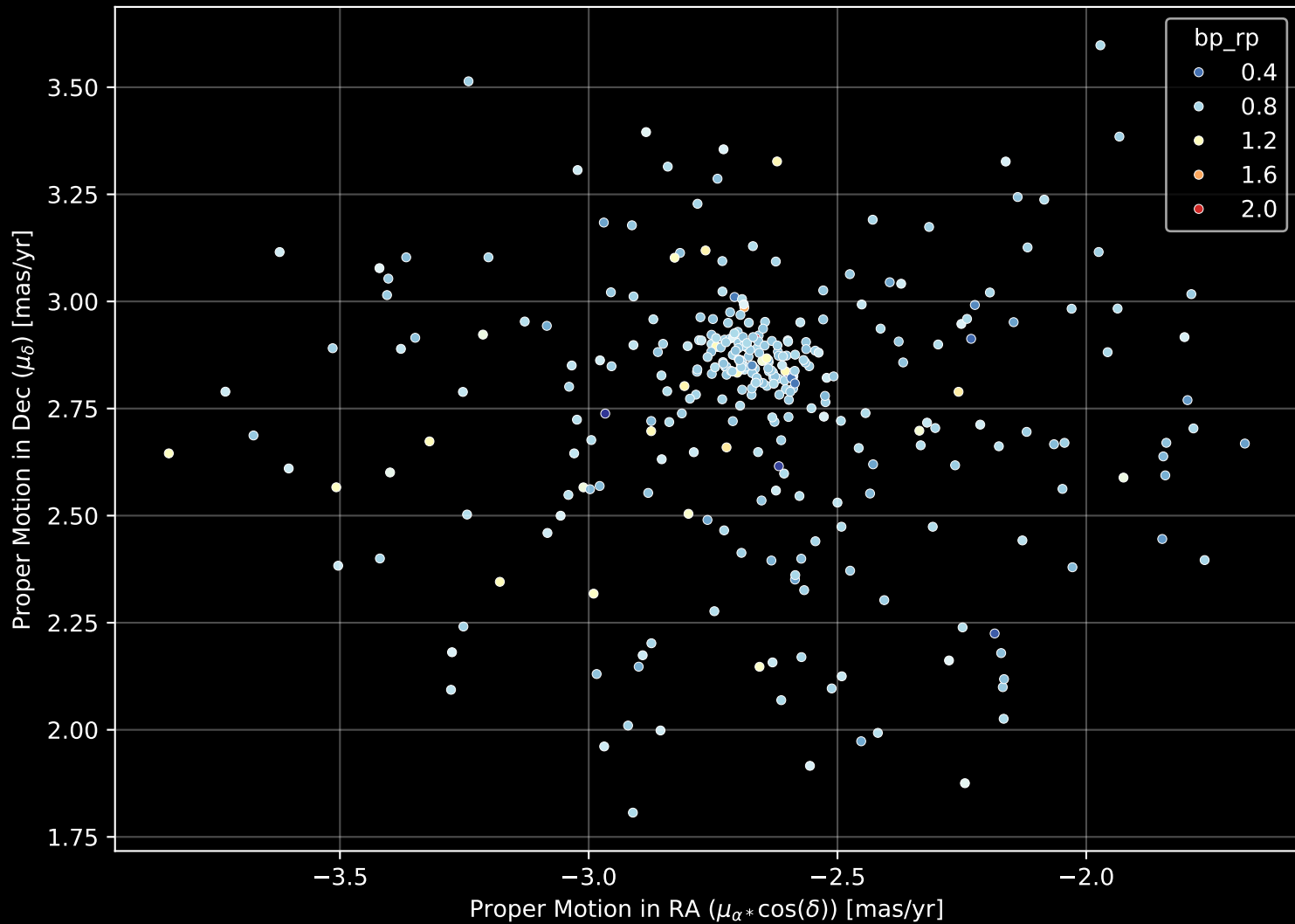
Gaia Cluster: [Ruprecht_45] Proper Motion Diagram (n= 322)
