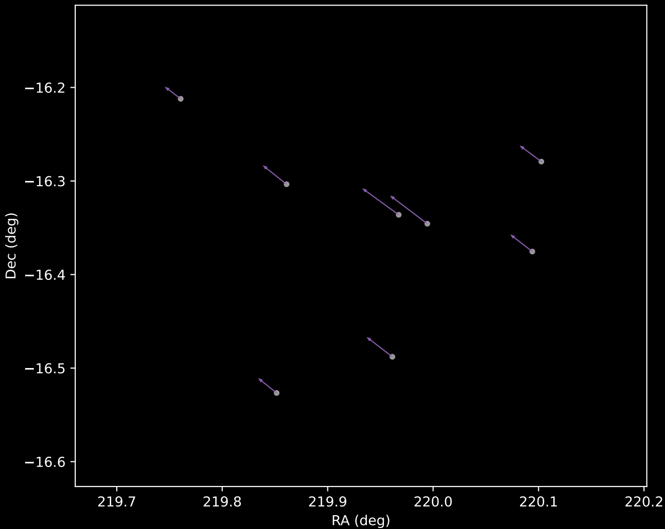
Gaia DR3 Cluster 8 Proper Motion Vectors (n=8)
