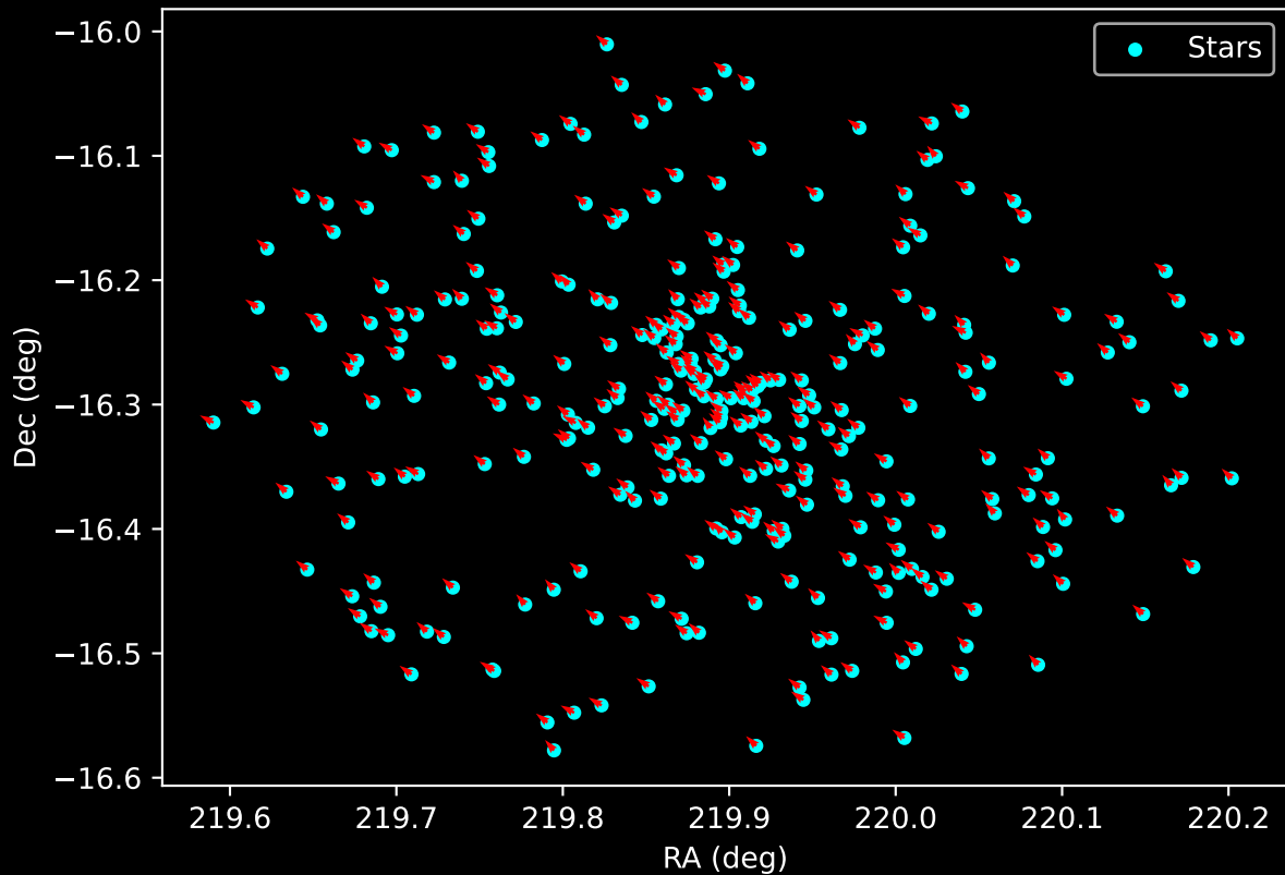
Gaia Cluster: [Ruprecht_45] Proper Motion Vectors for Gaia Star Field (n= 322)
