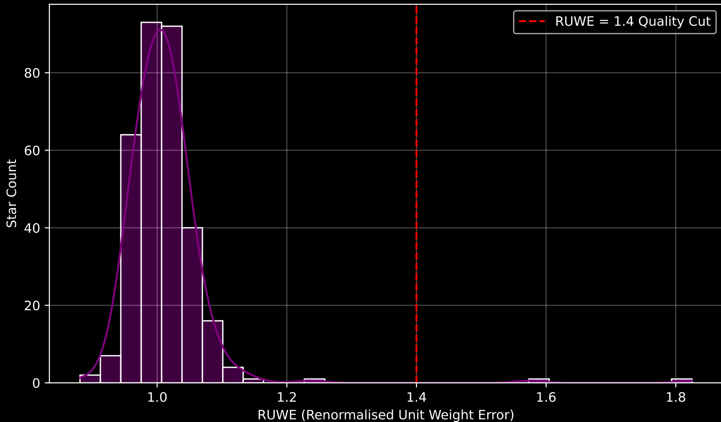
Gaia Cluster: [Ruprecht_45] RUWE Distribution (n= 322)
