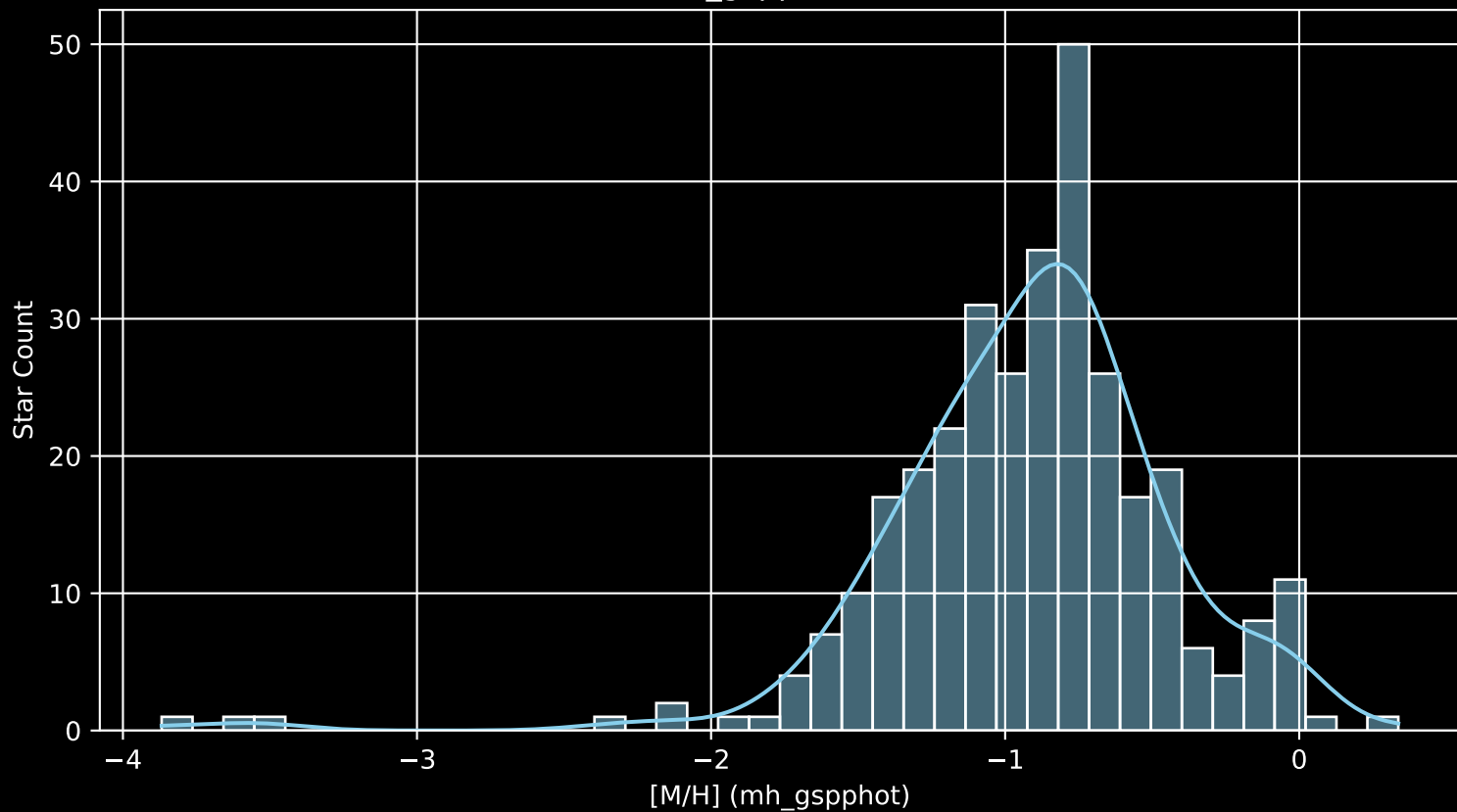
Gaia Cluster: [Ruprecht_45 [M/H] (mh_gspphot) (n= 322)
