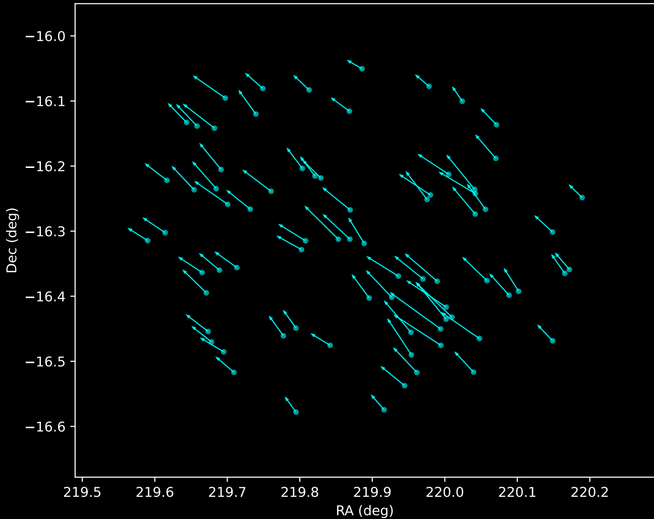
Gaia DR3 Noise Stream Proper Motion Vectors (n=75)
