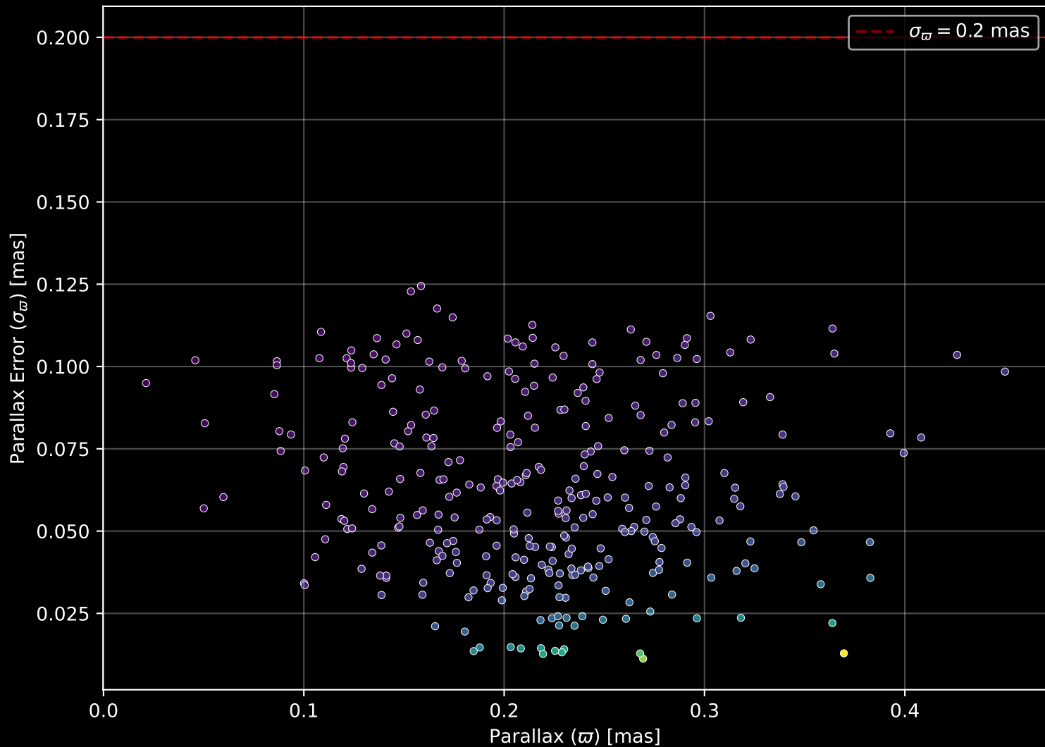
Gaia Cluster: [Ruprecht_45] Parallax Quality (n= 322)
