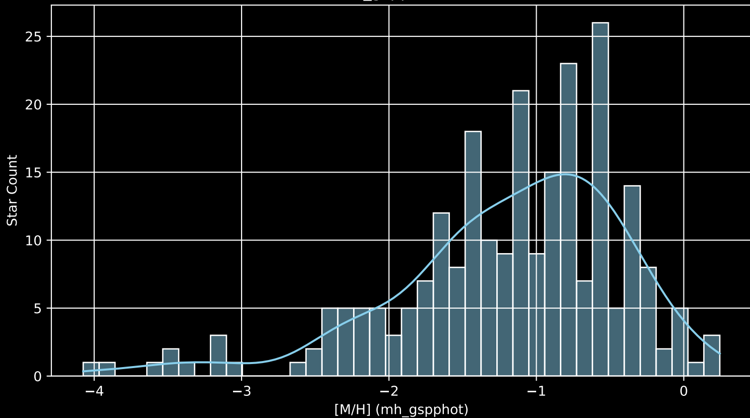
Gaia Cluster: [Ruprecht_47 [M/H] (mh_gspphot) (n= 244)
