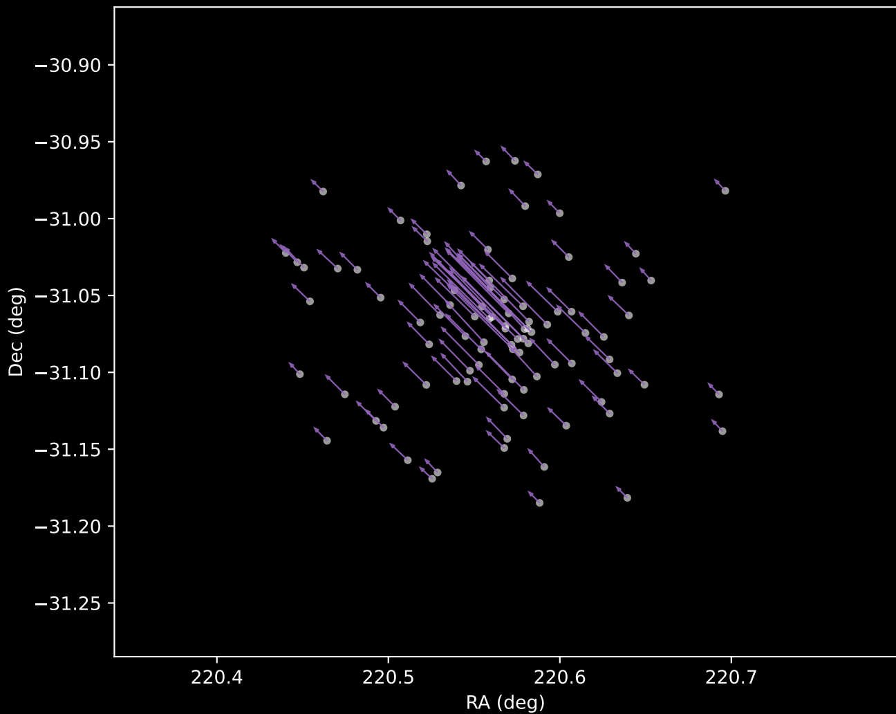
Gaia DR3 Cluster 8 Proper Motion Vectors (n=94)
