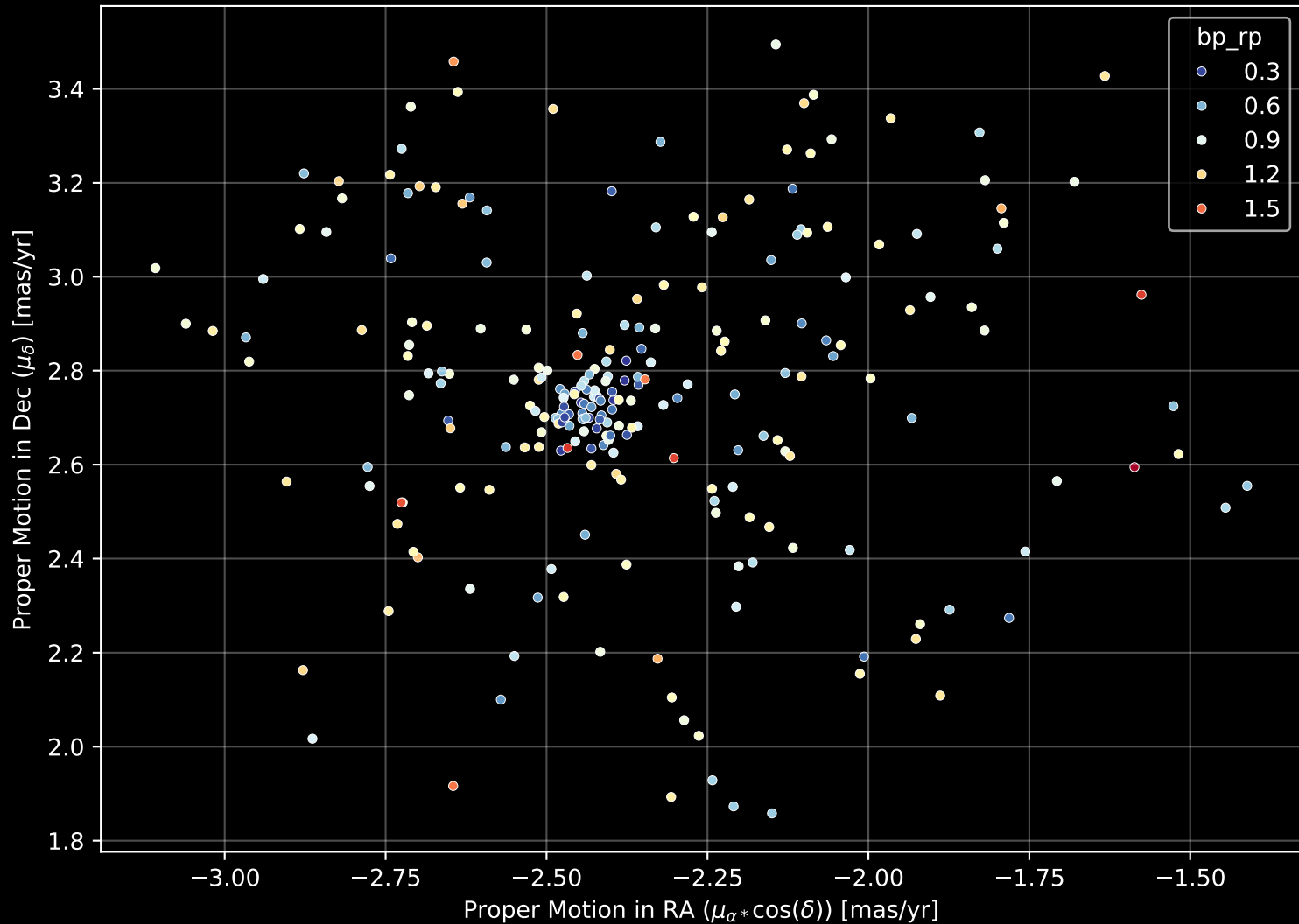
Gaia Cluster: [Ruprecht_47] Proper Motion Diagram (n= 245)
