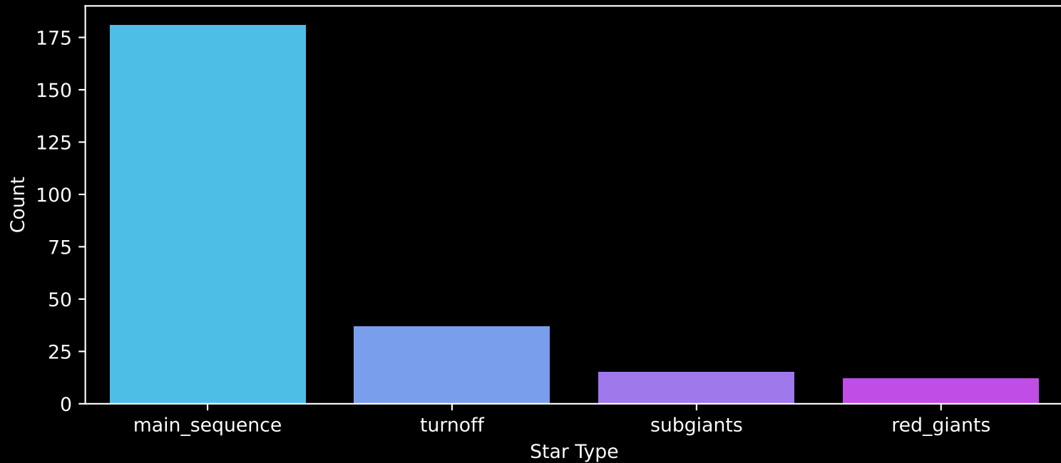
Gaia Cluster: [Ruprecht_47] Count plot of Star Type
