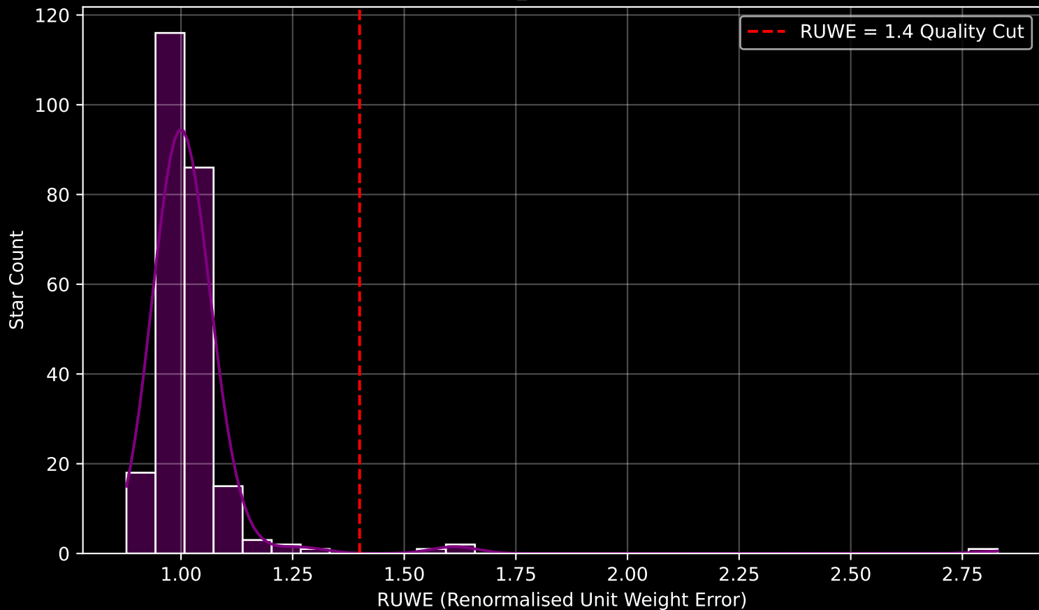
Gaia Cluster: [Ruprecht_47] RUWE Distribution (n= 245)
