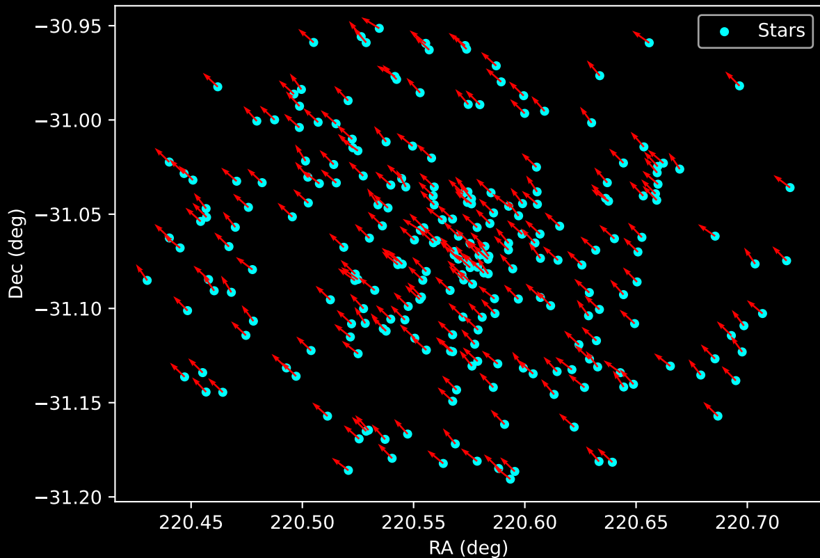
Gaia Cluster: [Ruprecht_47] Proper Motion Vectors for Gaia Star Field (n= 245)
