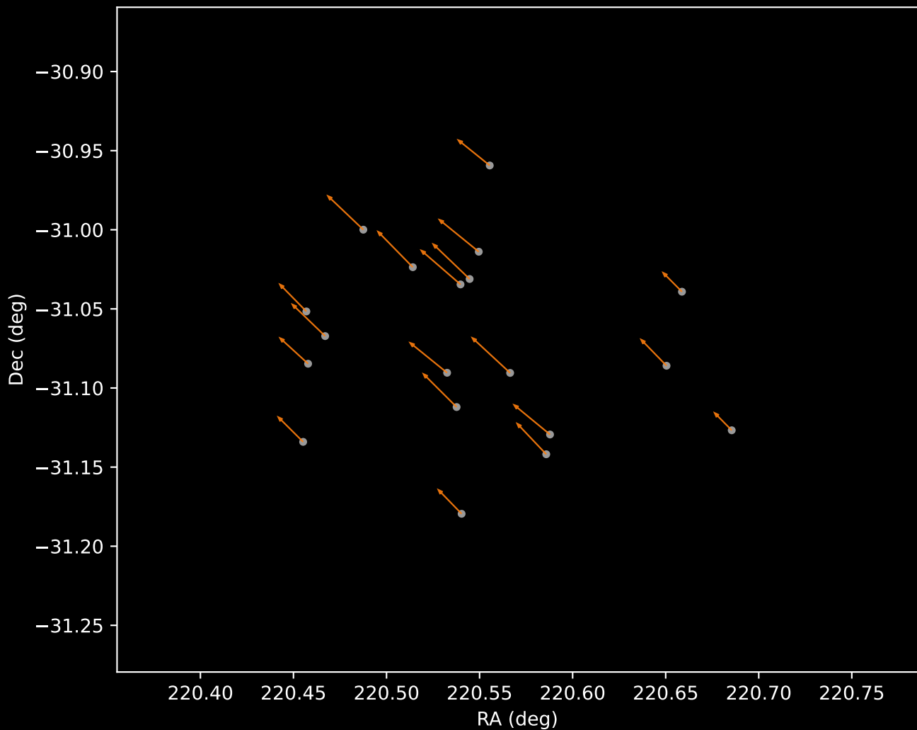
Gaia DR3 Cluster 2 Proper Motion Vectors (n=19)
