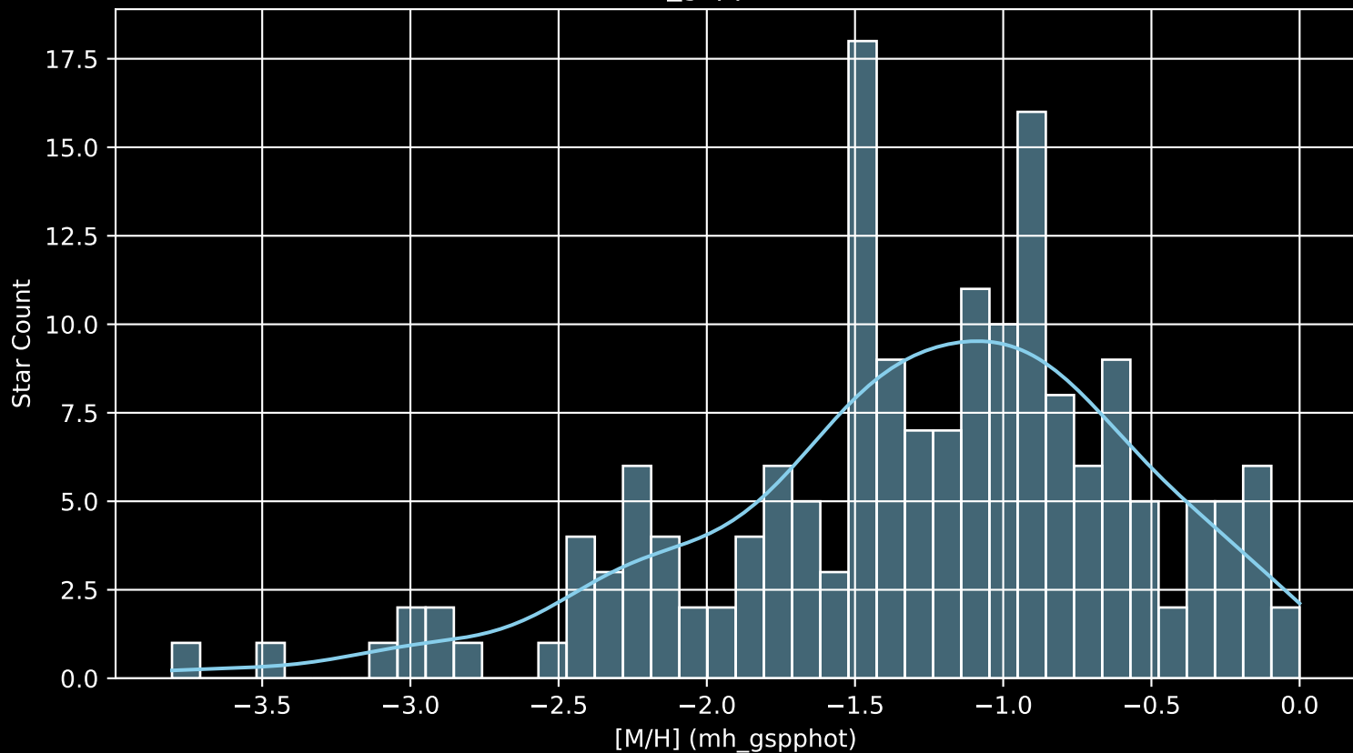
Gaia Cluster: [Ruprecht_48 [M/H] (mh_gspphot) (n= 174)
