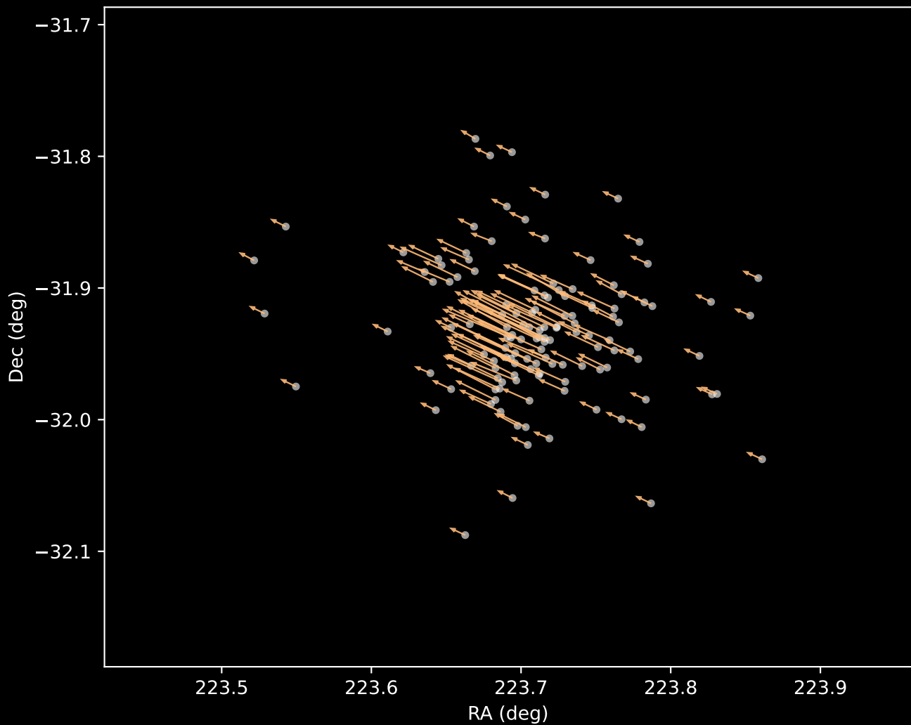
Gaia DR3 Cluster 3 Proper Motion Vectors (n=131)
