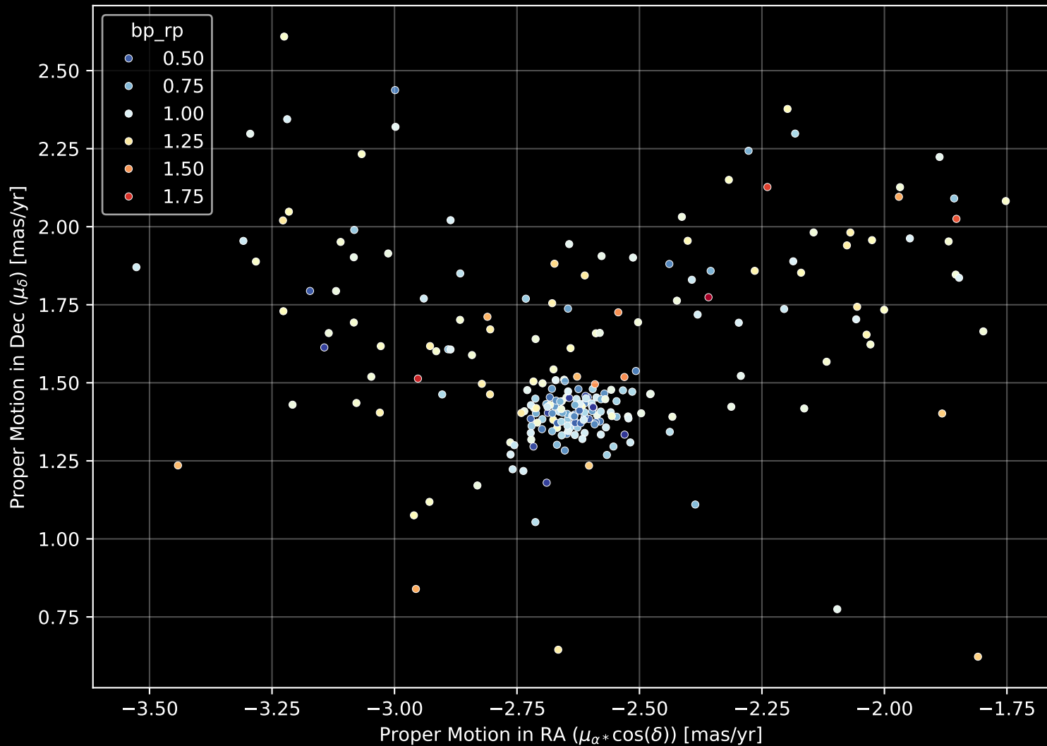
Gaia Cluster: [Ruprecht_58] Proper Motion Diagram (n= 234)
