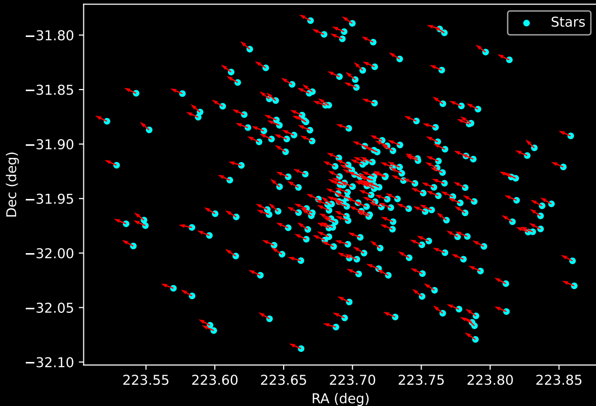
Gaia Cluster: [Ruprecht_58] Proper Motion Vectors for Gaia Star Field (n= 234)
