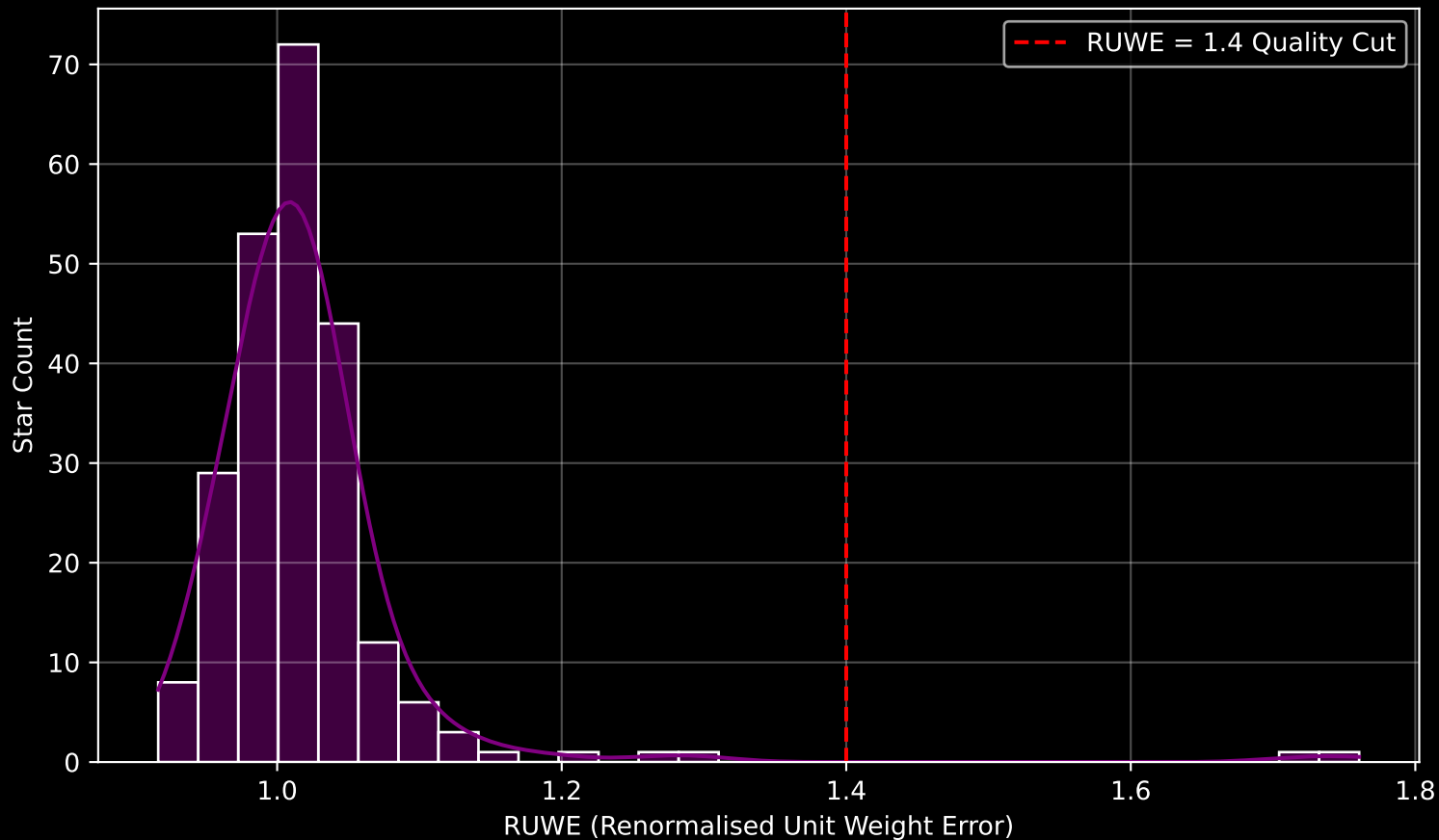
Gaia Cluster: [Ruprecht_58] RUWE Distribution (n= 233)
