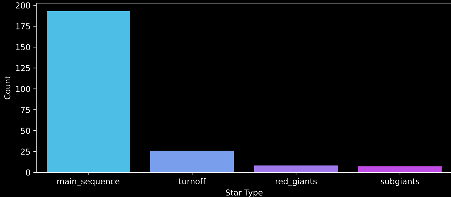
Gaia Cluster: [Ruprecht_58] Count plot of Star Type
