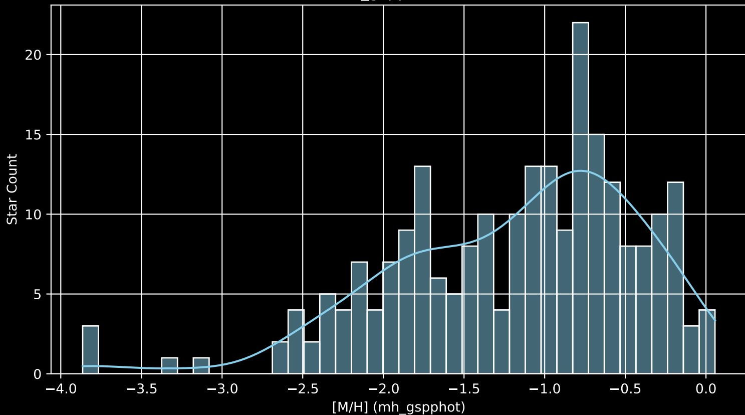
Gaia Cluster: [Ruprecht_58 [M/H] (mh_gspphot) (n= 234)
