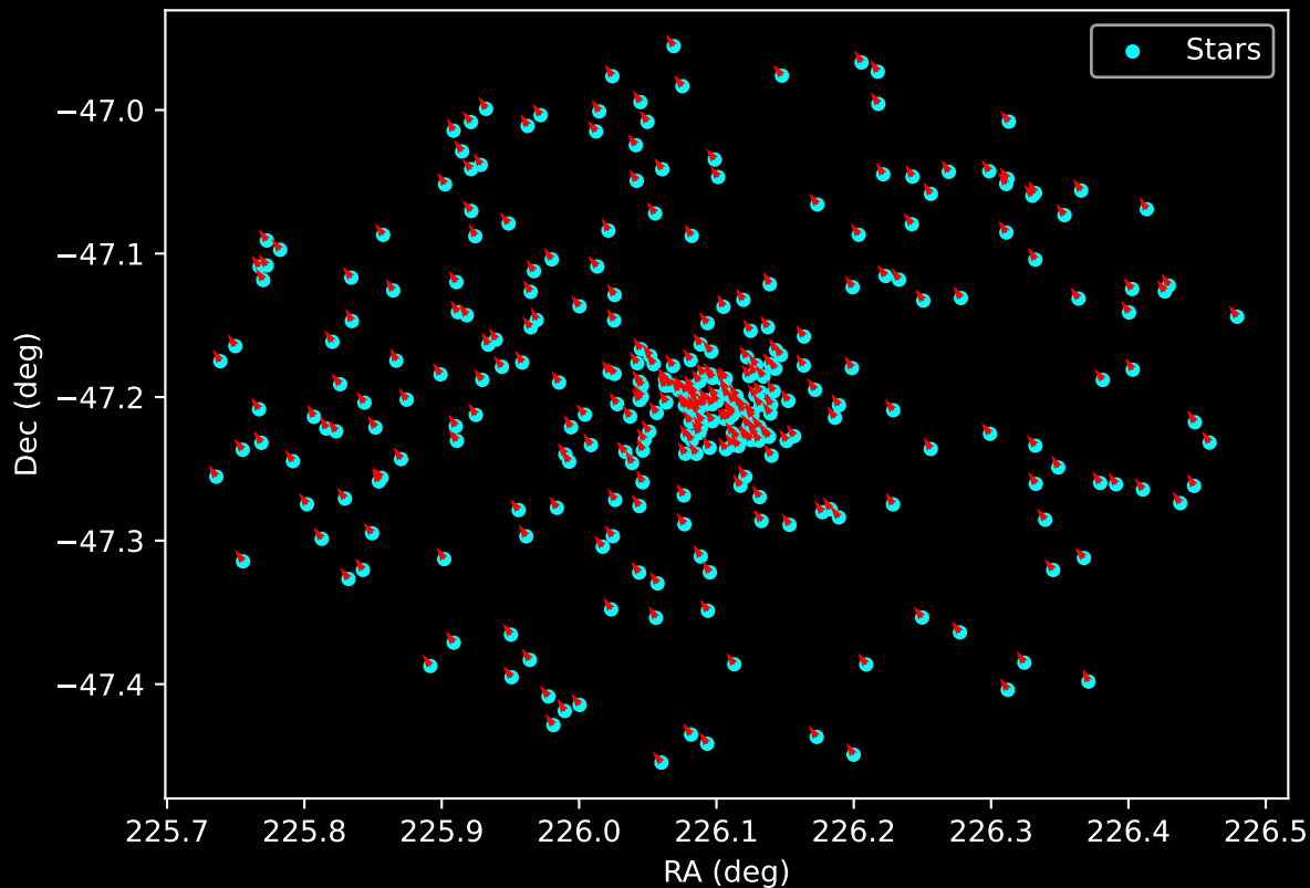
Gaia Cluster: [Ruprecht_60] Proper Motion Vectors for Gaia Star Field (n= 309)
