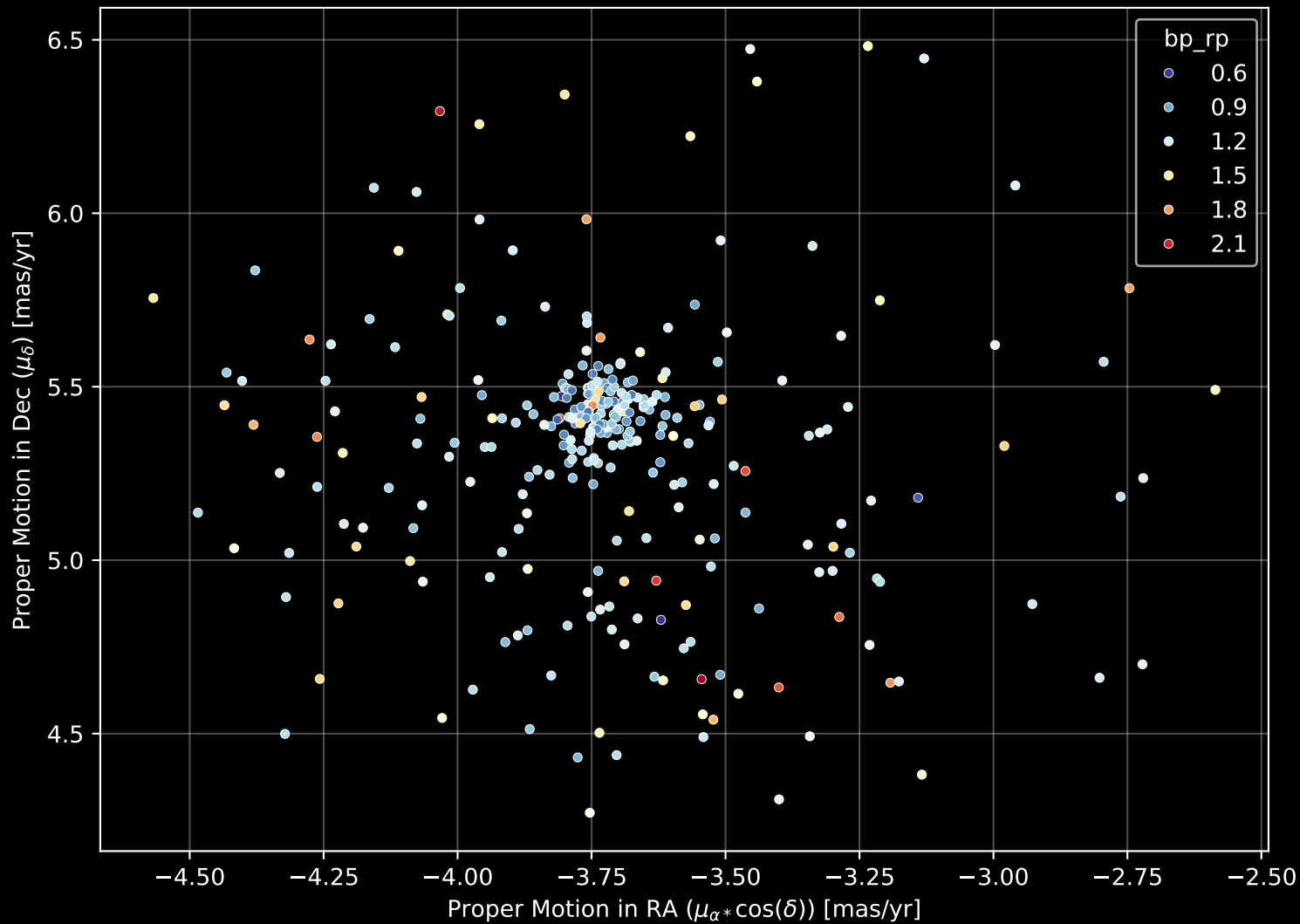
Gaia Cluster: [Ruprecht_60] Proper Motion Diagram (n= 309)
