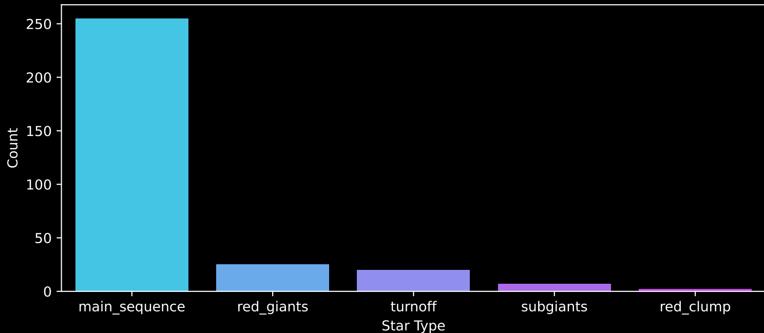
Gaia Cluster: [Ruprecht_60] Count plot of Star Type
