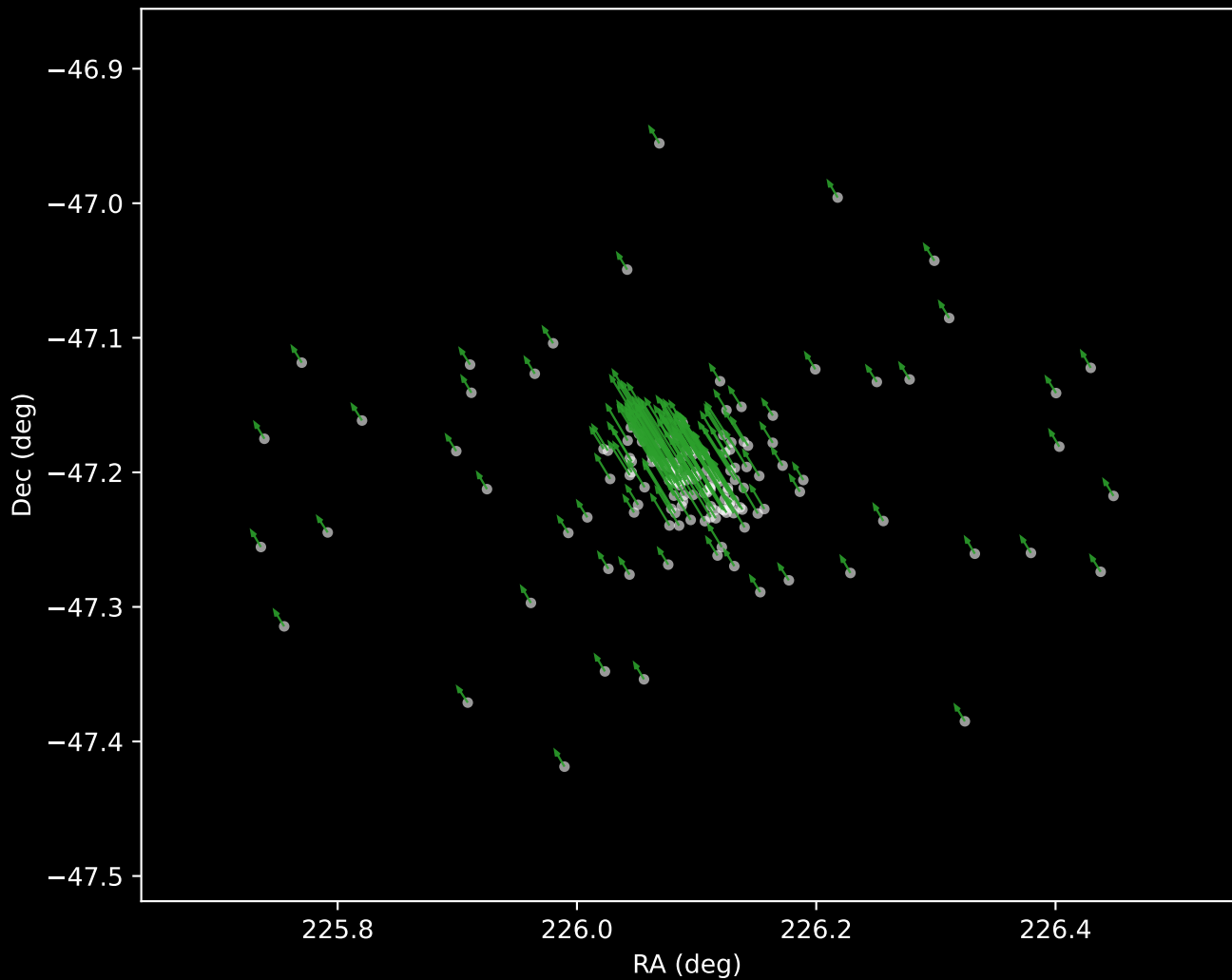
Gaia DR3 Cluster 4 Proper Motion Vectors (n=150)
