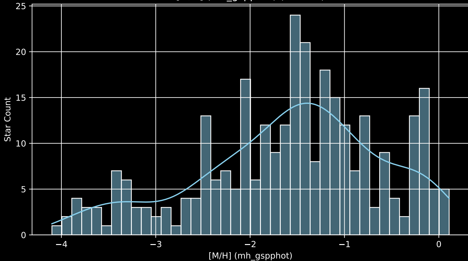
Gaia Cluster: [Ruprecht_60 [M/H] (mh_gspphot) (n= 309)
