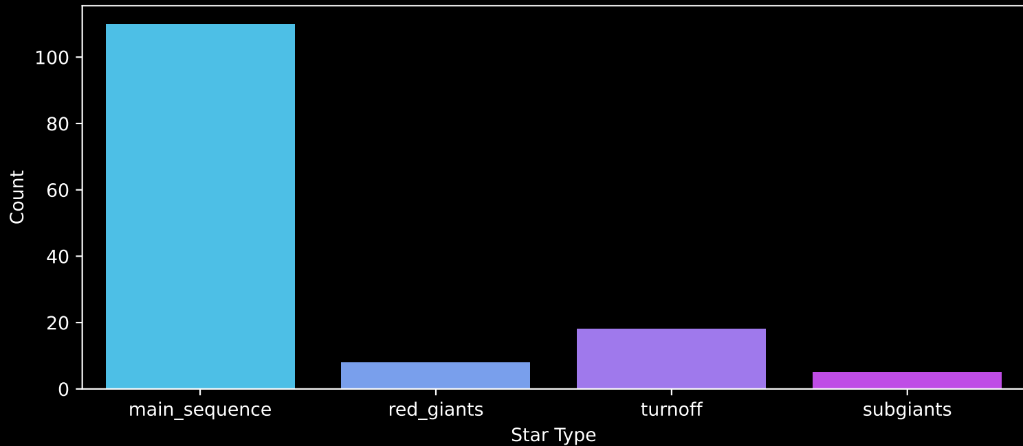
Gaia Cluster: [Ruprecht_61] Count plot of Star Type
