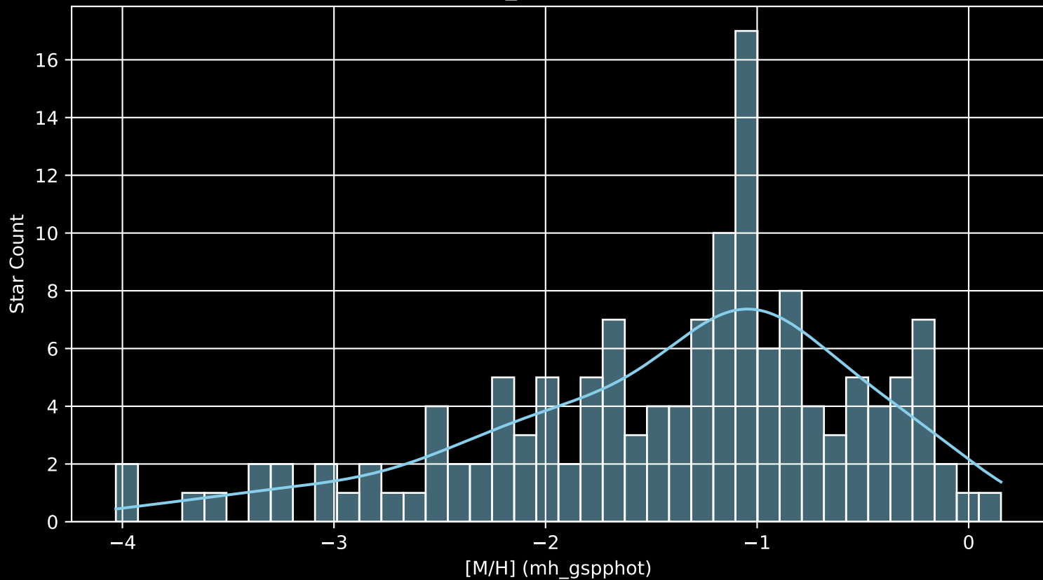
Gaia Cluster: [Ruprecht_61 [M/H] (mh_gspphot) (n= 141)
