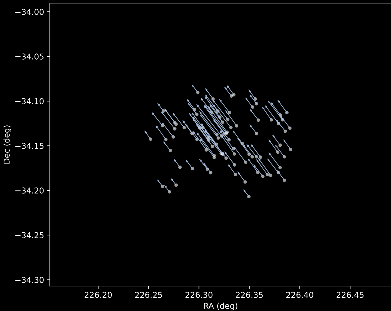
Gaia DR3 Cluster 1 Proper Motion Vectors (n=88)
