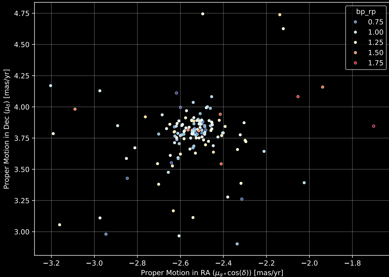
Gaia Cluster: [Ruprecht_61] Proper Motion Diagram (n= 141)
