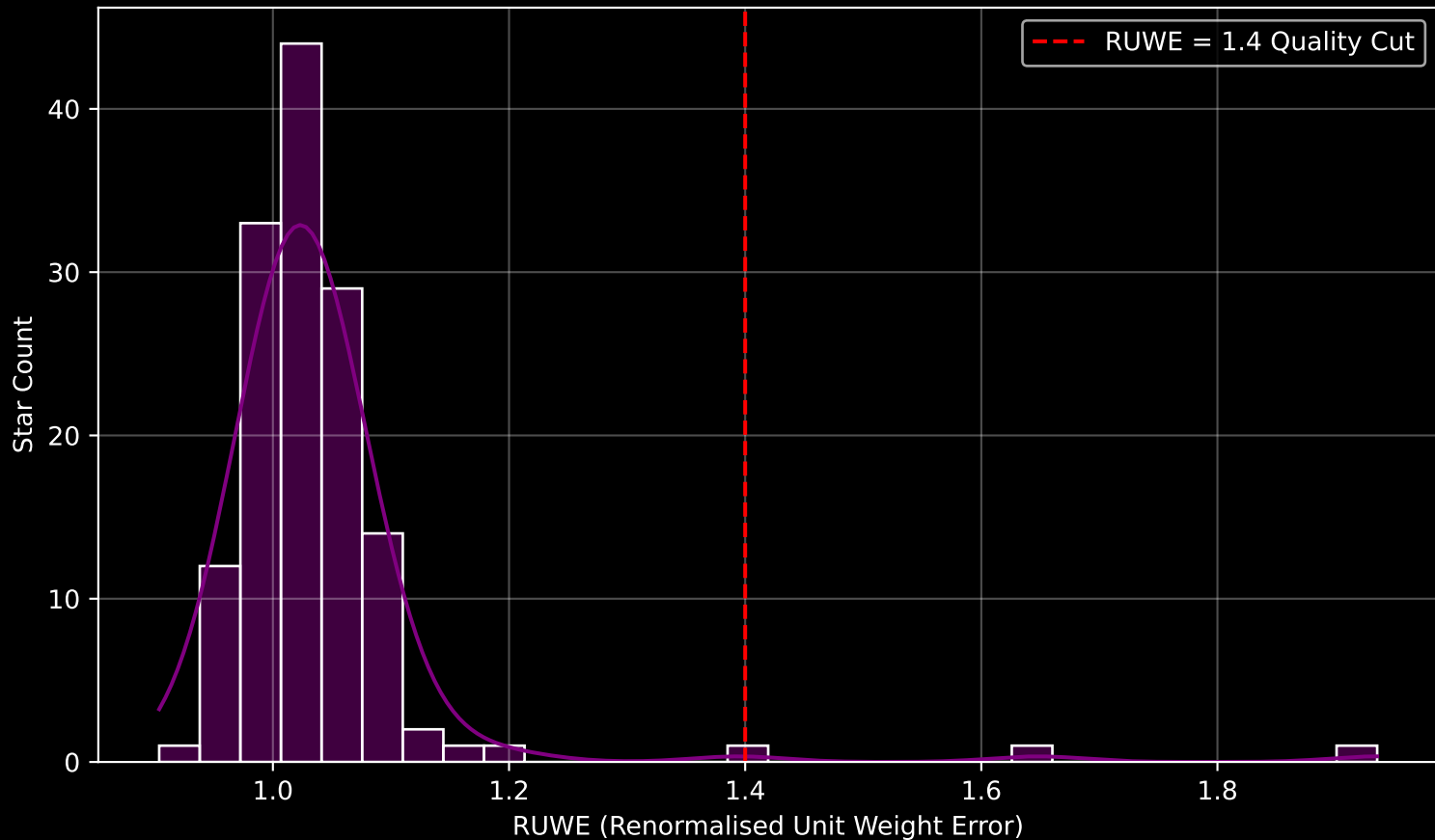
Gaia Cluster: [Ruprecht_61] RUWE Distribution (n= 140)
