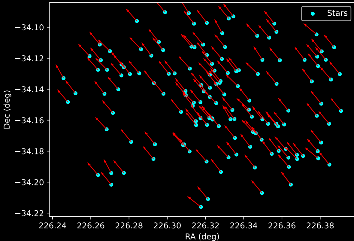
Gaia Cluster: [Ruprecht_61] Proper Motion Vectors for Gaia Star Field (n= 141)
