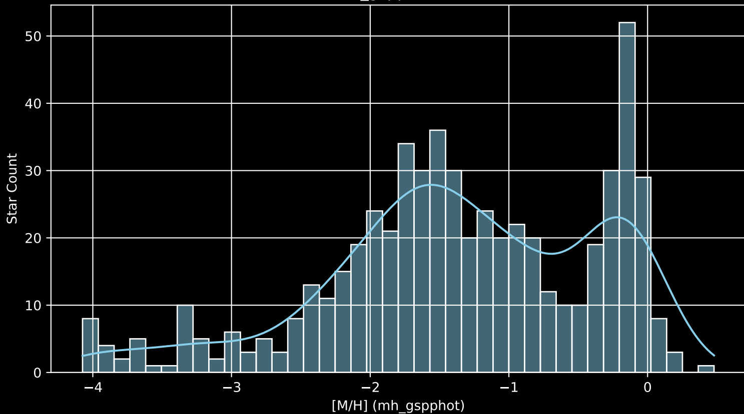
Gaia Cluster: [Ruprecht_66 [M/H] (mh_gspphot) (n= 576)
