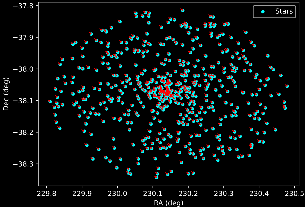
Gaia Cluster: [Ruprecht_66] Proper Motion Vectors for Gaia Star Field (n= 577)
