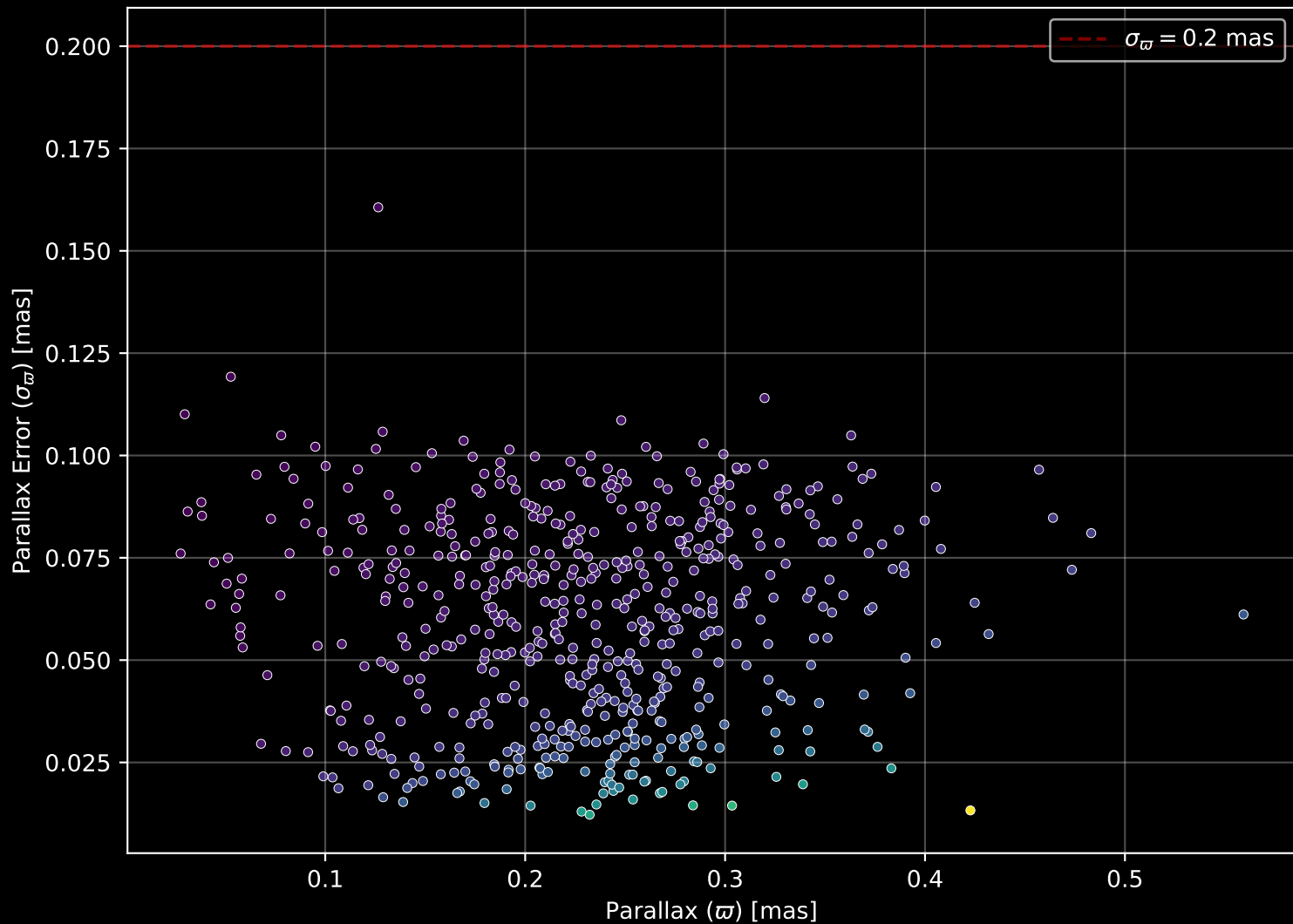
Gaia Cluster: [Ruprecht_66] Parallax Quality (n= 577)
