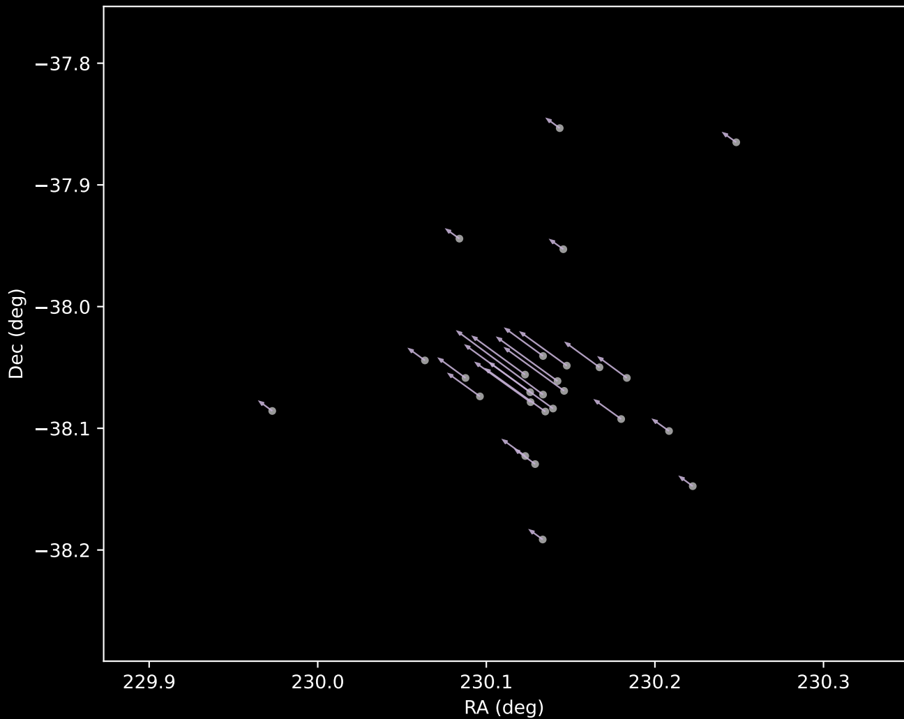
Gaia DR3 Cluster 29 Proper Motion Vectors (n=26)
