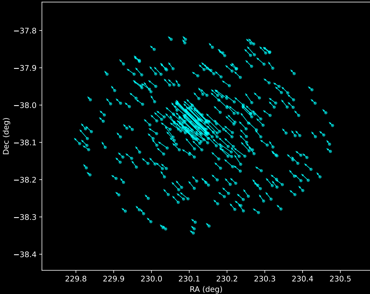
Gaia DR3 Noise Stream Proper Motion Vectors (n=278)
