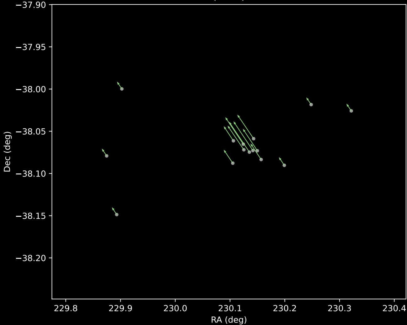
Gaia DR3 Cluster 25 Proper Motion Vectors (n=15)
