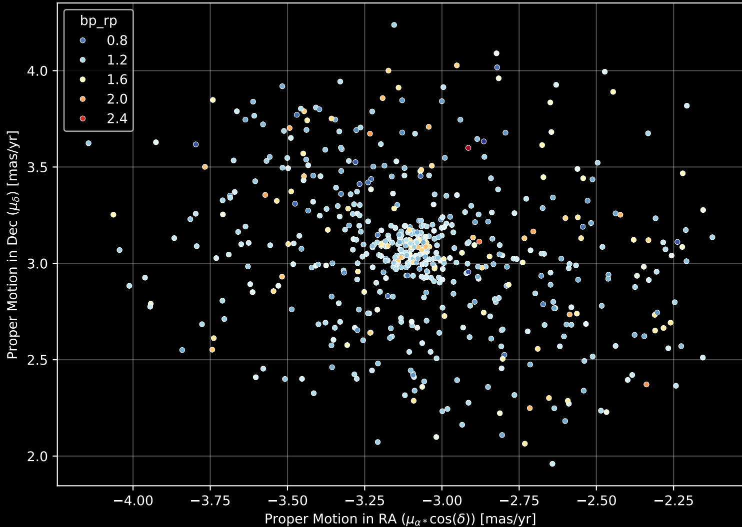
Gaia Cluster: [Ruprecht_66] Proper Motion Diagram (n= 577)
