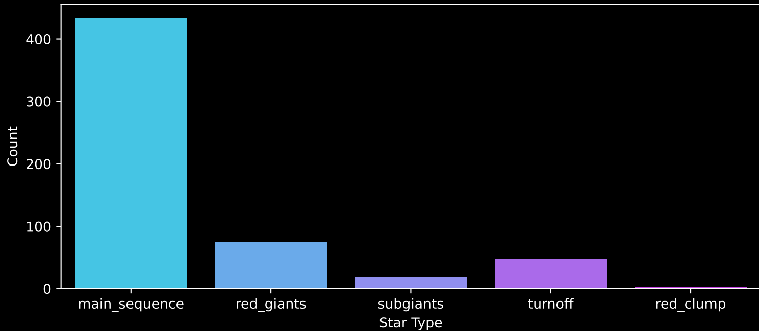
Gaia Cluster: [Ruprecht_66] Count plot of Star Type
