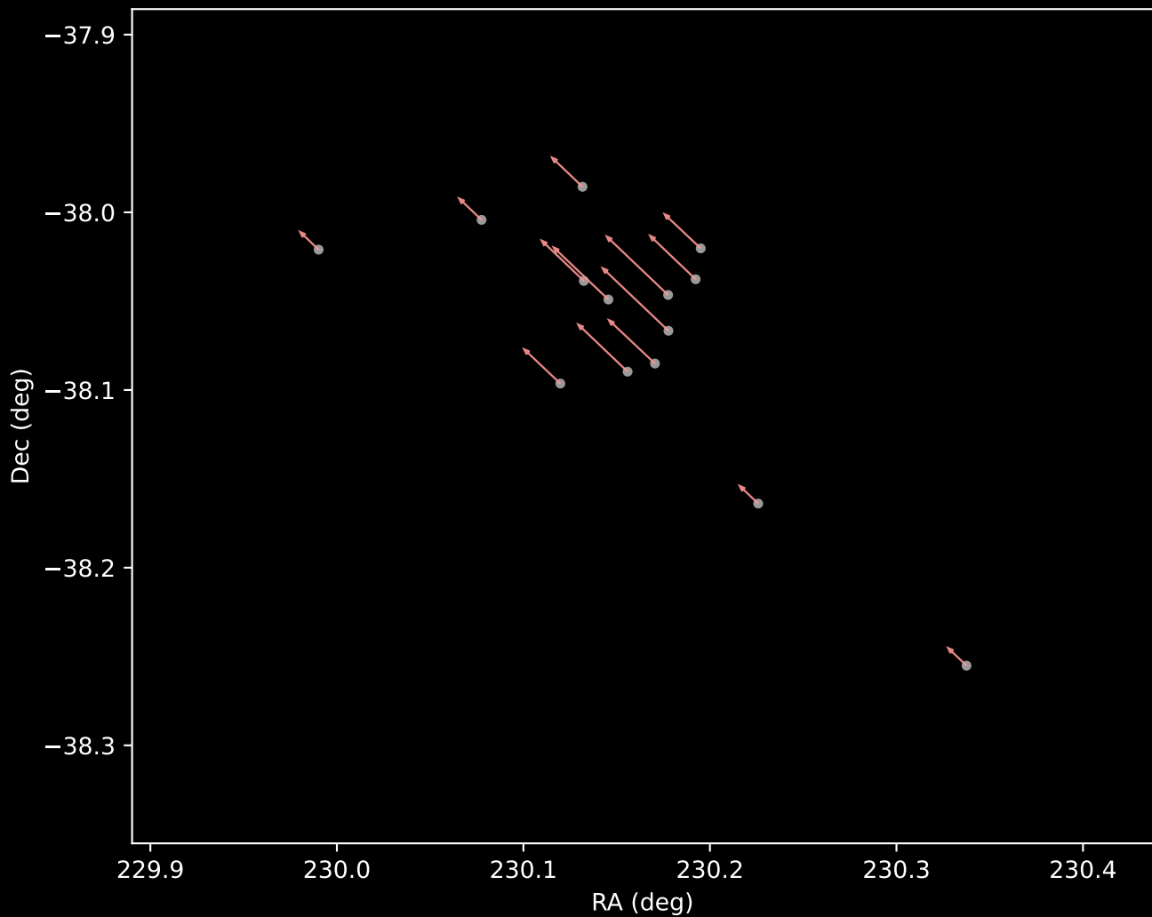
Gaia DR3 Cluster 27 Proper Motion Vectors (n=14)
