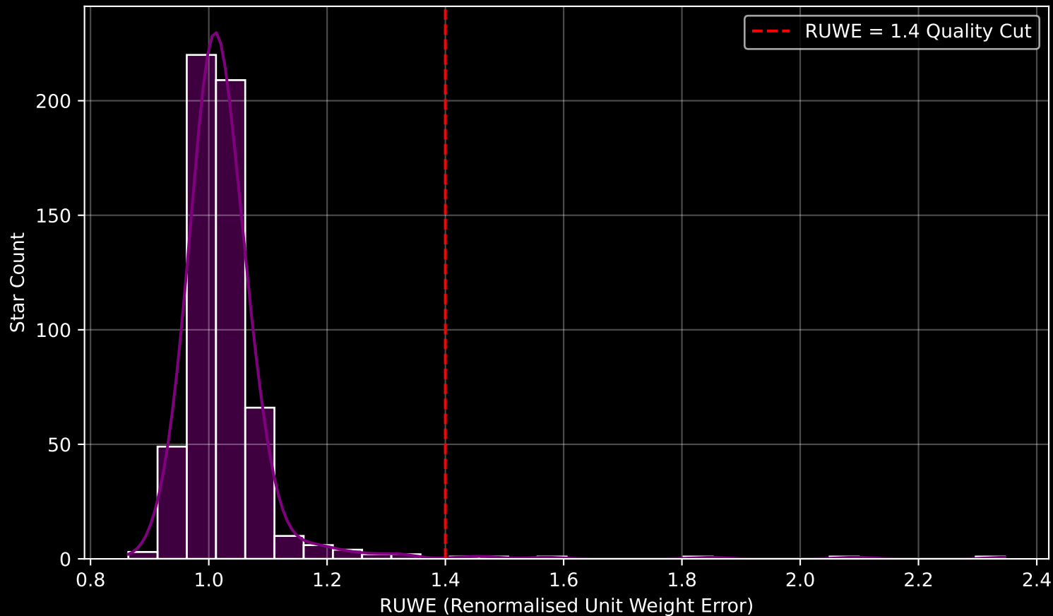
Gaia Cluster: [Ruprecht_66] RUWE Distribution (n= 577)
