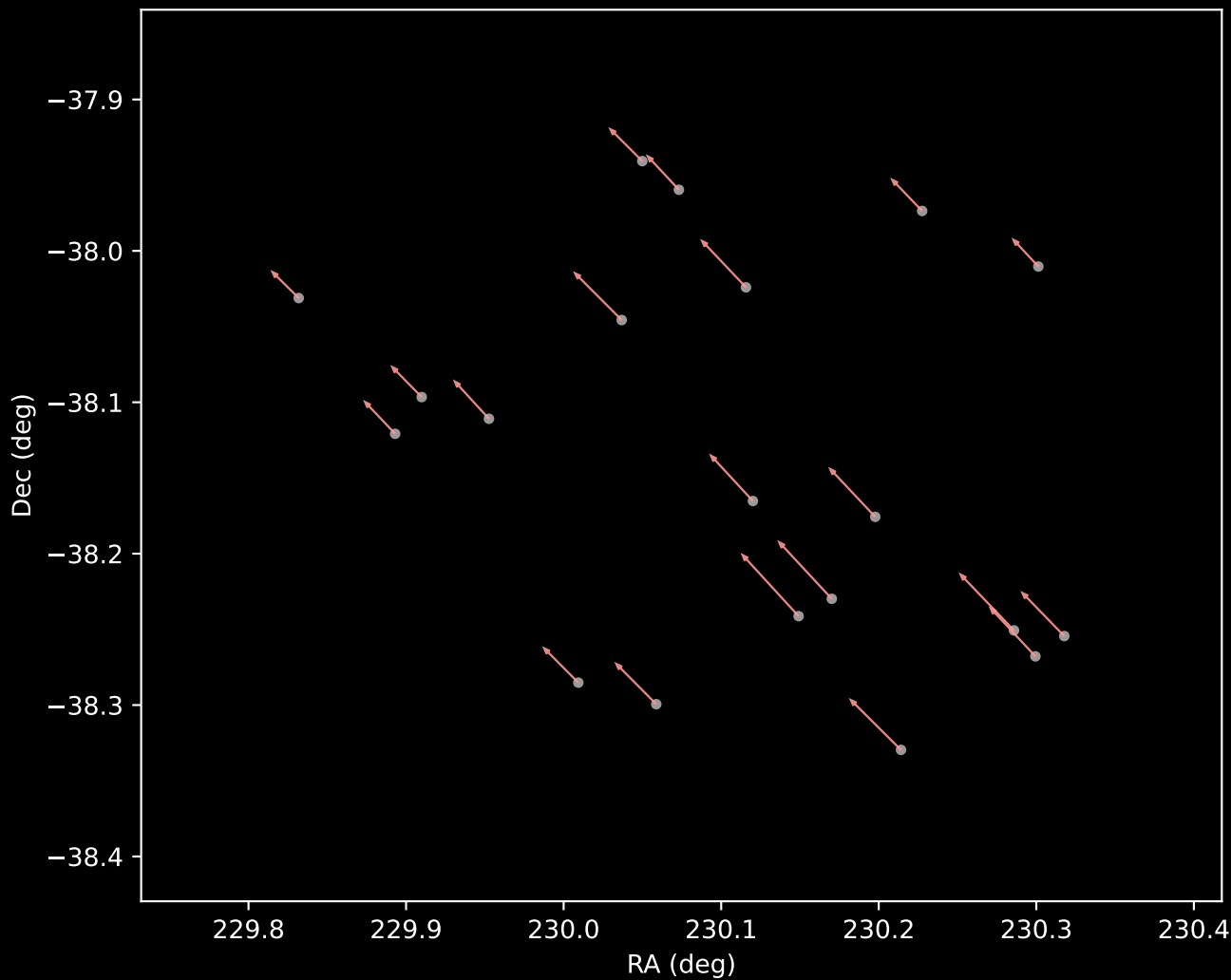
Gaia DR3 Cluster 7 Proper Motion Vectors (n=20)
