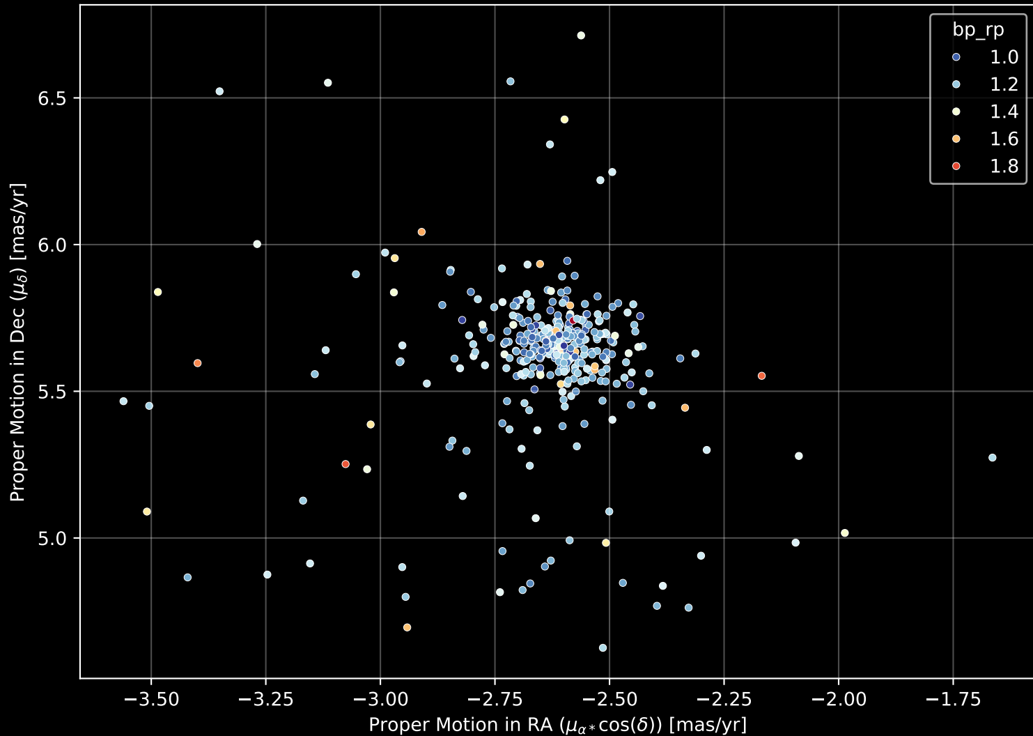
Gaia Cluster: [Ruprecht_68] Proper Motion Diagram (n= 382)
