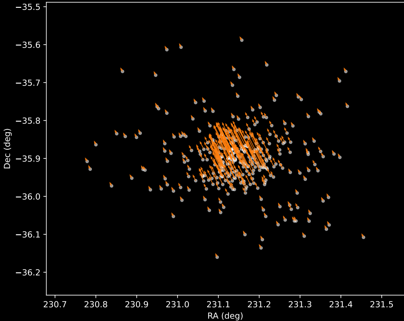
Gaia DR3 Cluster 2 Proper Motion Vectors (n=334)
