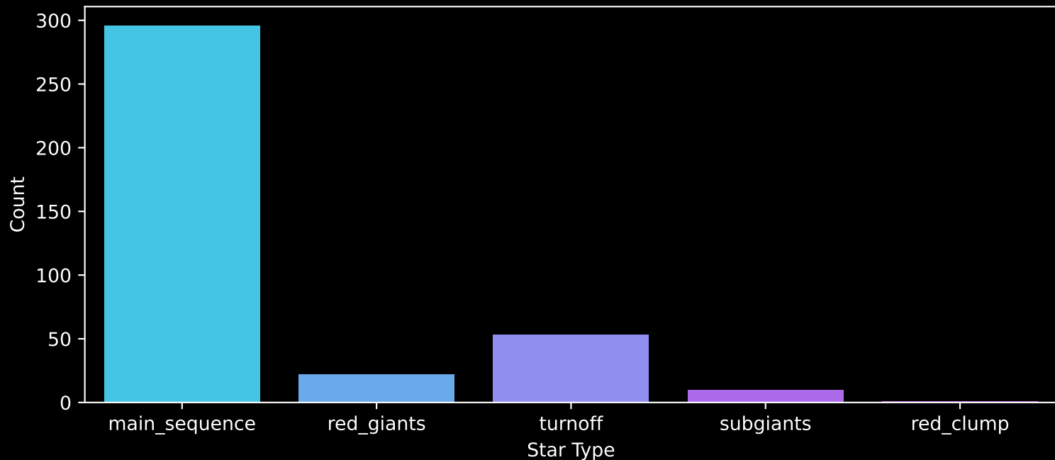
Gaia Cluster: [Ruprecht_68] Count plot of Star Type
