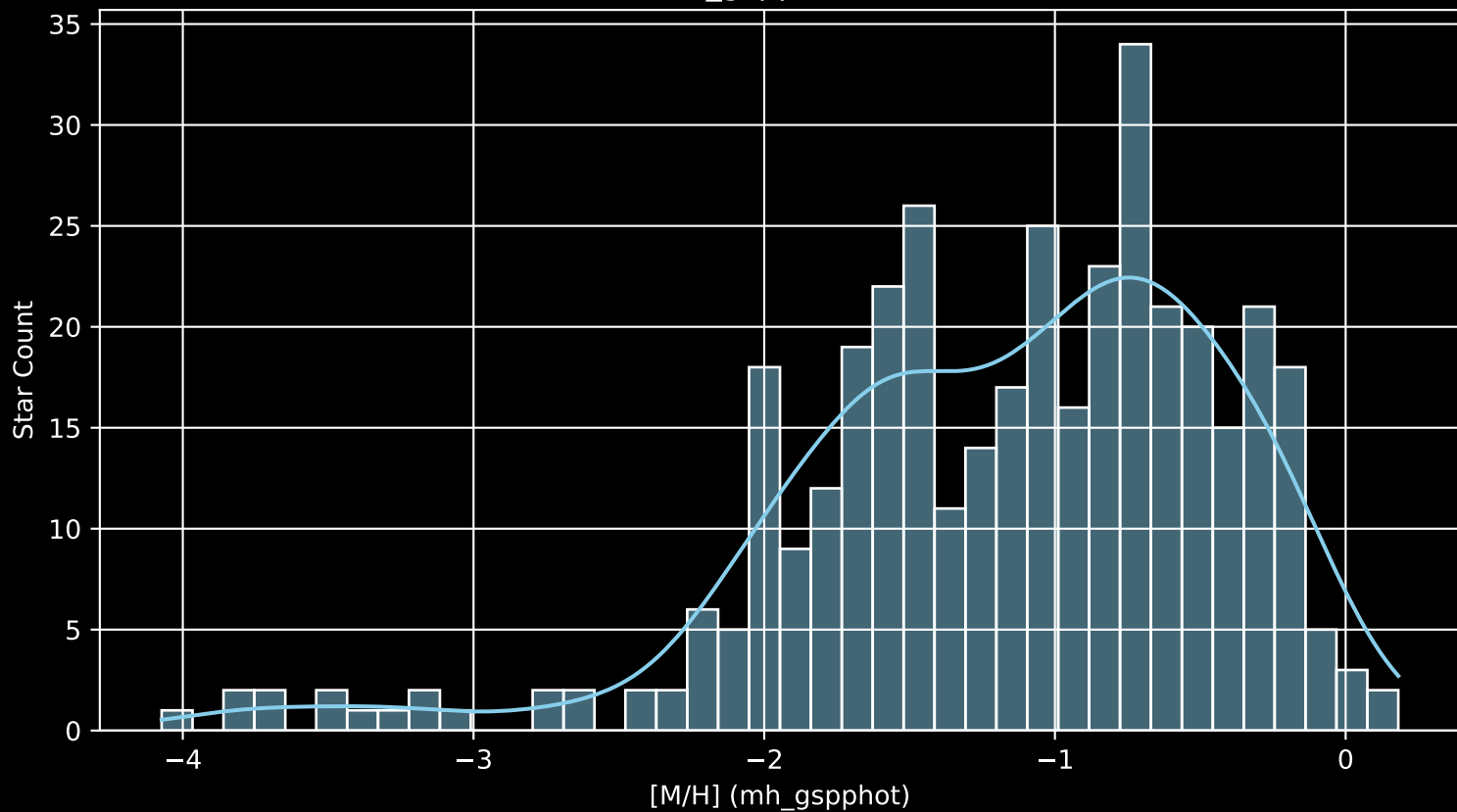
Gaia Cluster: [Ruprecht_68 [M/H] (mh_gspphot) (n= 382)
