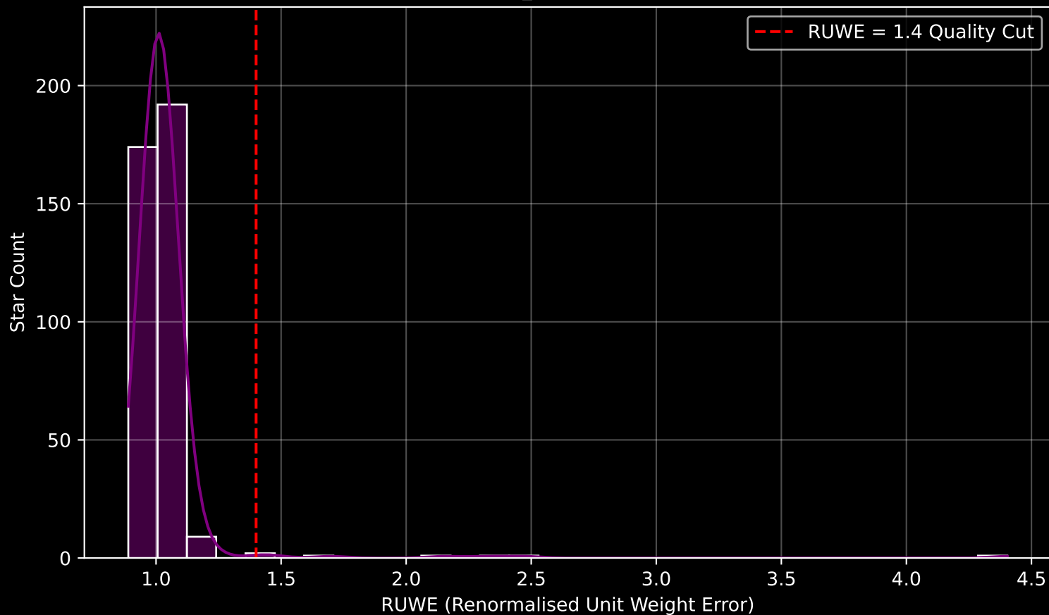
Gaia Cluster: [Ruprecht_68] RUWE Distribution (n= 382)
