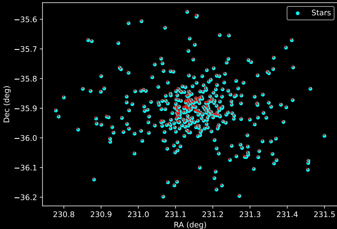
Gaia Cluster: [Ruprecht_68] Proper Motion Vectors for Gaia Star Field (n= 382)
