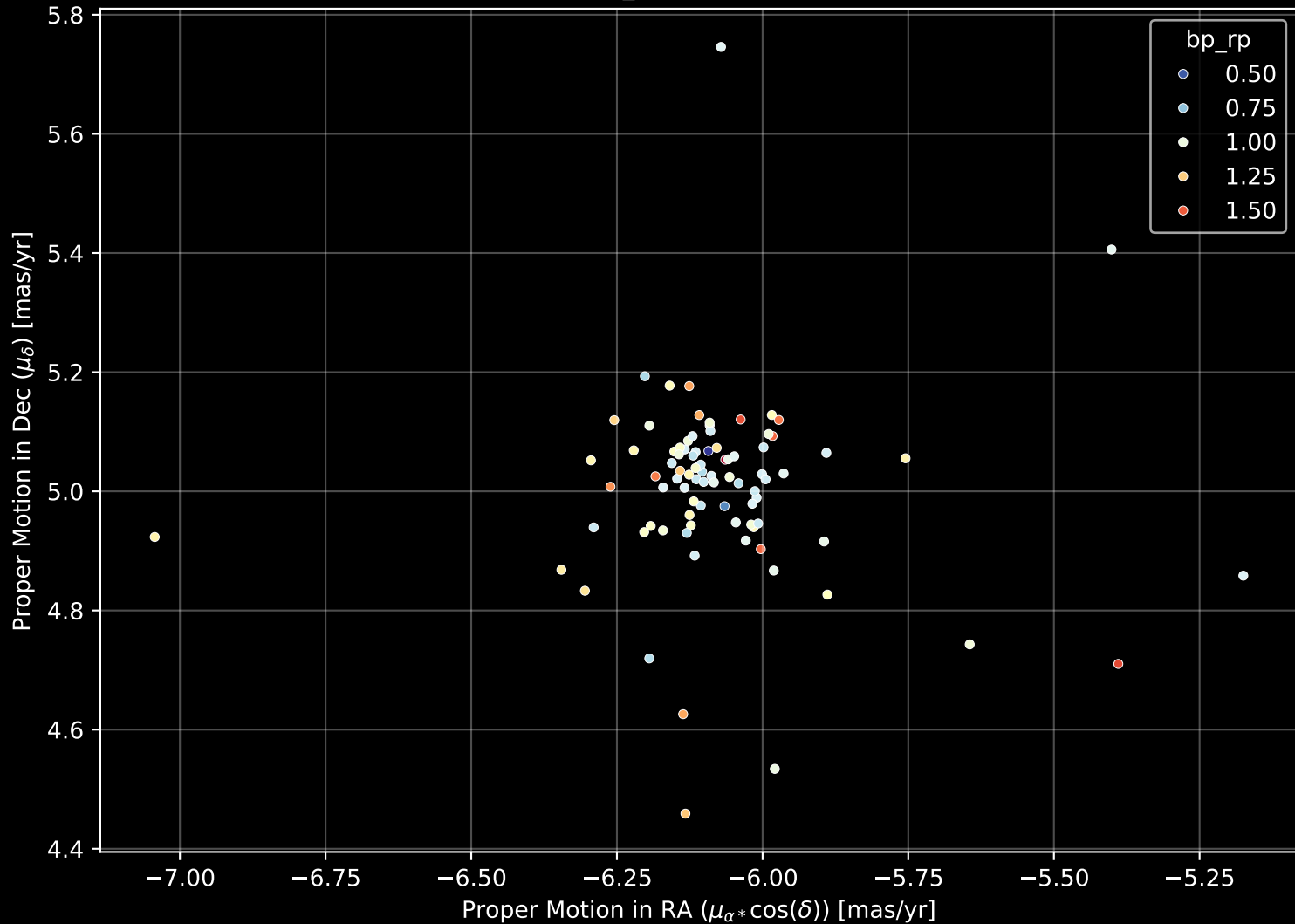
Gaia Cluster: [Ruprecht_75] Proper Motion Diagram (n= 88)
