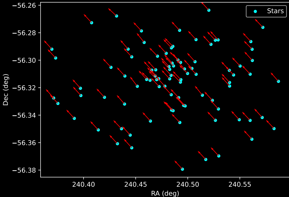
Gaia Cluster: [Ruprecht_75] Proper Motion Vectors for Gaia Star Field (n= 88)
