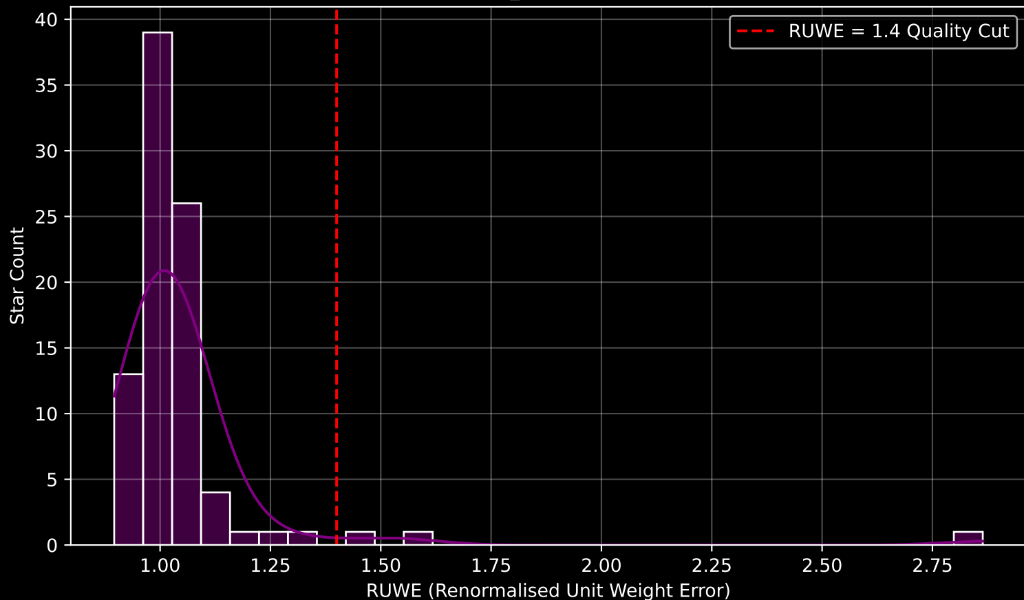
Gaia Cluster: [Ruprecht_75] RUWE Distribution (n= 88)
