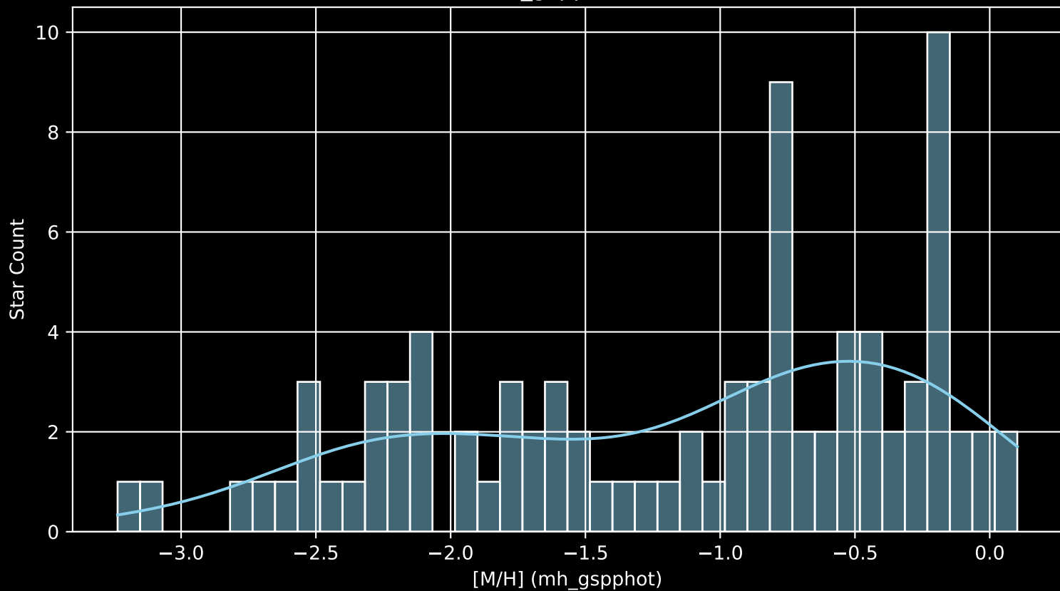
Gaia Cluster: [Ruprecht_75 [M/H] (mh_gspphot) (n= 88)
