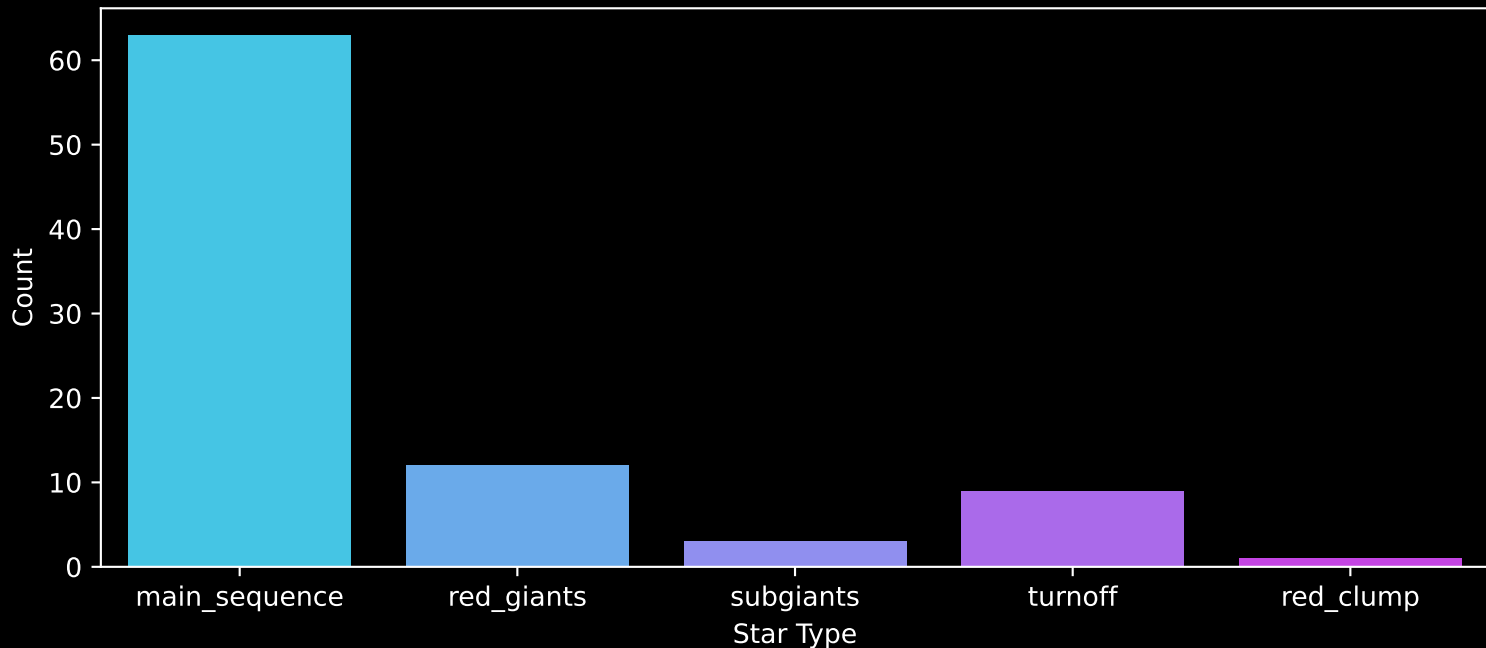
Gaia Cluster: [Ruprecht_75] Count plot of Star Type
