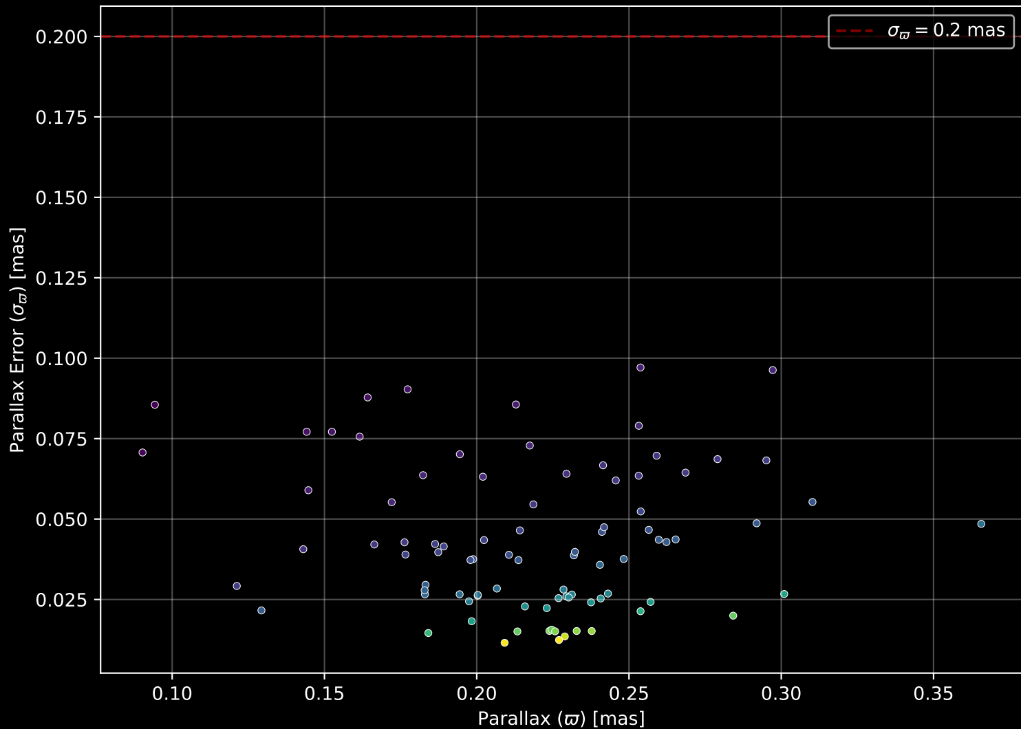
Gaia Cluster: [Ruprecht_75] Parallax Quality (n= 88)
