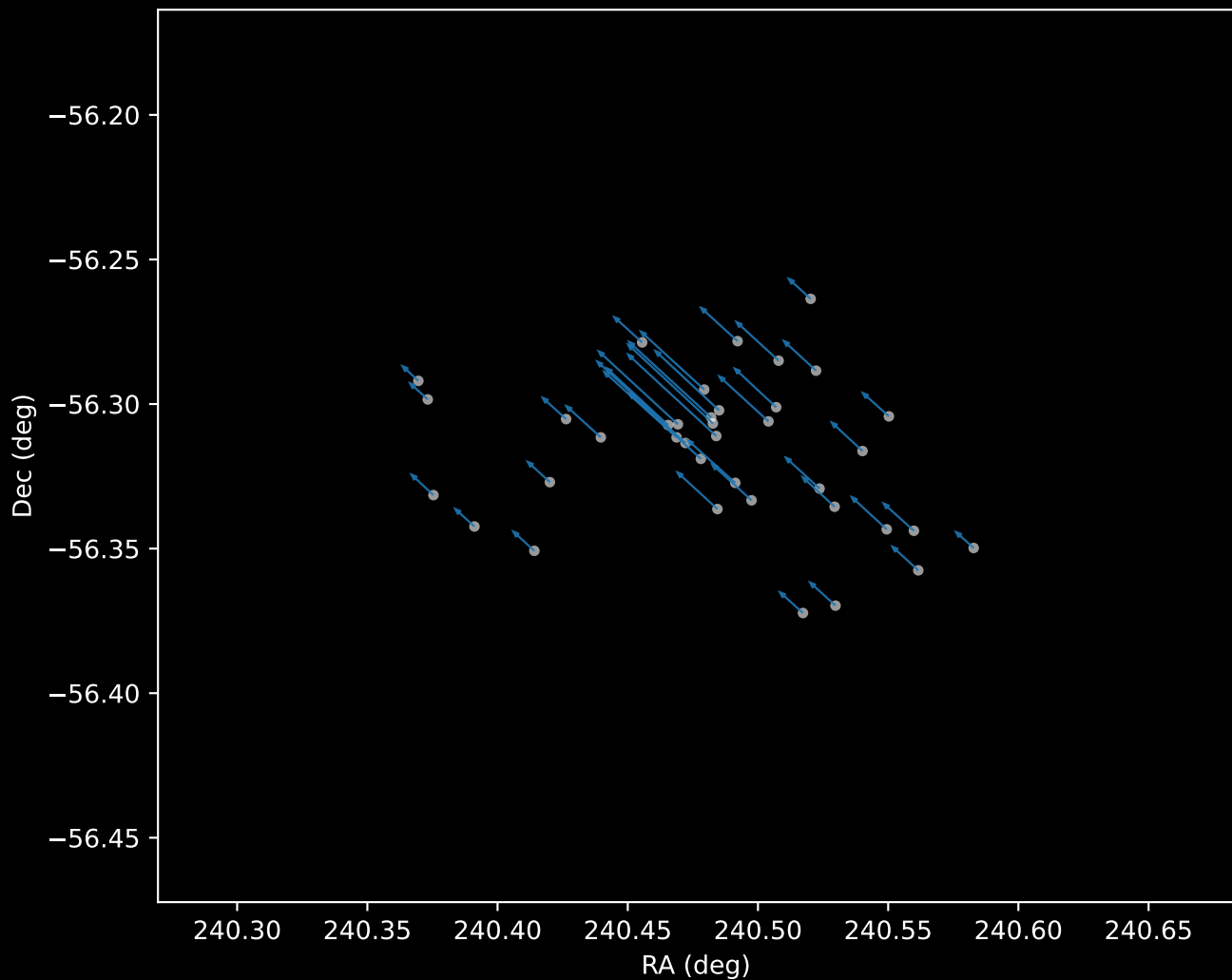
Gaia DR3 Cluster 0 Proper Motion Vectors (n=38)
