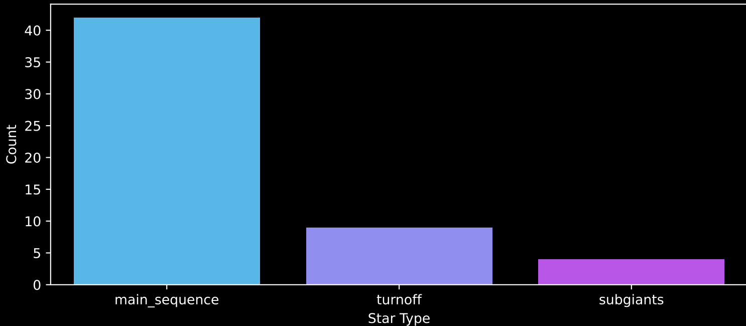
Gaia Cluster: [Ruprecht_76] Count plot of Star Type
