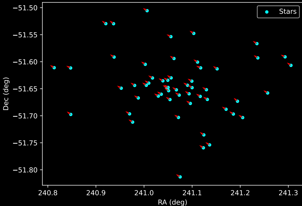
Gaia Cluster: [Ruprecht_76] Proper Motion Vectors for Gaia Star Field (n= 55)
