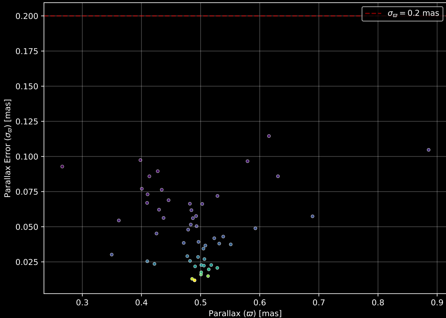
Gaia Cluster: [Ruprecht_76] Parallax Quality (n= 55)
