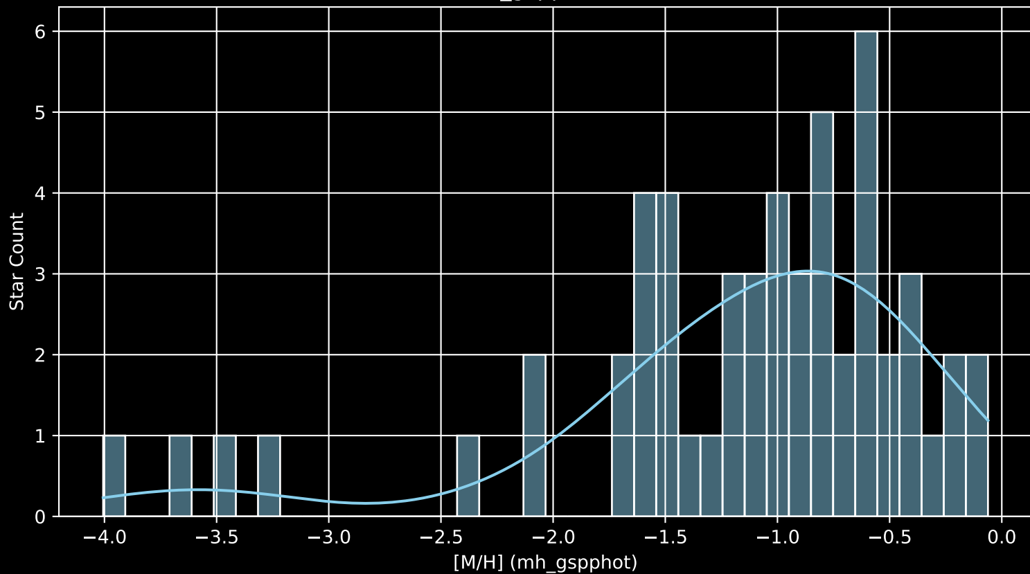
Gaia Cluster: [Ruprecht_76 [M/H] (mh_gspphot) (n= 55)
