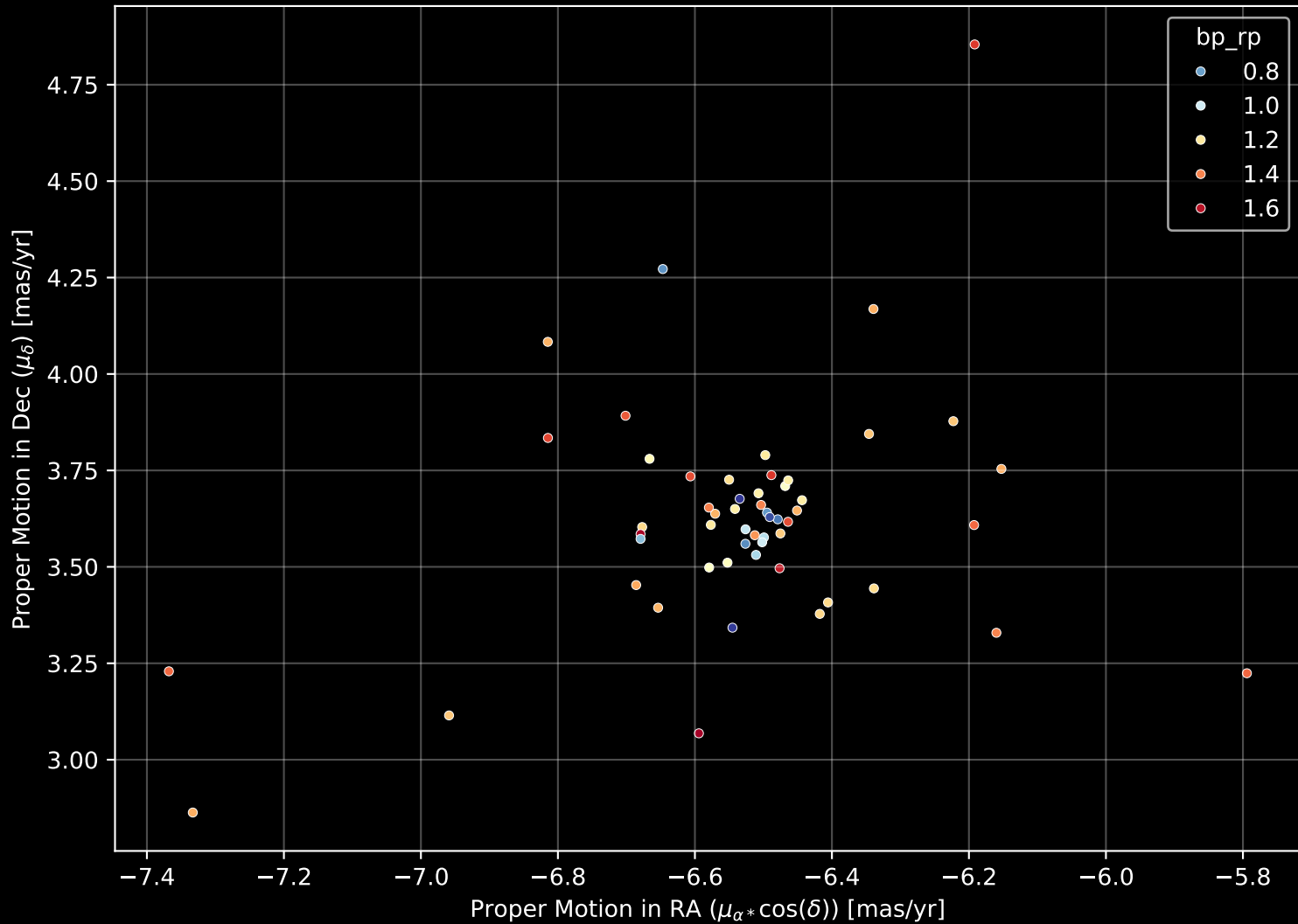
Gaia Cluster: [Ruprecht_76] Proper Motion Diagram (n= 55)
