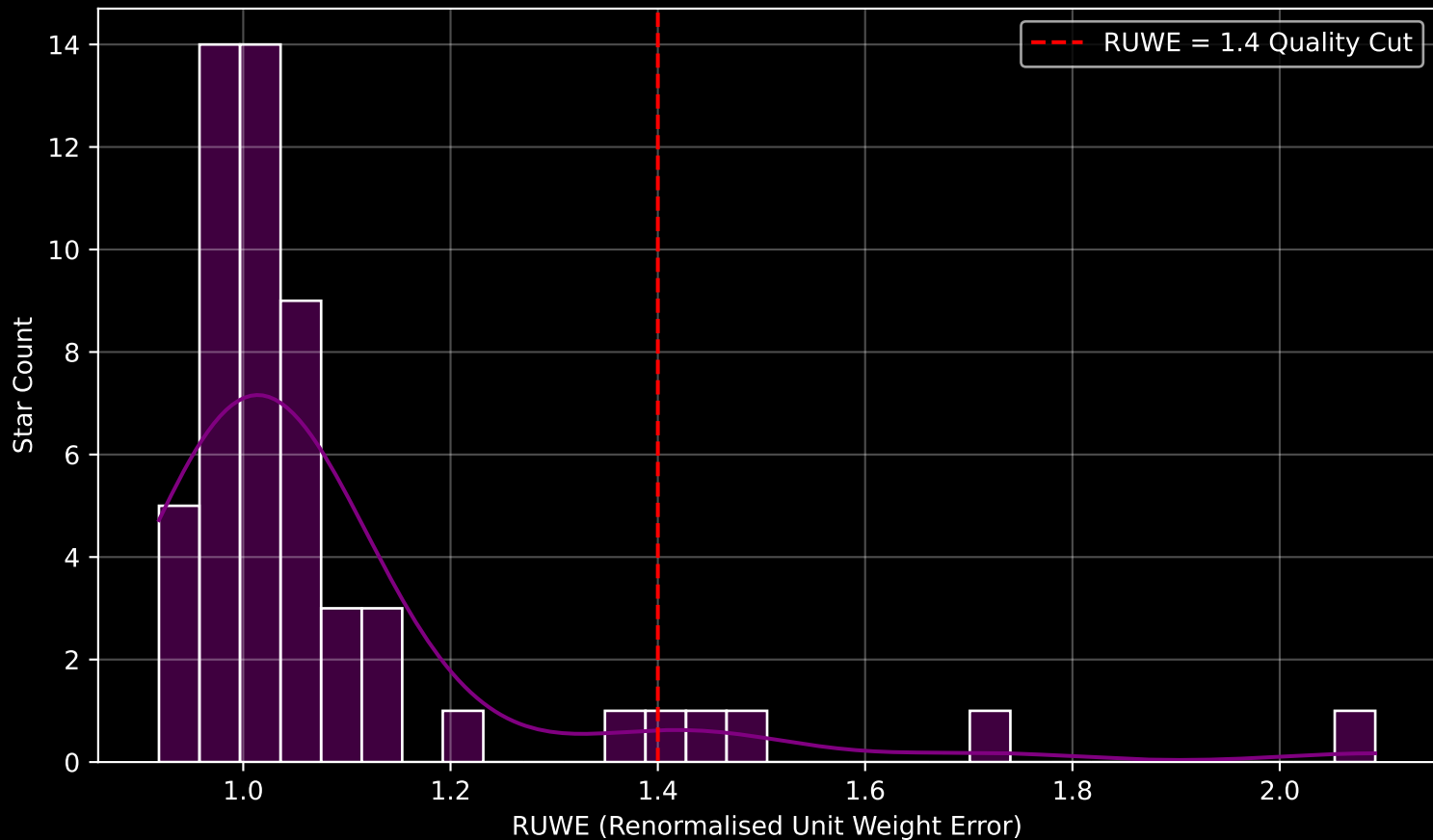
Gaia Cluster: [Ruprecht_76] RUWE Distribution (n= 55)
