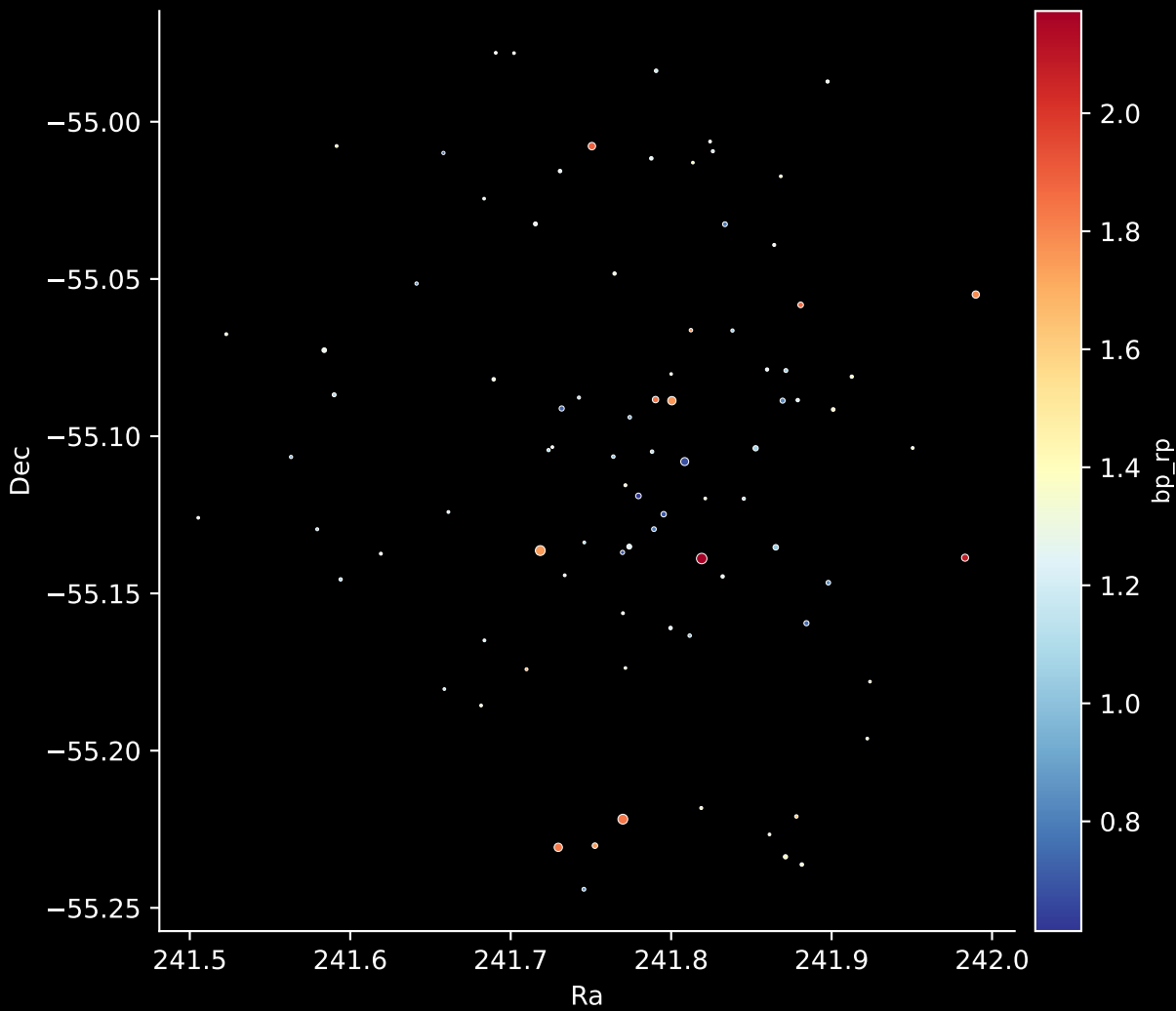
Gaia Cluster: [Ruprecht_77] Stars: 88
