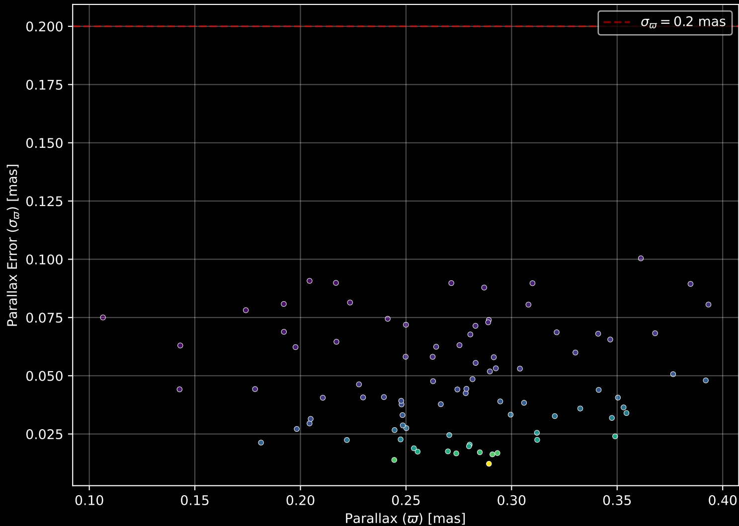
Gaia Cluster: [Ruprecht_77] Parallax Quality (n= 88)
