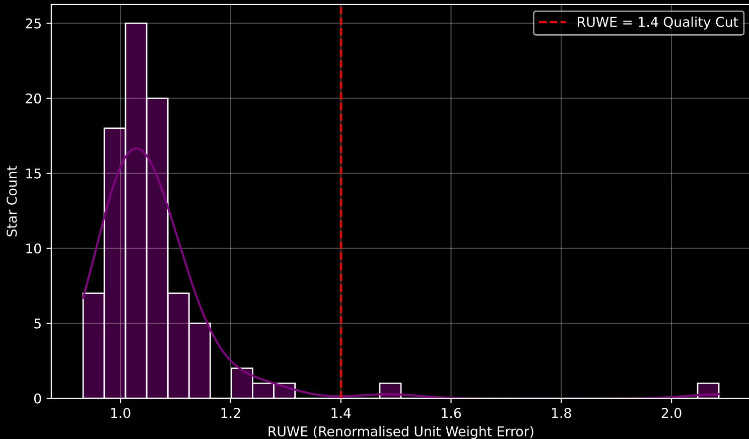
Gaia Cluster: [Ruprecht_77] RUWE Distribution (n= 88)
