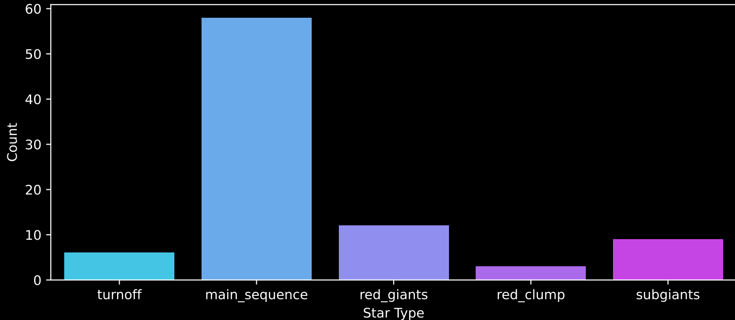
Gaia Cluster: [Ruprecht_77] Count plot of Star Type
