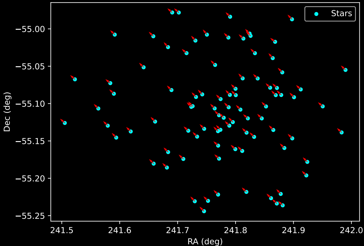
Gaia Cluster: [Ruprecht_77] Proper Motion Vectors for Gaia Star Field (n= 88)
