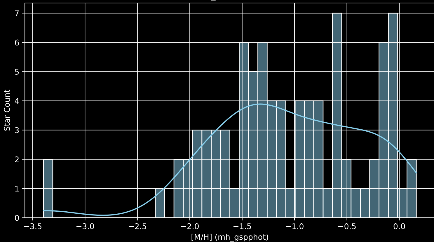
Gaia Cluster: [Ruprecht_77 [M/H] (mh_gspphot) (n= 88)
