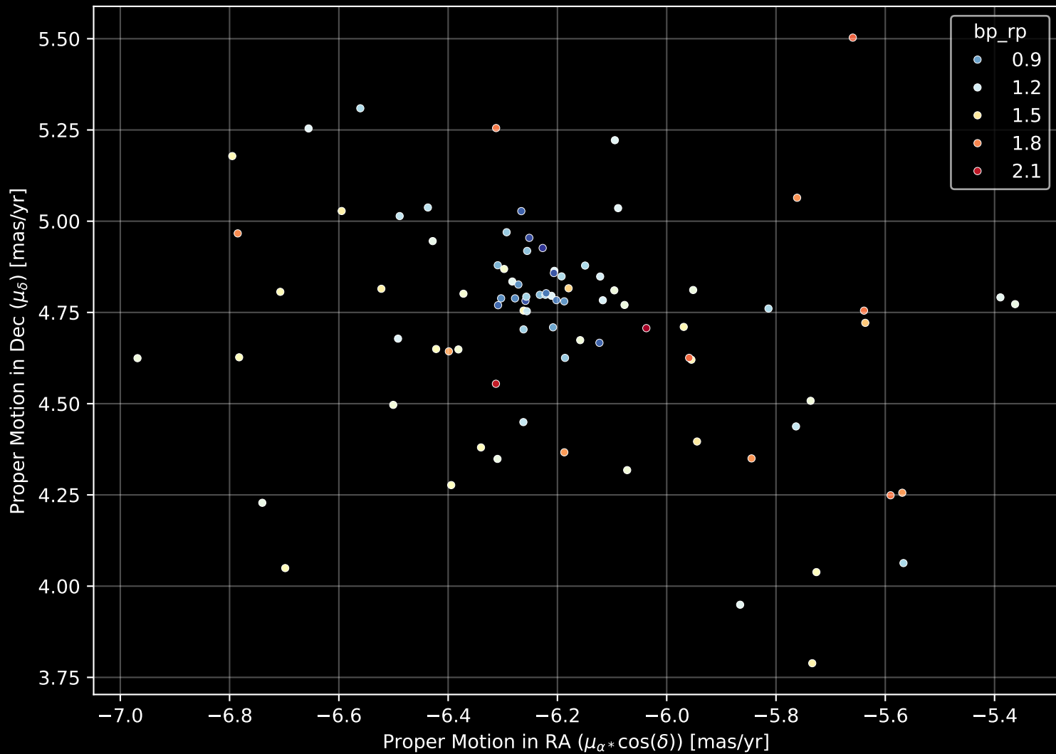
Gaia Cluster: [Ruprecht_77] Proper Motion Diagram (n= 88)
