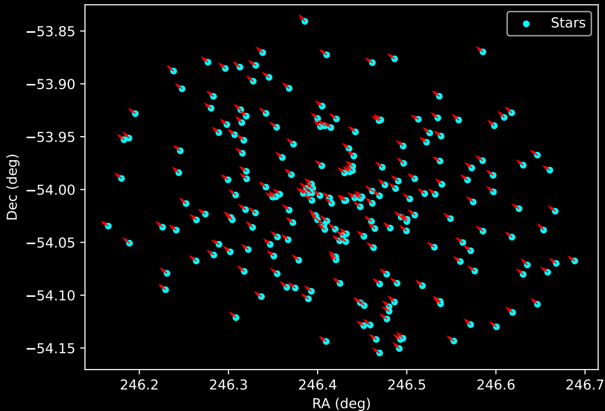
Gaia Cluster: [Ruprecht_82] Proper Motion Vectors for Gaia Star Field (n= 208)
