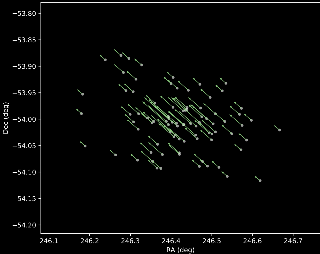
Gaia DR3 Cluster 5 Proper Motion Vectors (n=85)
