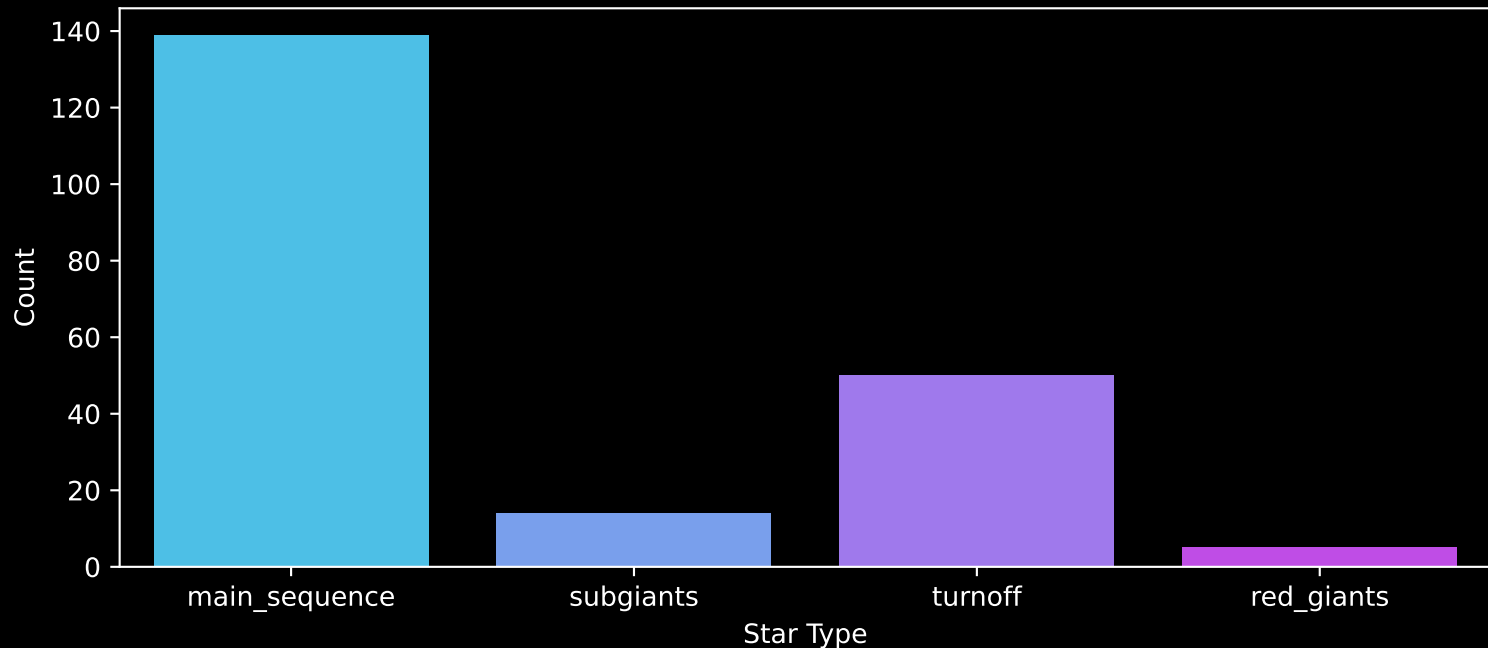
Gaia Cluster: [Ruprecht_82] Count plot of Star Type
