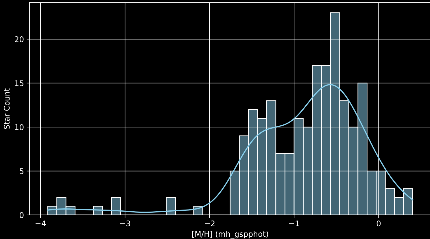
Gaia Cluster: [Ruprecht_82 [M/H] (mh_gspphot) (n= 208)
