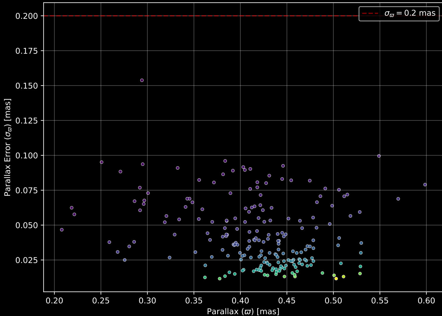
Gaia Cluster: [Ruprecht_82] Parallax Quality (n= 208)
