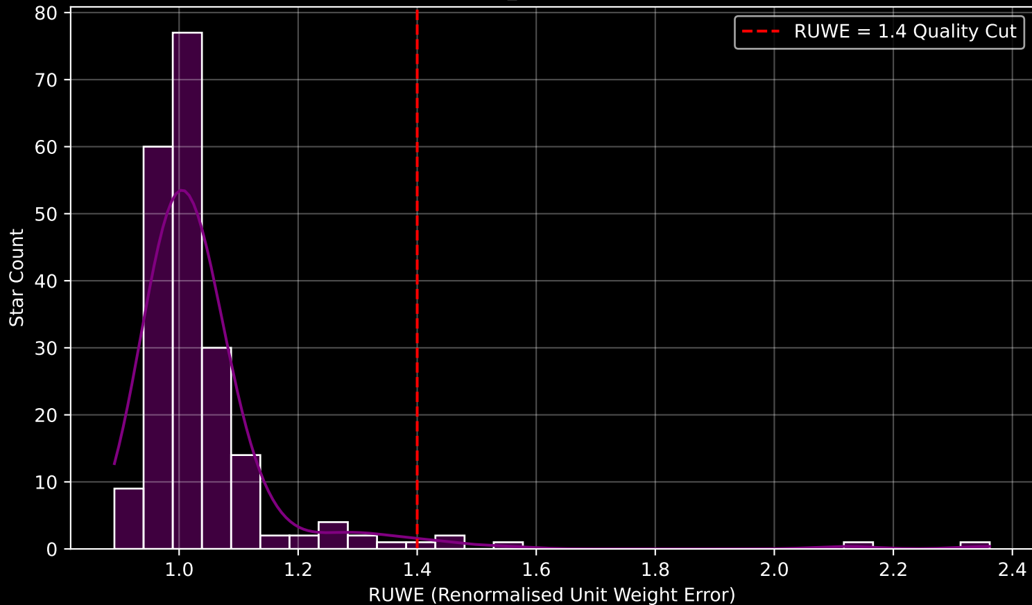
Gaia Cluster: [Ruprecht_82] RUWE Distribution (n= 207)
