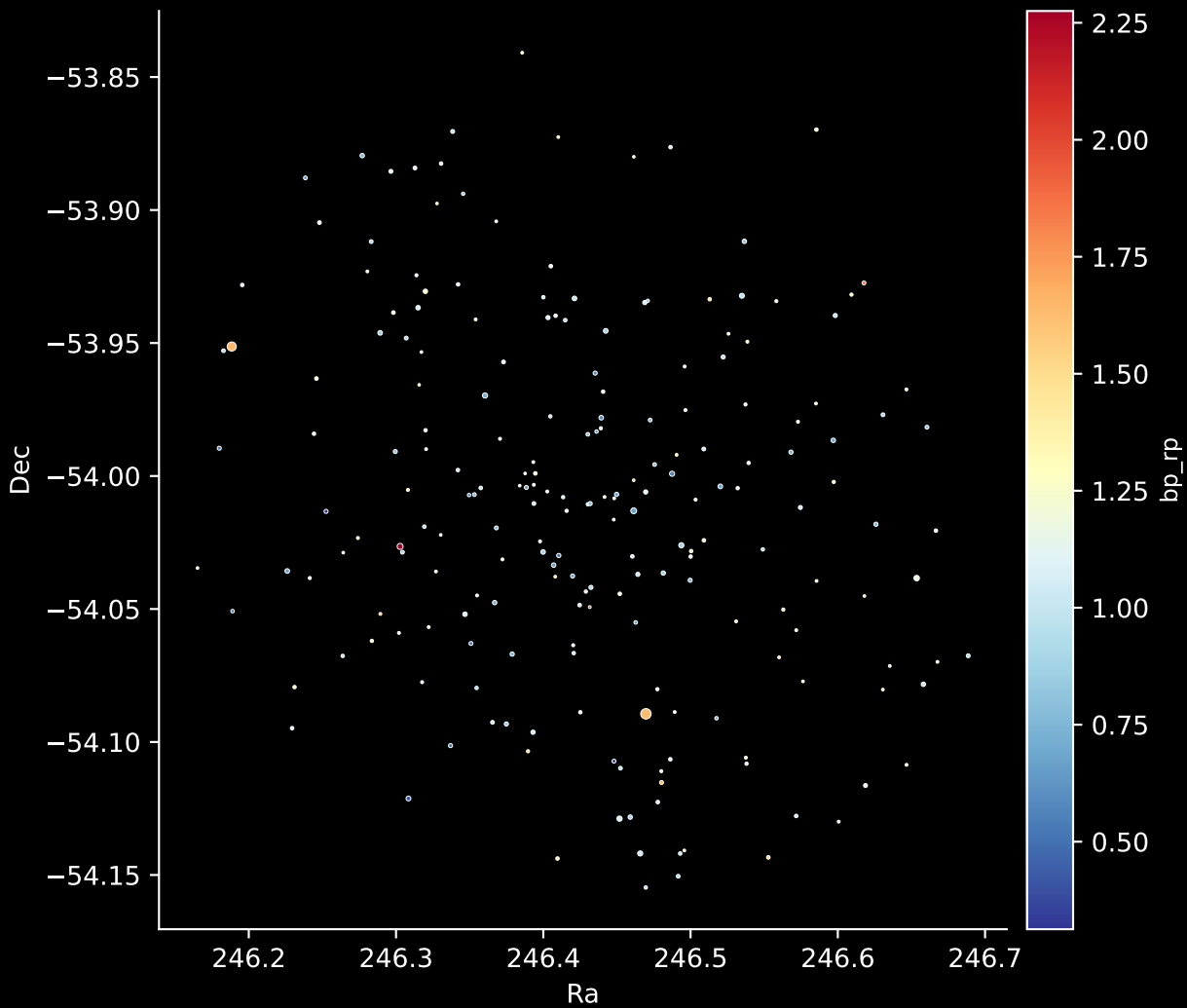
Gaia Cluster: [Ruprecht_82] Stars: 208
