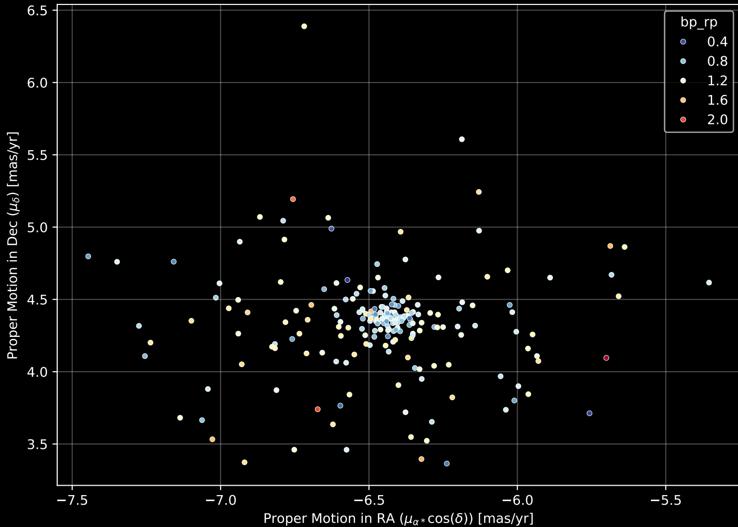
Gaia Cluster: [Ruprecht_82] Proper Motion Diagram (n= 208)
