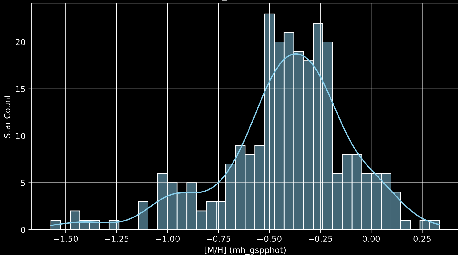
Gaia Cluster: [Ruprecht_91 [M/H] (mh_gspphot) (n= 260)
