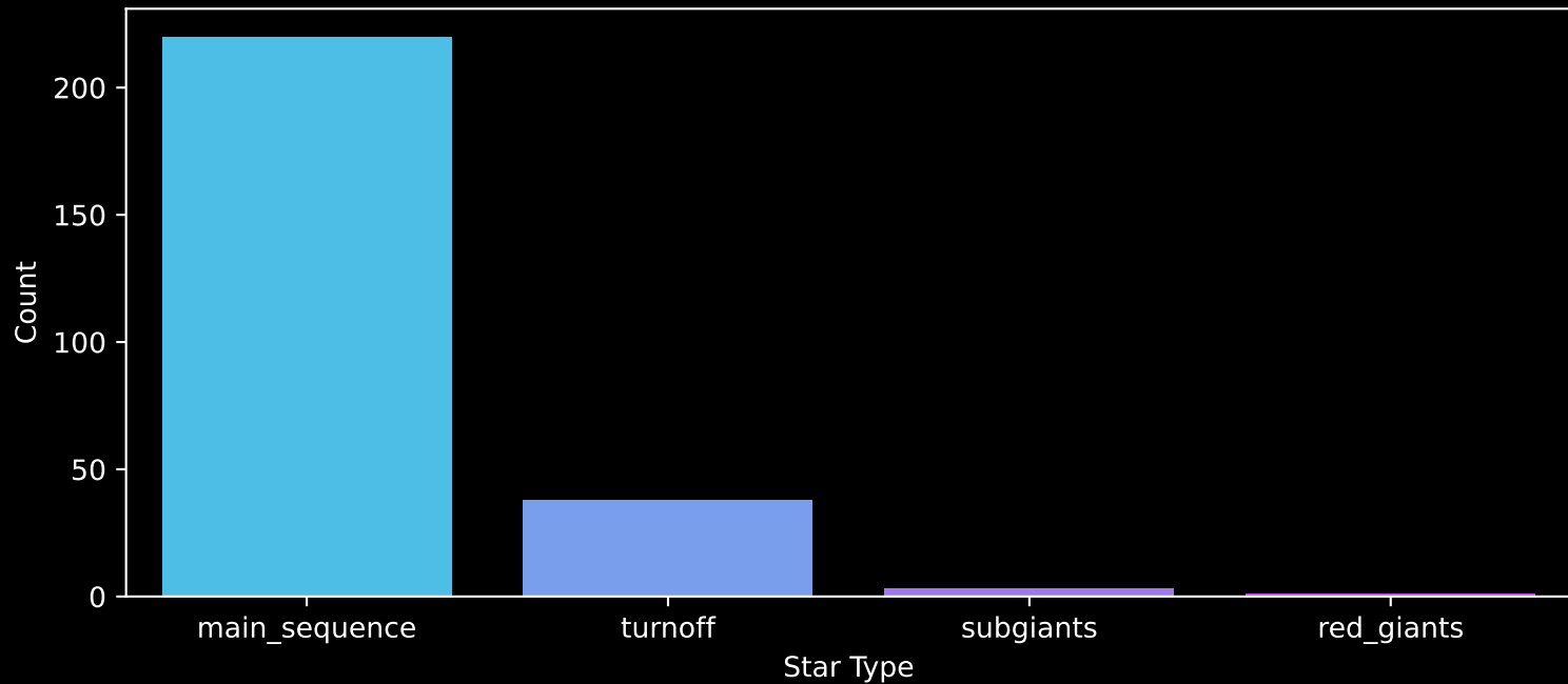
Gaia Cluster: [Ruprecht_91] Count plot of Star Type
