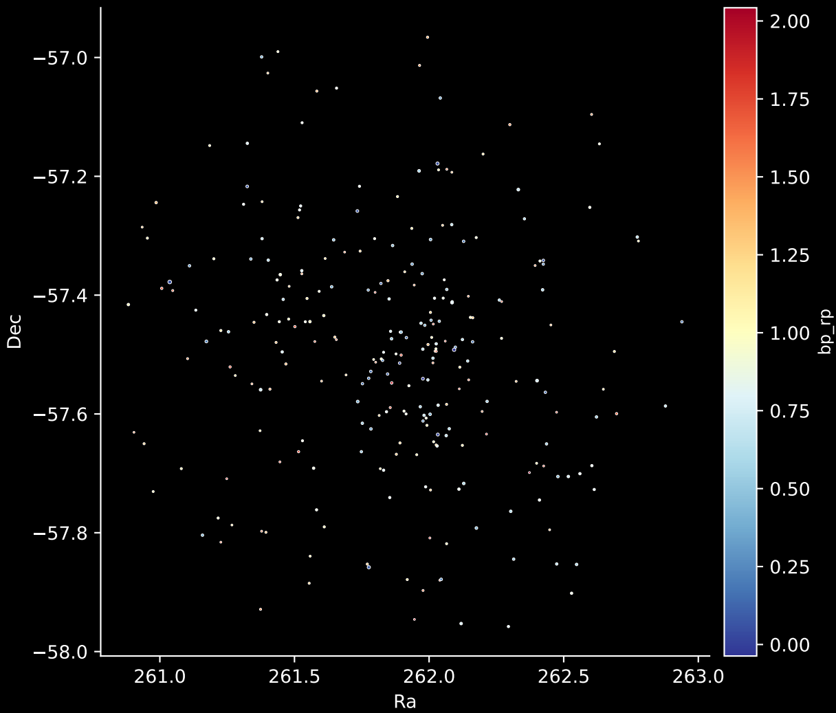
Gaia Cluster: [Ruprecht_91] Stars: 262
