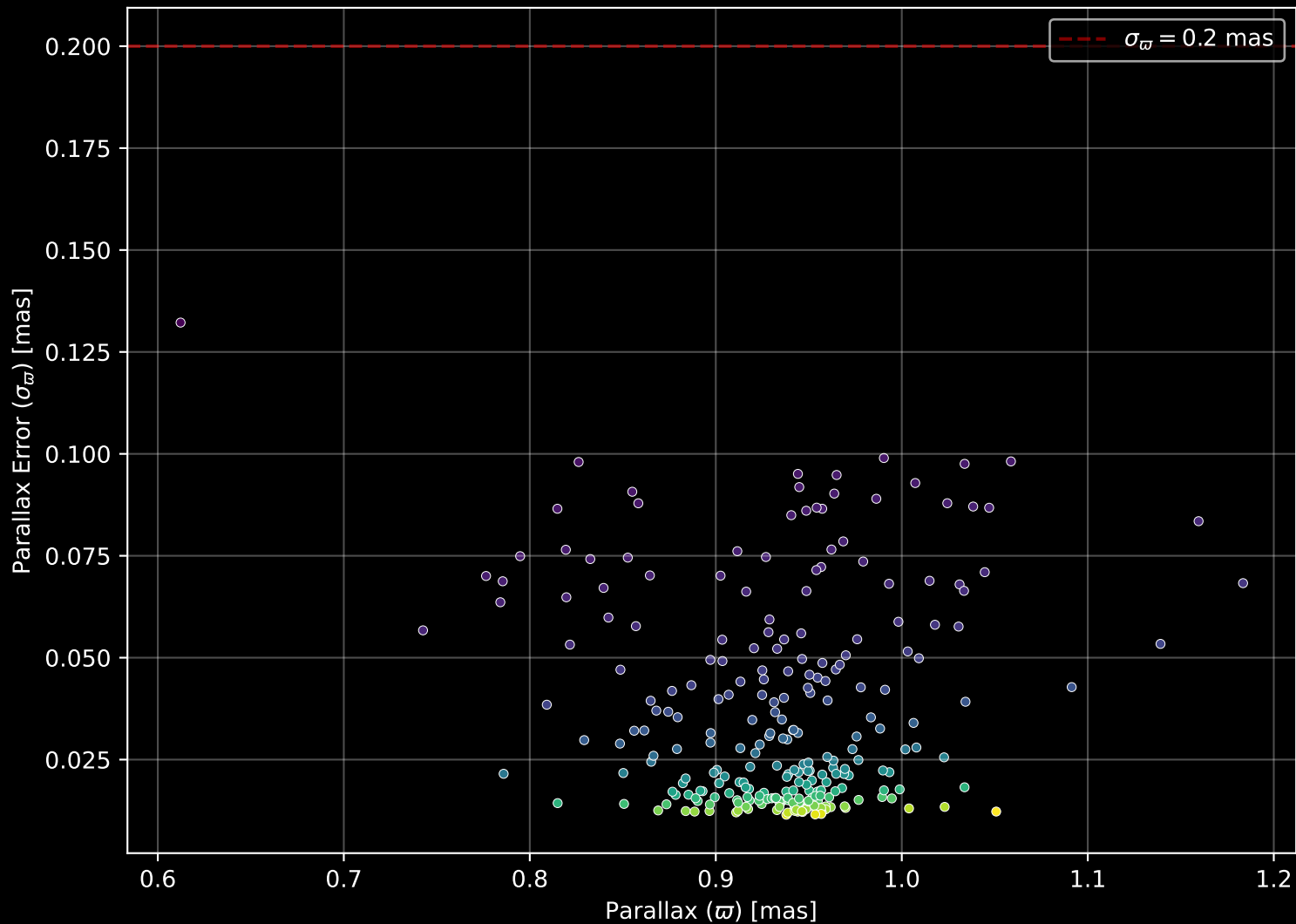
Gaia Cluster: [Ruprecht_91] Parallax Quality (n= 262)
