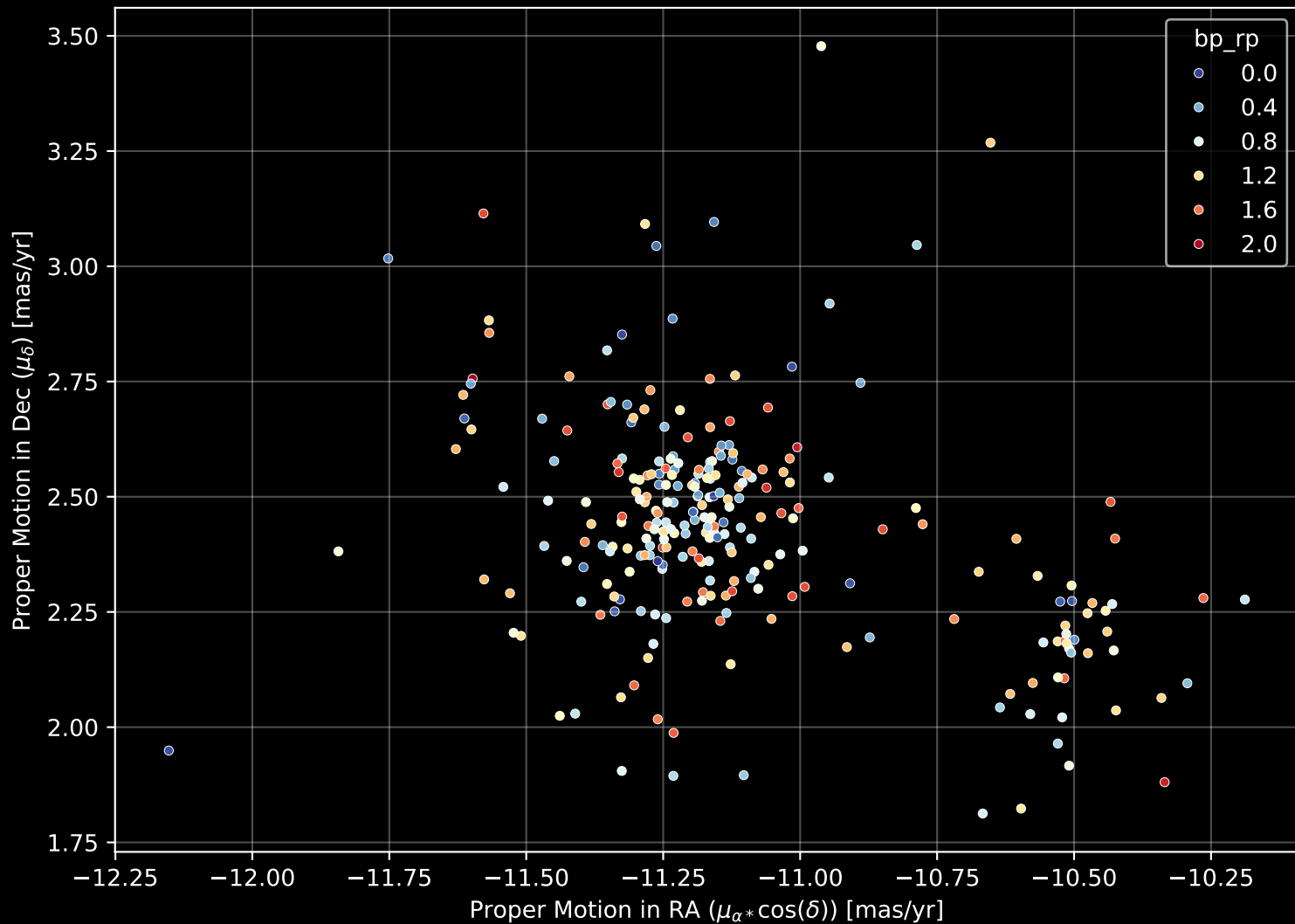
Gaia Cluster: [Ruprecht_91] Proper Motion Diagram (n= 262)
