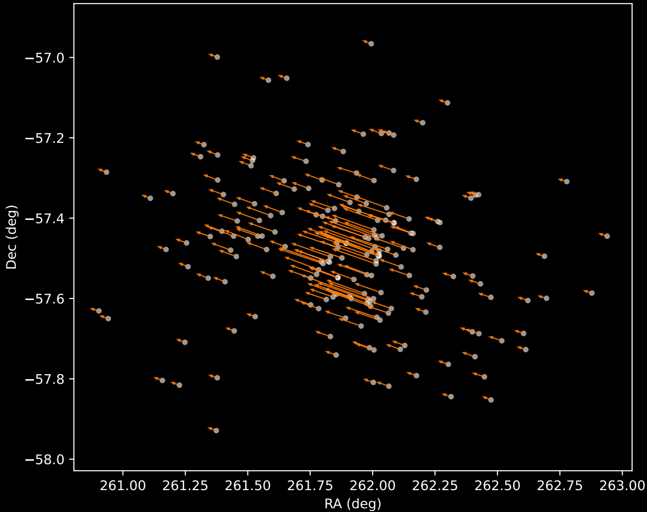
Gaia DR3 Cluster 2 Proper Motion Vectors (n=181)
