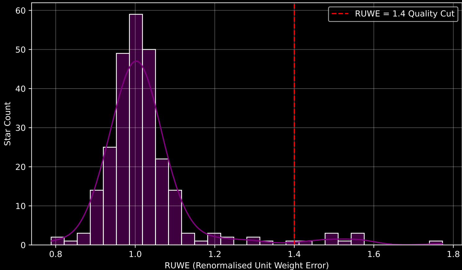
Gaia Cluster: [Ruprecht_91] RUWE Distribution (n= 261)
