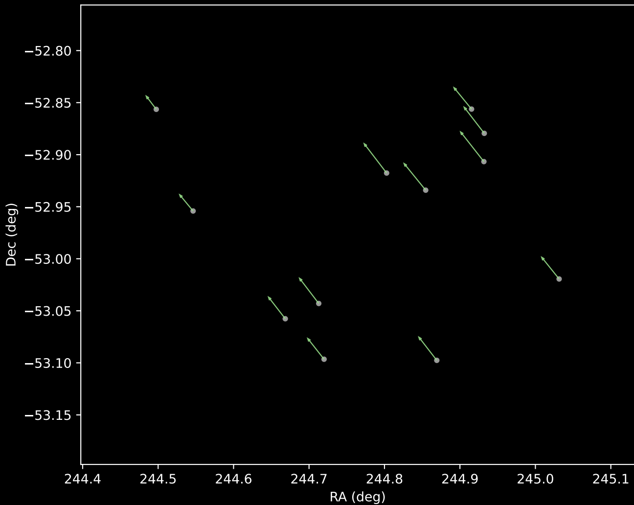
Gaia DR3 Cluster 5 Proper Motion Vectors (n=12)
