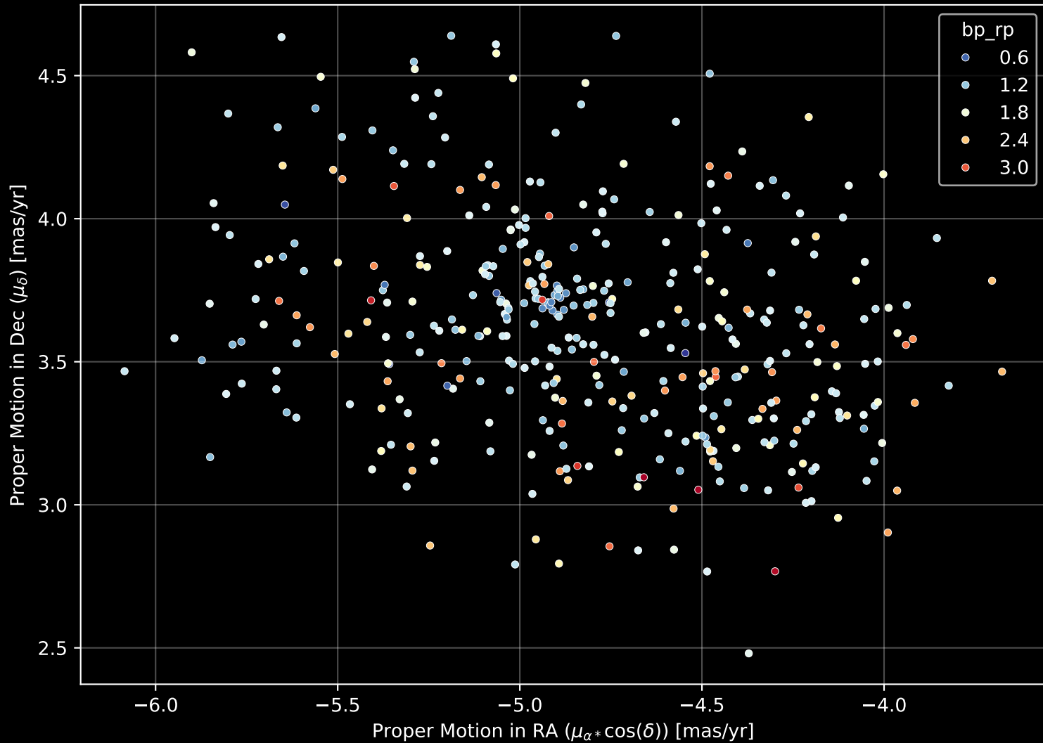
Gaia Cluster: [SAI_108] Proper Motion Diagram (n= 402)
