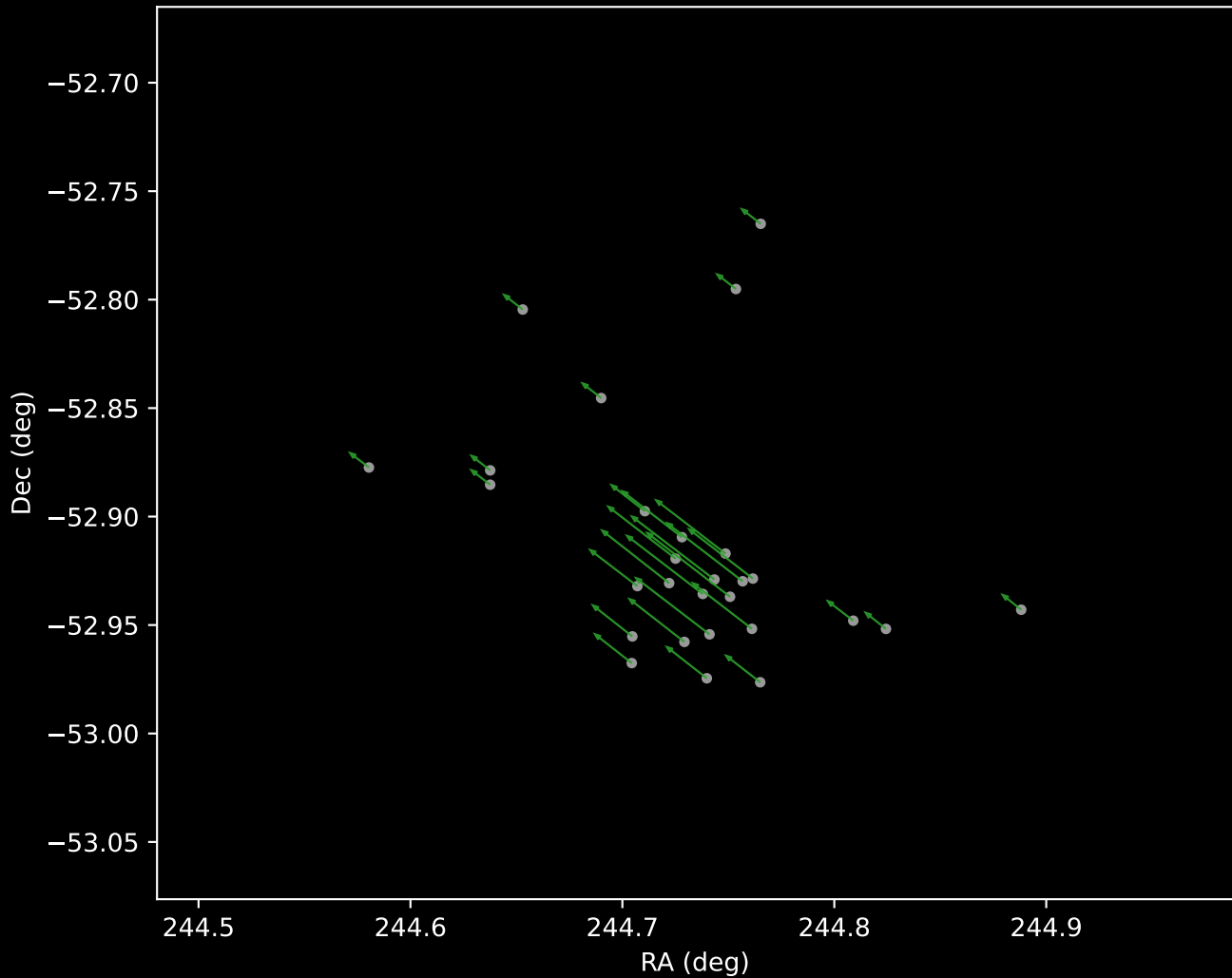
Gaia DR3 Cluster 24 Proper Motion Vectors (n=28)
