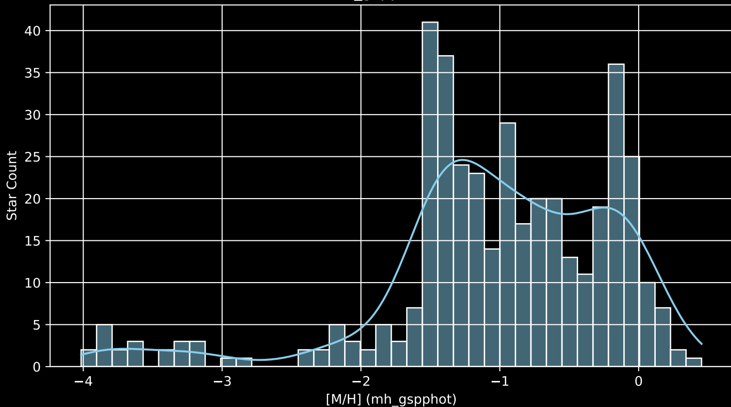
Gaia Cluster: [SAI_108 [M/H] (mh_gspphot) (n= 400)
