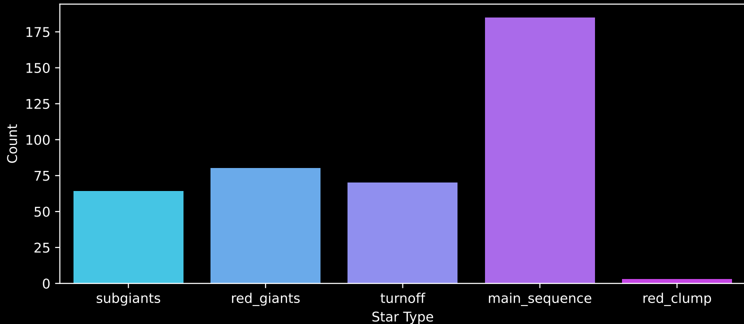
Gaia Cluster: [SAI_108] Count plot of Star Type
