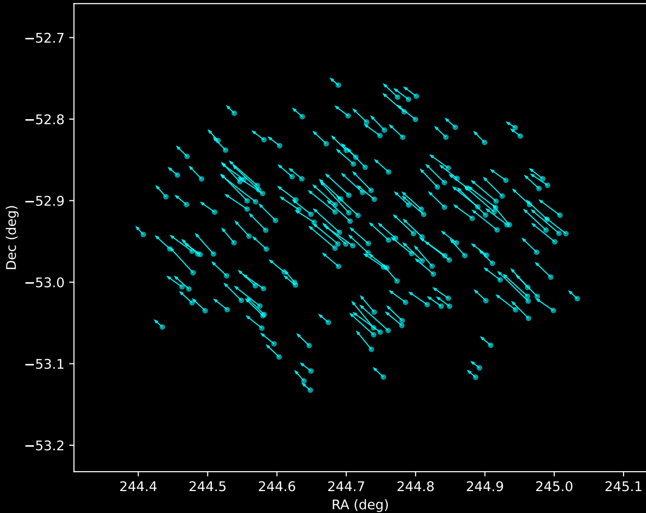
Gaia DR3 Noise Stream Proper Motion Vectors (n=178)
