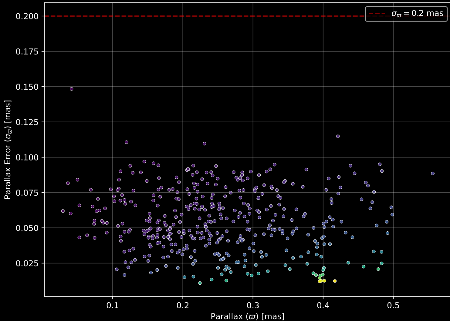
Gaia Cluster: [SAI_108] Parallax Quality (n= 402)
