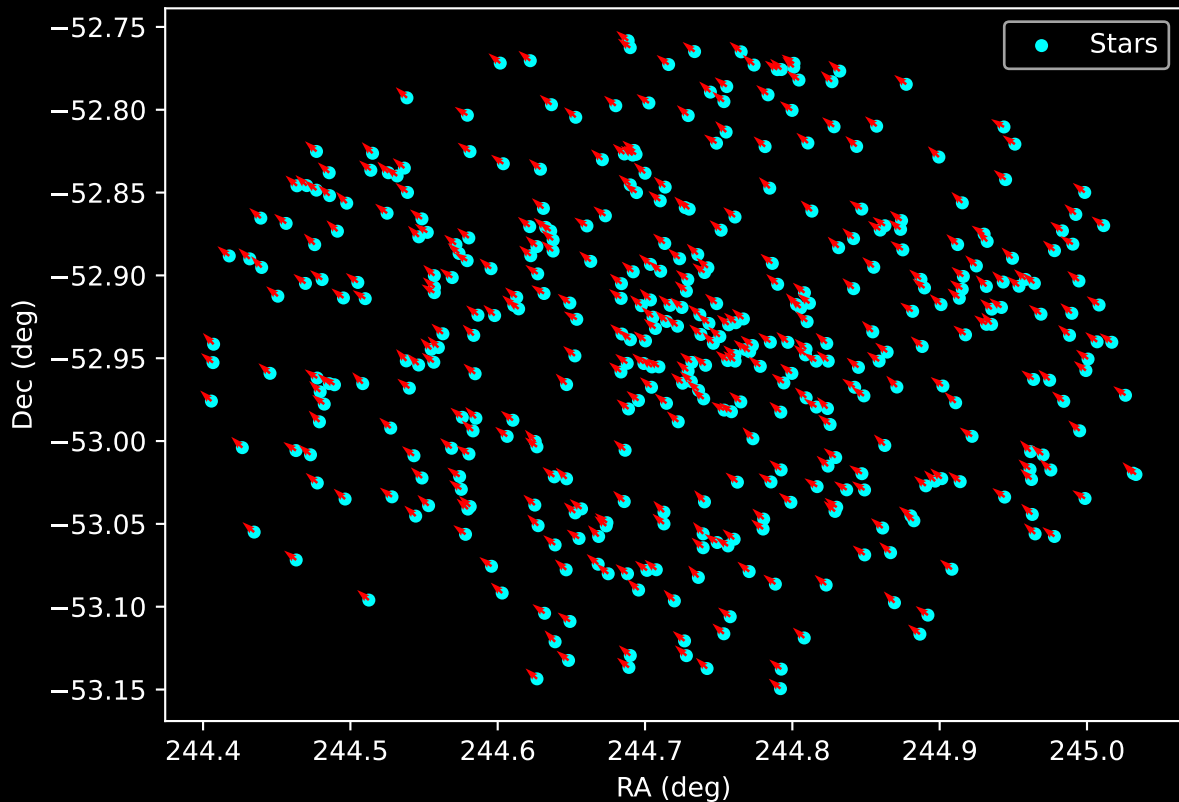
Gaia Cluster: [SAI_108] Proper Motion Vectors for Gaia Star Field (n= 402)
