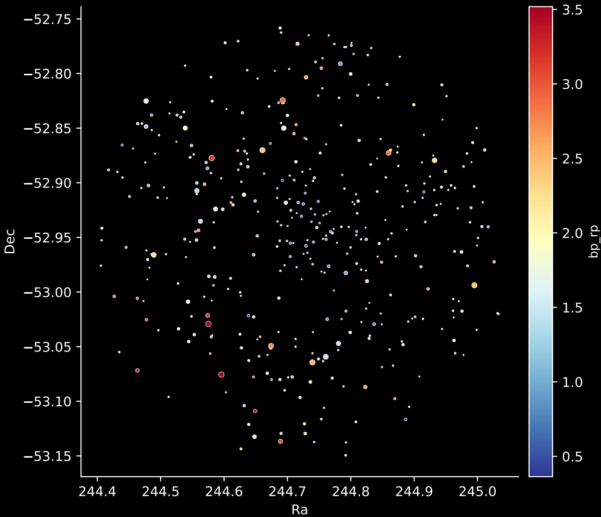
Gaia Cluster: [SAI_108] Stars: 402
