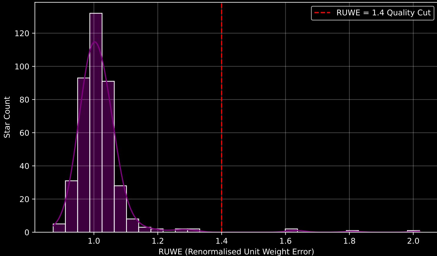
Gaia Cluster: [SAI_108] RUWE Distribution (n= 401)
