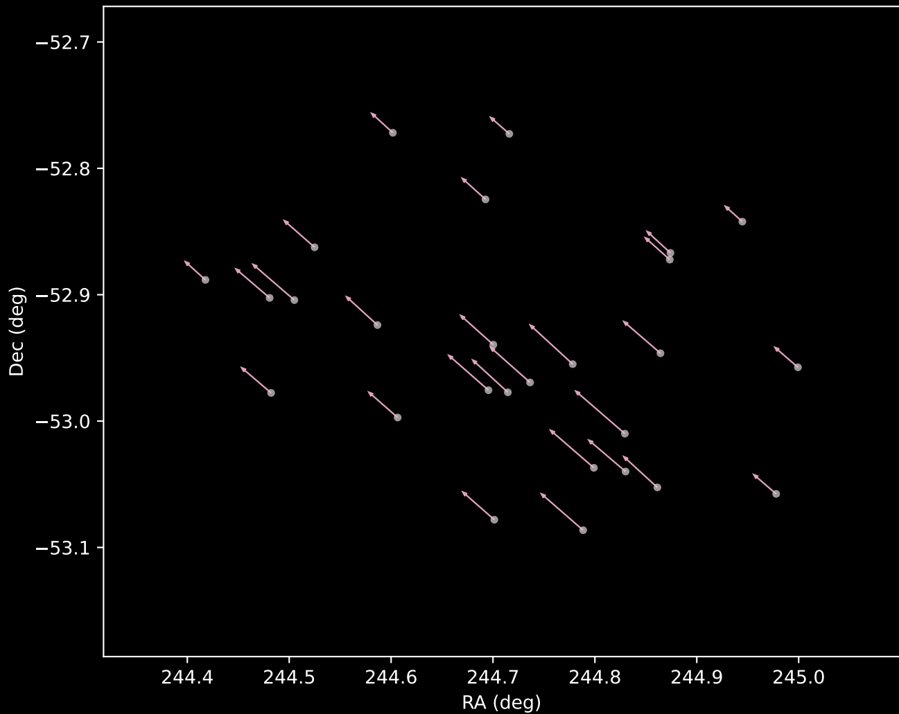
Gaia DR3 Cluster 13 Proper Motion Vectors (n=27)
