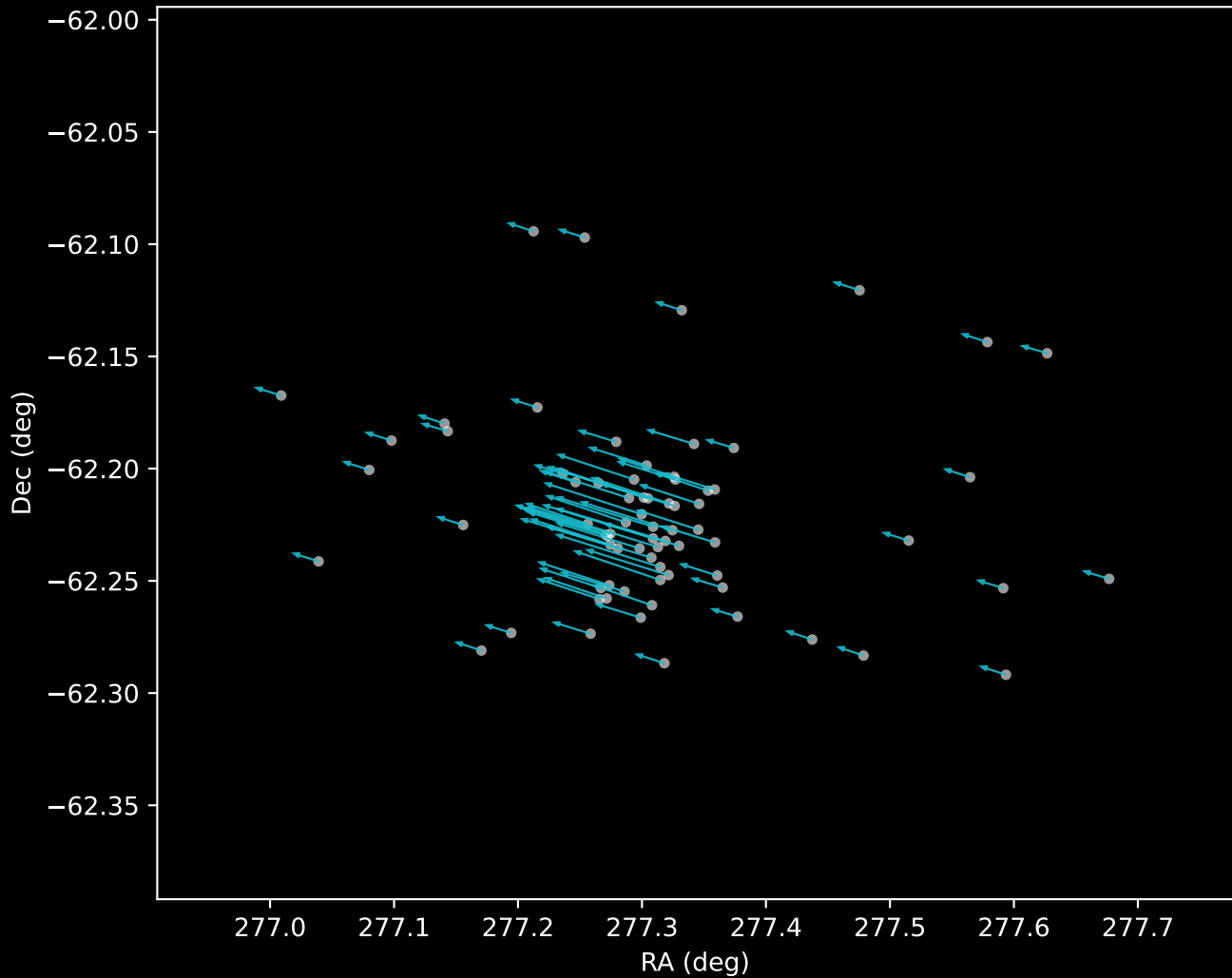
Gaia DR3 Cluster 18 Proper Motion Vectors (n=74)
