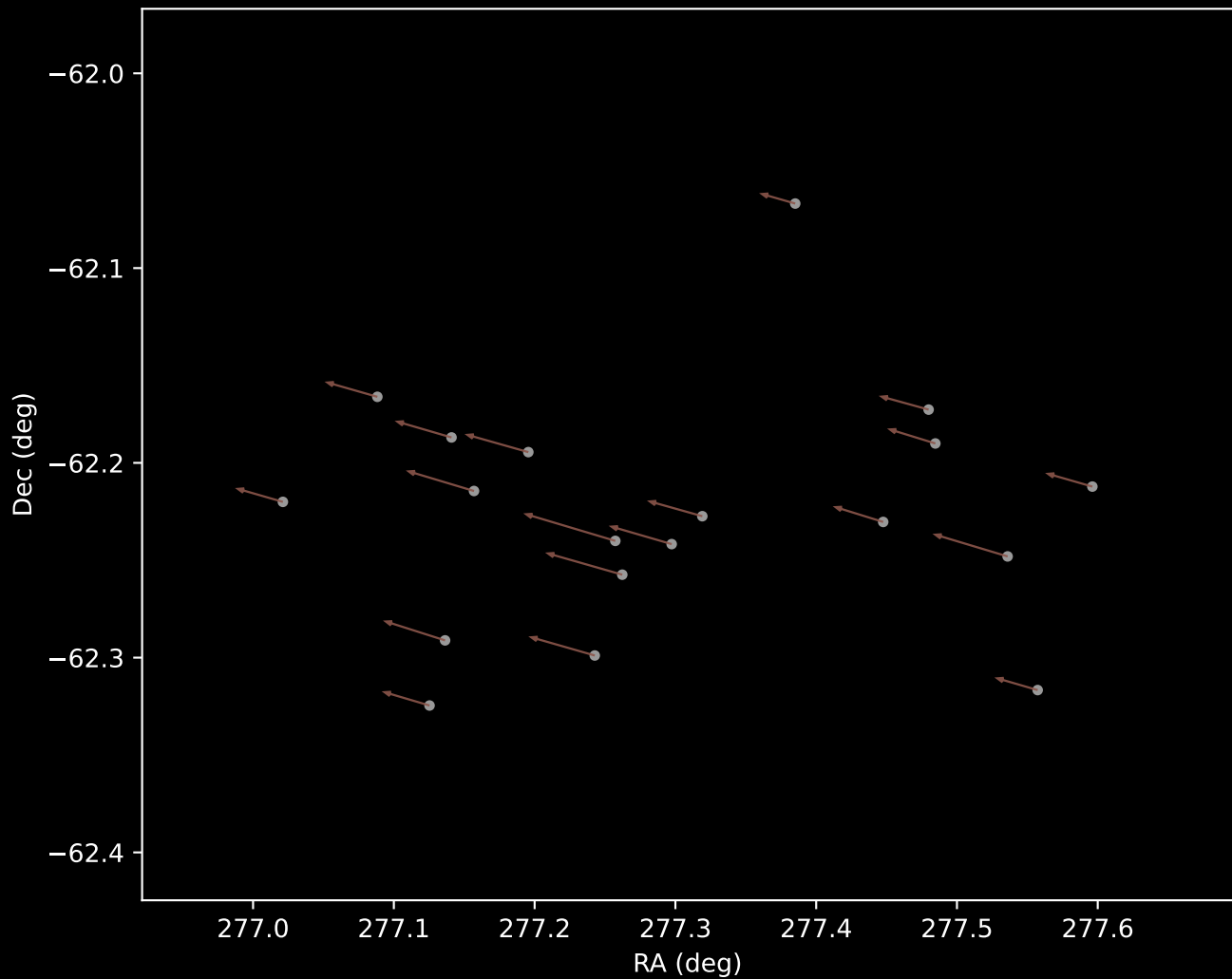
Gaia DR3 Cluster 10 Proper Motion Vectors (n=19)
