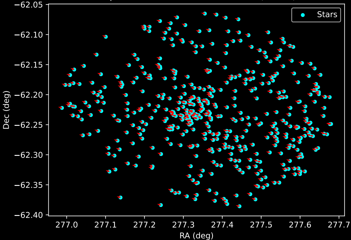
Gaia Cluster: [SAI_116] Proper Motion Vectors for Gaia Star Field (n= 472)
