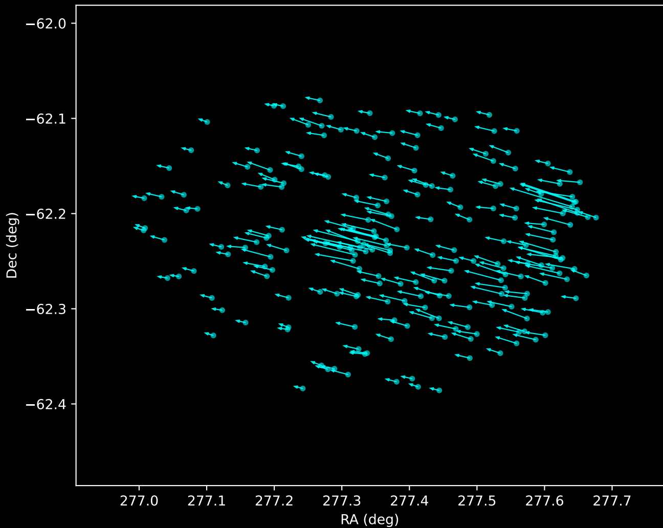
Gaia DR3 Noise Stream Proper Motion Vectors (n=214)
