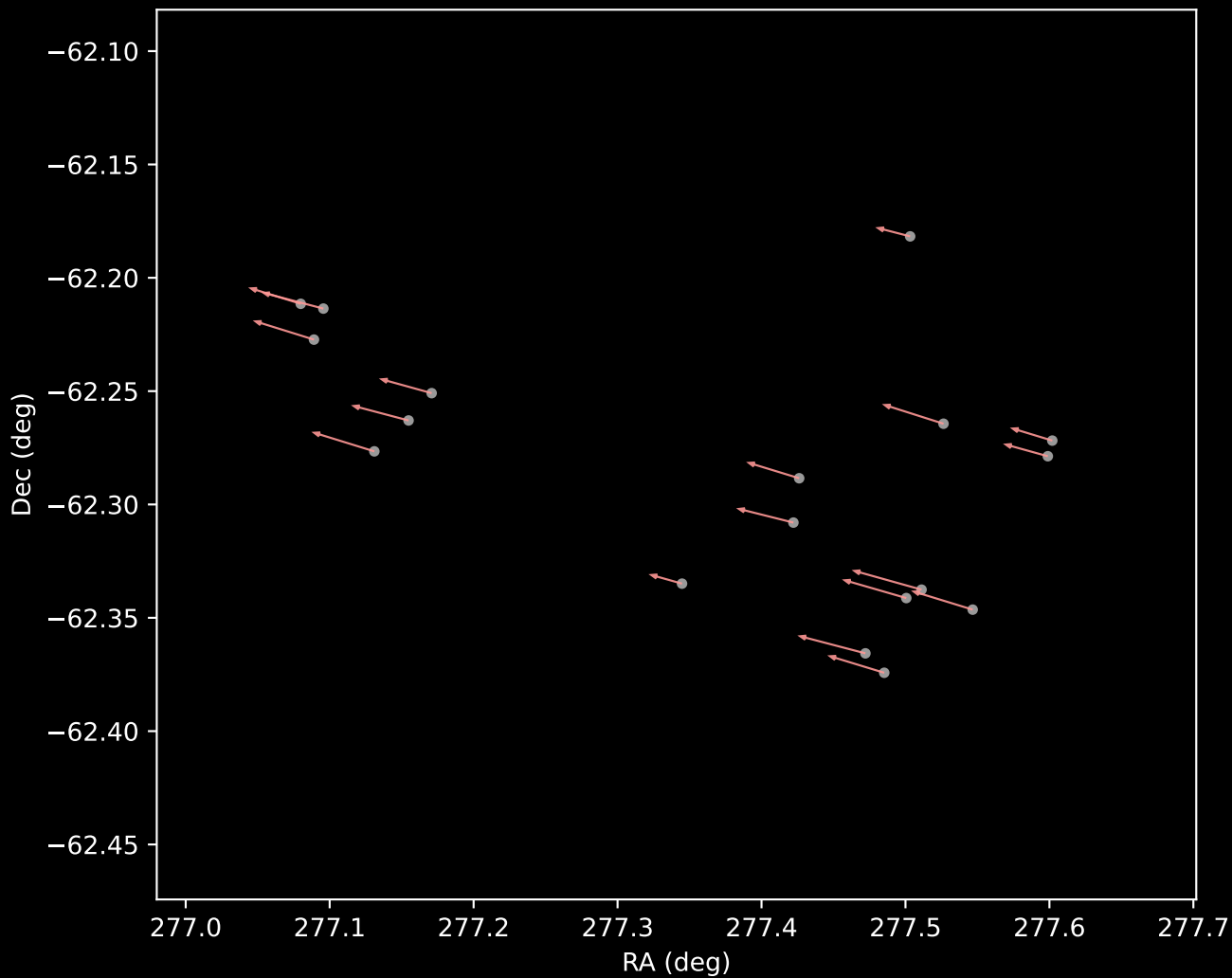
Gaia DR3 Cluster 7 Proper Motion Vectors (n=18)
