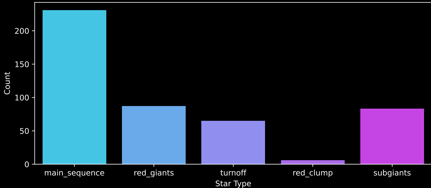
Gaia Cluster: [SAI_116] Count plot of Star Type
