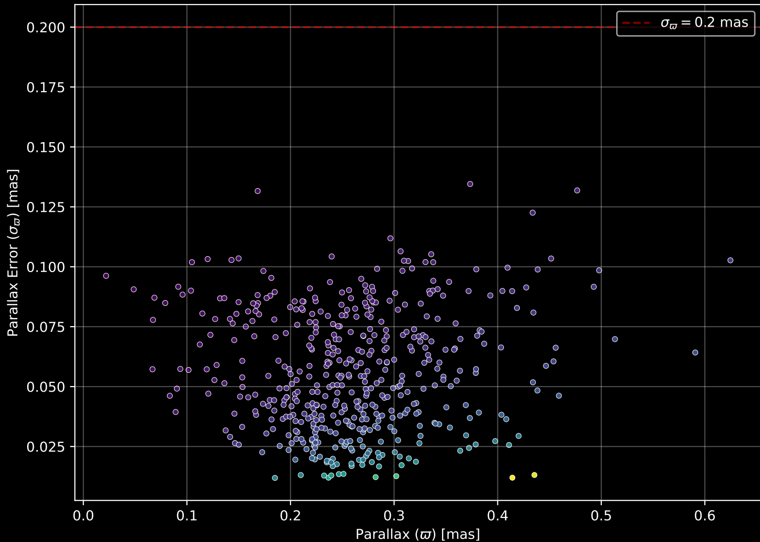
Gaia Cluster: [SAI_116] Parallax Quality (n= 472)
