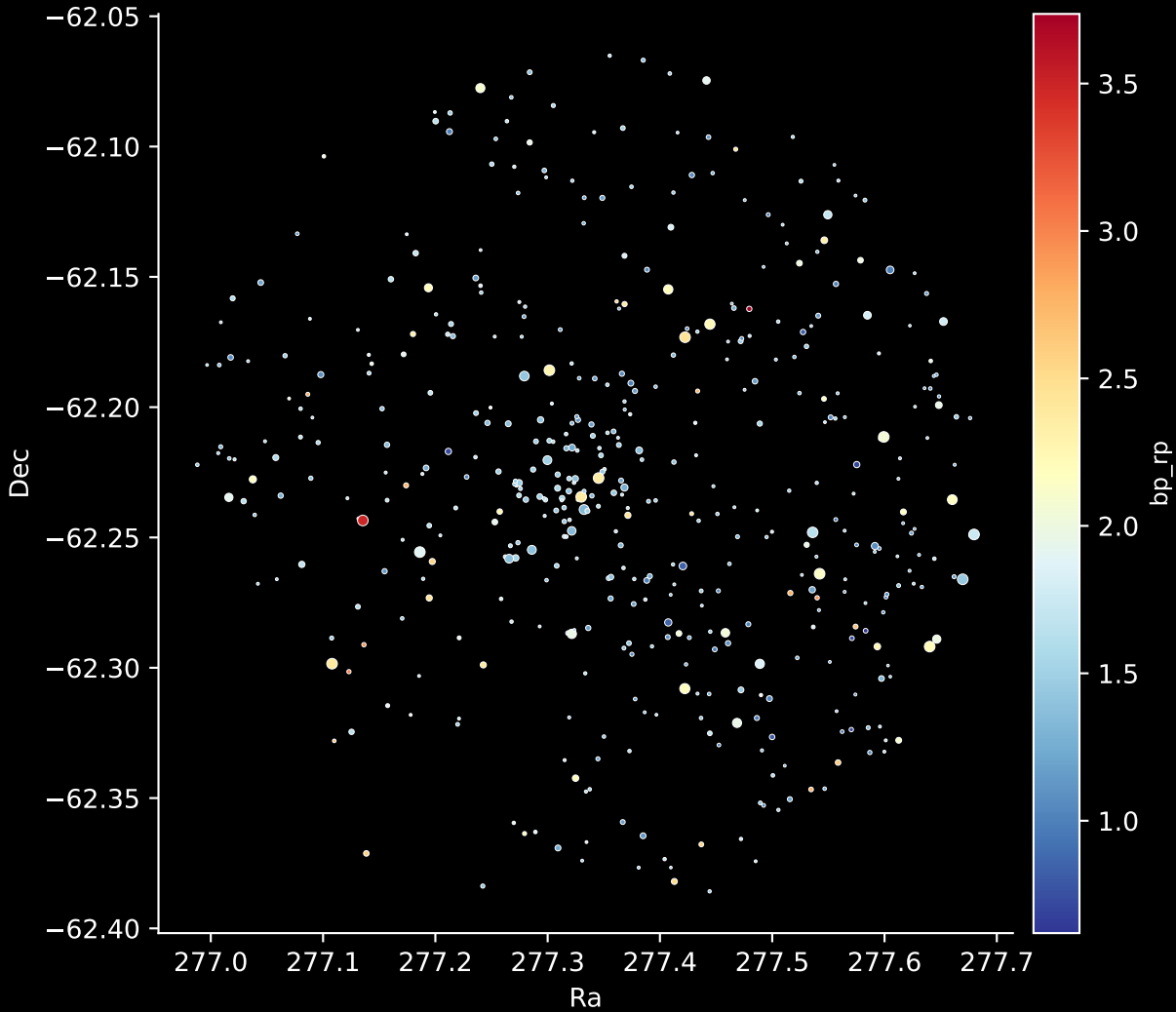
Gaia Cluster: [SAI_116] Stars: 472
