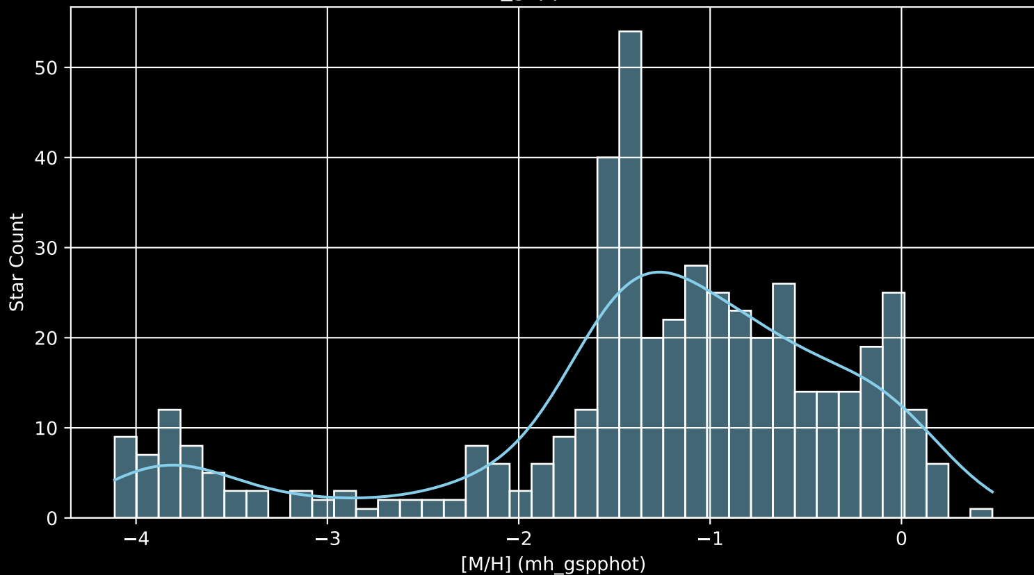
Gaia Cluster: [SAI_116 [M/H] (mh_gspphot) (n= 471)
