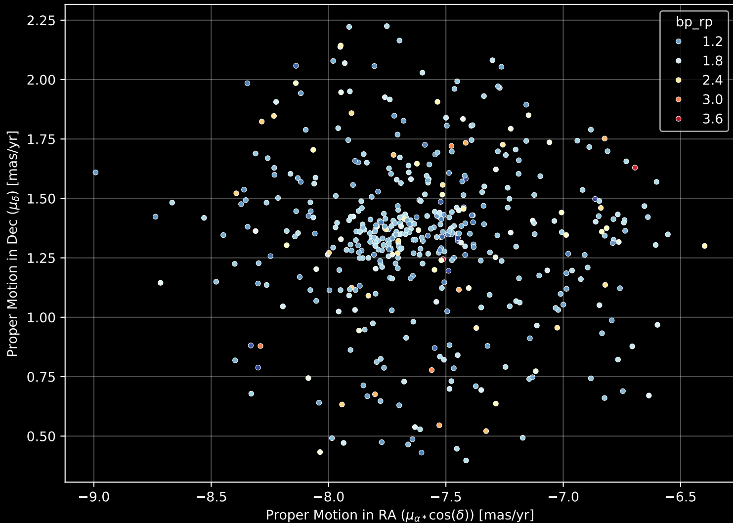
Gaia Cluster: [SAI_116] Proper Motion Diagram (n= 472)
