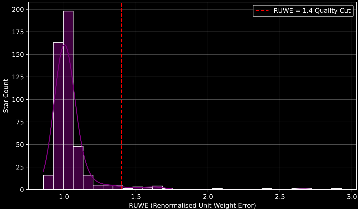
Gaia Cluster: [SAI_116] RUWE Distribution (n= 472)
