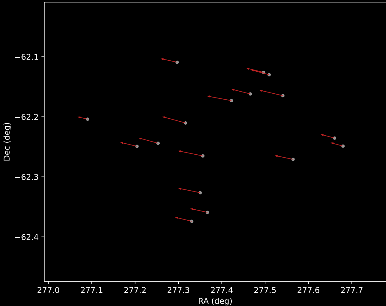
Gaia DR3 Cluster 6 Proper Motion Vectors (n=17)
