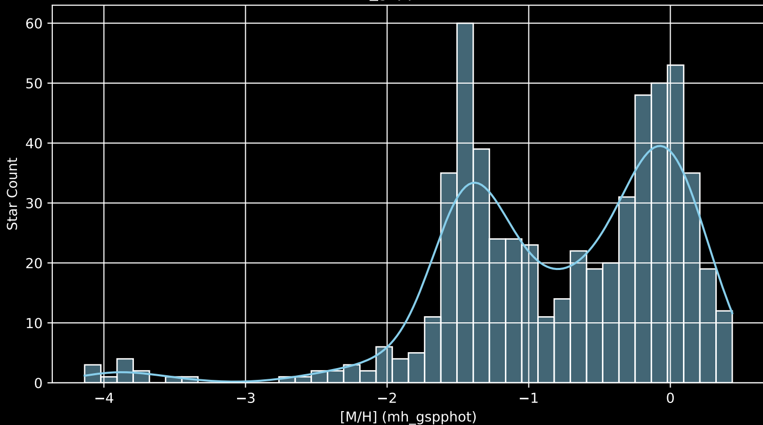
Gaia Cluster: [SAI_132 [M/H] (mh_gspphot) (n= 588)
