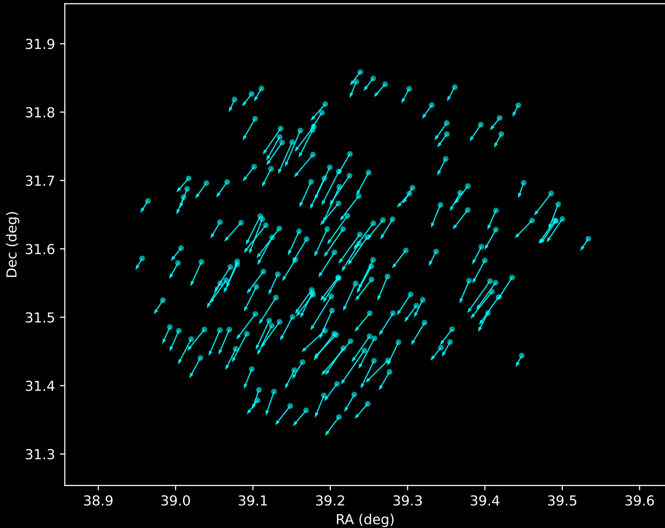
Gaia DR3 Noise Stream Proper Motion Vectors (n=168)
