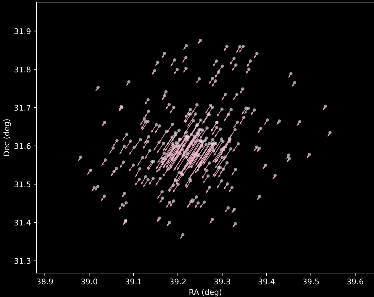
Gaia DR3 Cluster 13 Proper Motion Vectors (n=239)
