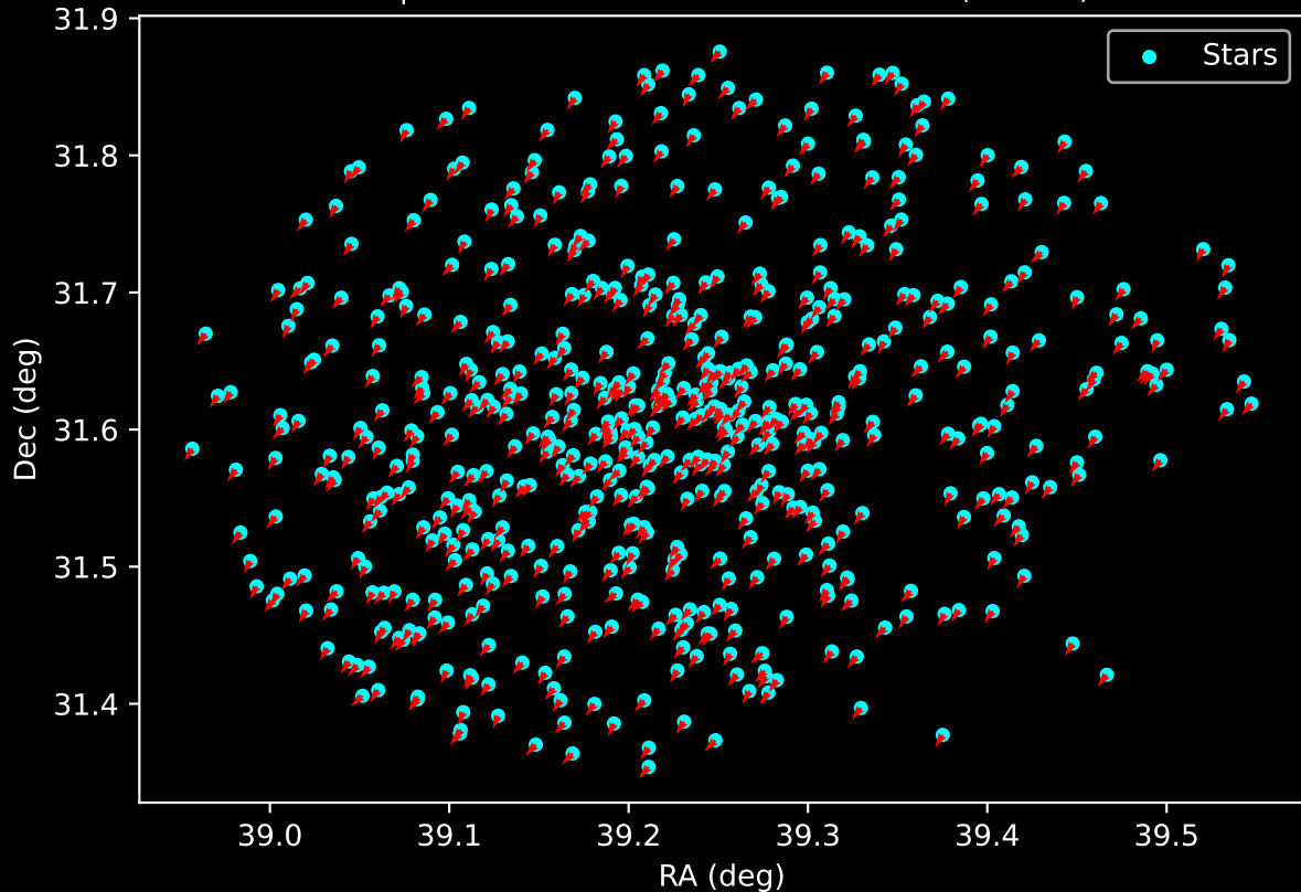
Gaia Cluster: [SAI_132] Proper Motion Vectors for Gaia Star Field (n= 599)
