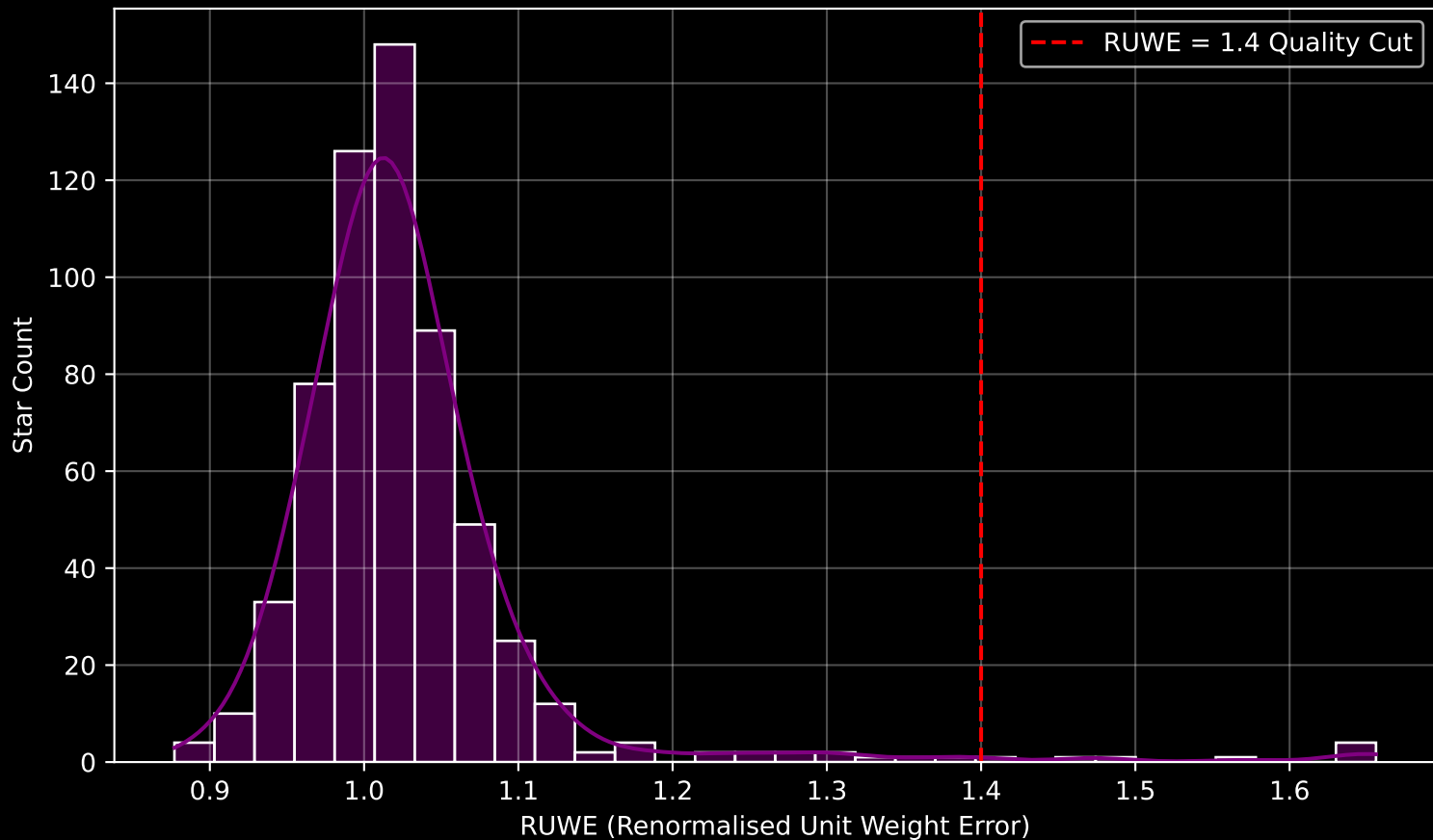
Gaia Cluster: [SAI_132] RUWE Distribution (n= 599)
