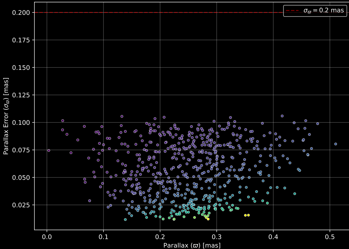
Gaia Cluster: [SAI_132] Parallax Quality (n= 599)
