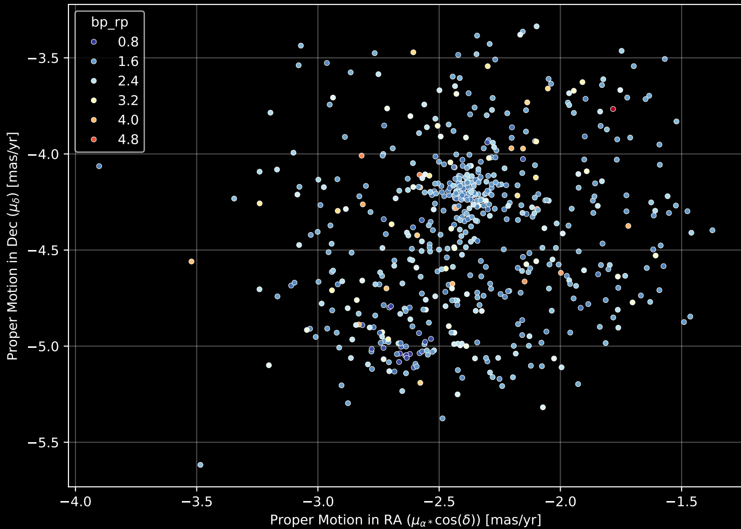
Gaia Cluster: [SAI_132] Proper Motion Diagram (n= 599)
