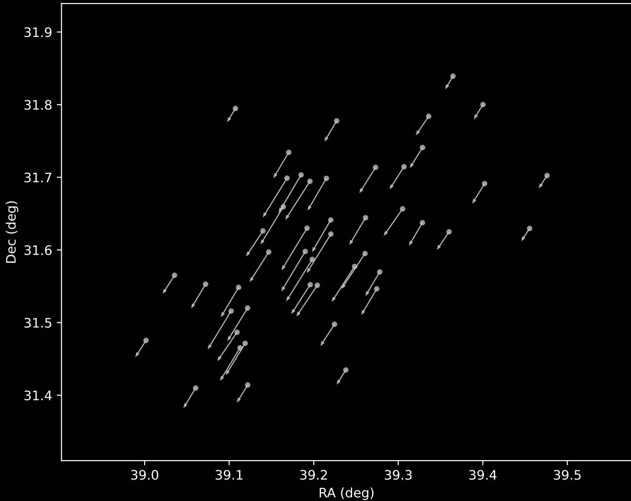
Gaia DR3 Cluster 15 Proper Motion Vectors (n=47)
