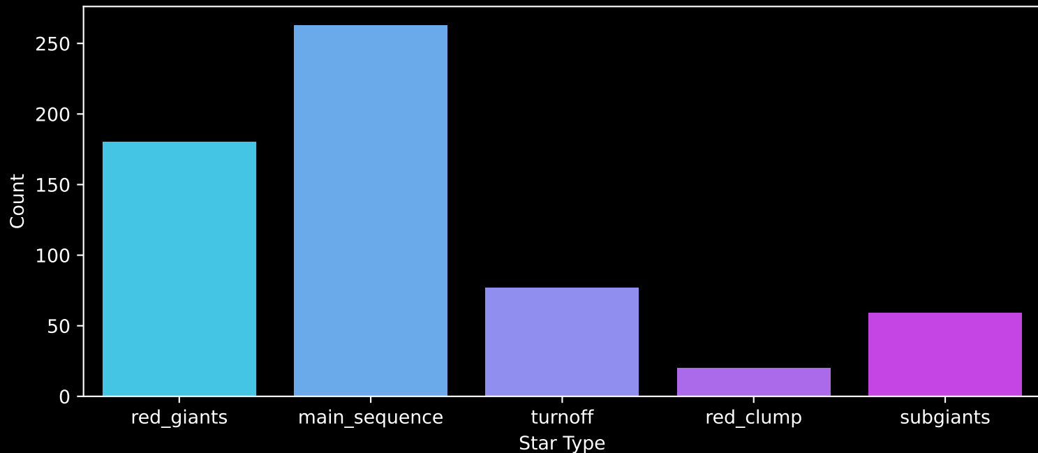
Gaia Cluster: [SAI_132] Count plot of Star Type
