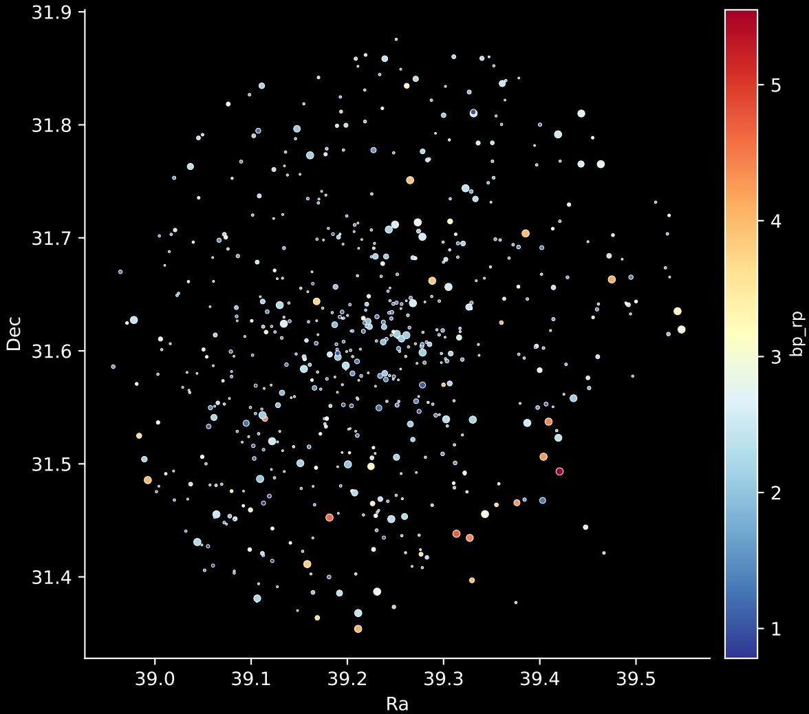
Gaia Cluster: [SAI_132] Stars: 599
