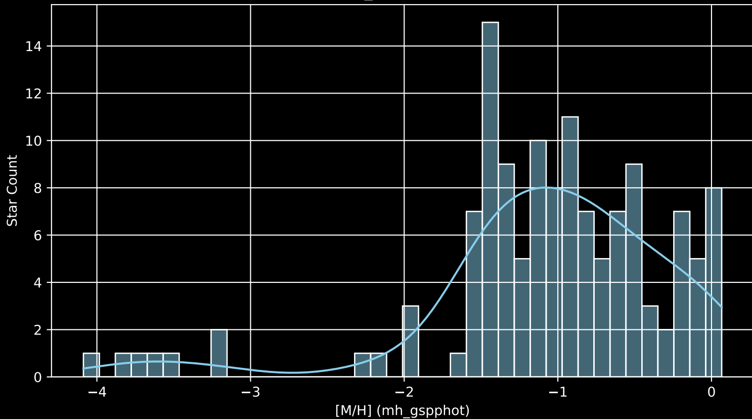
Gaia Cluster: [SAI_149 [M/H] (mh_gspphot) (n= 131)
