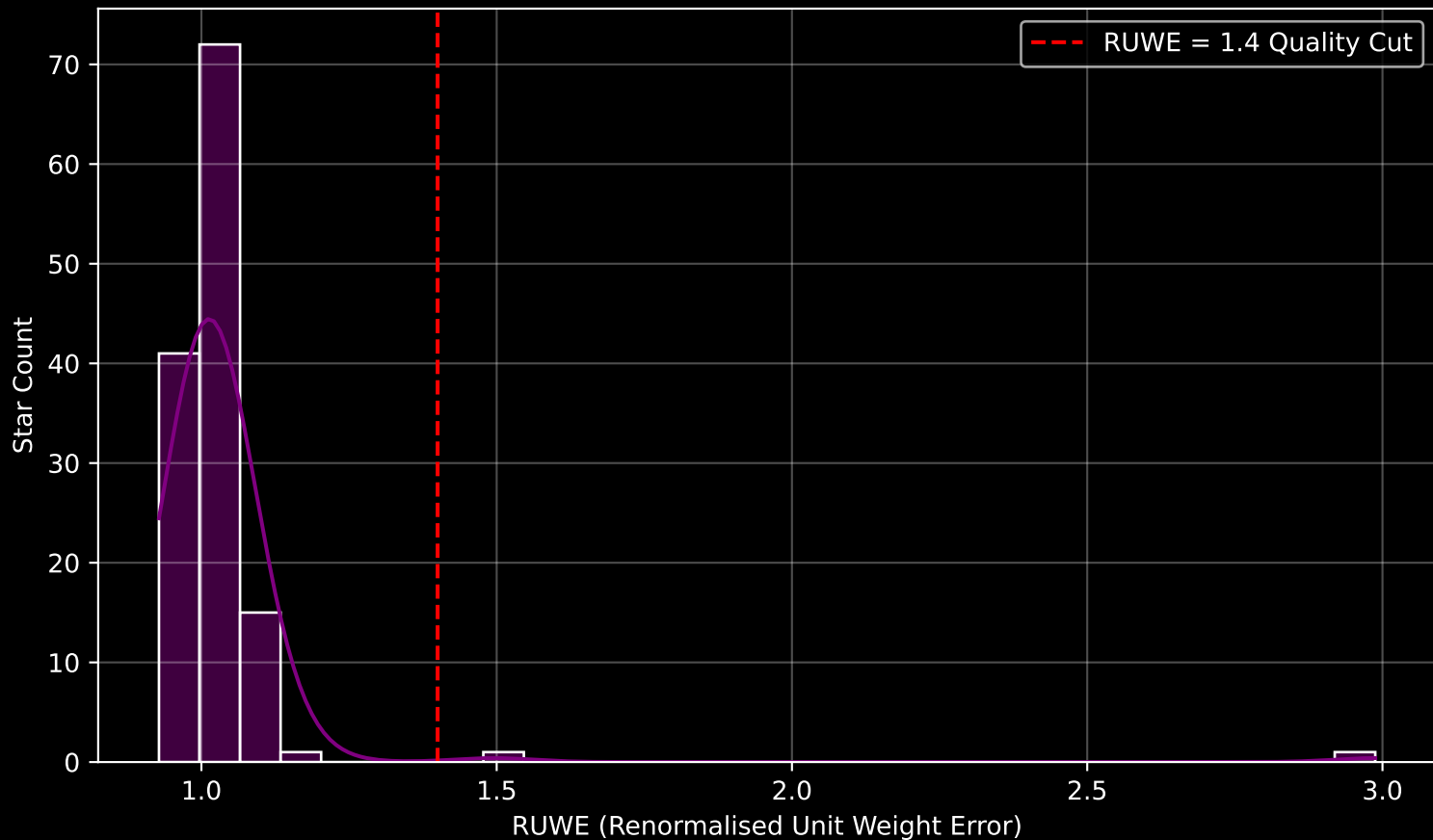
Gaia Cluster: [SAI_149] RUWE Distribution (n= 131)
