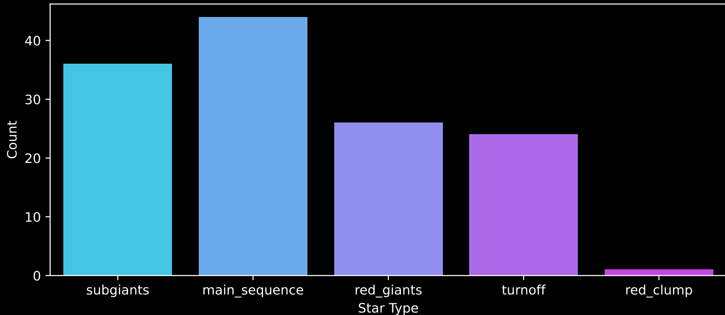
Gaia Cluster: [SAI_149] Count plot of Star Type
