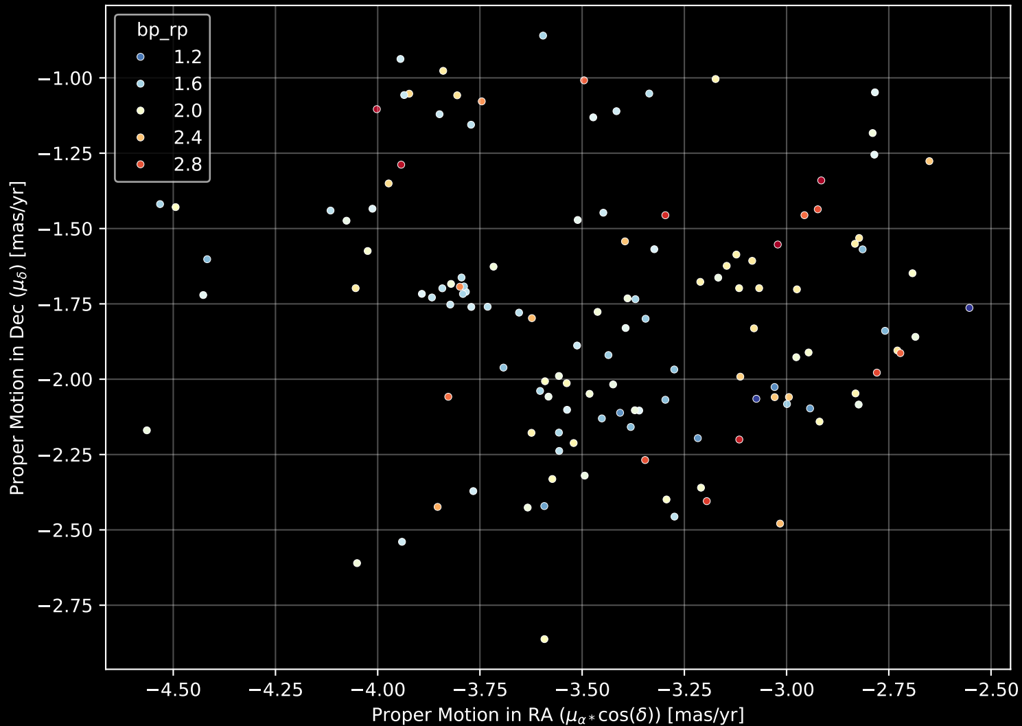
Gaia Cluster: [SAI_149] Proper Motion Diagram (n= 131)
