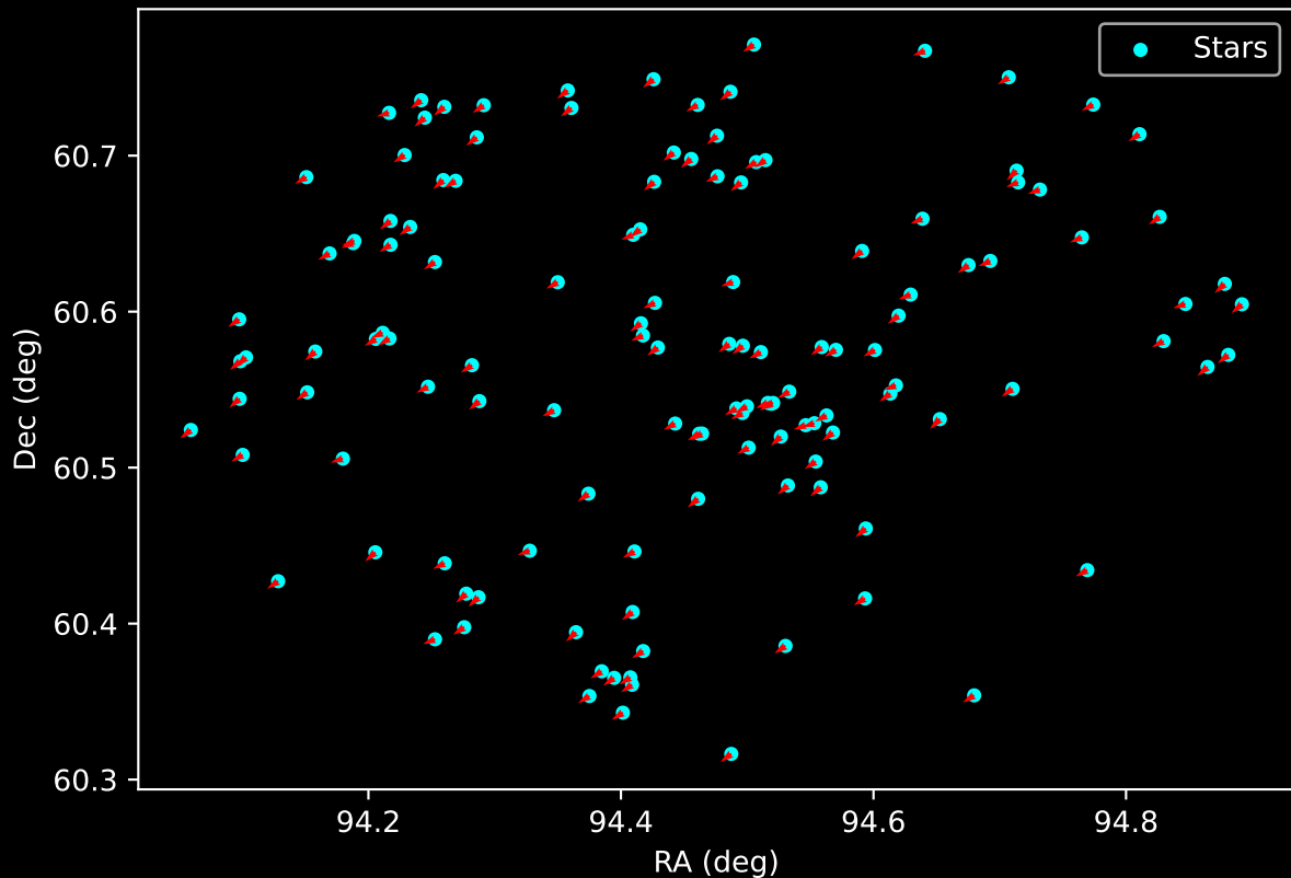
Gaia Cluster: [SAI_149] Proper Motion Vectors for Gaia Star Field (n= 131)
