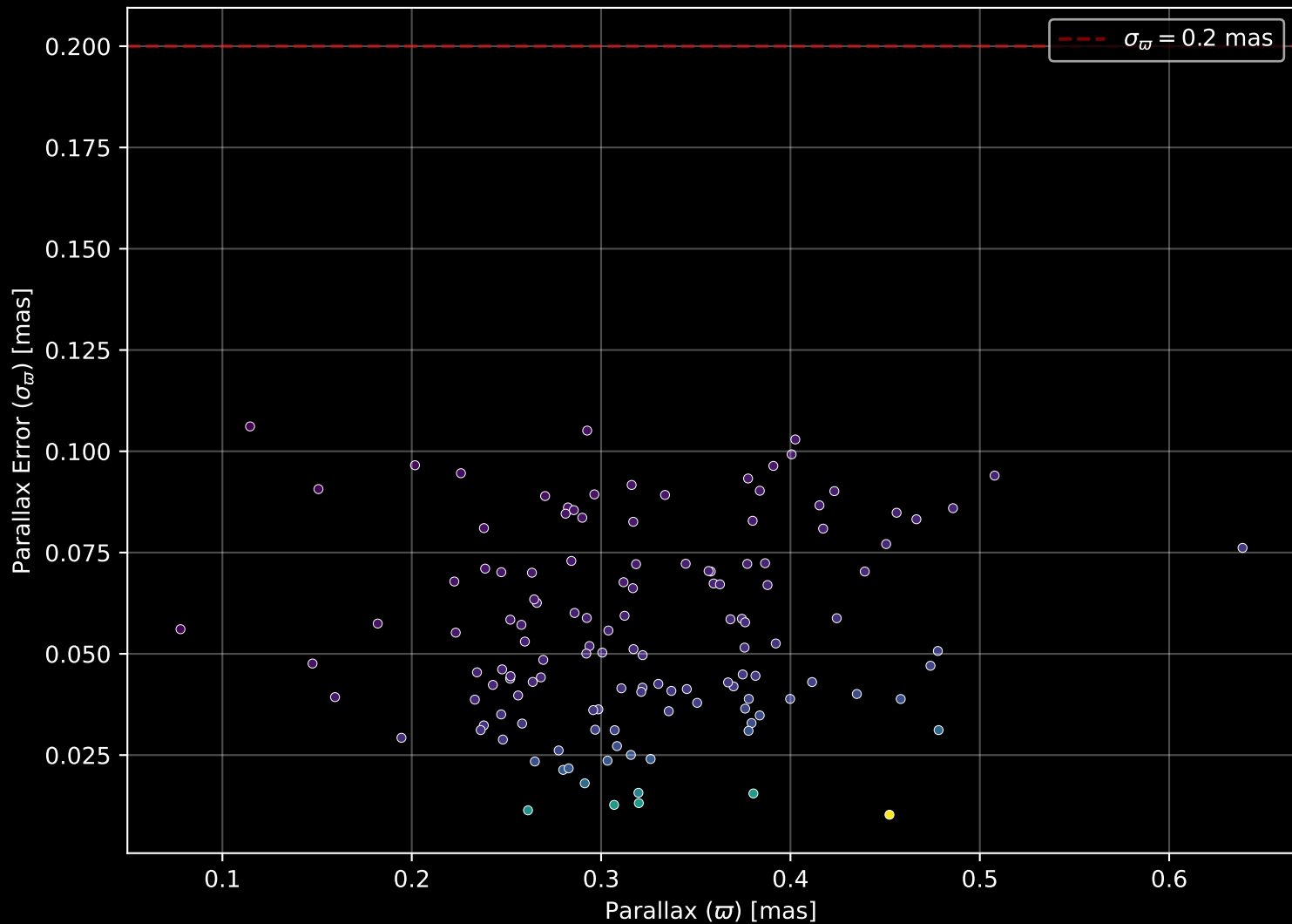
Gaia Cluster: [SAI_149] Parallax Quality (n= 131)
