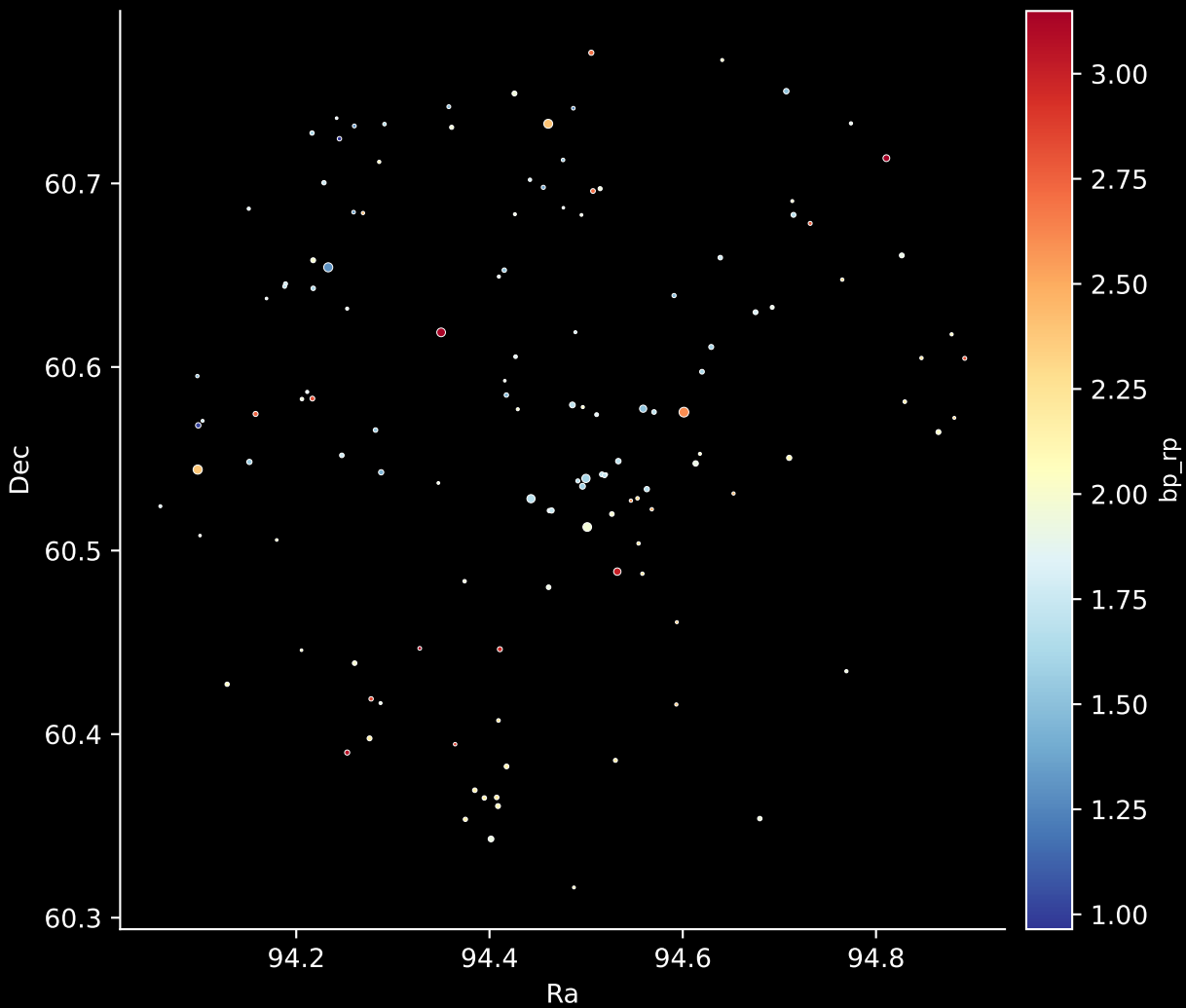
Gaia Cluster: [SAI_149] Stars: 131
