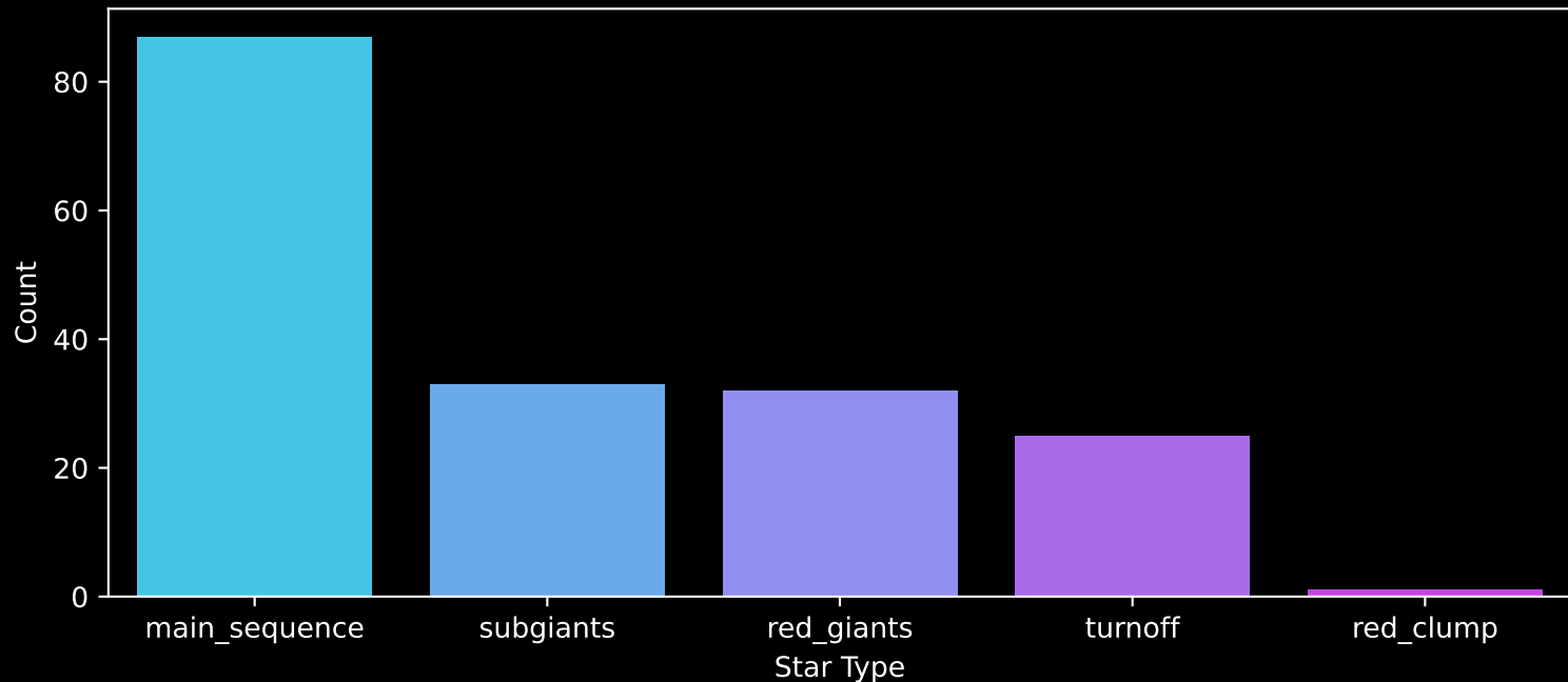
Gaia Cluster: [SAI_16] Count plot of Star Type
