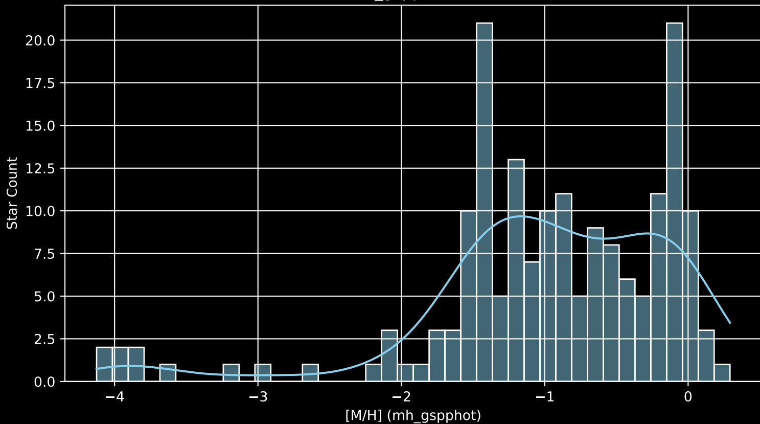
Gaia Cluster: [SAI_16 [M/H] (mh_gspphot) (n= 178)
