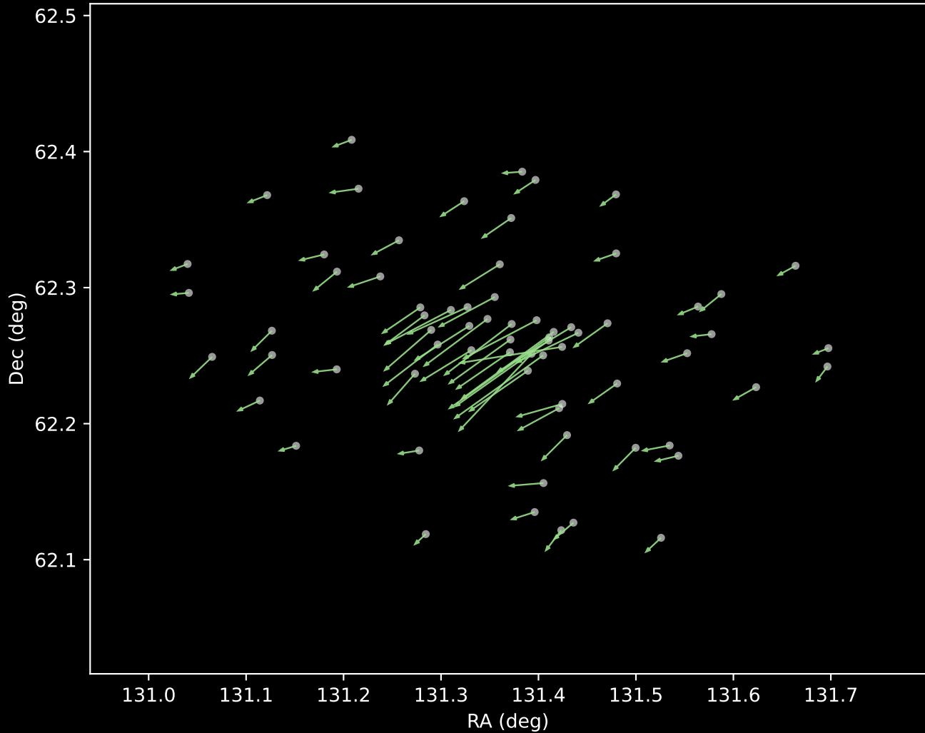
Gaia DR3 Cluster 5 Proper Motion Vectors (n=69)
