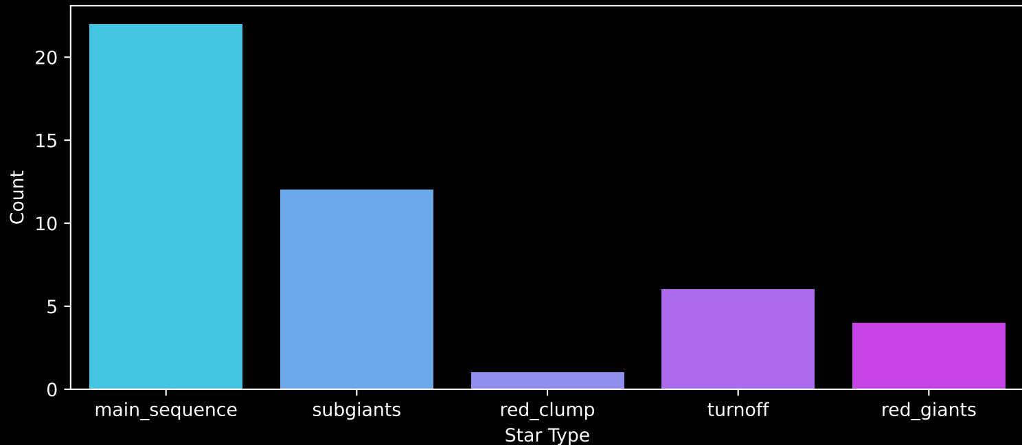
Gaia Cluster: [SAI_17] Count plot of Star Type
