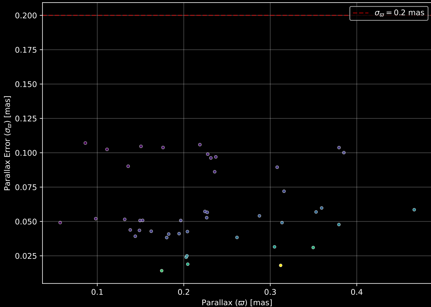
Gaia Cluster: [SAI_17] Parallax Quality (n= 45)
