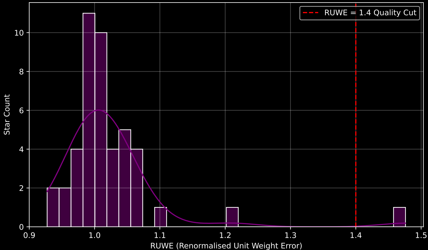
Gaia Cluster: [SAI_17] RUWE Distribution (n= 45)
