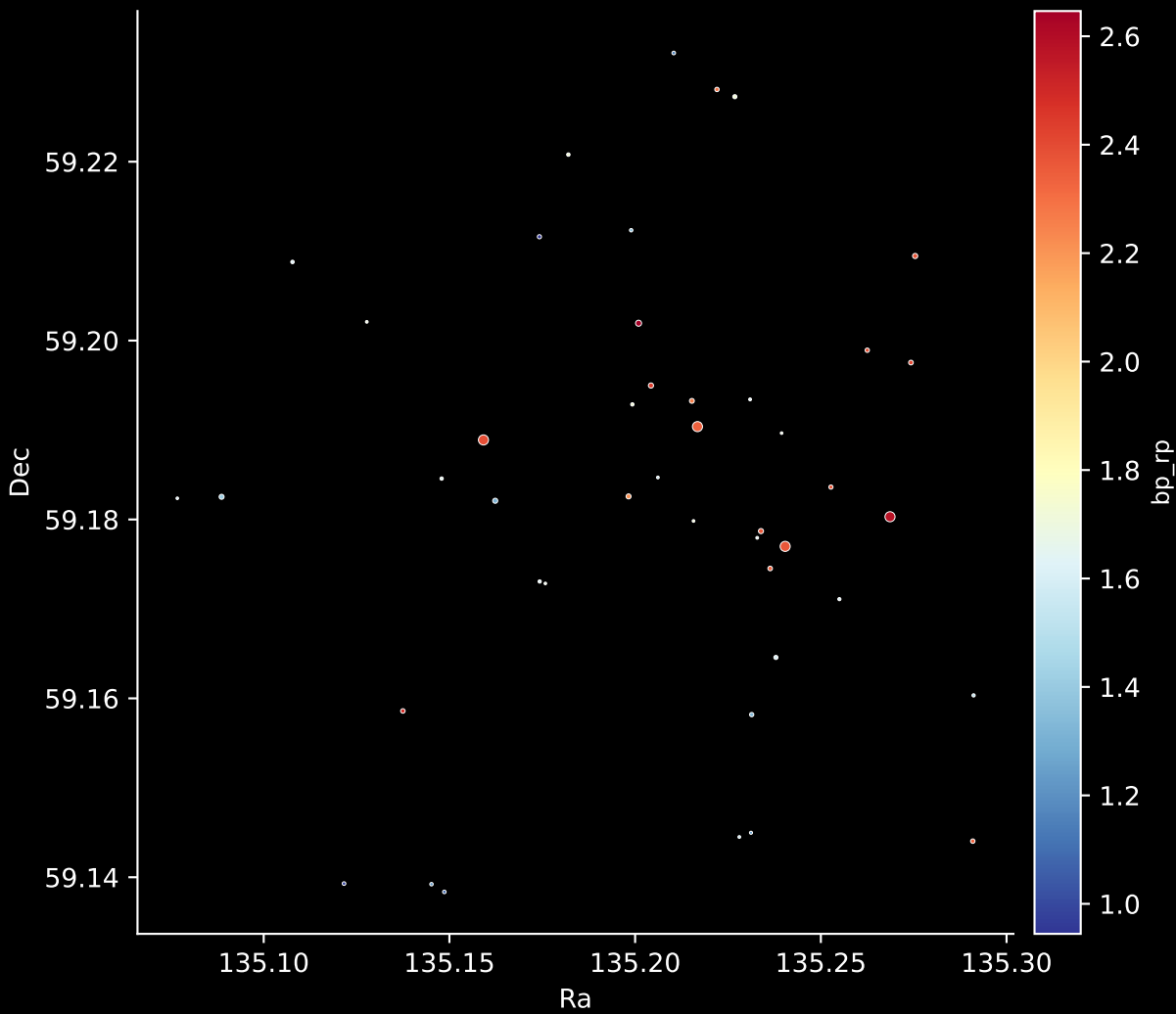
Gaia Cluster: [SAI_17] Stars: 45
