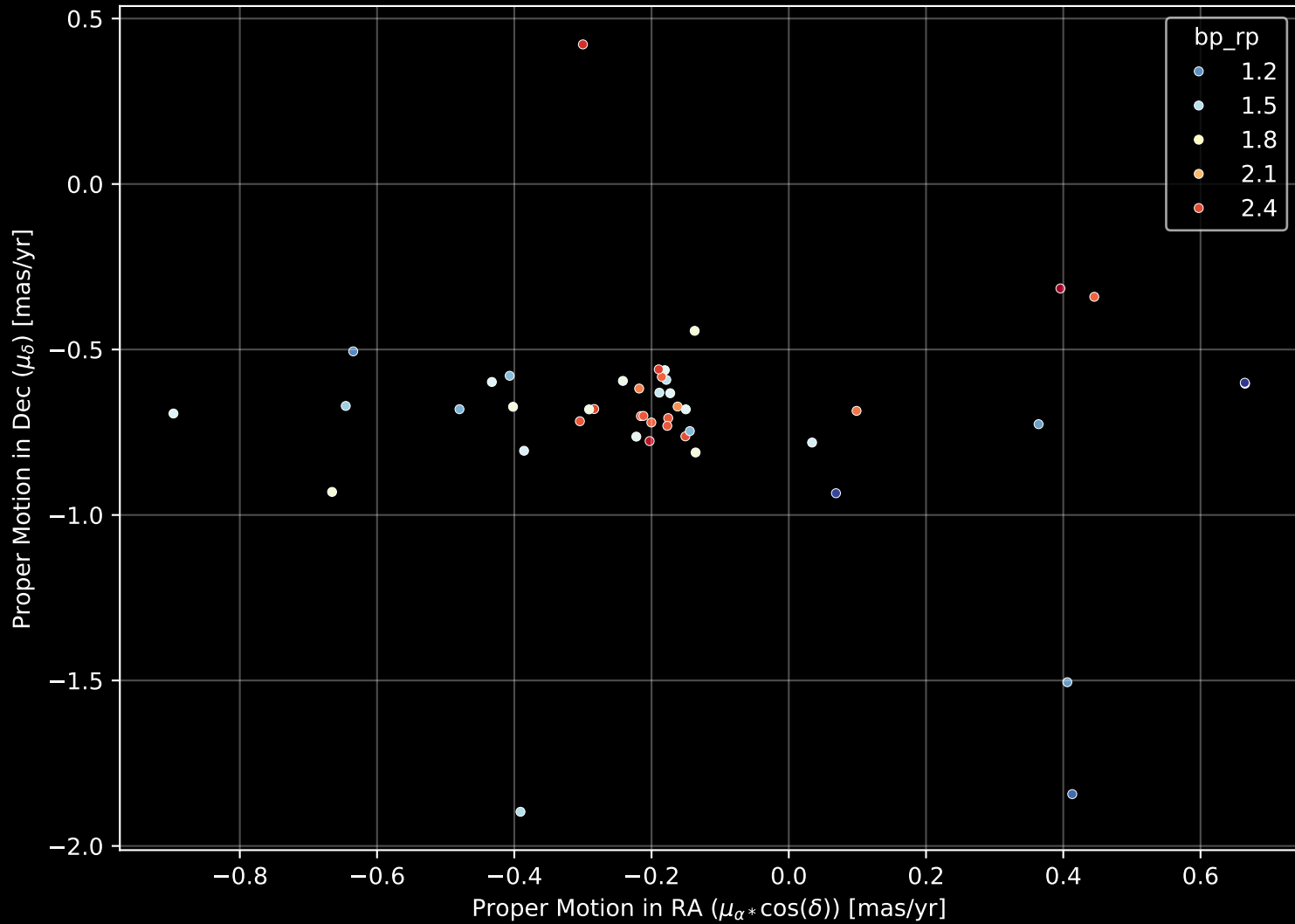
Gaia Cluster: [SAI_17] Proper Motion Diagram (n= 45)
