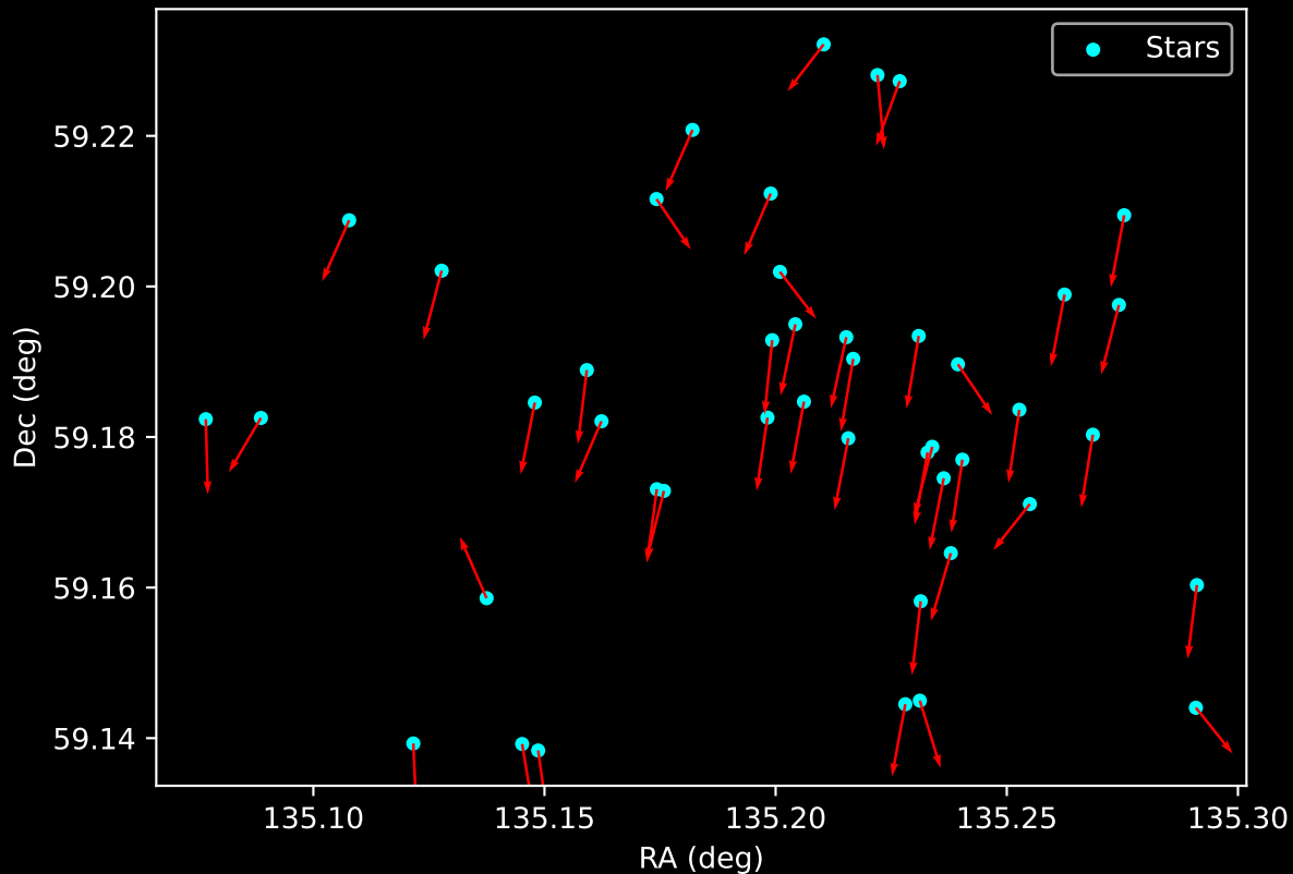
Gaia Cluster: [SAI_17] Proper Motion Vectors for Gaia Star Field (n= 45)
