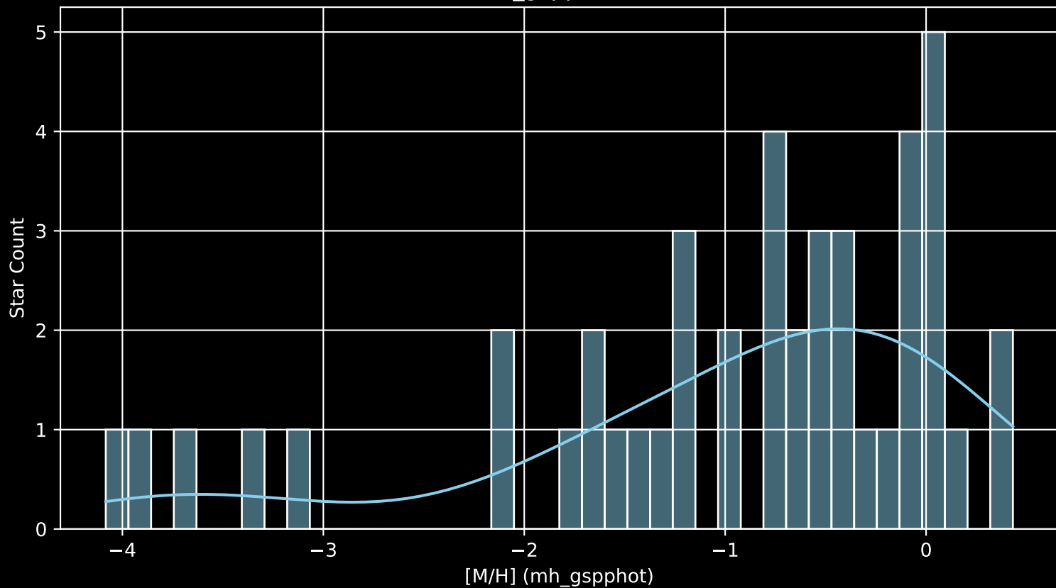
Gaia Cluster: [SAI_17 [M/H] (mh_gspphot) (n= 44)
