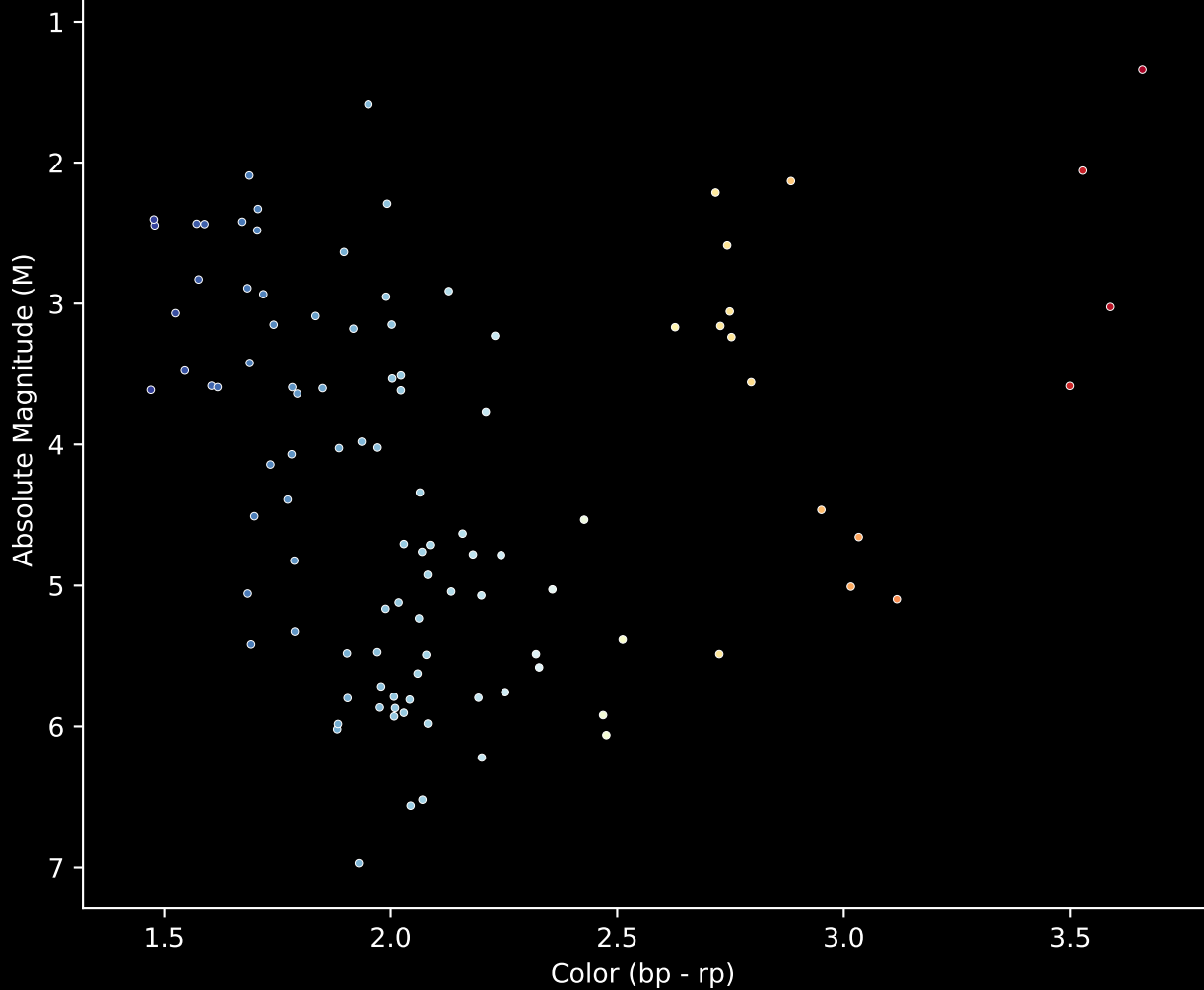
Gaia Cluster: [SAI_25] Stars (n= 105) Hertzsprung-Russel Diagram
