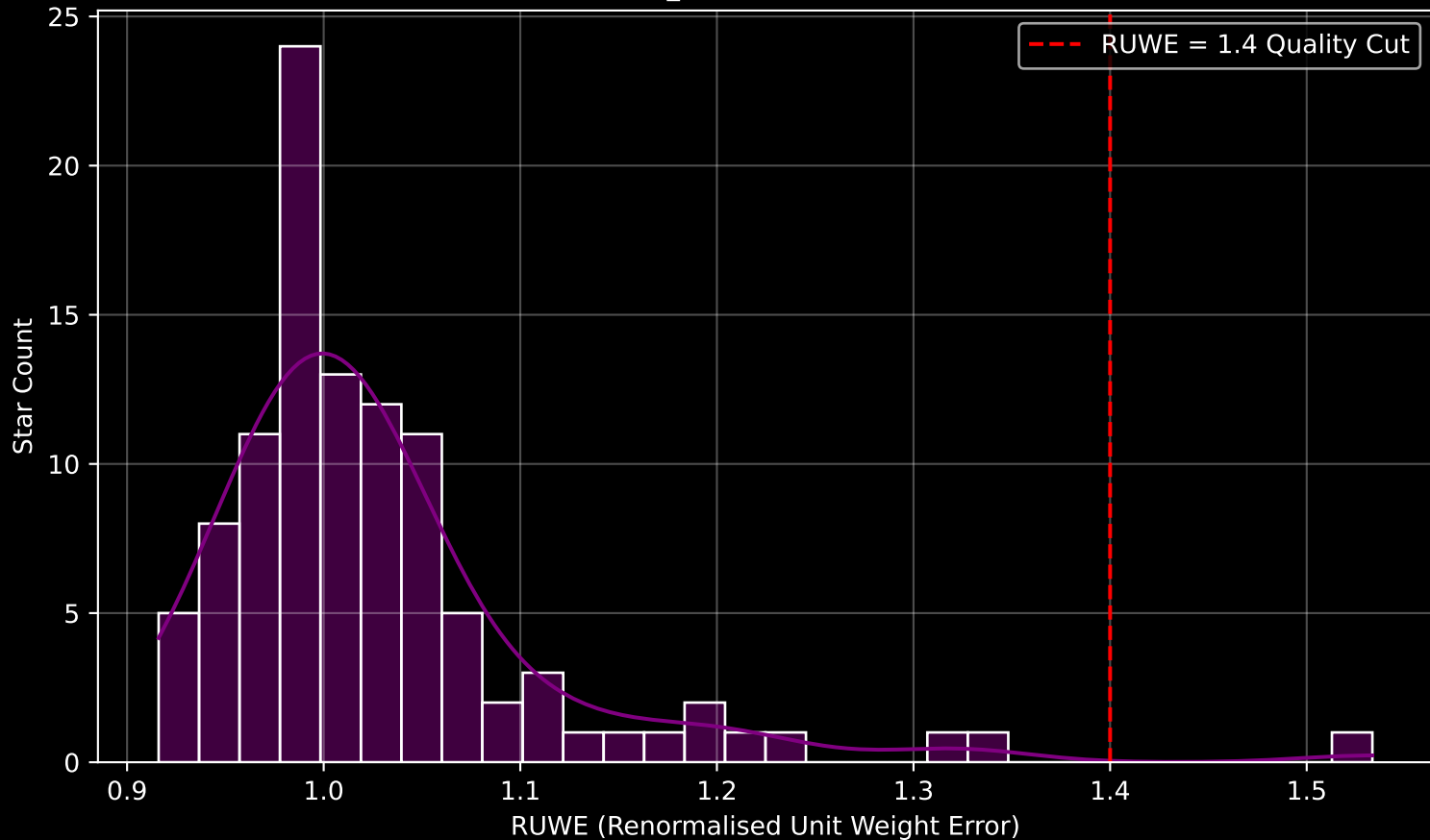
Gaia Cluster: [SAI_25] RUWE Distribution (n= 104)
