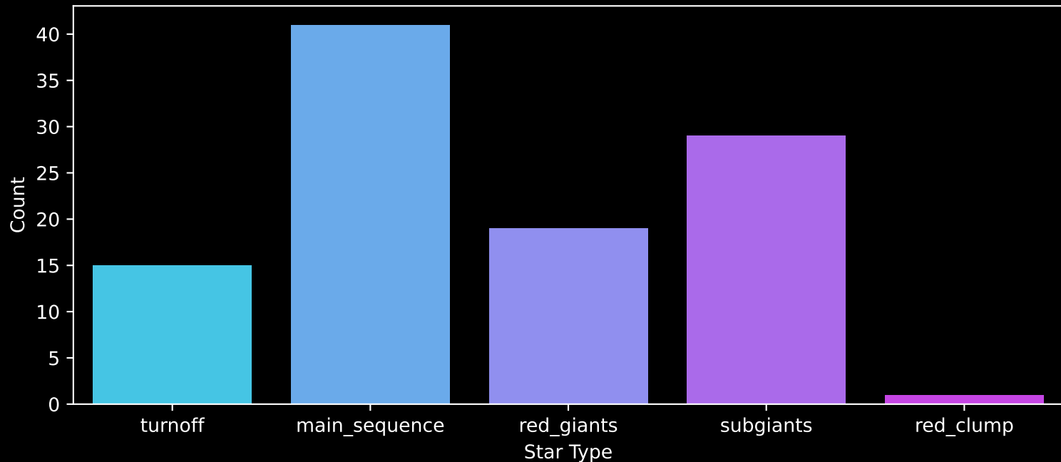
Gaia Cluster: [SAI_25] Count plot of Star Type
