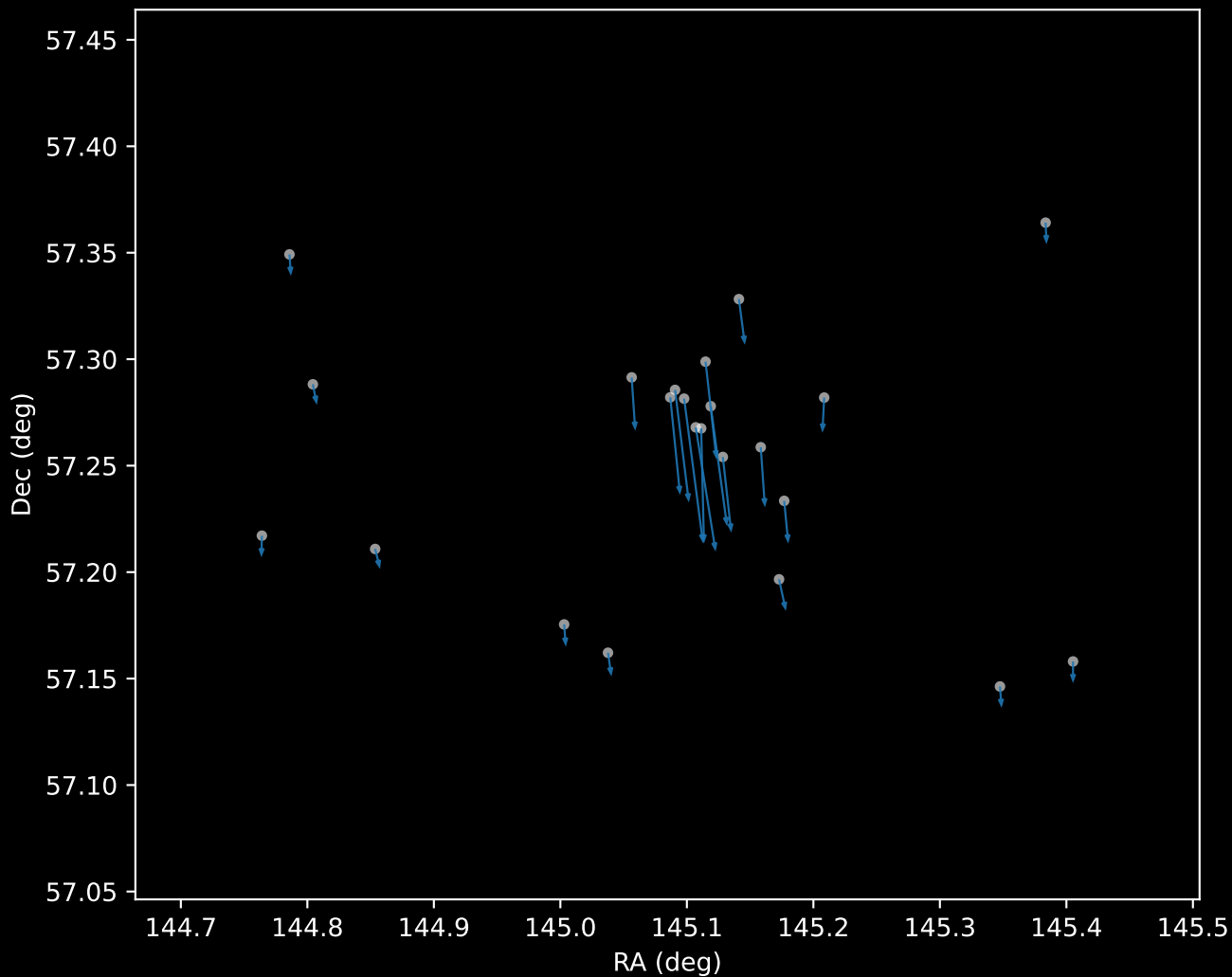
Gaia DR3 Cluster 0 Proper Motion Vectors (n=23)
