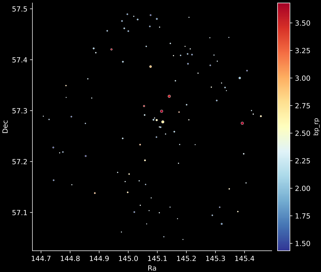
Gaia Cluster: [SAI_25] Stars: 105
