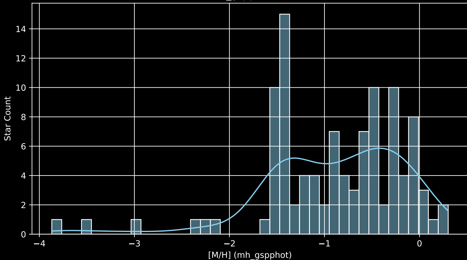
Gaia Cluster: [SAI_25 [M/H] (mh_gspphot) (n= 105)
