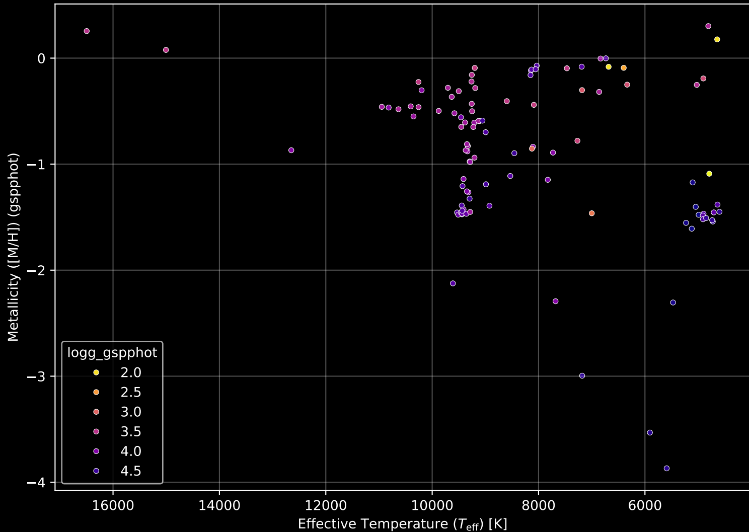
Gaia Cluster: [SAI_25] Stellar Population Parameters (n= 105)
