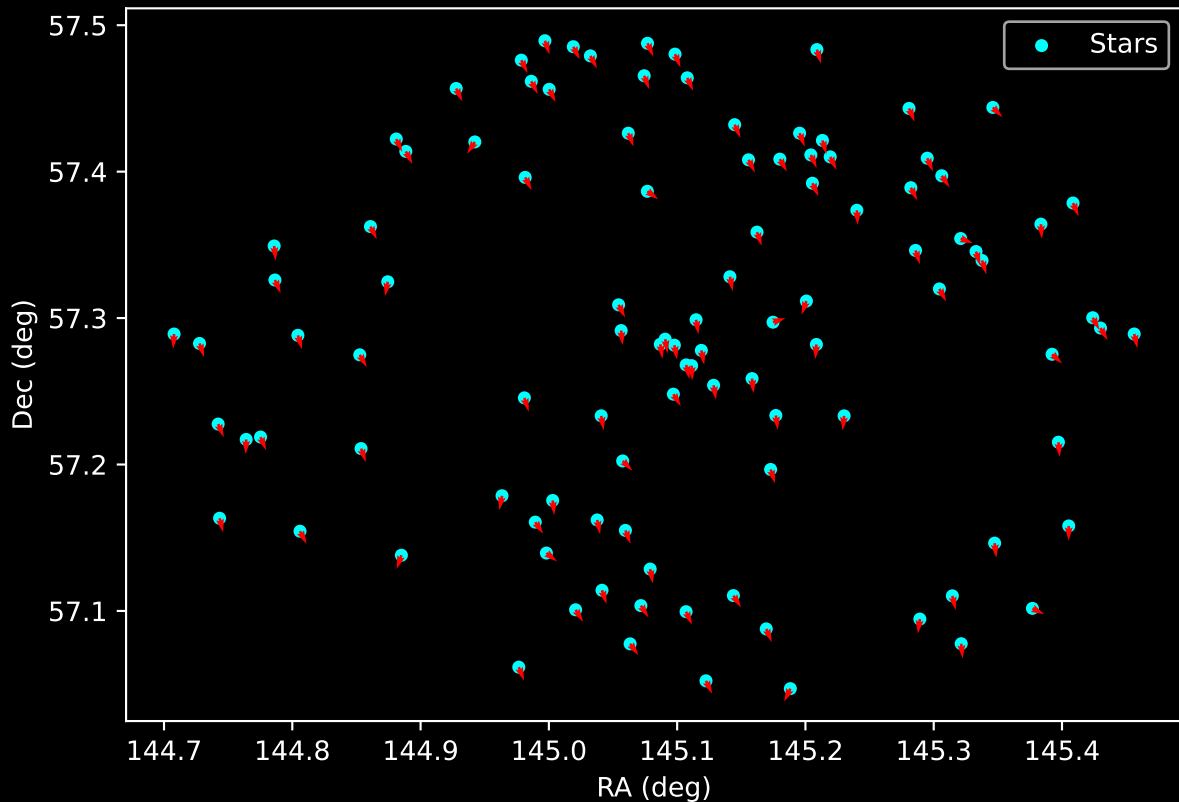
Gaia Cluster: [SAI_25] Proper Motion Vectors for Gaia Star Field (n= 105)
