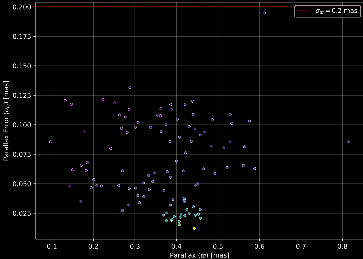
Gaia Cluster: [SAI_25] Parallax Quality (n= 105)
