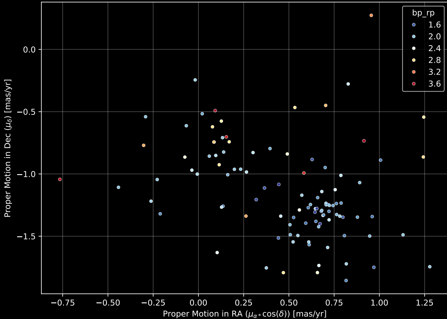
Gaia Cluster: [SAI_25] Proper Motion Diagram (n= 105)
