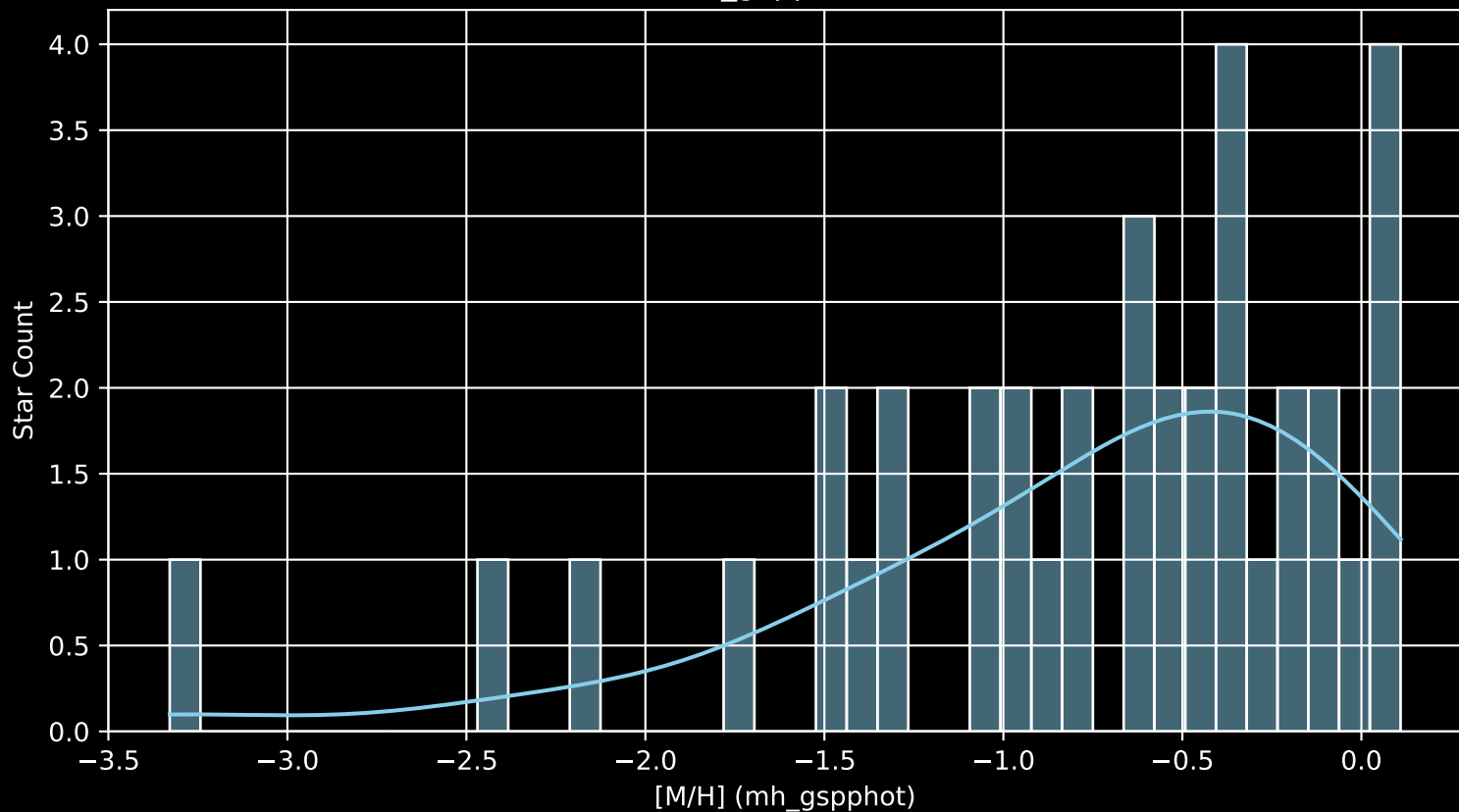
Gaia Cluster: [Saurer_2 [M/H] (mh_gspphot) (n= 37)
