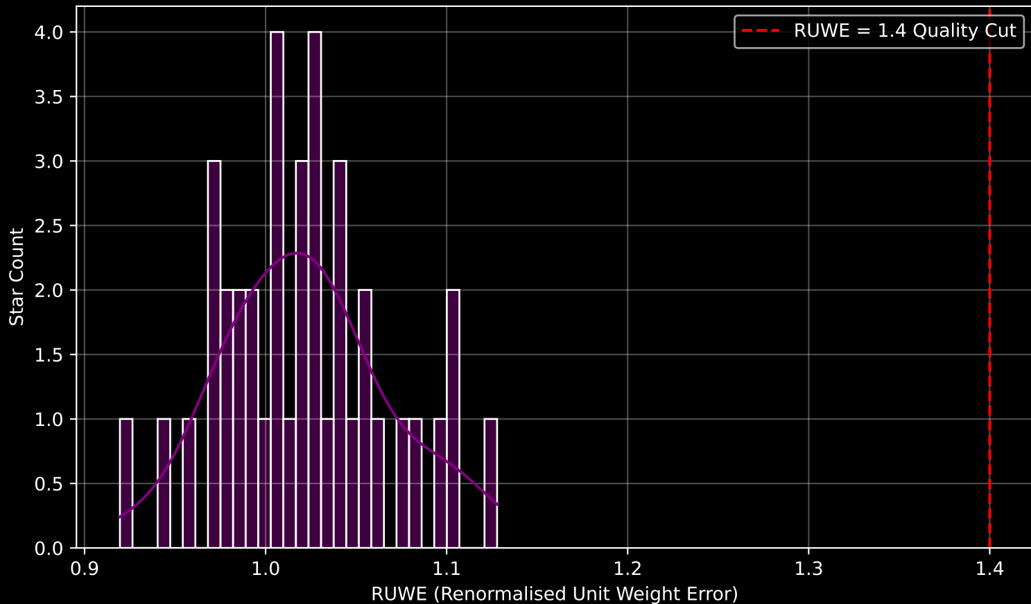
Gaia Cluster: [Saurer_2] RUWE Distribution (n= 39)
