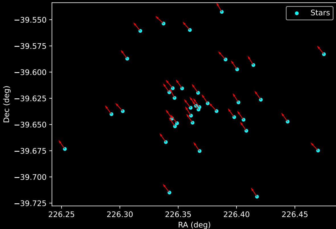
Gaia Cluster: [Saurer_2] Proper Motion Vectors for Gaia Star Field (n= 39)
