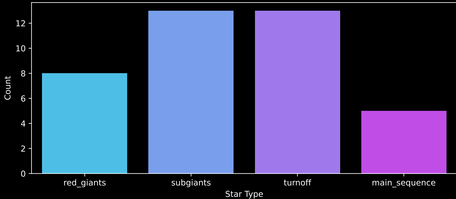
Gaia Cluster: [Saurer_2] Count plot of Star Type
