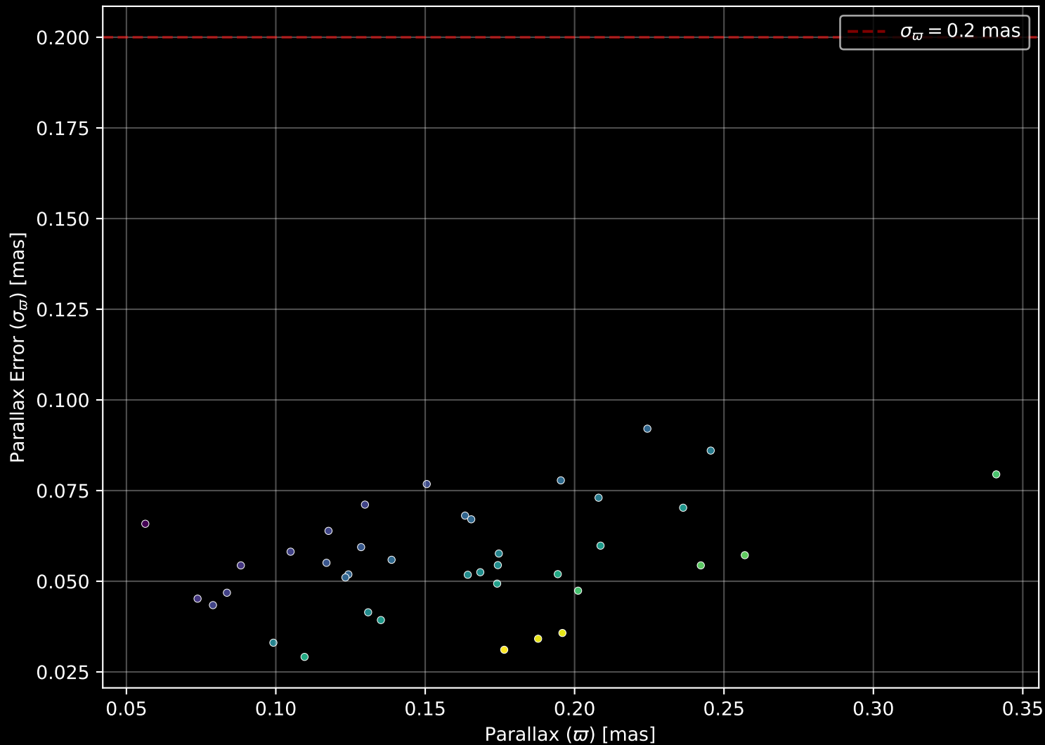
Gaia Cluster: [Saurer_2] Parallax Quality (n= 39)
