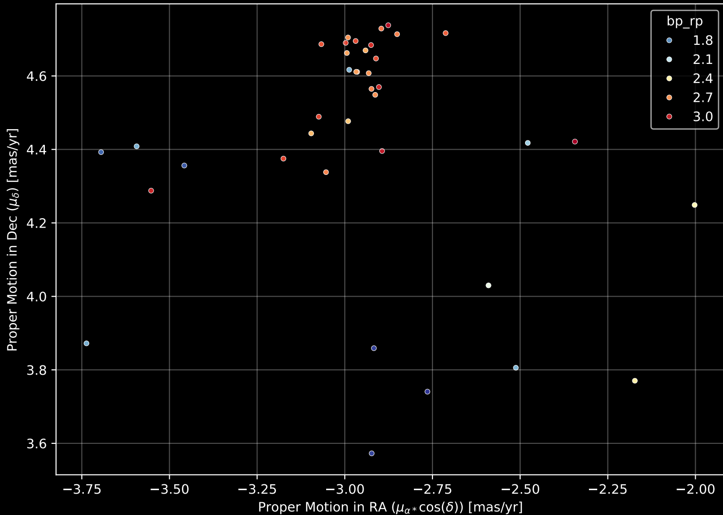
Gaia Cluster: [Saurer_2] Proper Motion Diagram (n= 39)
