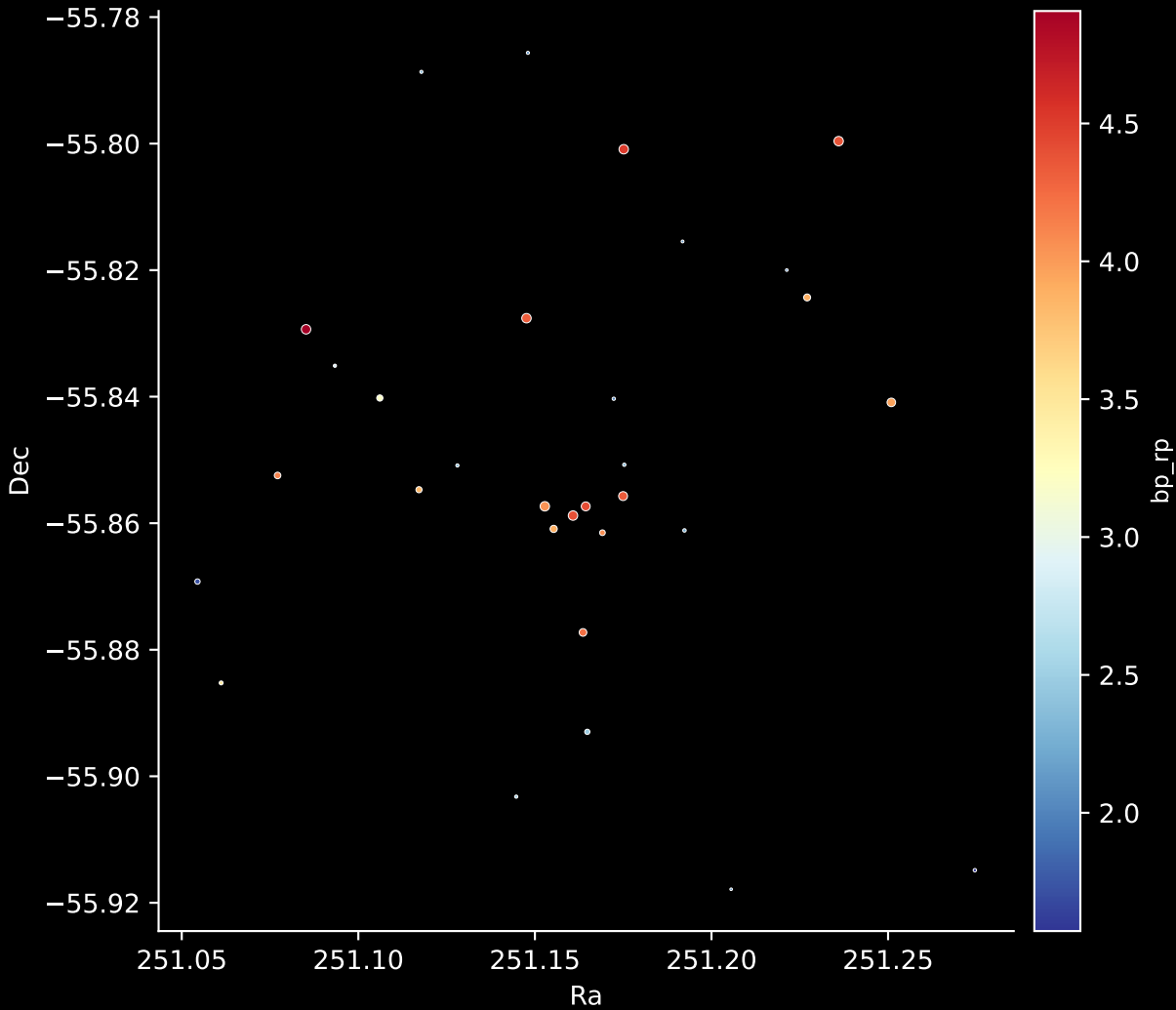
Gaia Cluster: [Schuster_1] Stars: 31
