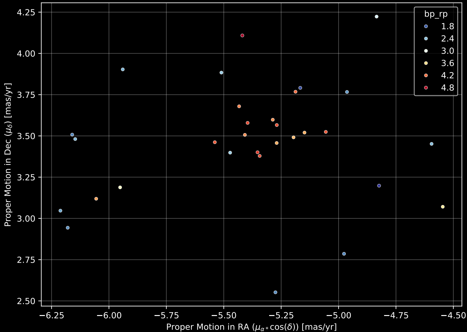
Gaia Cluster: [Schuster_1] Proper Motion Diagram (n= 31)
