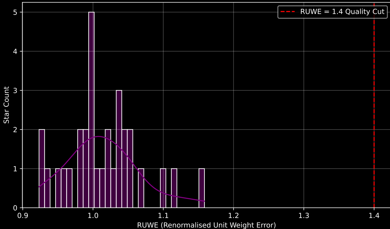
Gaia Cluster: [Schuster_1] RUWE Distribution (n= 31)
