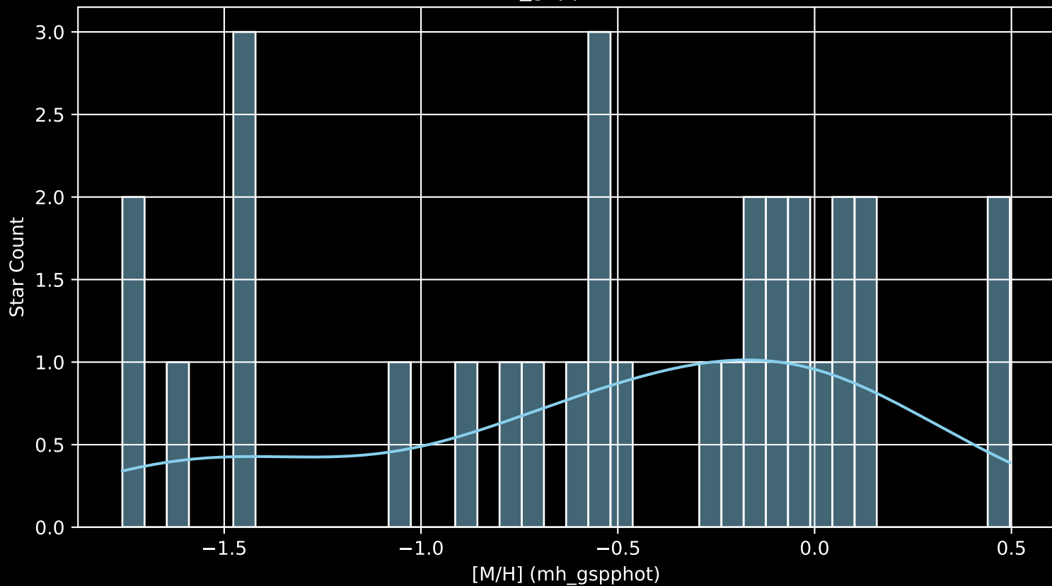
Gaia Cluster: [Schuster_1 [M/H] (mh_gspphot) (n= 30)
