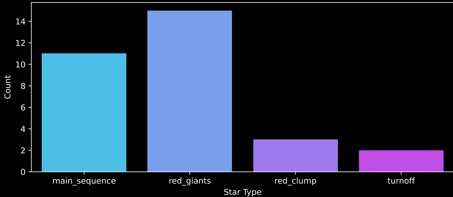
Gaia Cluster: [Schuster_1] Count plot of Star Type
