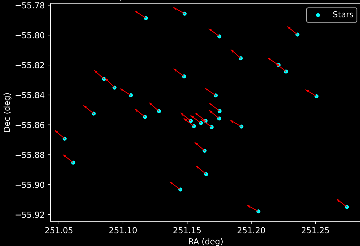
Gaia Cluster: [Schuster_1] Proper Motion Vectors for Gaia Star Field (n= 31)
