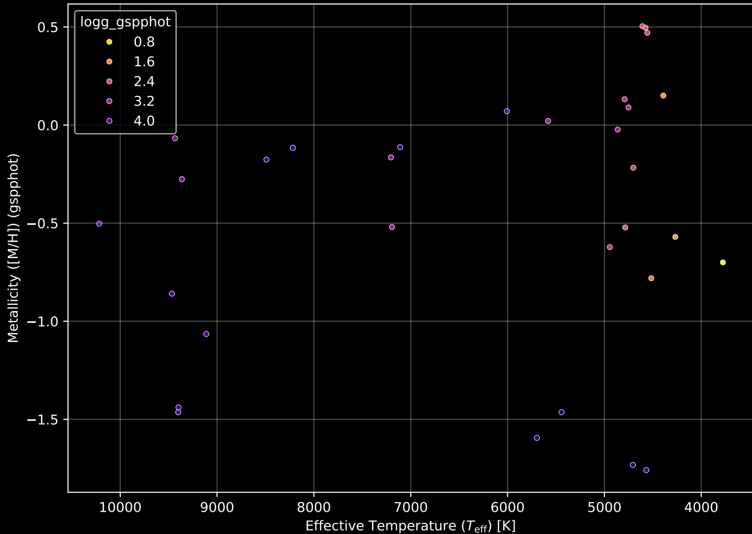
Gaia Cluster: [Schuster_1] Stellar Population Parameters (n= 31)
