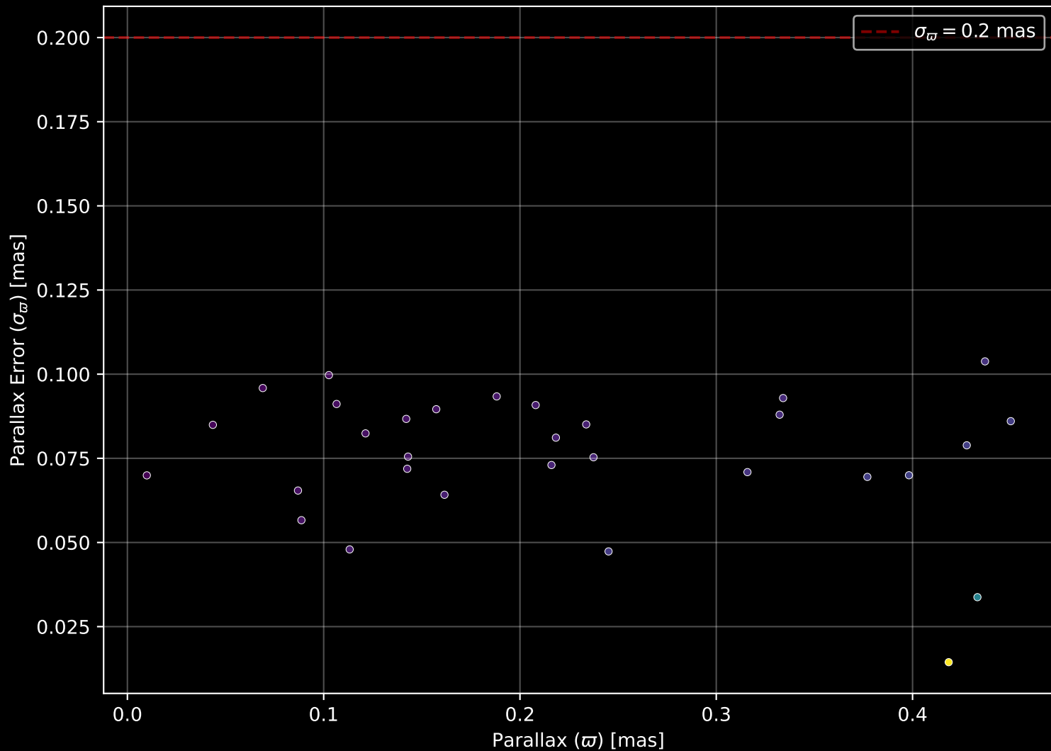
Gaia Cluster: [Schuster_1] Parallax Quality (n= 31)
