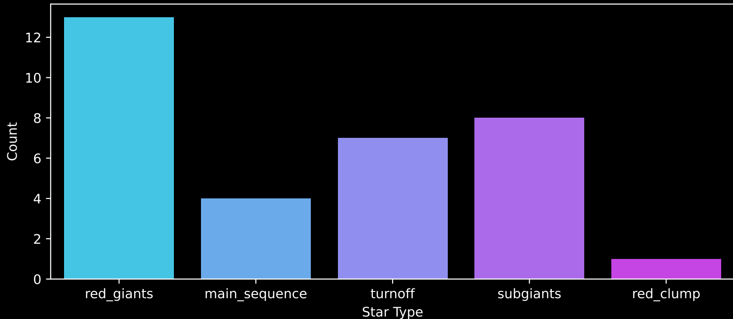
Gaia Cluster: [Sher_1] Count plot of Star Type
