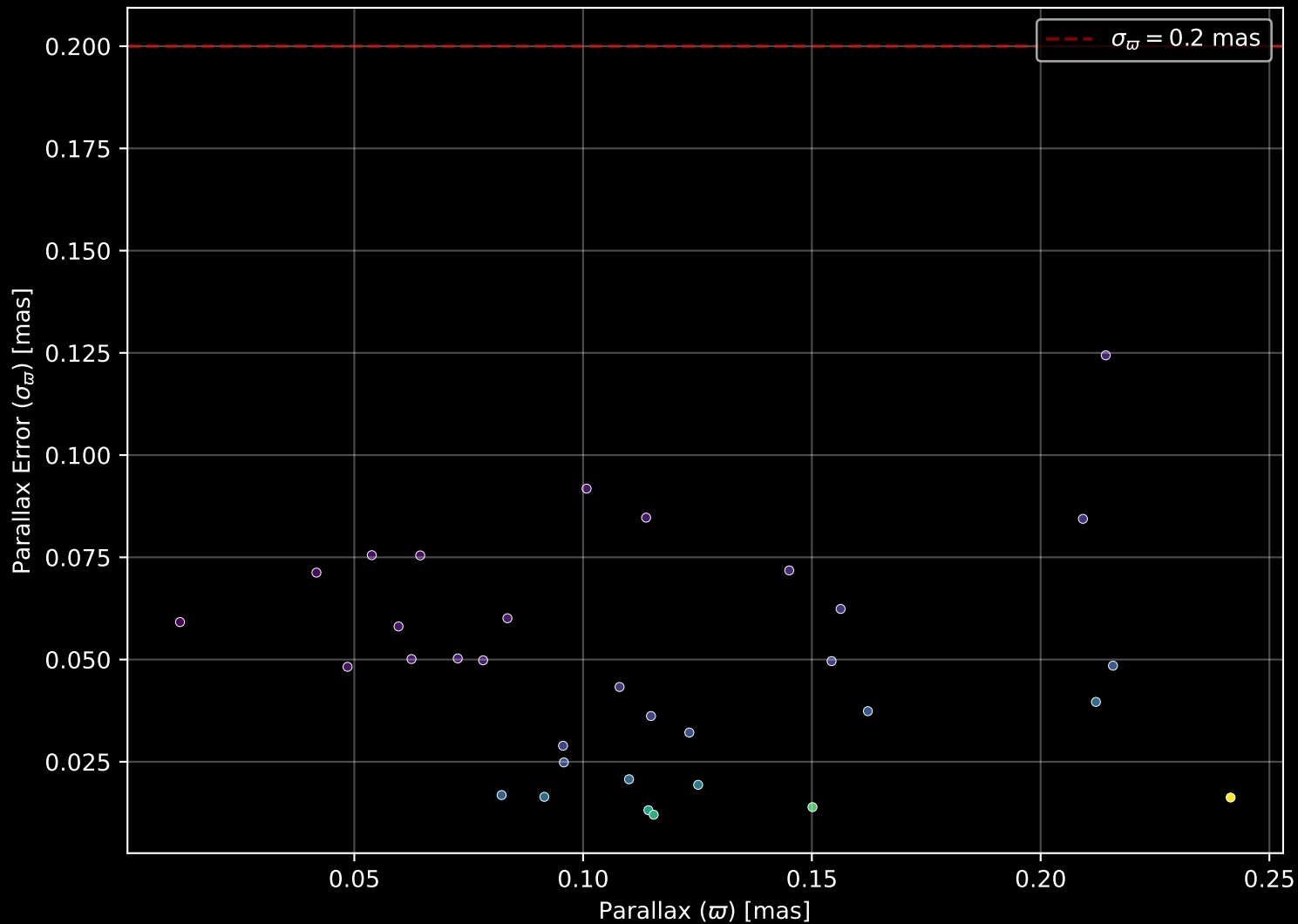
Gaia Cluster: [Sher_1] Parallax Quality (n= 33)
