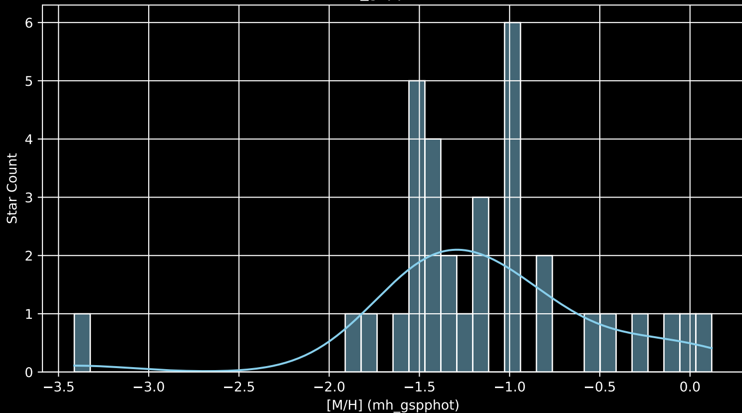
Gaia Cluster: [Sher_1 [M/H] (mh_gspphot) (n= 33)
