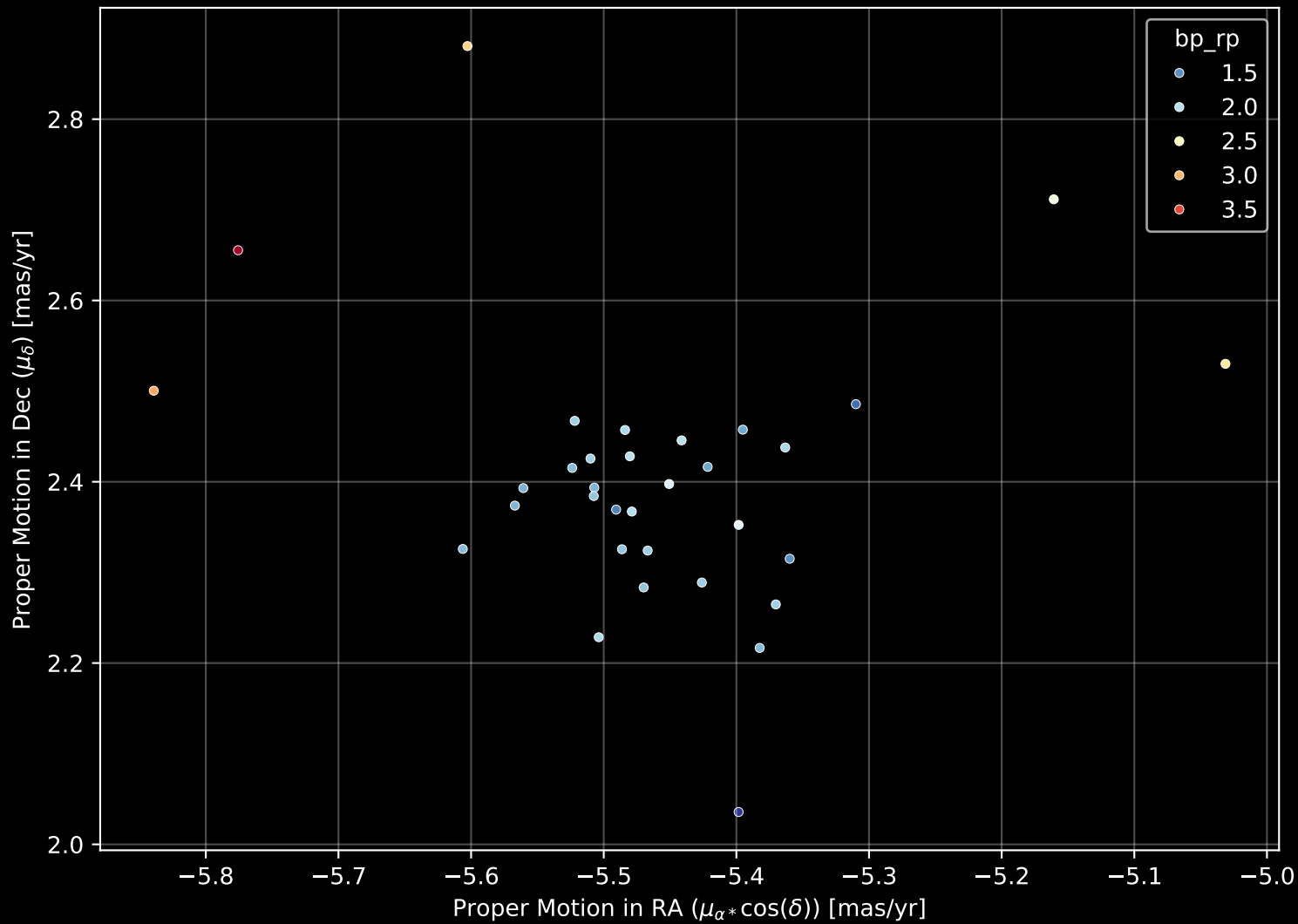
Gaia Cluster: [Sher_1] Proper Motion Diagram (n= 33)
