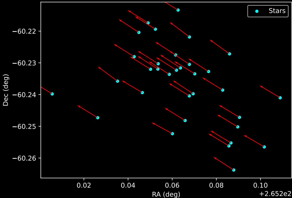
Gaia Cluster: [Sher_1] Proper Motion Vectors for Gaia Star Field (n= 33)
